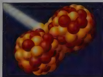
A slow neutron about to split a uranium nucleus.
