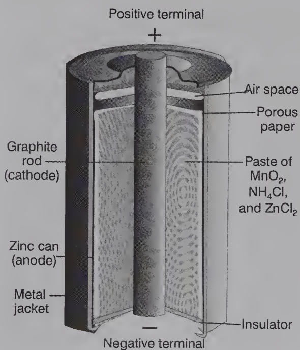
Figure 14.8 Dry Cell Battery (Rae Déjur)
