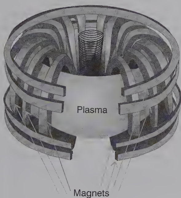
Figure 17.8 Tokamak Design (Rae Déjur)
