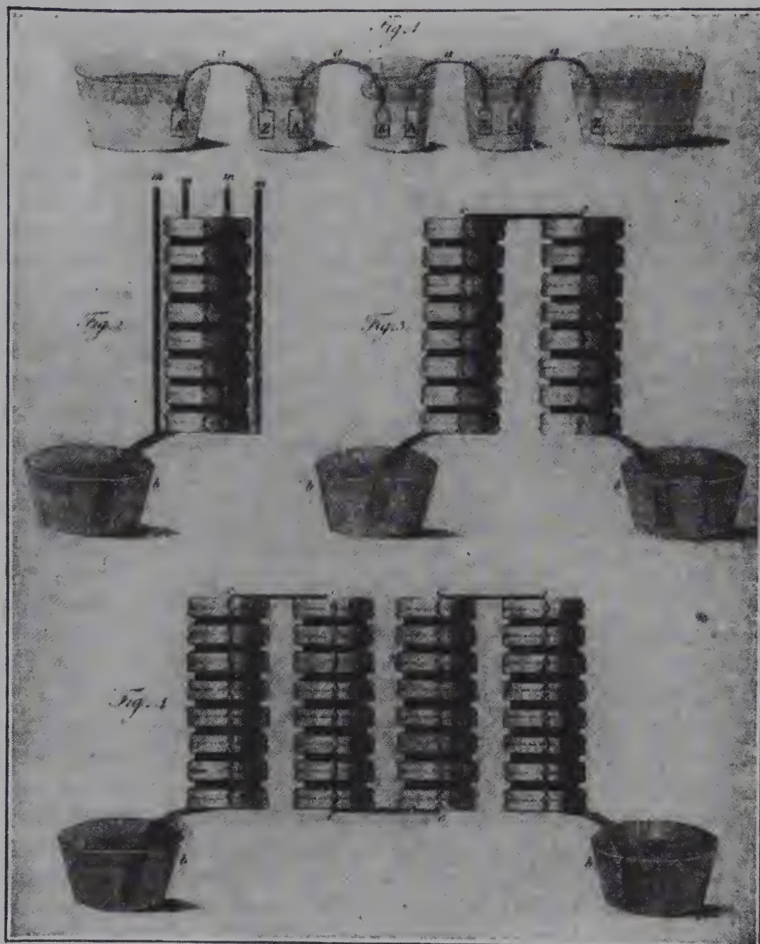
Figure 14.4 Volta's Crown of Cups (top) and Pile
