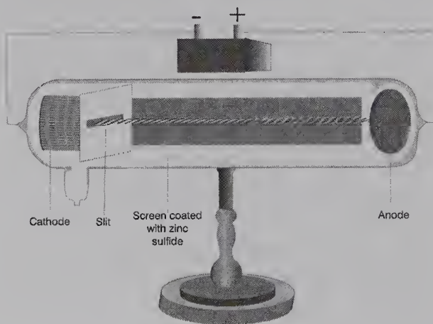
Figure 4.1 Cathode-Ray Tube (Rae Déjur)
