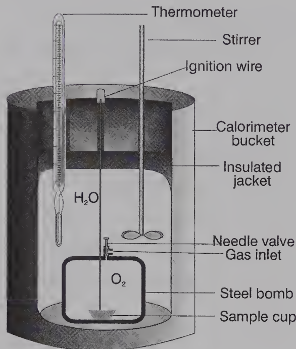
Figure 10.4 Bomb Calorimeter (Rae Déjur)
