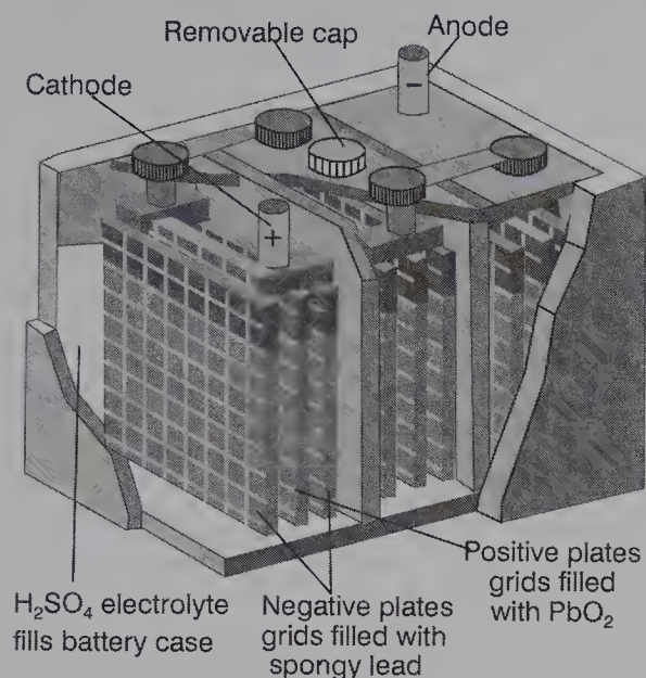
Figure 14.9 Lead Storage Battery (Rae Déjur)
