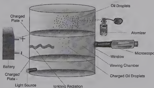
Figure 4.2 Picture of Millikan's Instrument (Rae Déjur)
