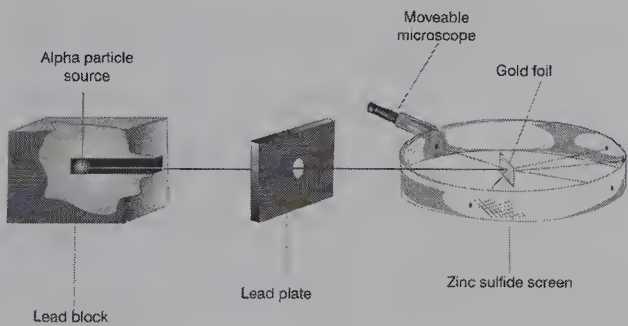
Figure 4.4 Rutherford’s Set-Up (Rae Déjur)
