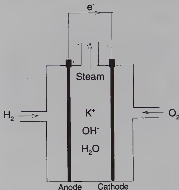
Figure 14.10 Schematic of Hydrogen-Oxygen Fuel Cell
