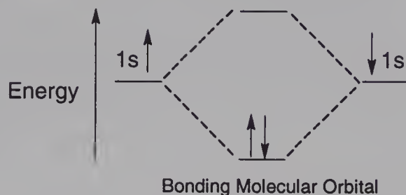
Figure 7.9 Bonding Molecular Orbital Diagram for H_2
