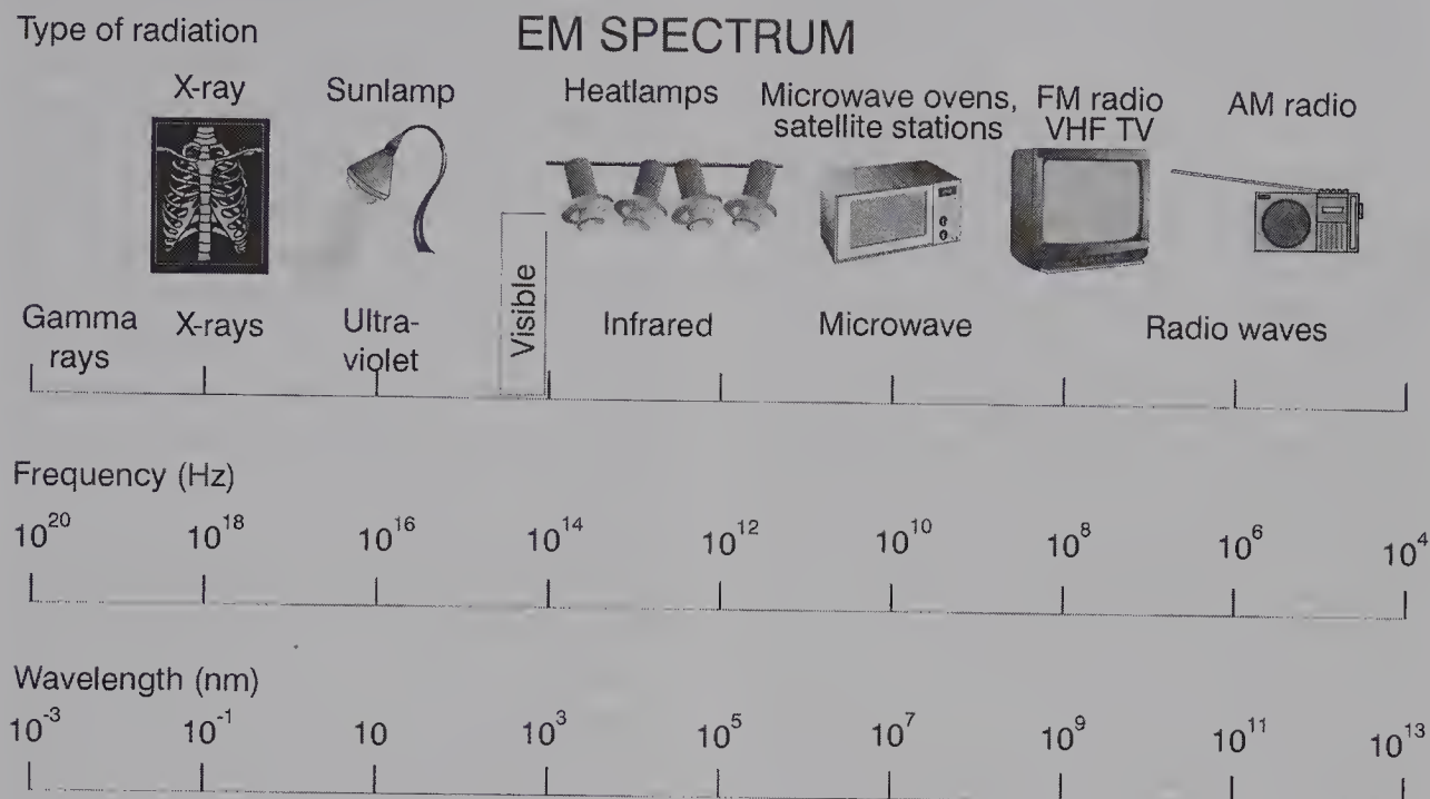
Figure 18.1 The E-M Spectrum (Rae Déjur)
