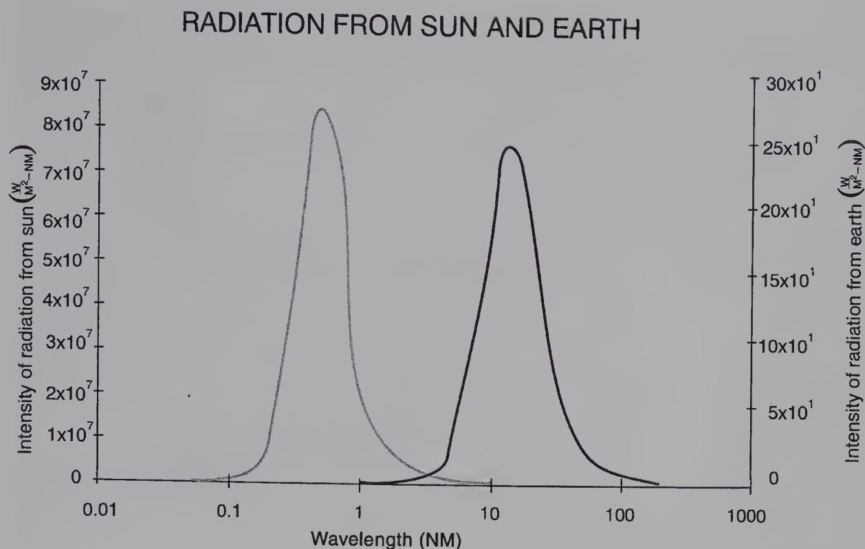
Figure 18.2 Peaks of Solar and Earth Radiation (Rae Déjur)
