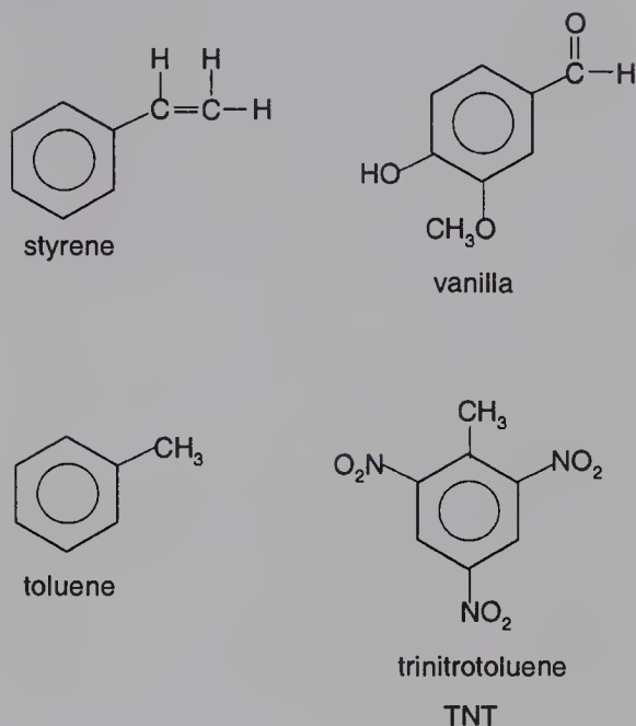
Figure 15.6 Several Common Benzene Derivatives
