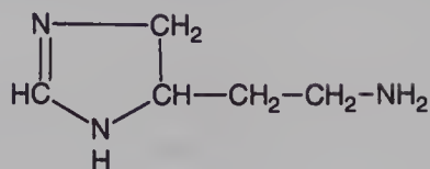
Figure 15.20 Histamine
