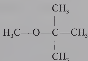
MTBE
