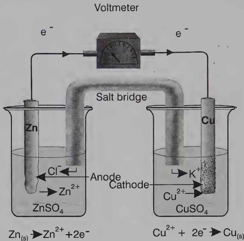
Figure 14.5 Daniell Cell (Rae Déjur)
