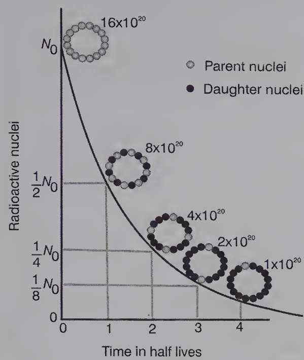
Figure 17.3 Exponential Decay (Rae Déjur)
