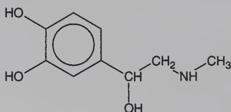
Figure 15.21 Adrenaline
