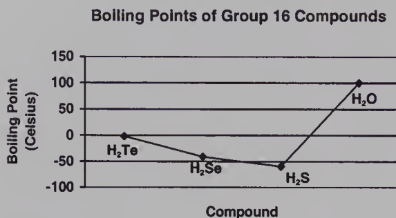
Figure 8.3 Trend in Boiling of Several Group 16 Compounds
