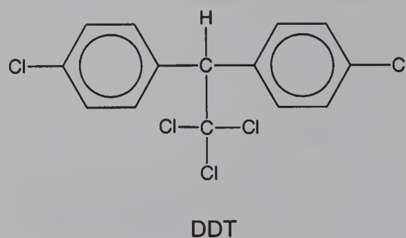
Figure 18.6 DDT
