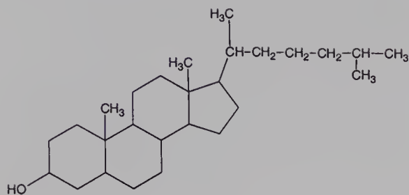
Figure 16.8 Cholesterol
