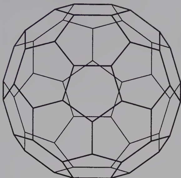
Figure 8.14 Buckminsterfullerene
