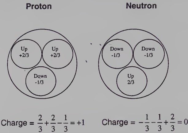
Figure 4.8 Structure of Protons and Neutrons
