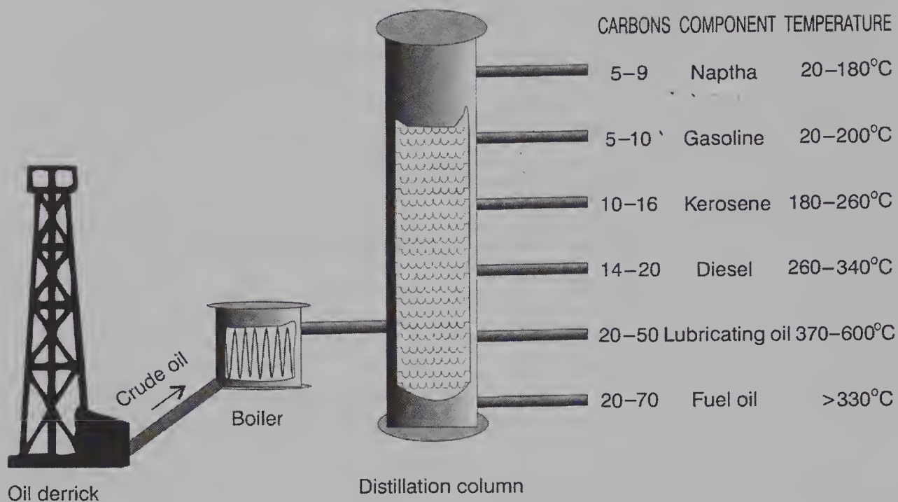
Figure 15.22 Fractionating Column for Oil (Rae Déjur)
