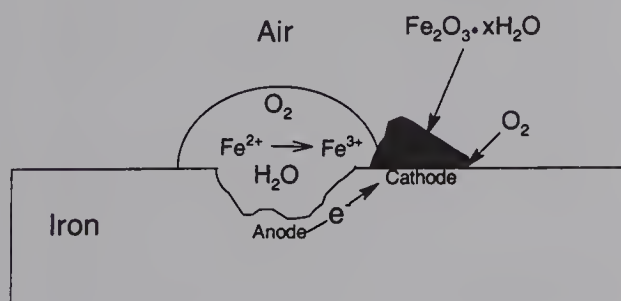
Figure 14.11 The formation of rust involves an electrochemical reaction taking place between two different regions in the metal.
