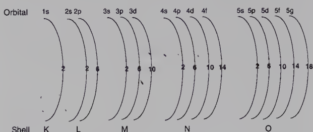
Figure 4.7 Maximum Numbers of Electrons per Orbital
