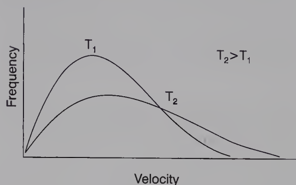
Figure 9.5 Boltzmann Curves at Higher and Lower Temperatures (Rae Déjur)
