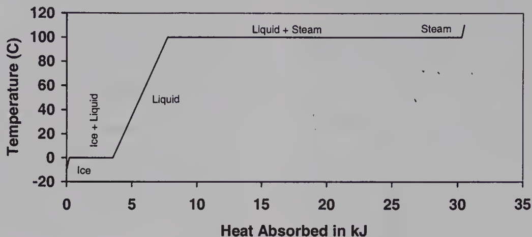
Figure 10.2 The Heating Curve for Water
