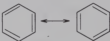
Figure 15.5 Kekulé proposed that the structure for benzene resonated between two alternate structures in which the position of the double and single bonds switched positions.
