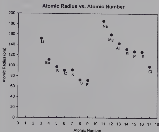
Figure 6.4 Change in Atomic Radii for Periods 2 and 3
