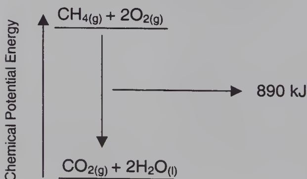
Figure 10.5 Energy involved in the combustion of methane, \text{CH}_4 . In the combustion process, the chemical potential energy of the reactants is higher than the products. The difference in potential energy is the heat involved in the reaction
