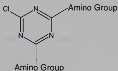
Triazine Structure
