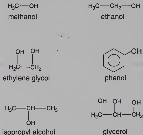
Figure 15.8 Some Common Alcohols
