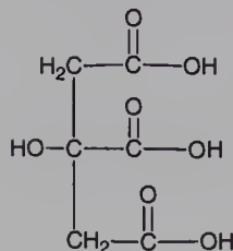
citric acid
