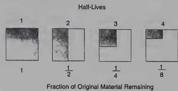
Figure 17.4 The amount of a radioactive substance is cut in half after each consecutive half-life. The amount of the original material remaining after n half-lives is (\frac{1}{2})^n .
