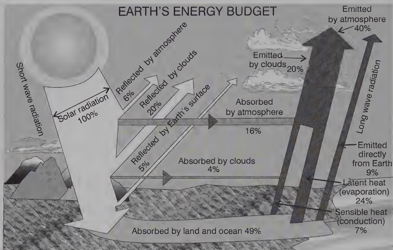
Figure 18.3 Earth's Radiation Budget (Rae Déjur)
