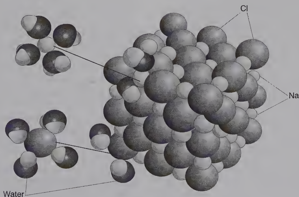
Figure 11.1 Diagram of Hydration of NaCl (Rae Déjur)
