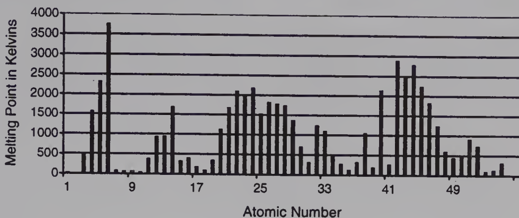
Figure 6.2 Periodic Trend of Melting Point
