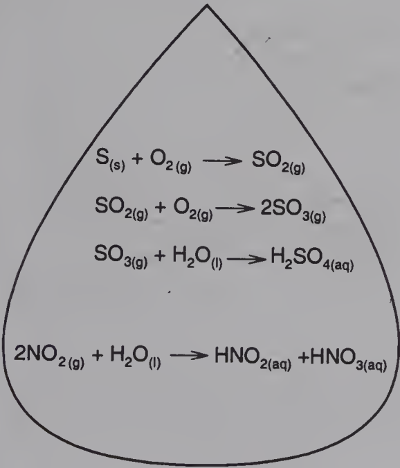
Figure 13.2 Acid rain occurs when reactions in the atmosphere lead to the formation of various acids lowering the pH below the natural pH of rain, which is approximately 5.5. The acidic pH of natural rain water is due to the formation of carbonic acid by the reaction: CO 2(g) + H 2 O → H 2 CO 3 .
