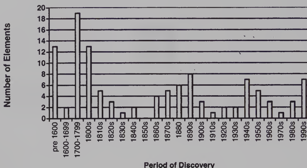
Figure 6.1 Discovery Dates of the Elements
