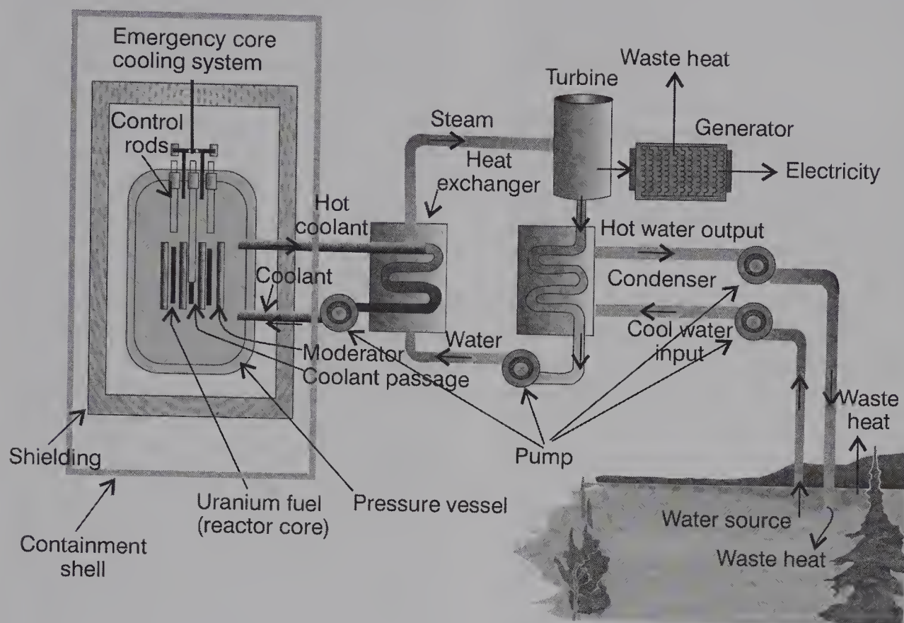
Figure 17.7 Schematic of Nuclear Power Plant (Rae Déjur)
