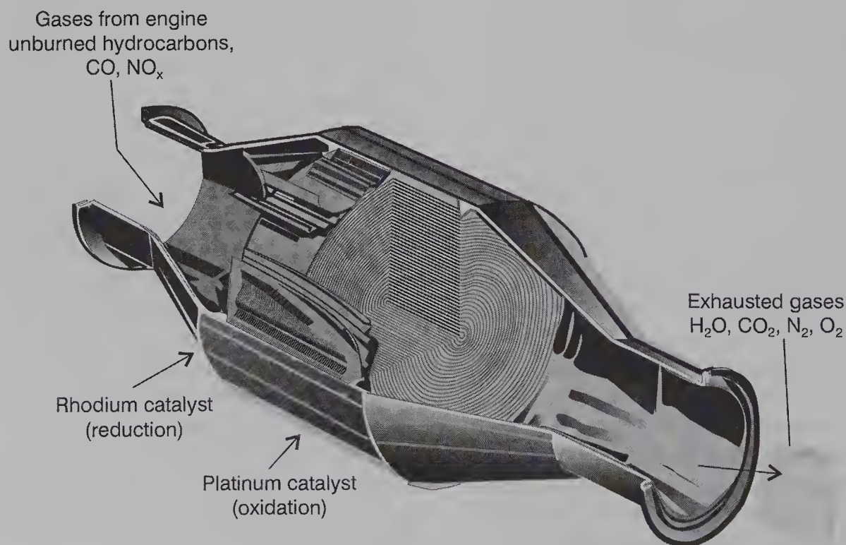
Figure 12.4 Catalytic Converter (Rae Déjur)
