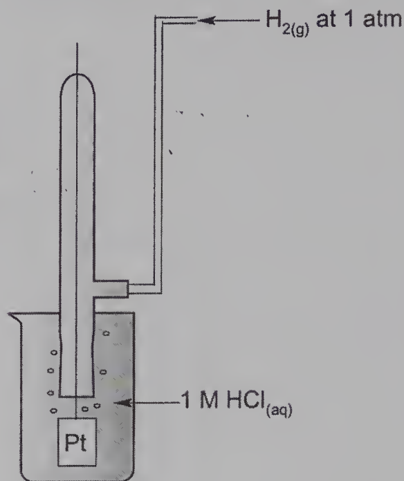
Figure 14.6 Standard Hydrogen Electrode (SHE)
