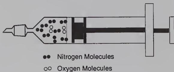
Figure 9.3 Pushing in on the plunger decreases the volume, which causes an increase in pressure due to the collision frequency increasing
