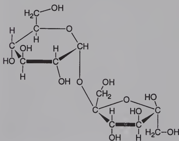
Figure 16.5 Common table sugar, sucrose, is a disaccharide composed of a hexose form of glucose bonded to a pentose form of fructose.
