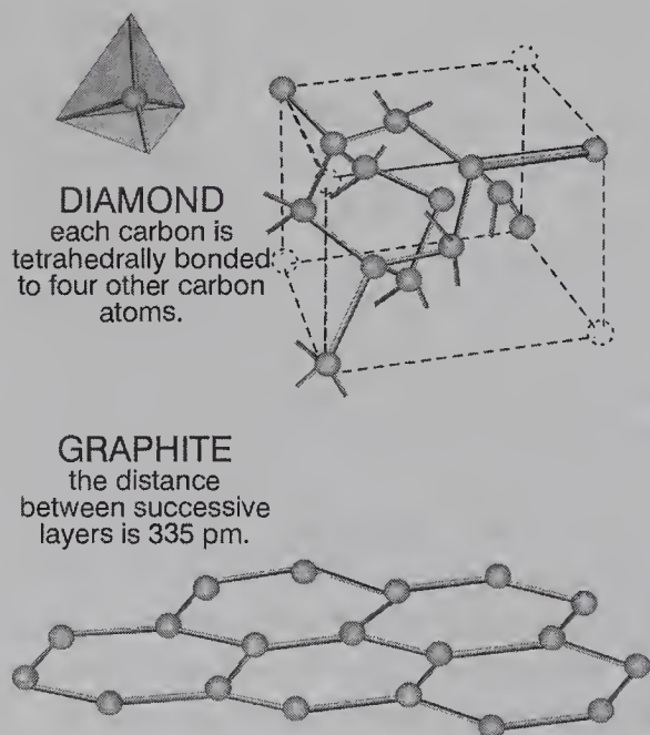
Figure 1.1 Diamond and Graphite Structure (Rae Déjur)
