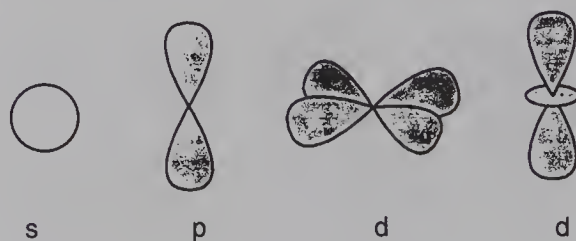
Figure 4.6 Representation of Several Different Orbitals
