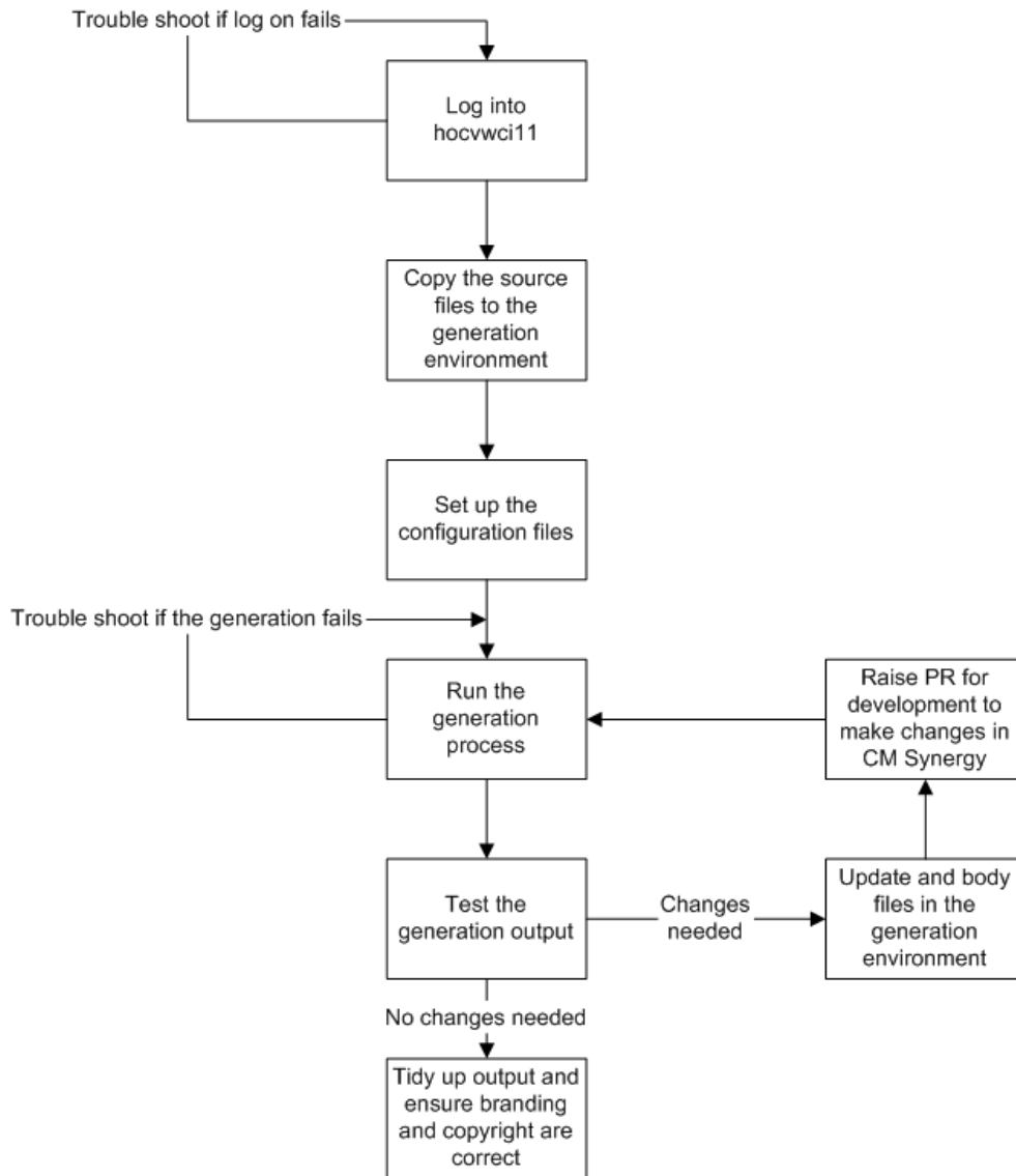
Figure 1: Flow Diagram for the Stored Procedures Generation Process
