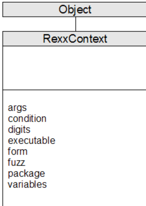
Figure 5-46. The REXXContext class and methods
