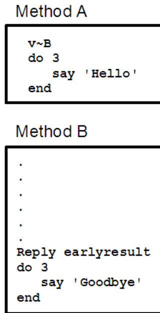
Figure 12-2. Before REPLY
