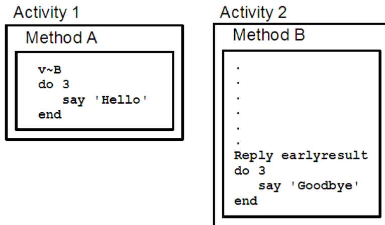
Figure 12-3. After REPLY
