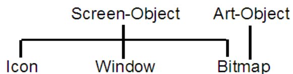
Figure 1-10. Multiple Inheritance
