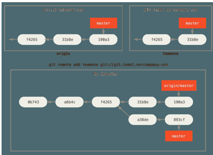
Figure 33. Adding another server as a remote
