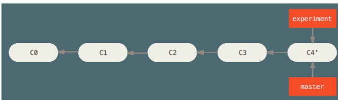
Figure 38. Fast-forwarding the master branch
