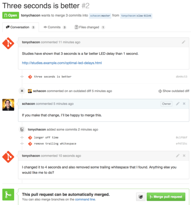
Figure 96. Pull Request final
