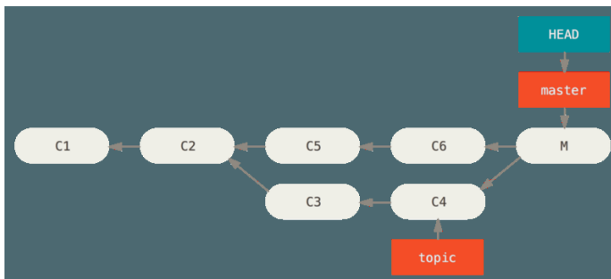
Figure 138. Accidental merge commit
