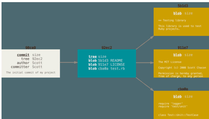
Figure 9. A commit and its tree
