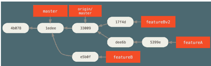
Figure 72. Commit history after featureBv2 work.
