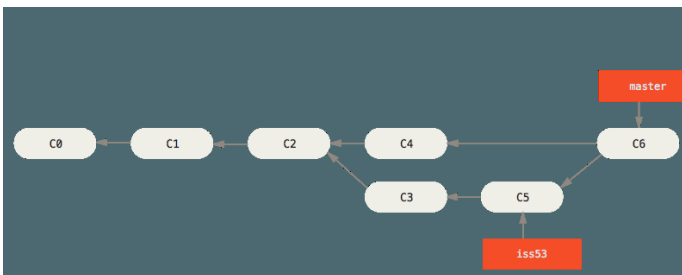
Figure 25. A merge commit
