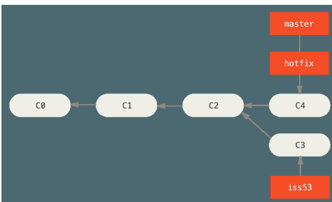
Figure 22. master is fast-forwarded to hotfix
