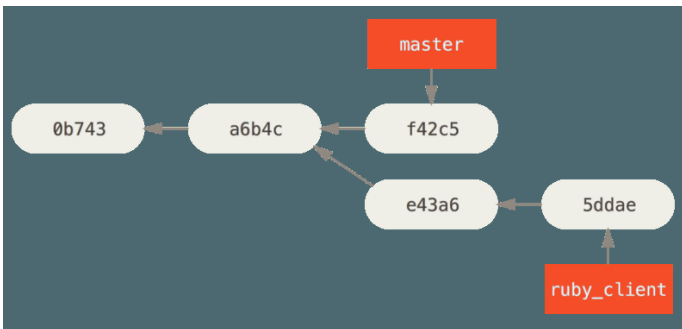
Figure 80. Example history before a cherry-pick.
