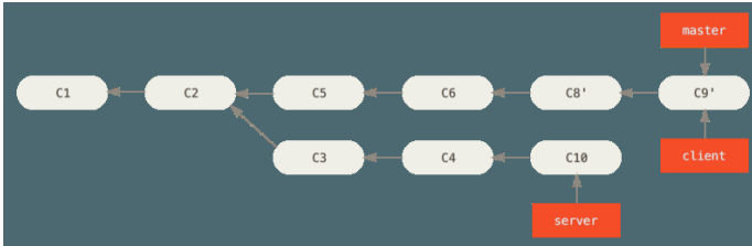
Figure 41. Fast-forwarding your master branch to include the client branch changes
