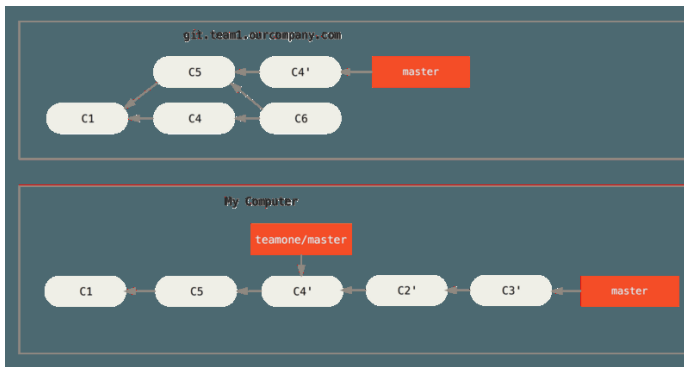
Figure 48. Rebase on top of force-pushed rebase work.
