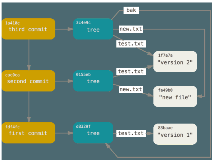
Figure 151. All the reachable objects in your Git directory.
