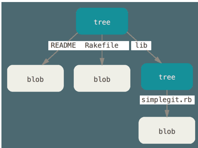
Figure 149. Simple version of the Git data model.
