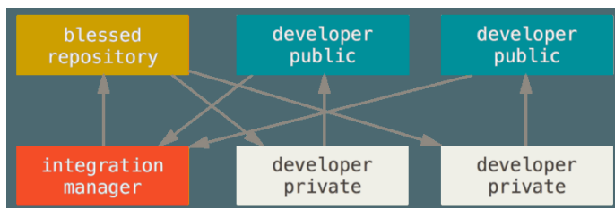
Figure 55. Integration-manager workflow.
