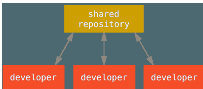
Figure 54. Centralized workflow.
