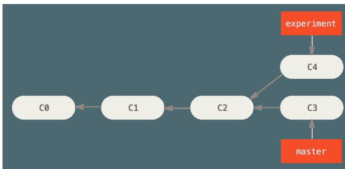
Figure 35. Simple divergent history
