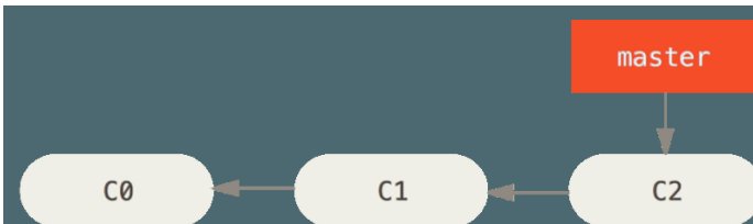
Figure 18. A simple commit history
