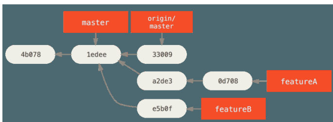
Figure 70. Initial commit history with featureB work.
