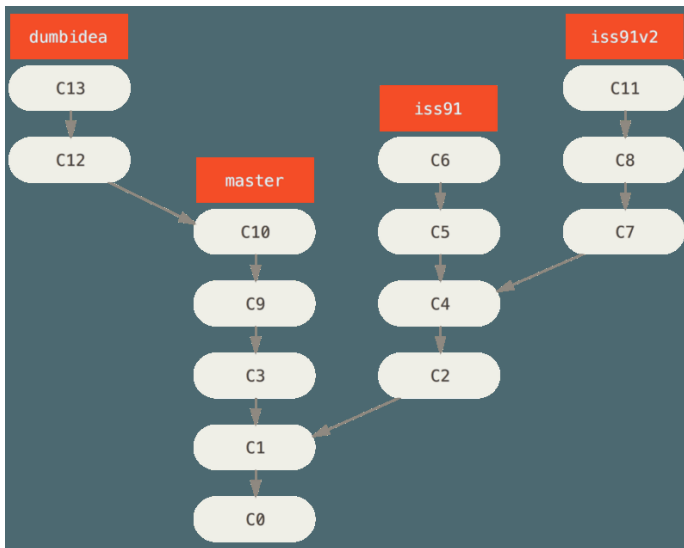
Figure 28. Multiple topic branches
