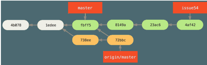
Figure 62. Jessica's history after fetching John's changes.
