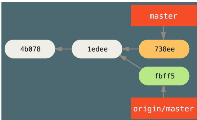
Figure 58. John's divergent history.
