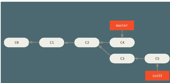
Figure 23. Work continues on iss53
