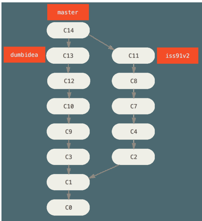
Figure 29. History after merging dumbidea and iss91v2
