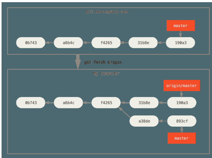
Figure 32. git fetch updates your remote references
