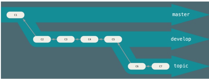
Figure 27. A “silo” view of progressive-stability branching
