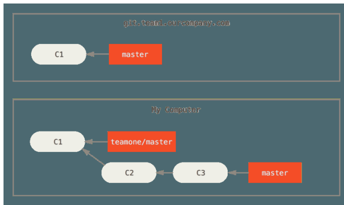
Figure 44. Clone a repository, and base some work on it
