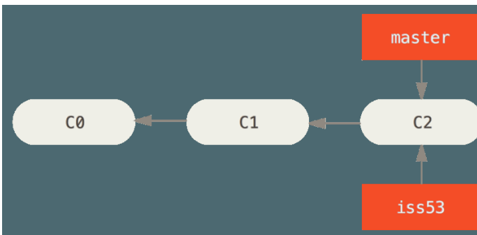
Figure 19. Creating a new branch pointer
