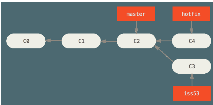
Figure 21. Hotfix branch based on master
