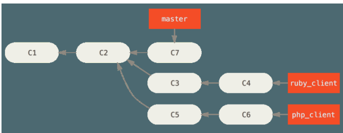
Figure 73. History with several topic branches.
