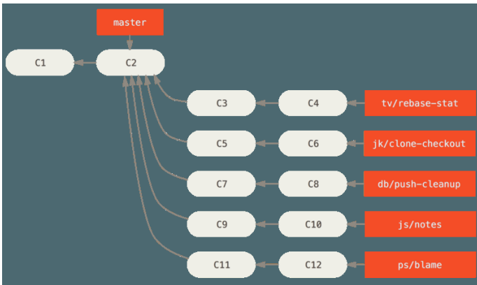
Figure 78. Managing a complex series of parallel contributed topic branches.
