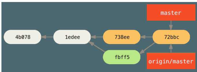
Figure 60. John's history after pushing to the origin server.
