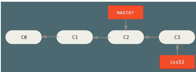
Figure 20. The iss53 branch has moved forward with your work
