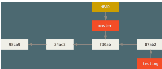
Figure 16. HEAD moves when you checkout
