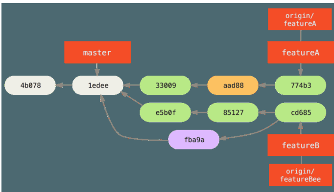
Figure 67. Jessica's history after committing on a feature branch.
