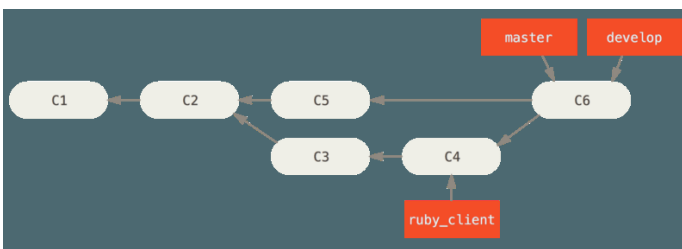
Figure 77. After a project release.
