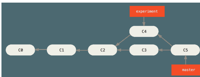
Figure 36. Merging to integrate diverged work history
