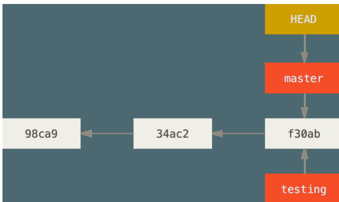
Figure 13. HEAD pointing to a branch
