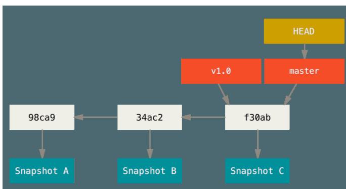
Figure 11. A branch and its commit history
