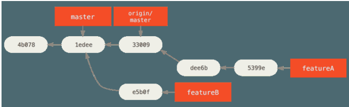
Figure 71. Commit history after featureA work.
