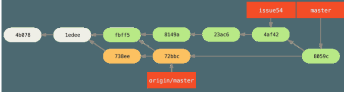
Figure 63. Jessica’s history after merging John’s changes.
