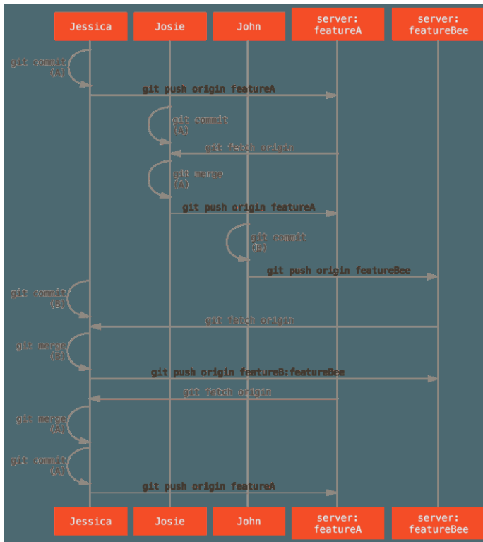
Figure 69. Basic sequence of this managed-team workflow.
