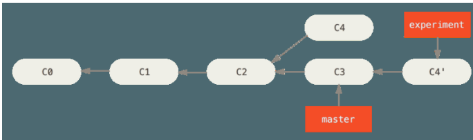
Figure 37. Rebasing the change introduced in C4 onto C3
