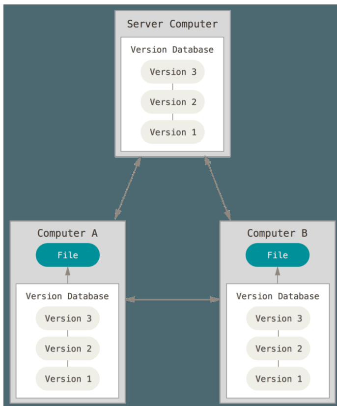
Figure 3. Distributed version control.
