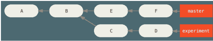
Figure 137. Example history for range selection.
