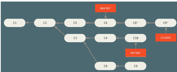
Figure 40. Rebasing a topic branch off another topic branch
