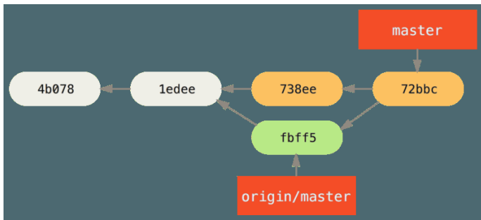
Figure 59. John's repository after merging origin/master .
