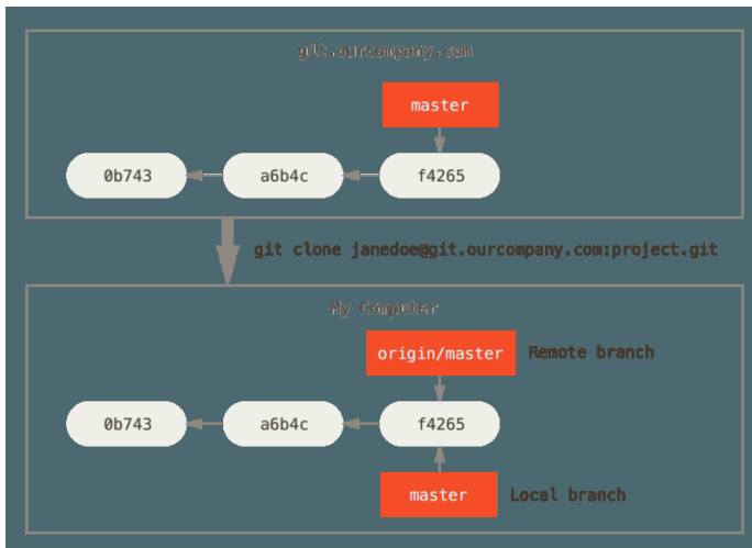
Figure 30. Server and local repositories after cloning
