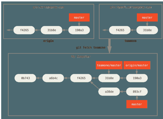
Figure 34. Remote tracking branch for teamone/master
