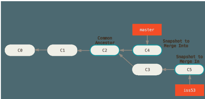
Figure 24. Three snapshots used in a typical merge
