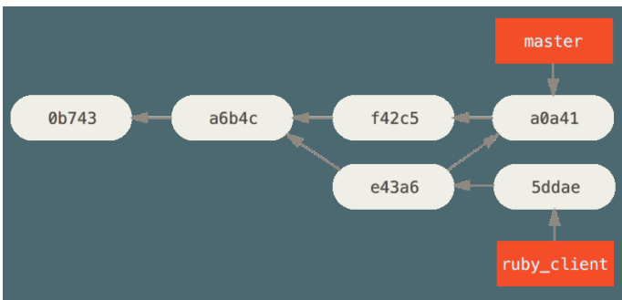
Figure 81. History after cherry-picking a commit on a topic branch.
