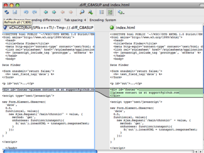
Figure 143. P4Merge.
