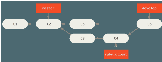
Figure 76. After a topic branch merge.
