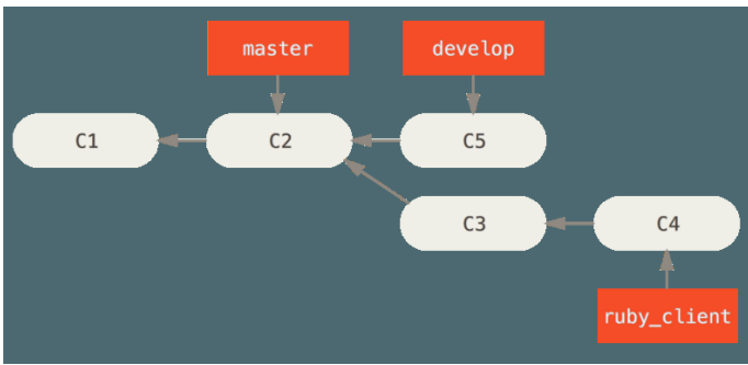
Figure 75. Before a topic branch merge.
