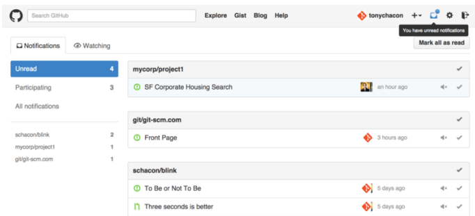
Figure 122. Notification center.
