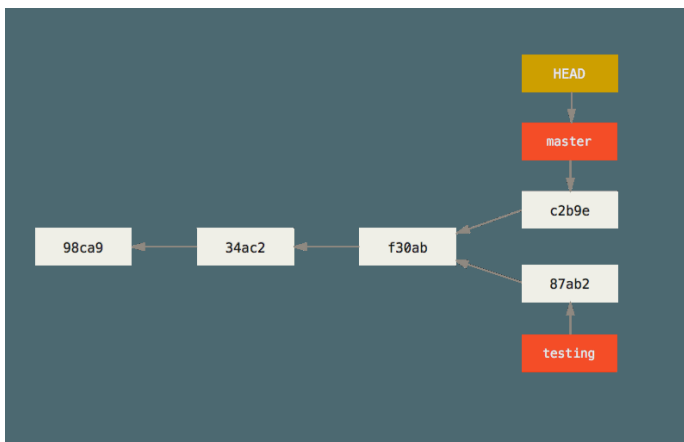
Figure 17. Divergent history
