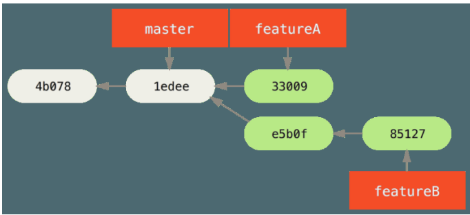
Figure 66. Jessica's initial commit history.
