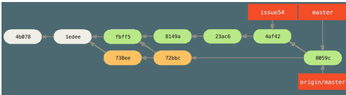
Figure 64. Jessica’s history after pushing all changes back to the server.
