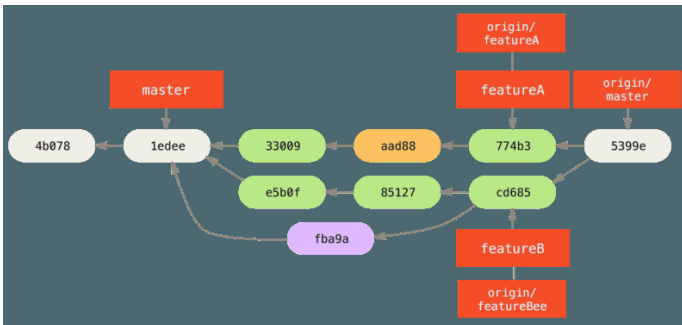
Figure 68. Jessica's history after merging both her topic branches.
