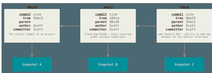
Figure 10. Commits and their parents
