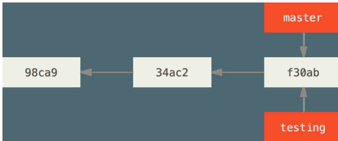
Figure 12. Two branches pointing into the same series of commits
