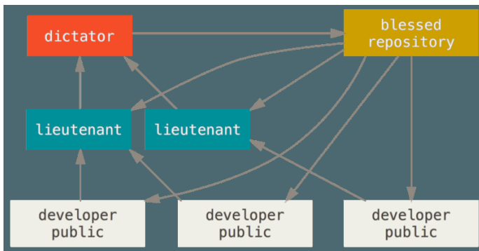
Figure 56. Benevolent dictator workflow.
