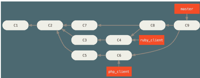
Figure 74. After a topic branch merge.
