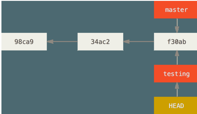
Figure 14. HEAD points to the current branch
