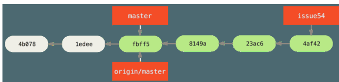
Figure 61. Jessica's topic branch.
