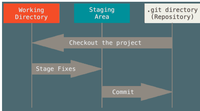
Figure 6. Working tree, staging area, and Git directory.
