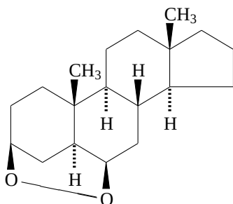
3β,6β-epidioxy-5α-androstane
