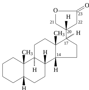
5β-cardanolide
