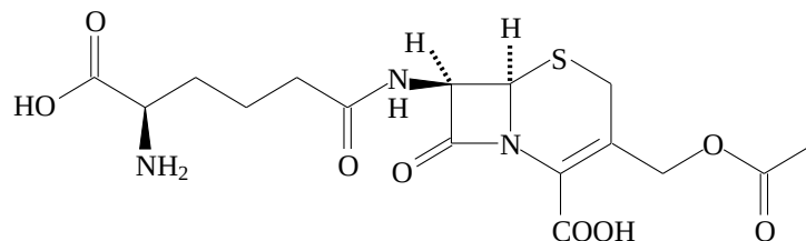
3-57 (cephalosporin C)
