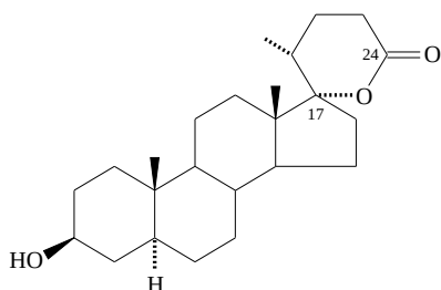
3 \beta -hydroxy-5 \alpha -cholano-24,17-lactone
