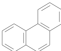
2-28 \phenanthrenev{}
