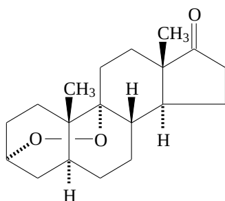
3α,9-epidioxy-5α-androstan-17-one
