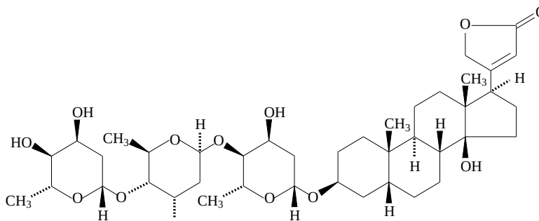
digitoxin
