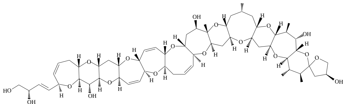
31-40 (Ciguatoxin 1B)
