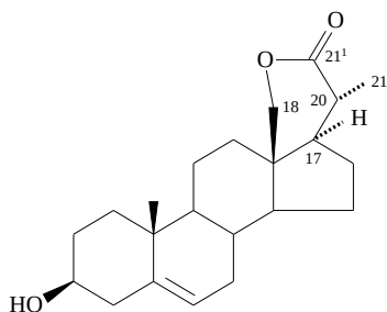
(20 R )-3β-hydroxypregn-5-ene-20,18-carbolactone
