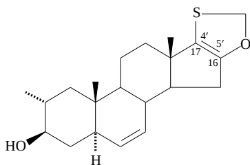
2 \alpha -methyl[1,3]oxathiol[5',4':16,17]-5 \alpha -androst-6-en-3 \beta -ol
