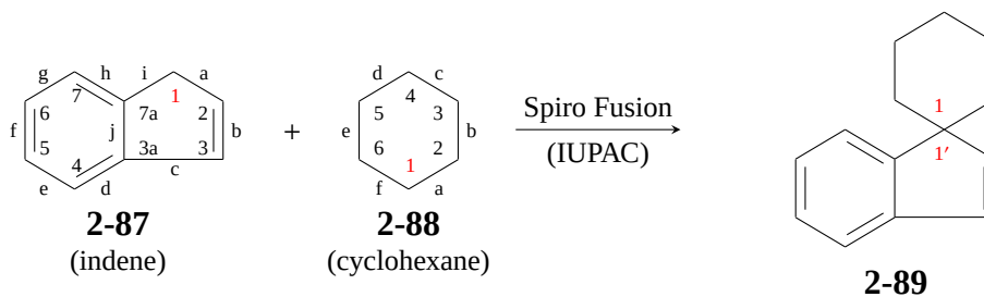
2-89 (spiro[cyclohexane-1,1'-indene])
