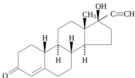
17 \alpha -ethynyl-17 \beta -hydroxyestr-4-en-3-one norethindrone (or norethinsterone)
