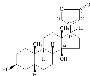
3β,14-dihydroxy-5β-card-20(22)-enolide digitoxigenin
