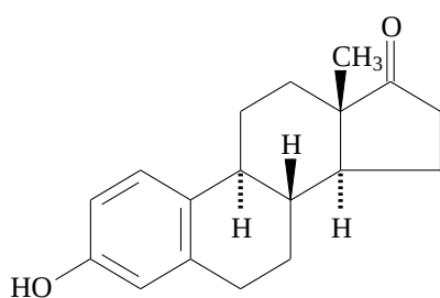
3-hydroxyestra-1,3,5(10)-trien-17-one estrone
