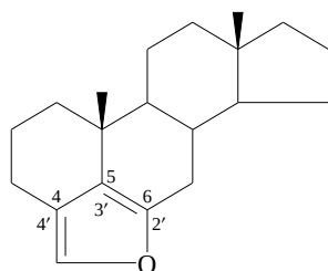
furo[ 4',3',2':4,5,6 ]androstane
