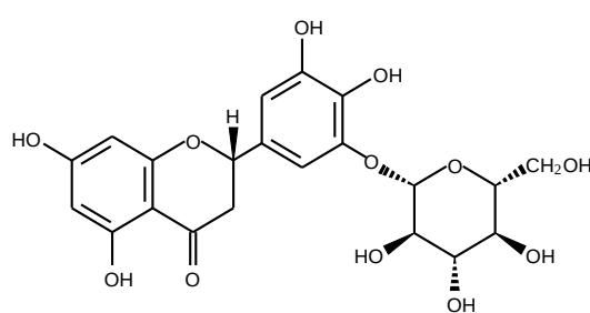
29-35 plantagoside
