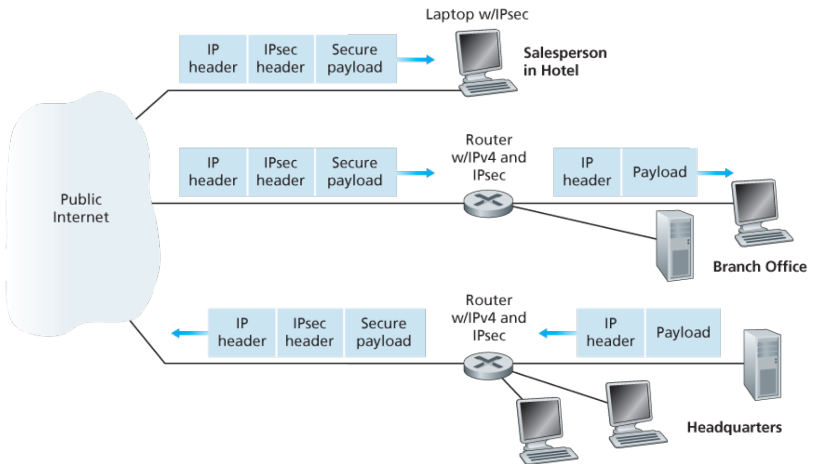
Figure 8.27 Virtual private network (VPN)
