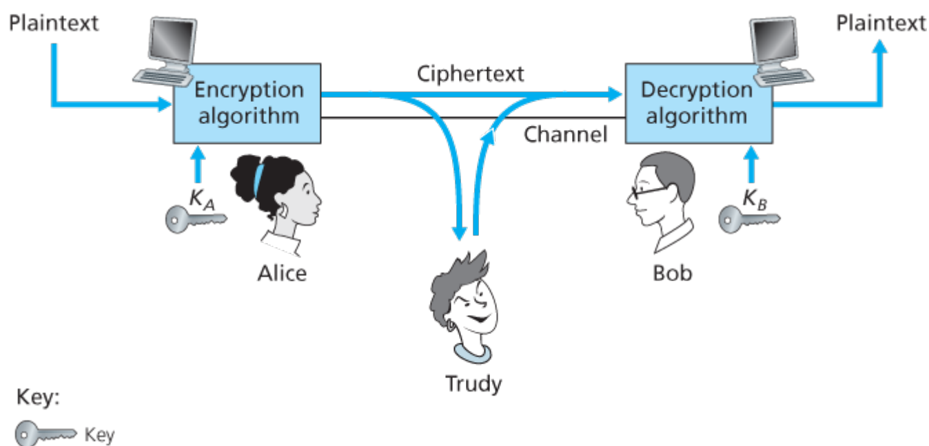
Figure 8.2 Cryptographic components
