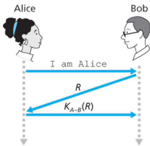
Figure 8.18 Protocol ap4.0 and a failure scenario
