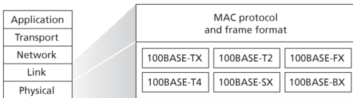
Figure 6.21 100 Mbps Ethernet standards: A common link layer, different physical layers
