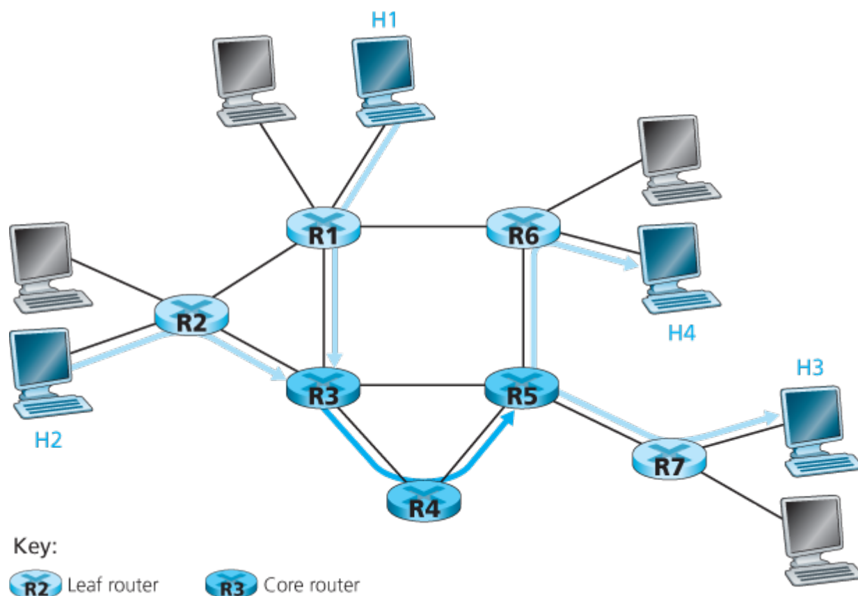
Figure 9.16 A simple Diffserv network example
