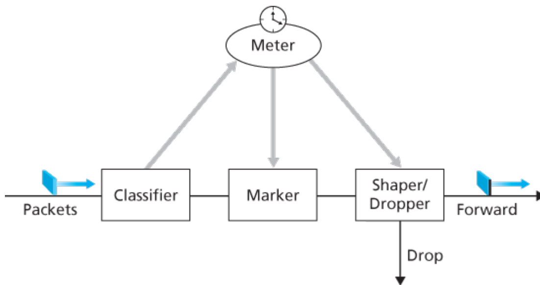
Figure 9.17 A simple Diffserv network example
