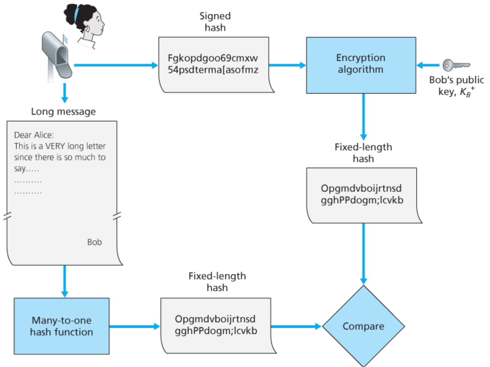
Figure 8.12 Verifying a signed message
