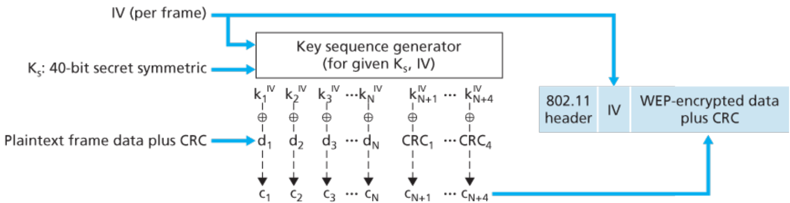
Figure 8.30 802.11 WEP protocol
