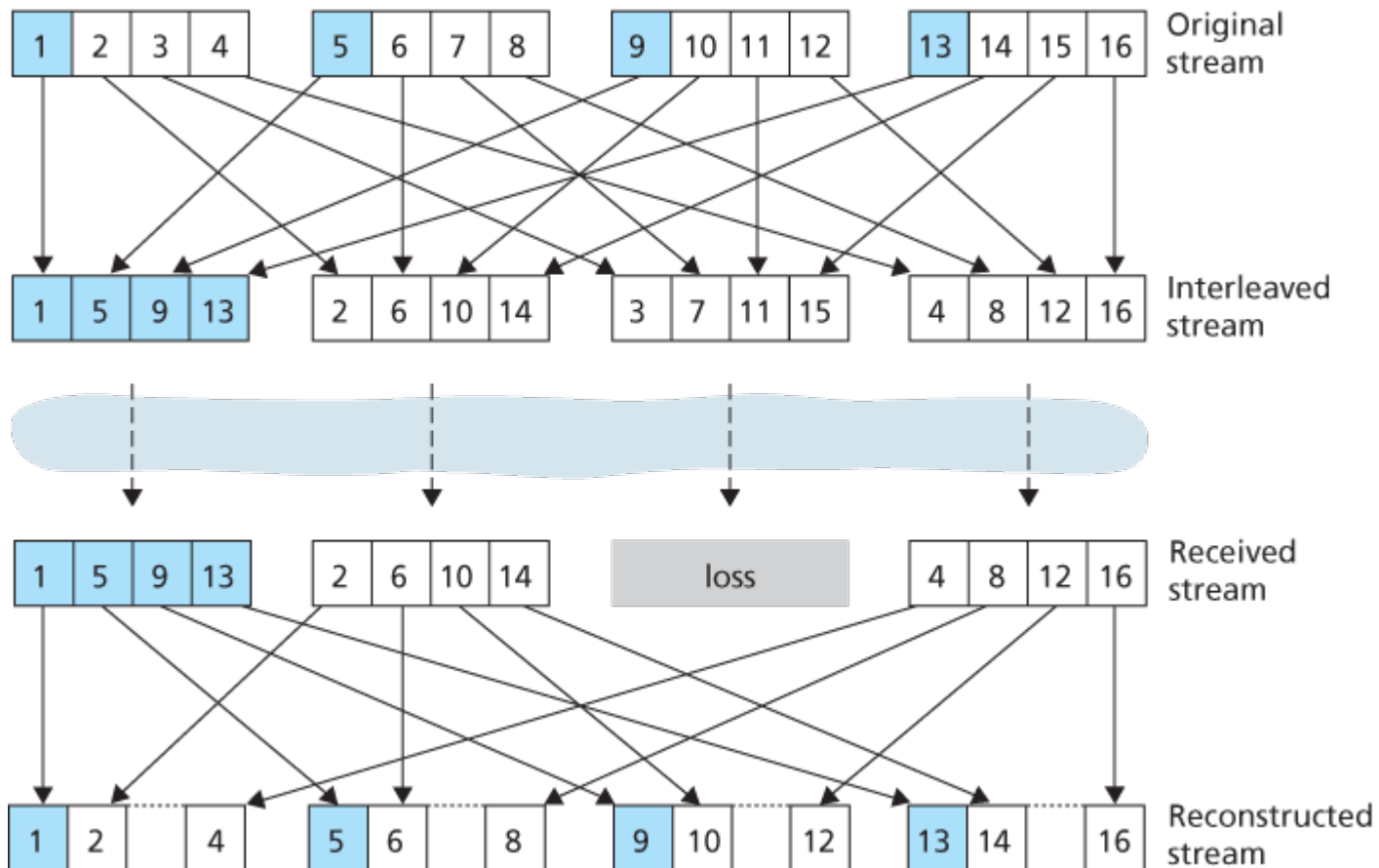
Figure 9.6 Sending interleaved audio
