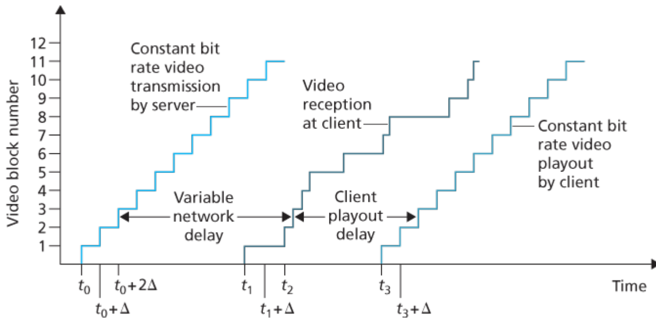
Figure 9.1 Client playout delay in video streaming
