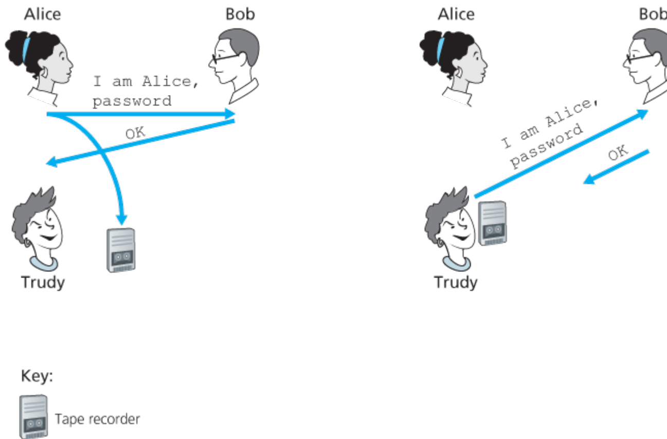
Figure 8.17 Protocol ap3.0 and a failure scenario
