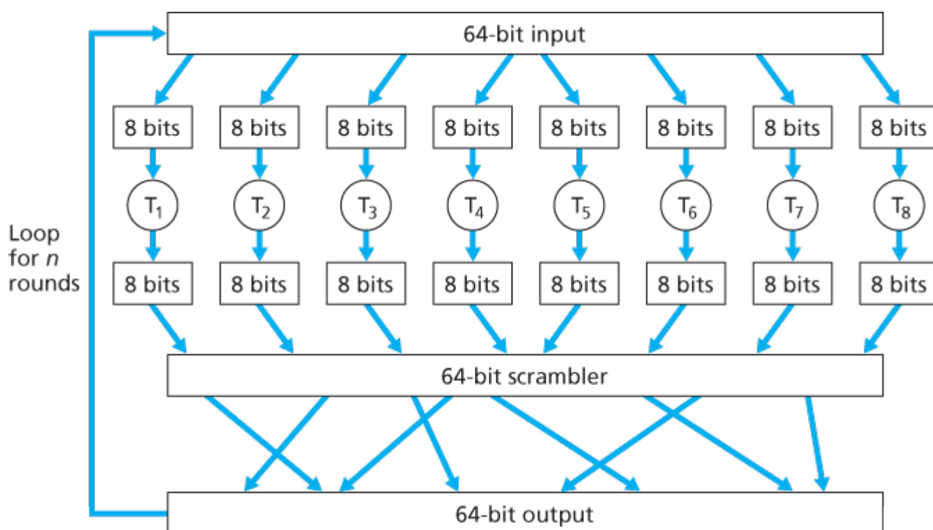
Figure 8.5 An example of a block cipher
