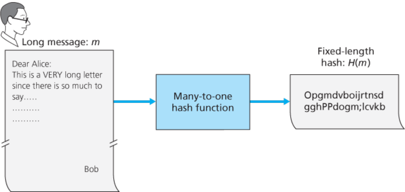
Figure 8.7 Hash functions
