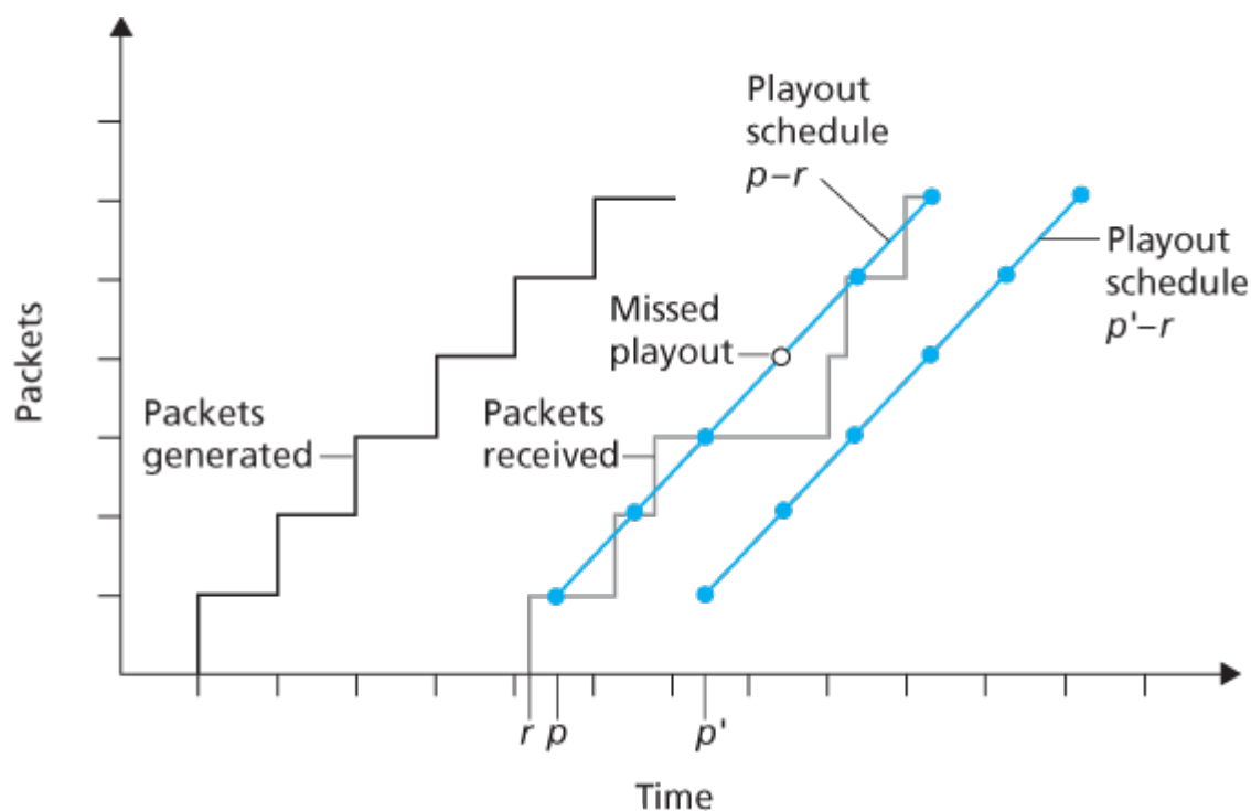
Figure 9.4 Packet loss for different fixed playout delays
