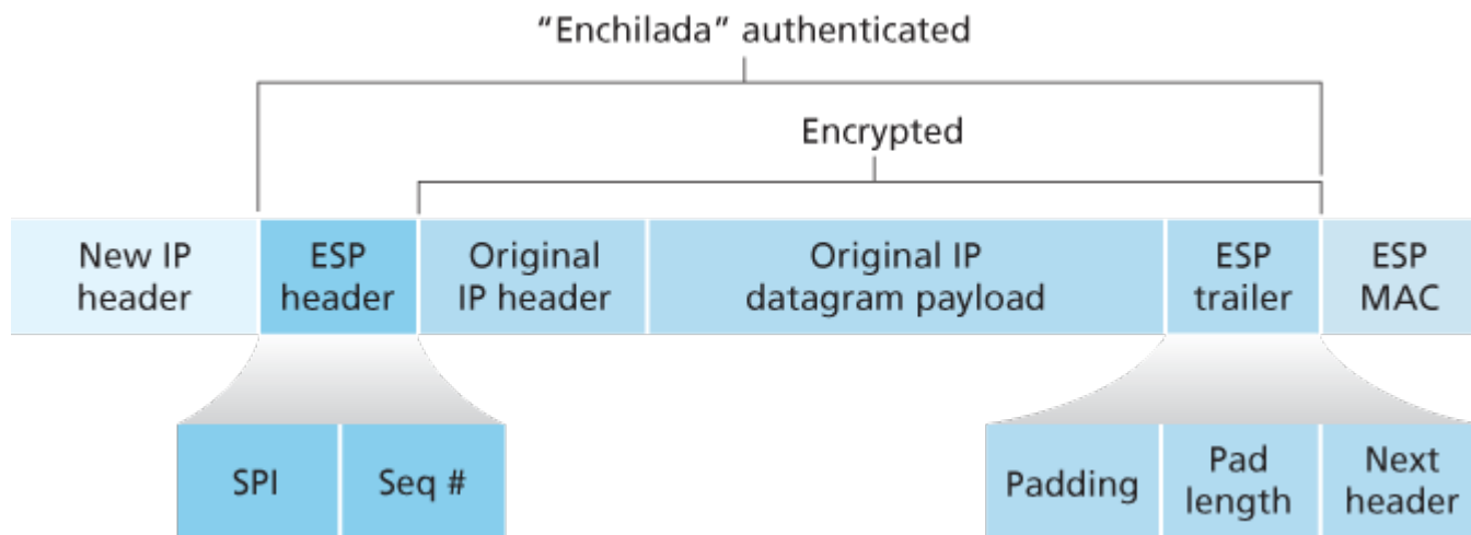
Figure 8.29 IPsec datagram format
