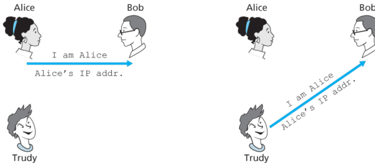
Figure 8.16 Protocol ap2.0 and a failure scenario
