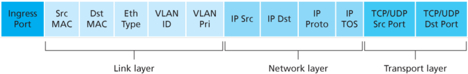
Figure 4.29 Packet matching fields, OpenFlow 1.0 flow table
