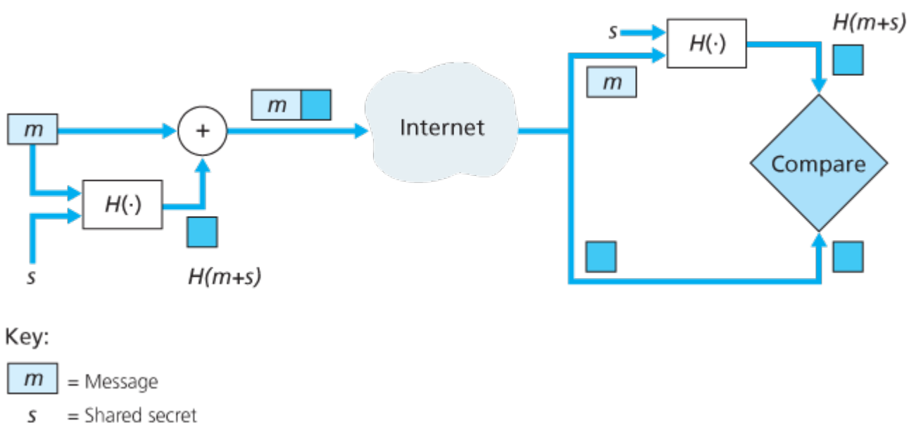
Figure 8.9 Message authentication code (MAC)
