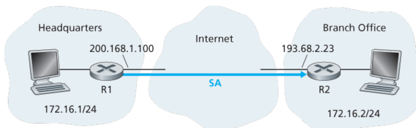
Figure 8.28 Security association (SA) from R1 to R2
