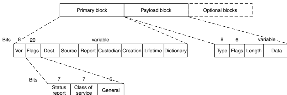
Figure 6-59. Bundle protocol message format.
