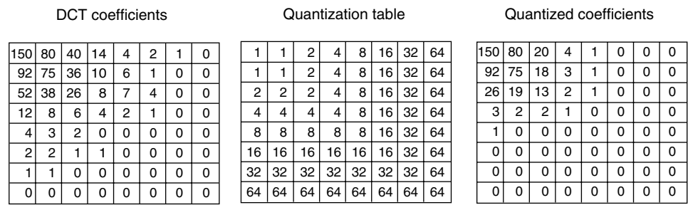
Figure 7-47. Computation of the quantized DCT coefficients.
