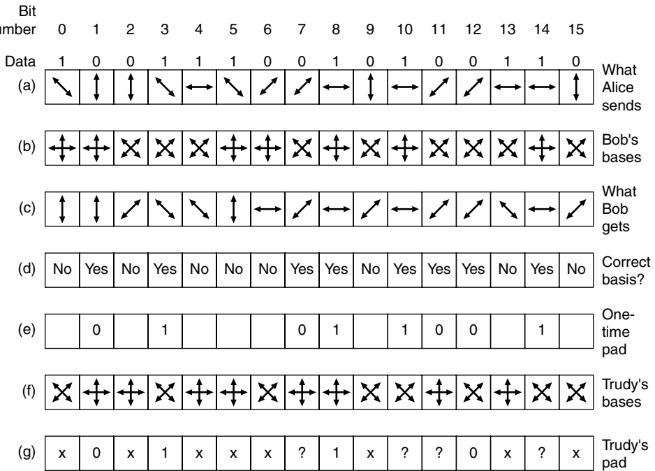
Figure 8-5. An example of quantum cryptography.
