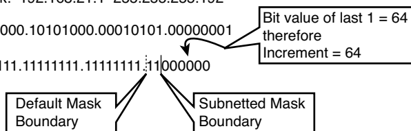
FIGURE 3.4 IP address and subnetted mask.
