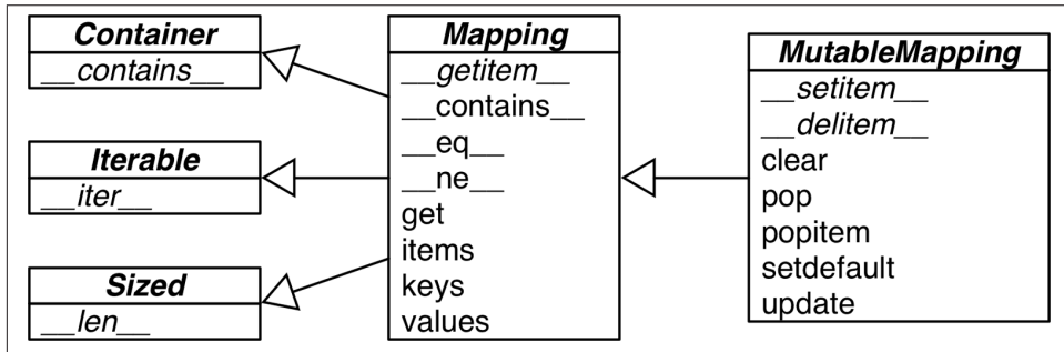
Figure 3-1. UML class diagram for the MutableMapping and its superclasses from collections.abc (inheritance arrows point from subclasses to superclasses; names in italics are abstract classes and abstract methods)
