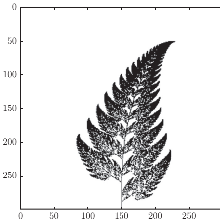
Figure 7.25 The Barnsley fern fractal.
