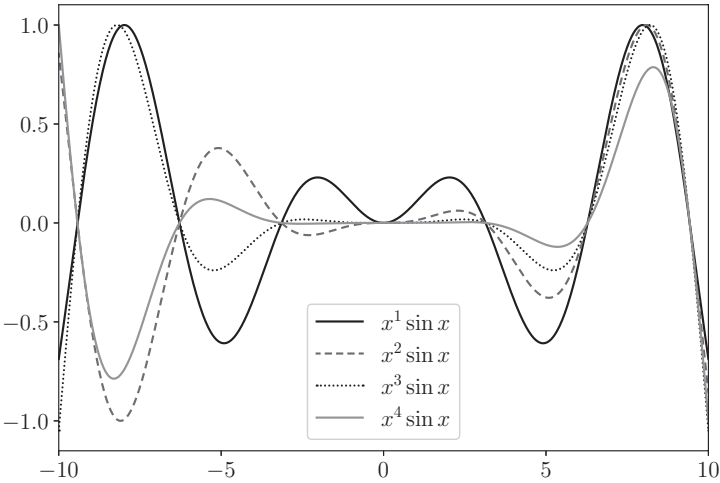
Figure 3.6 f_n(x) = x^n \sin x for n = 1, 2, 3, 4 .
