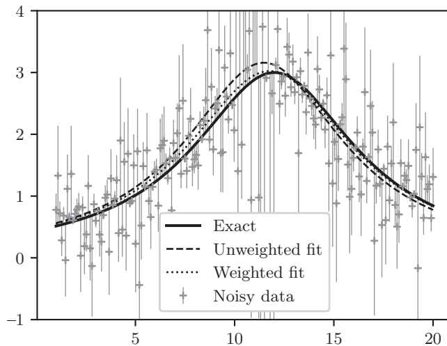
Figure 8.25 Example of least-squares fit with scipy.optimize.curve_fit .
