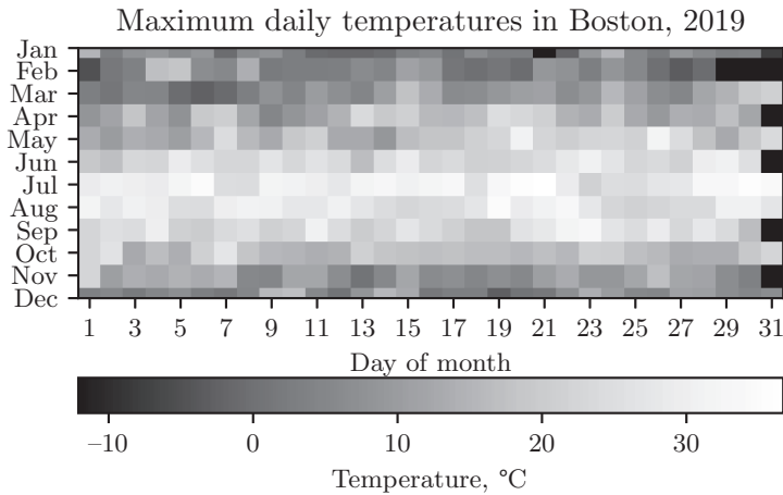
Figure 7.26 A heatmap of maximum daily temperatures in Boston during 2019.
