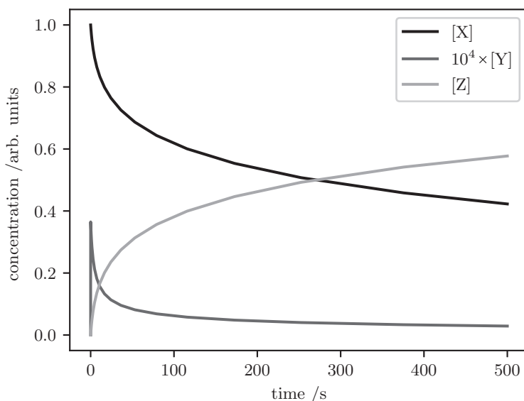
Figure 8.14 The Robertson chemical equation system, numerically integrated with the Radau IIA method.
