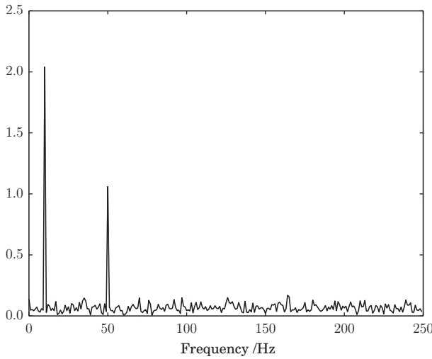
Figure 6.16 The positive-frequency components of the Fourier transform of a noisy waveform, normalized to show their intensities.
