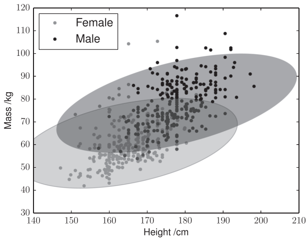
Figure 7.19 Scatter plots for each gender of mass and height for a total of 507 students, with their covariance ellipses annotated.
