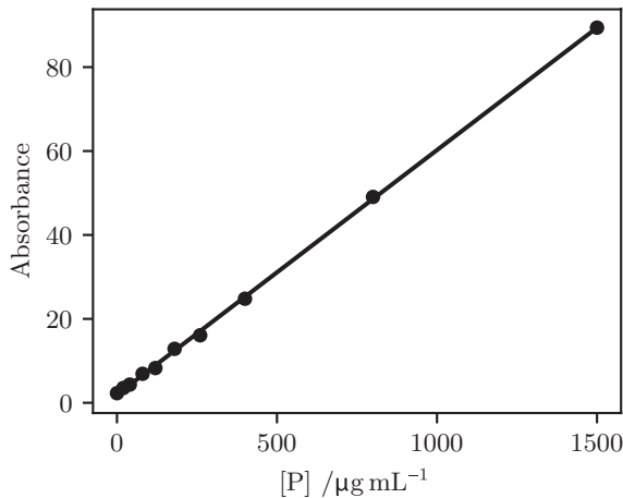
Figure 6.8 Line of least-squares best fit to absorbance data as a function of concentration.
