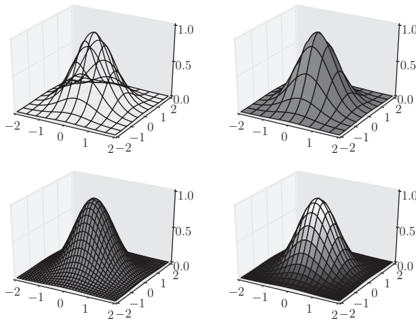
Figure 7.28 Four different three-dimensional surface plots of the same function.
