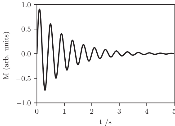
Figure 7.31 The final frame of an animation of a decaying sine curve.
