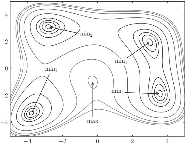
Figure 8.20 Contour plot of Himmelblau’s function.
