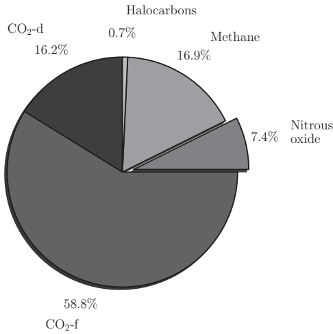
Figure 7.12 Greenhouse gas emissions by percentage for five different sources. CO 2 -d denotes CO 2 emissions from deforestation; CO 2 -f denotes CO 2 emissions from fossil fuel burning.
