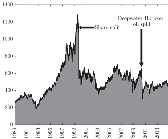
Figure 7.16 BP plc's share price on an annotated chart.
