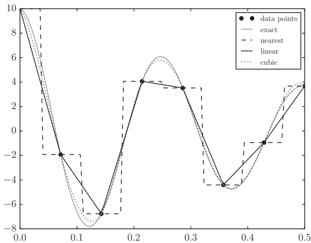
Figure 8.16 An illustration of different one-dimensional interpolation methods with scipy.interpolation.interp1d .
