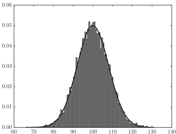
Figure 6.12 Histogram of 10 000 random samples from the normal distribution provided by np.random.normal .
