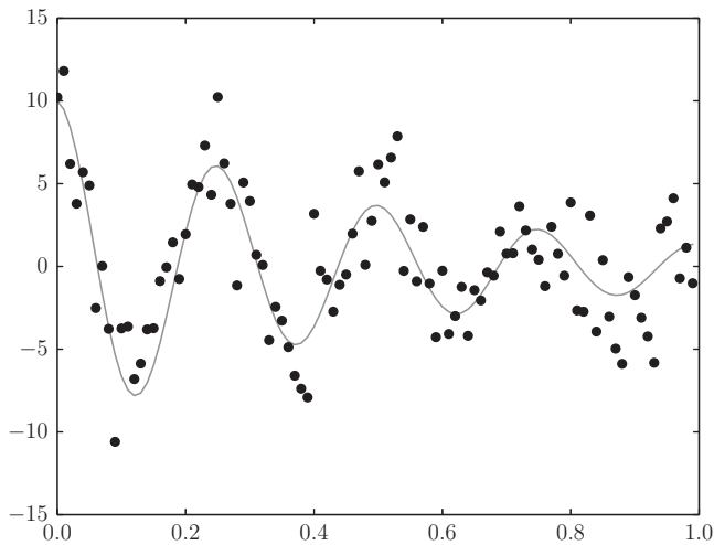
Figure 8.22 A synthetic noisy decaying cosine function.
