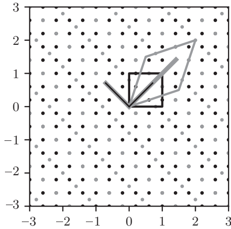
Figure 6.9 The effect of a linear transformation given by a matrix, \mathbf{T} , on the usual Cartesian basis: the unit square (black) is stretched along one diagonal and squeezed along the other; the scaled eigenvectors are also indicated.
