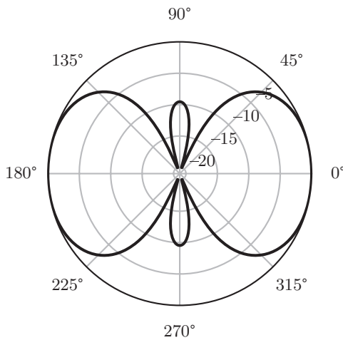
Figure 7.14 The directive gain of a many-antenna array with d = \lambda/2 , w_0 = 1 , w_1 = -1 , w_2 = 1 .
