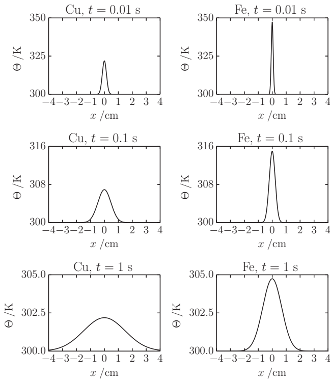
Figure 7.8 Numerical solutions of the one-dimensional diffusion equation for the temperatures of two metal bars.
