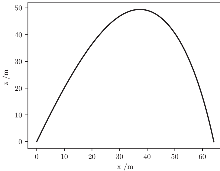
Figure 8.15 The trajectory of a spherical projectile launched with v_0 = 50 \text{ m s}^{-1} at \phi_0 = 50^\circ including air resistance.
