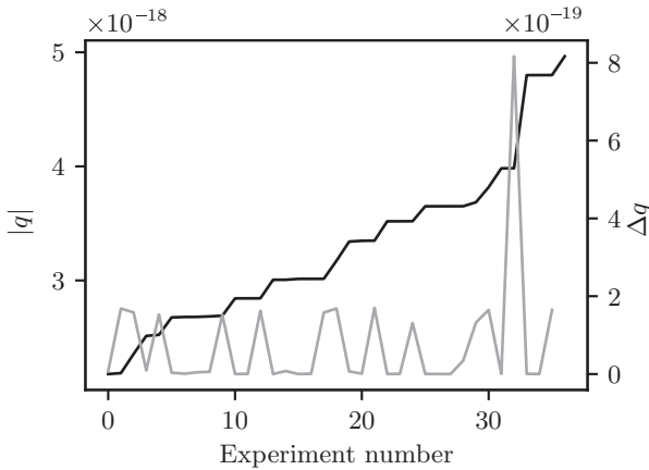
Figure 9.5 Sorted droplet charges, q , and neighbouring differences, \Delta q .
