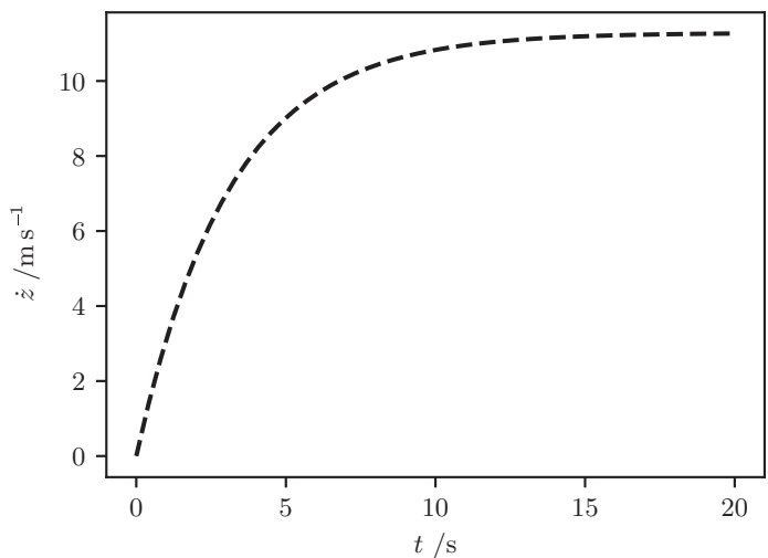
Figure 8.13 The velocity of a platinum sphere falling in mercury as a function of time, modeled with Stokes’ law.
