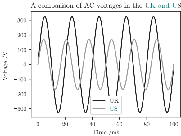
Figure 3.5 A comparison of AC voltages in the United Kingdom and United States.
