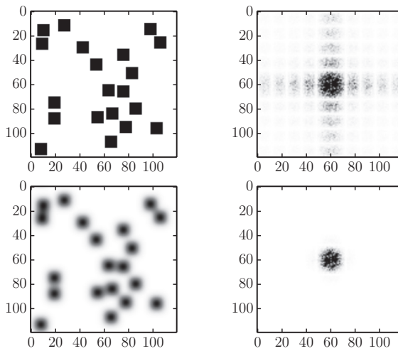
Figure 6.17 Blurring an image with a Gaussian filter applied to its two-dimensional Fourier transform.
