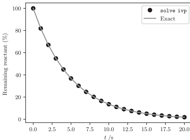
Figure 8.10 Exponential decay of a reactant in a first-order reaction: exact solution and numerical solution with pre-determined time points.
