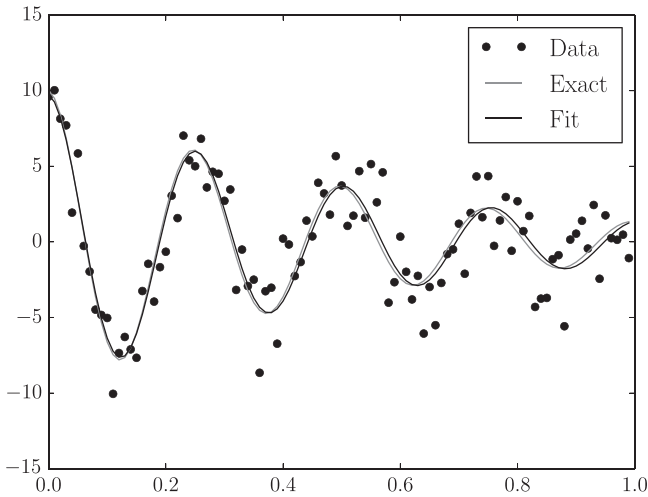
Figure 8.23 Non-linear least-squares fit to a noisy decaying cosine function.
