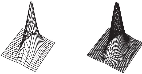
Figure 8.18 Two-dimensional interpolation from a coarse rectangular grid (left-hand plot) to a finer one (right-hand plot) with scipy.interpolate.RectBivariateSpline .
