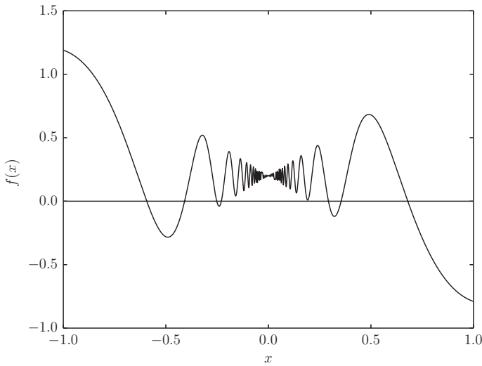
Figure 8.26 The function f(x) = \frac{1}{5} + x \cos(3/x) and its roots.
