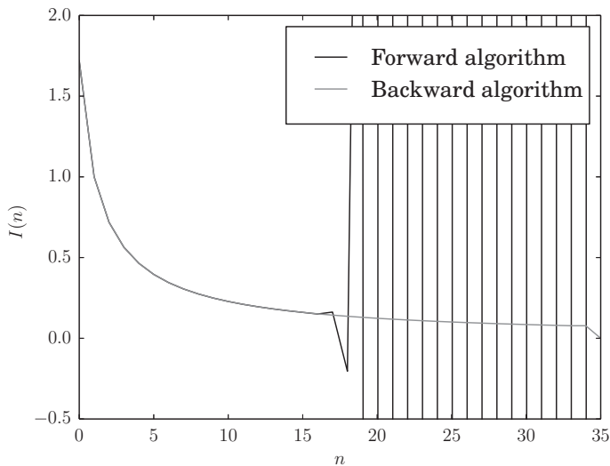
Figure 10.2 Instability of the forward recursion relation for I_n = \int_0^1 x^n e^x dx .
