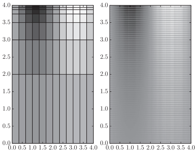
Figure 8.17 Two-dimensional interpolation with scipy.interpolate.interp2d .
