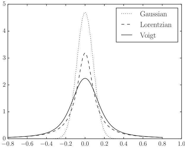
Figure 8.5 A comparison of the Lorentzian, Gaussian and Voigt line shapes with \gamma = \alpha = 0.1 .
