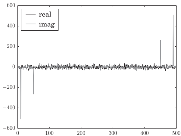
Figure 6.14 The Fourier transform of a noisy waveform with two frequency components, as returned by np.fft.fft .
