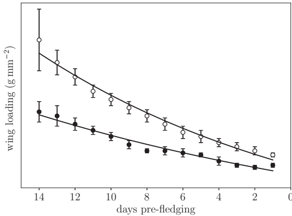
Figure 7.7 Fitted time series for wing-loading values in two cohorts of swift nestlings.
