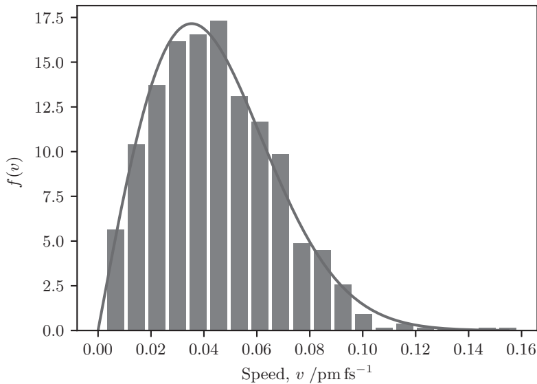
Figure 4.5 Distribution of particle speeds after equilibration to Maxwell–Boltzmann statistics through multiple collisions.
