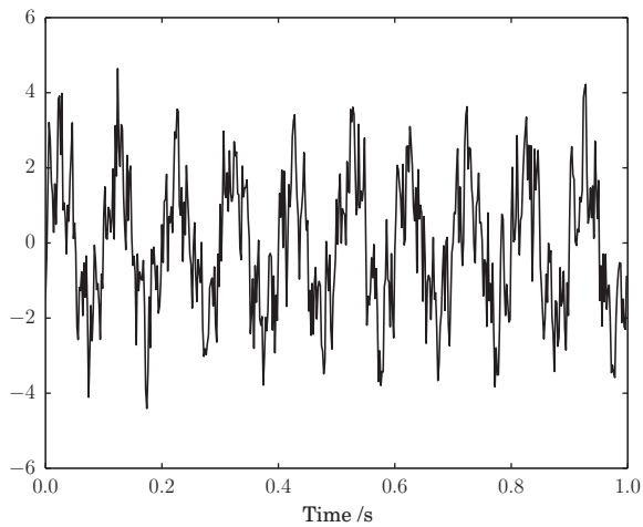
Figure 6.13 The noisy waveform referred to in the text.
