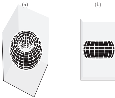
Figure 7.29 Two views of the same torus: (a) \theta = 36^\circ, \phi = 26^\circ , (b) \theta = 0^\circ, \phi = 0^\circ .
