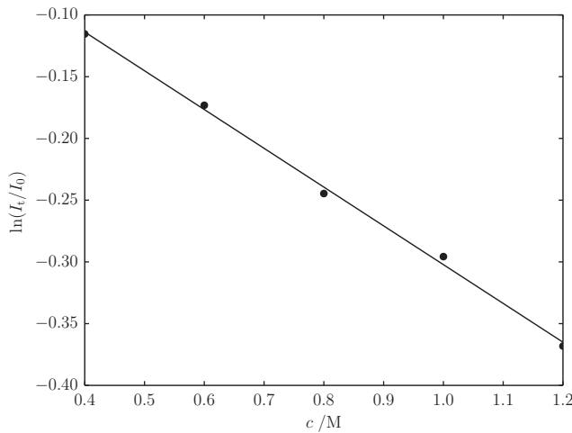
Figure 6.10 Line of least-squares best fit to absorbance data as a function of concentration.
