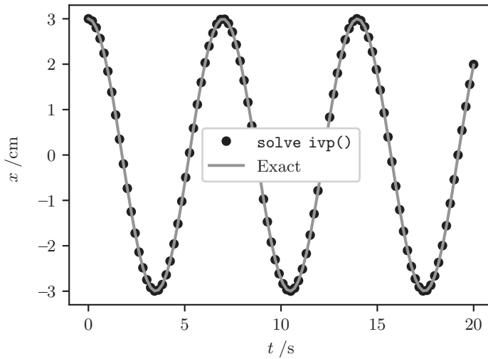
Figure 8.12 The harmonic oscillator: numerical and exact solutions.
