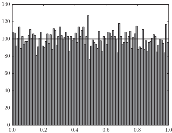
Figure 6.11 Histogram of 10 000 random samples from the uniform distribution on [0, 1) provided by np.random.random_sample() .
