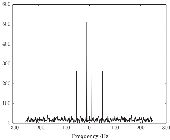
Figure 6.15 The Fourier Transform of a noisy waveform with two frequency components plotted against frequency.
