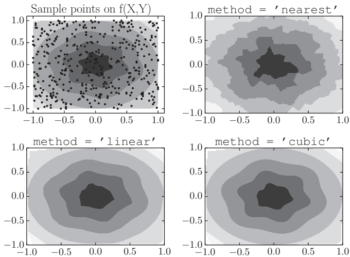
Figure 8.19 Some different interpolation schemes for scipy.interpolate.griddata .
