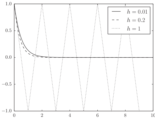
Figure 10.1 Instability of the forward Euler solution to dy/dx = -\alpha y for large step size, h .
