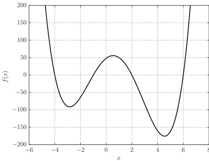
Figure 8.21 The polynomial f(x) = x^4 - 3x^3 - 24x^2 + 28x + 48 .
