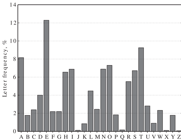
Figure 7.10 Letter frequencies in the novel Moby-Dick .
