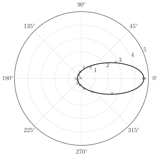
Figure 8.24 Nonlinear least-squares fitting of data to the equation of an ellipse in polar coordinates.
