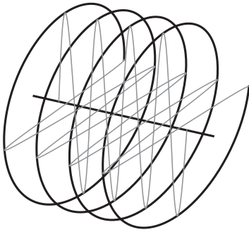
Figure 7.30 A depiction of circularly polarized light as a helix on a three-dimensional plot.
