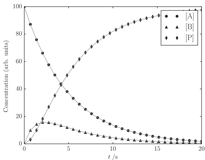
Figure 8.11 Two coupled first-order reactions: numerical and exact solutions.
