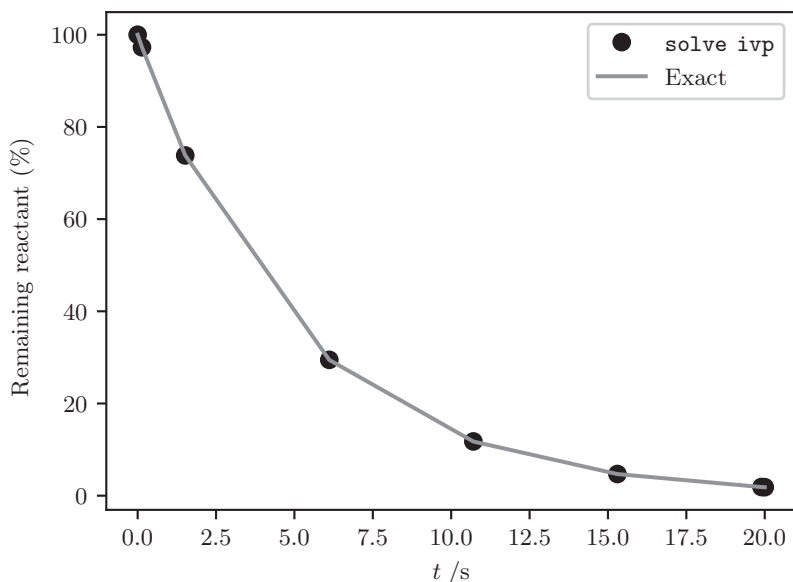
Figure 8.9 Exponential decay of a reactant in a first-order reaction: exact solution and numerical solution with time points selected by the ODE solver.
