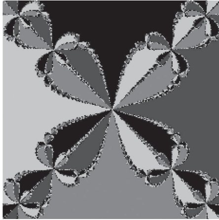
Figure 8.27 The Newton fractal for the function f(z) = z^4 - 1 . Intricate, self-similar structures are seen for initial guesses, z_0 , in between the roots (-1, 1, -i, i) .
