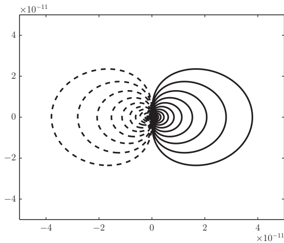
Figure 7.22 A contour plot of the electrostatic potential of a point dipole.
