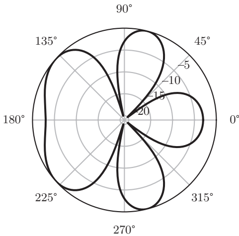
Figure 7.13 The directive gain of a two-antenna array with d = \lambda , w_0 = 1 , w_1 = -i .
