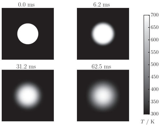
Figure 7.27 A representation of the temperature of a circular disc at four times after its instantaneous heating.
