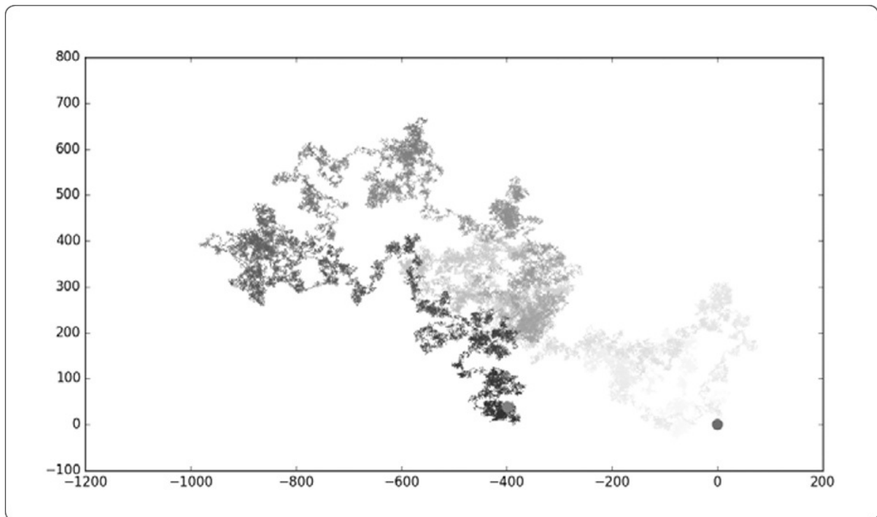
Figure 15-11: A walk with 50,000 points
