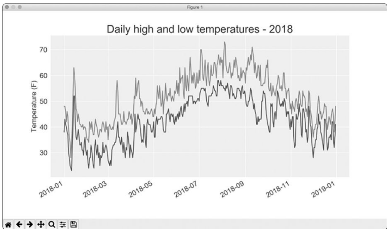
Figure 16-4: Two data series on the same plot
