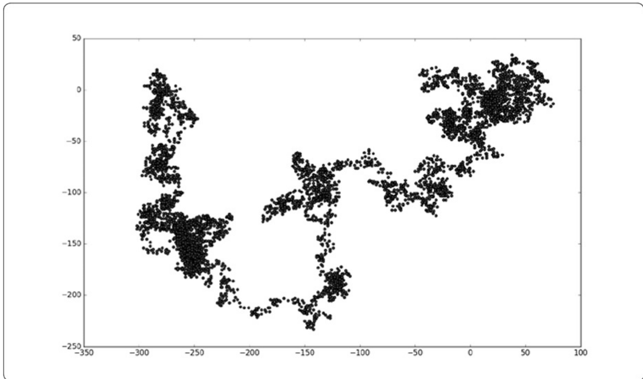
Figure 15-9: A random walk with 5000 points
