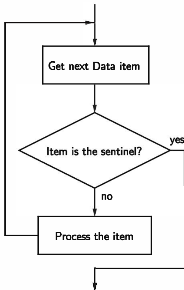
Figure 8.3: Loop-and-a-half implementation of sentinel loop pattern
