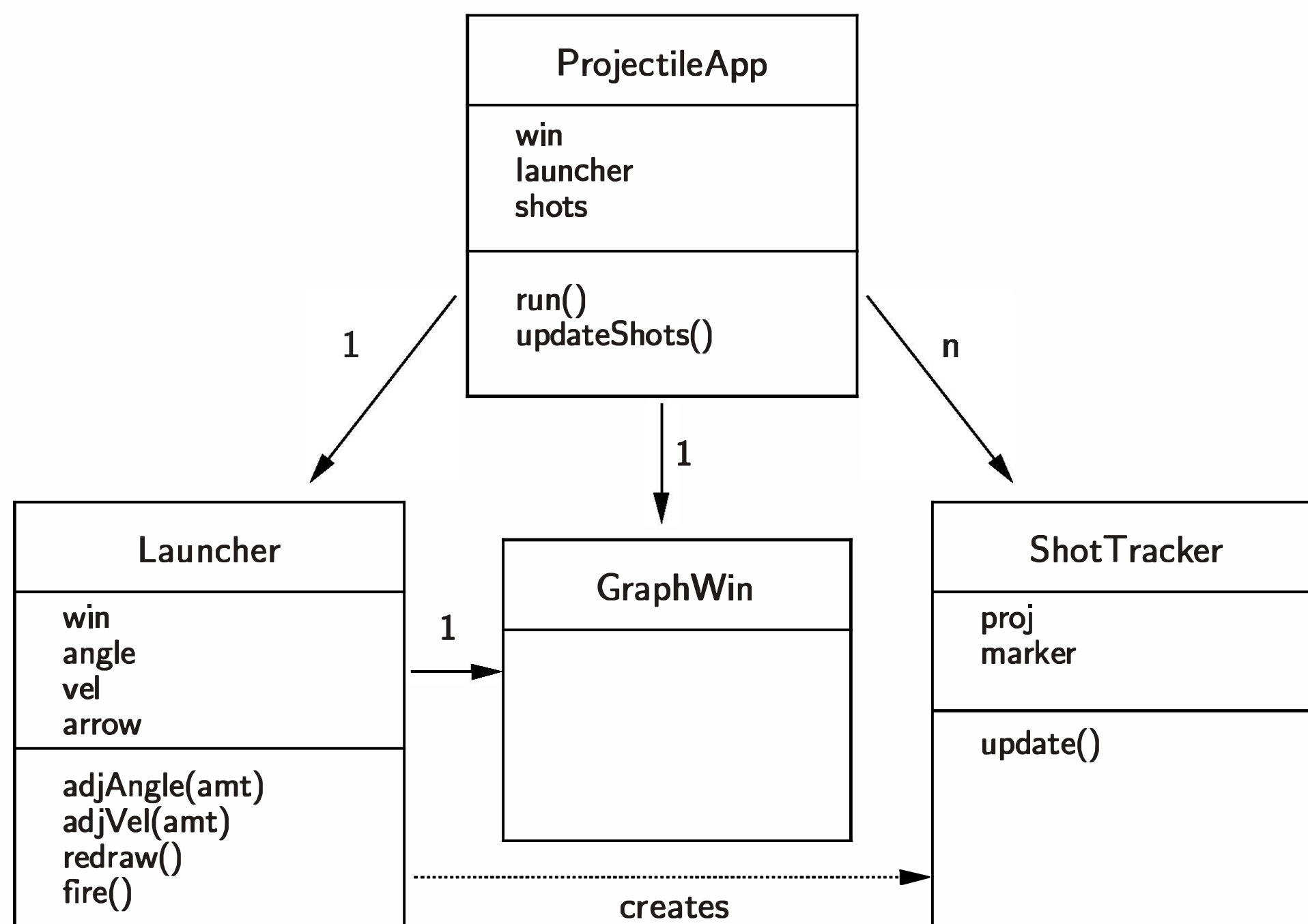
Figure 11.3: Class diagram for the multi-shot animation
