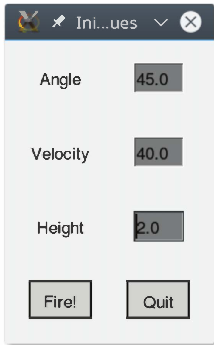
Figure 10.5: Custom input dialog for cannonball animation
