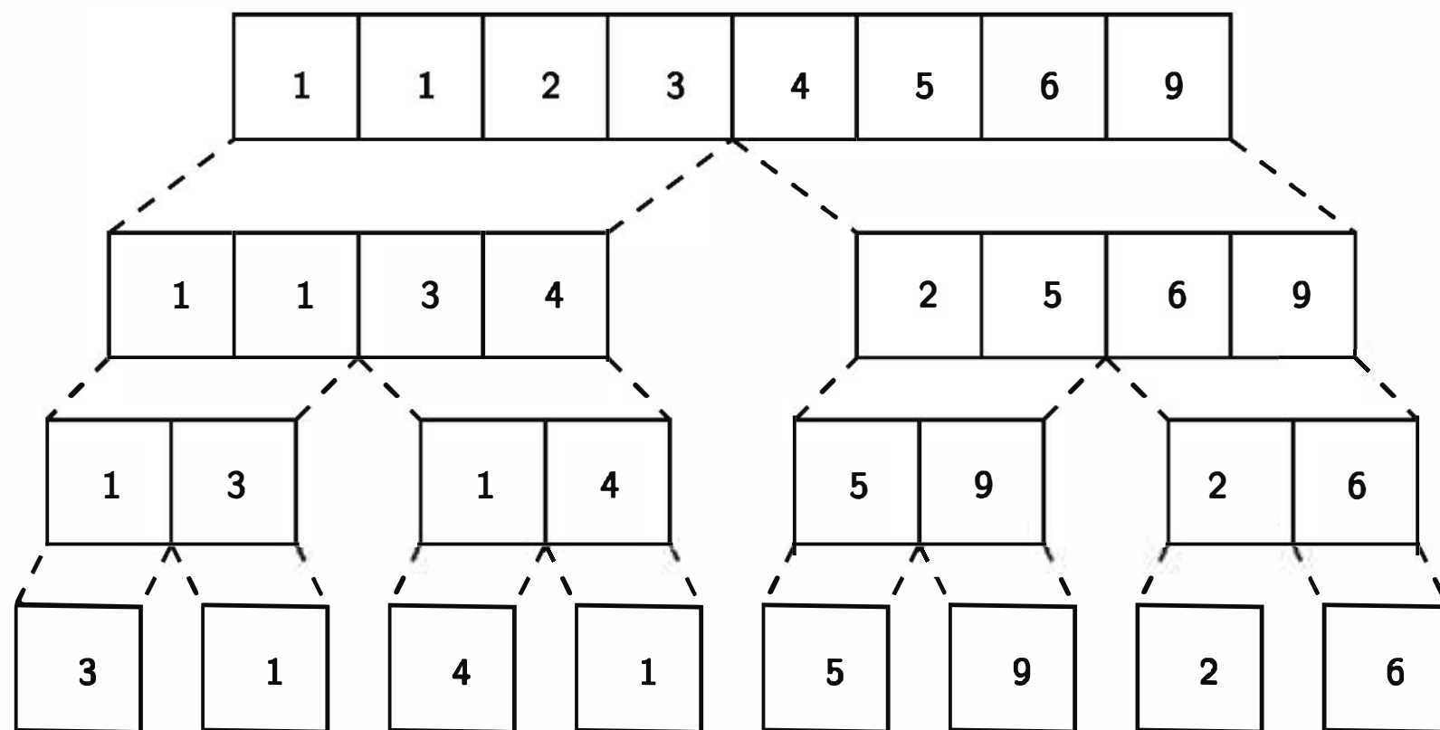
Figure 13.3: Merges required to sort [3, 1, 4, 1, 5, 9, 2, 6]
