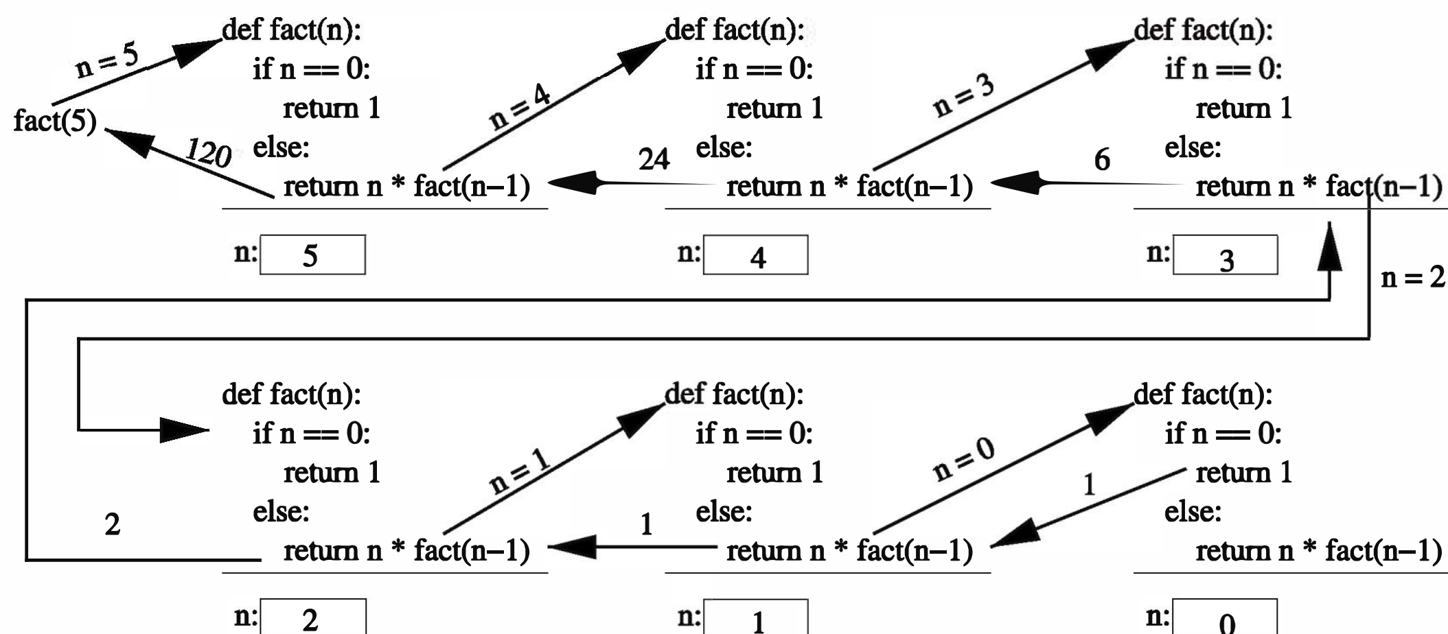
Figure 13.1: Recursive computation of 5!
