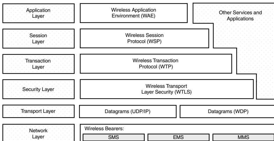
Figure 8.6 WAP layer structure.
