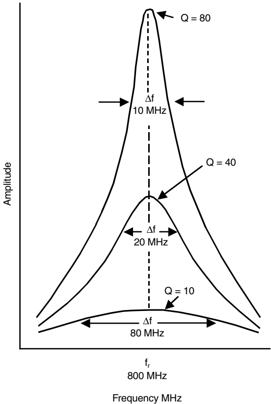
Figure 13.12 Q versus bandwidth.
