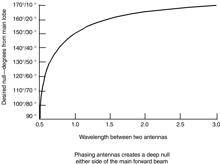
Figure 13.4 Nulling.
