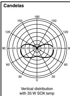
Figure 15.6 Photometric data from a Philips street lamp.
