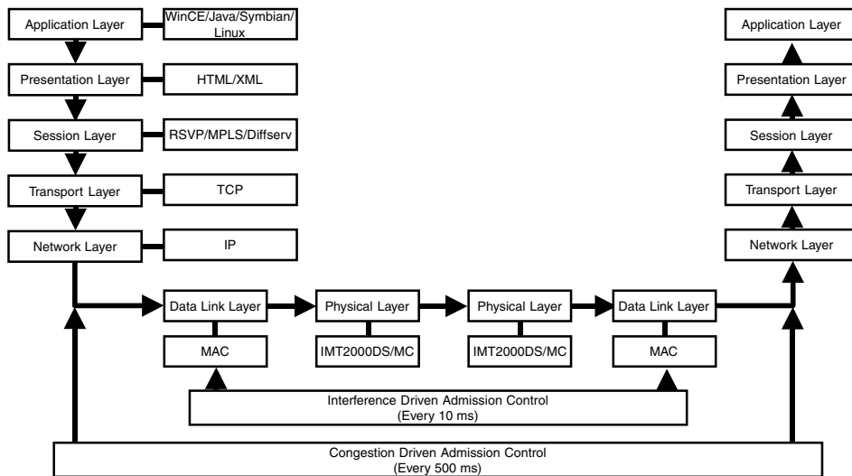
Figure 17.8 Admission control.
