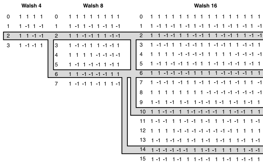
Figure 3.26 Variable length Walsh codes.
