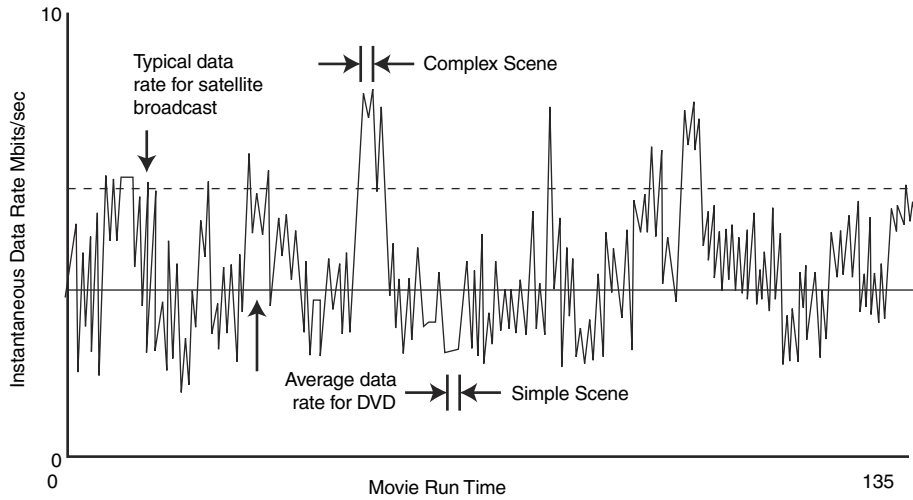
Figure 7.2 Variable-rate encoding.
