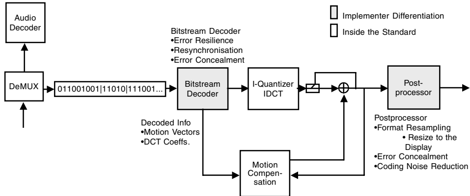
Figure 4.11 Video decoding.
