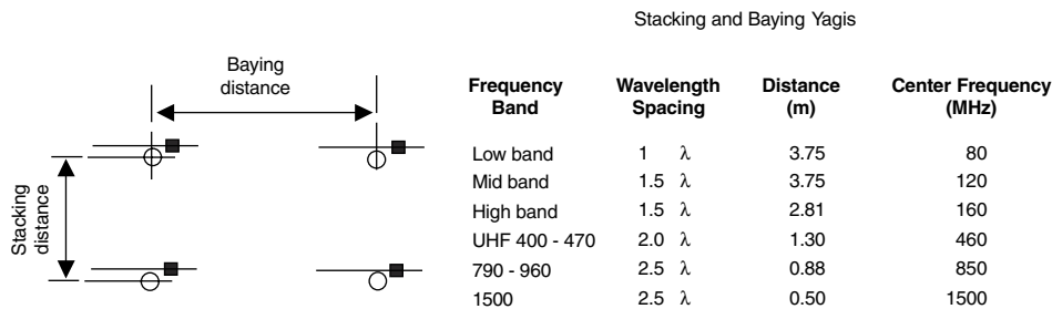
Figure 13.3 Stacking and baying.
