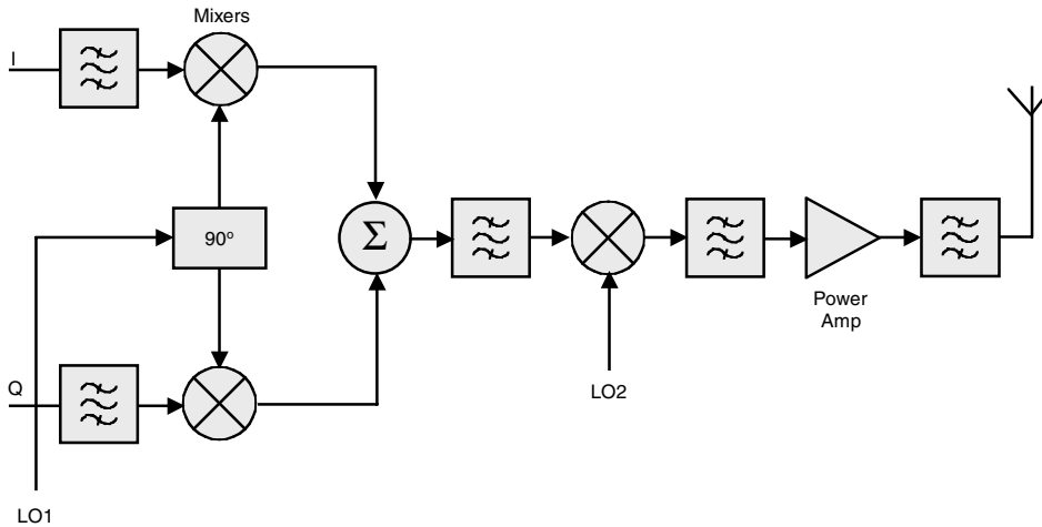
Figure 2.8 Upconverting transmitter.
