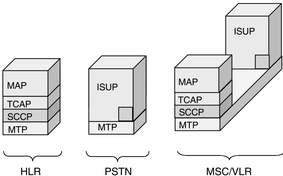
Figure 16.7 HLR/PSTN/MSC/VLR.
