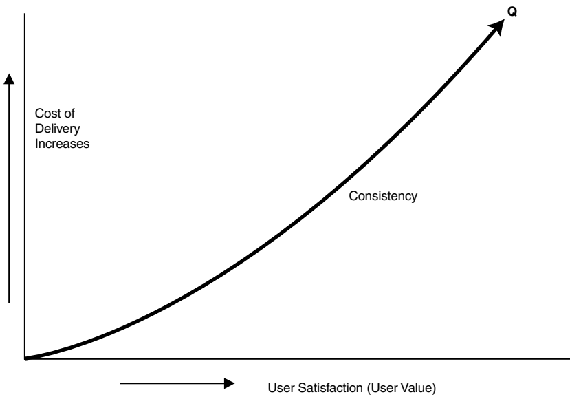
Figure 7.7 Consistency metric.
