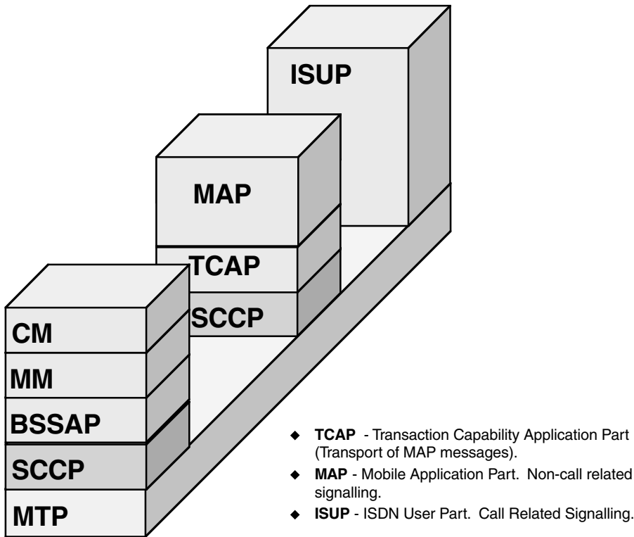
Figure 16.6 MSC/VLR.
