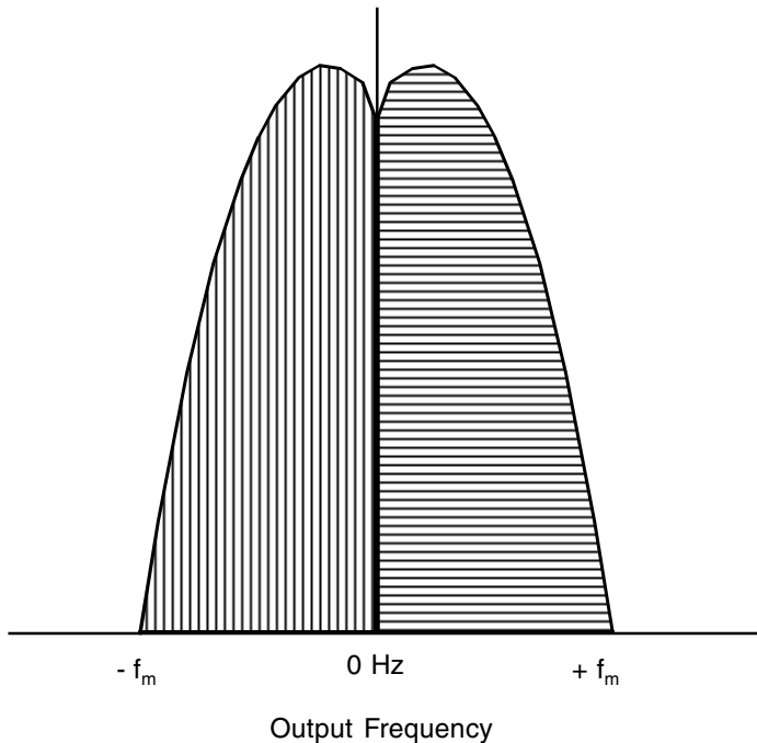
Figure 2.4 The negative frequency.
