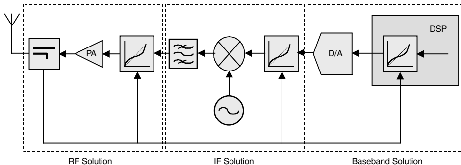
Figure 11.11 Location for predistorter components.
