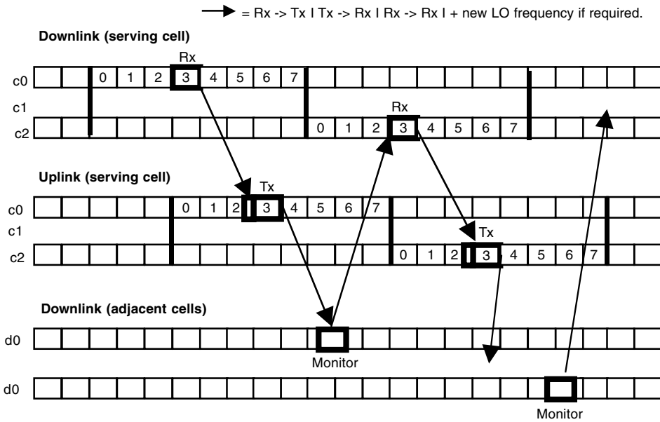
Figure 2.2 Rx/Tx offsets and the monitor channel (Rx/Tx channels shown with frequency hopping).
