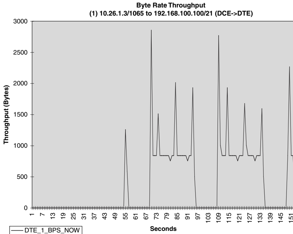
Figure 17.4 Network loading.
