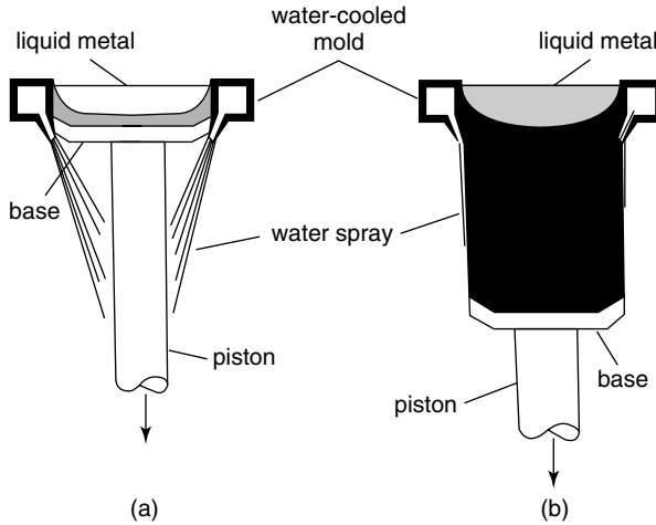
Figure 7.3 Schematic illustration of semicontinuous casting process in which (a) molten metal solidifies in a water-cooled mold with a movable base and (b) the base is moved downward so more metal can be poured into the reservoir. Reprinted, by permission, from the McGraw-Hill Encyclopedia of Science and Technology , Vol. 11, 8th ed., p. 31. Copyright © 1997 by McGraw-Hill.
