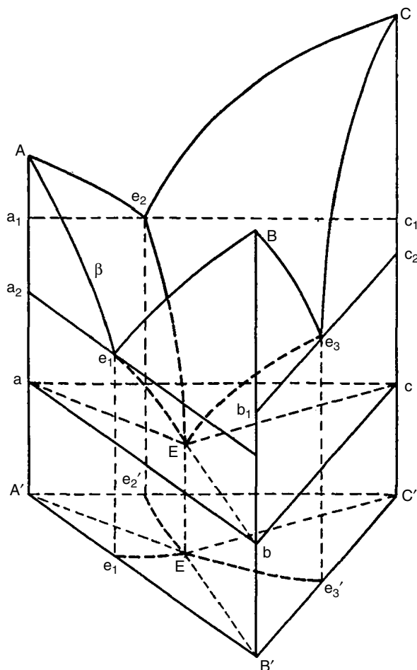
Figure 2.19 Perspective drawing of a ternary system with a simple eutectic and no ternary compound. Reprinted, by permission, from Phase Diagrams for Ceramists , Vol. 1, p. 15. Copyright © 1964, The American Ceramic Society.
