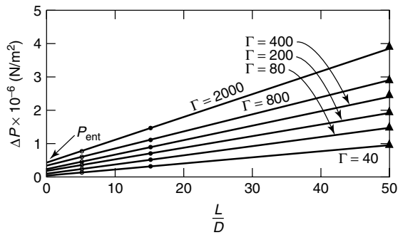
Figure 7.71 Bagley plots for a polystyrene melt at 200°C. From Z. Tadmor and C. G. Gogos, Principles of Polymer Processing . Copyright © 1979 by John Wiley & Sons, Inc. This material is used by permission of John Wiley & Sons, Inc.
