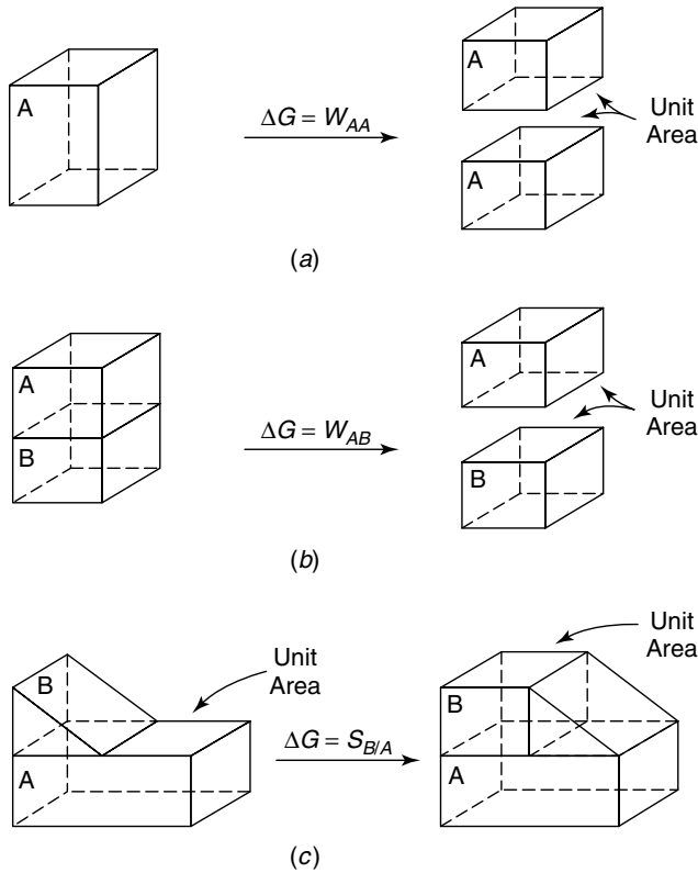
Figure 2.35 Schematic illustrations of the processes for which \Delta G equals (a) the work of cohesion, (b) the work of adhesion, and (c) the work of spreading. Reprinted, by permission, from P. Heimez, Principles of Colloid and Surface Chemistry , 2nd ed., p. 316. Copyright © 1986 by Marcel Dekker, Inc.
