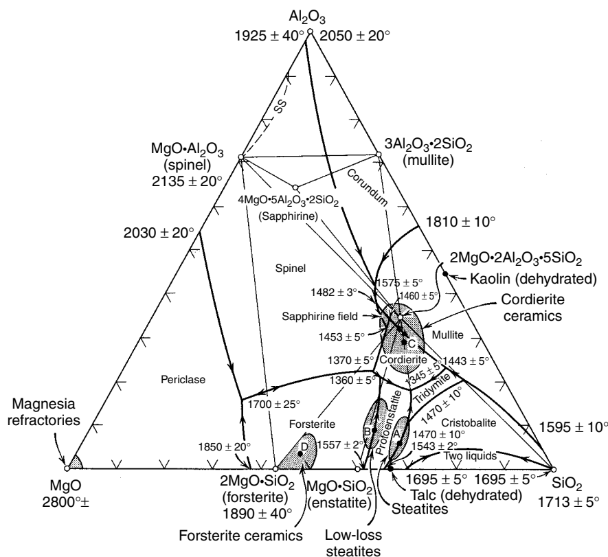
Figure 2.23 The \text{MgO}-\text{Al}_2\text{O}_3-\text{SiO}_2 phase diagram. Temperatures are in ^\circ\text{C} . From Introduction to Ceramics . W. D. Kingery, H. K. Bowen, and D. R. Uhlmann, Copyright © 1976 by John Wiley & Sons, Inc. This material is used by permission of John Wiley & Sons, Inc.
