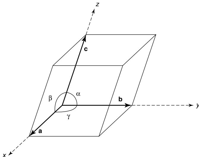
Figure 1.19 Definition of a coordinate system for crystal structures.
