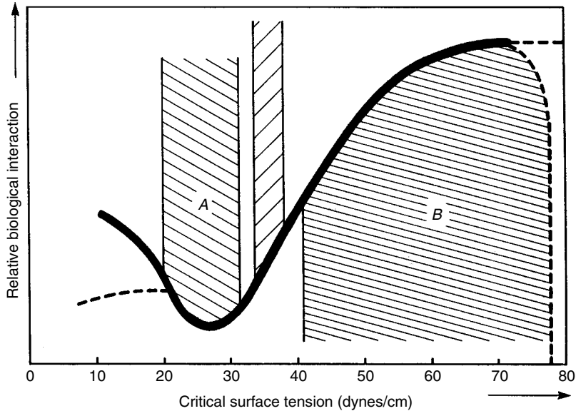
Figure 2.37 Relationship between the biological interactiveness and the critical surface tension of a biomaterial. Reprinted, by permission, from J. M. Schakenraad, Cells: Their Surfaces and Interactions with Materials , in Biomaterials Science: An Introduction to Materials in Medicine , B. D. Ratner, A. S. Hoffman, F. J. Schoen, and J. E. Lemons, p. 146. Copyright © 1996 by Academic Press.
