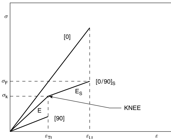
Figure 5.123 Schematic tensile stress–strain diagram for a symmetric (0, \pm 90^\circ) cross-ply laminate tested at 2 = 0^\circ . Reprinted, by permission, from P. K. Mallick, Fiber-Reinforced Composites , p. 187. Copyright © 1988 by Marcel Dekker, Inc.
