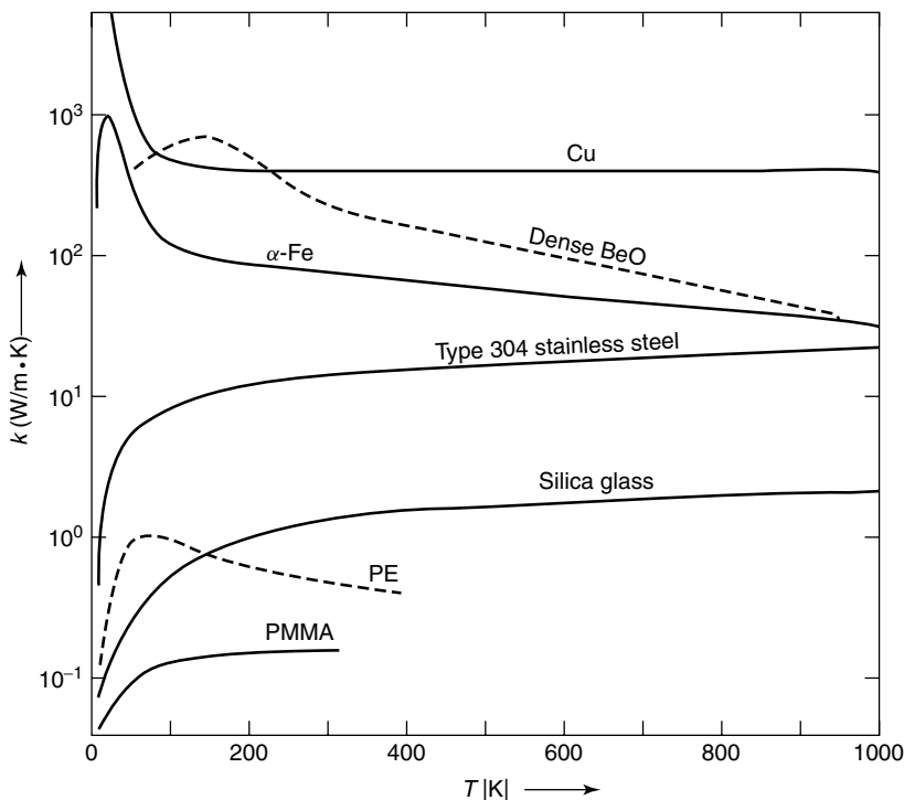
Figure 4.26 Variation of thermal conductivity with temperature for ordered (Cu, BeO, Fe, and PE) and disordered (SS, silica glass, and PMMA) with temperature. From K. M. Ralls, T. H. Courtney, and J. Wulff, Introduction to Materials Science and Engineering . Copyright © 1976 by John Wiley & Sons, Inc. This material is used by permission John Wiley & Sons, Inc.
