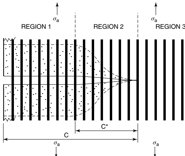
Figure 5.113 Microcrack parallel to fibers under applied stress, \sigma_a . Reprinted, by permission, from R. W. I. Davidge, and J. J. R. Davies, in Mechanical Testing of Engineering Ceramics at High Temperatures , B. F. Dyson, R. D. Lohr, and R. Morrell, eds., p. 253. Copyright © 1989 by Elsevier Science Publishers, Ltd.
