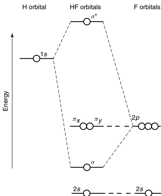
Figure 1.8 Molecular orbital diagram for HF. Reprinted, by permission, from R. E. Dickerson, H. B. Gray, and G. P. Haight, Jr., Chemical Principles , 3rd ed., p. 461. Copyright © 1979 by Pearson Education, Inc.
