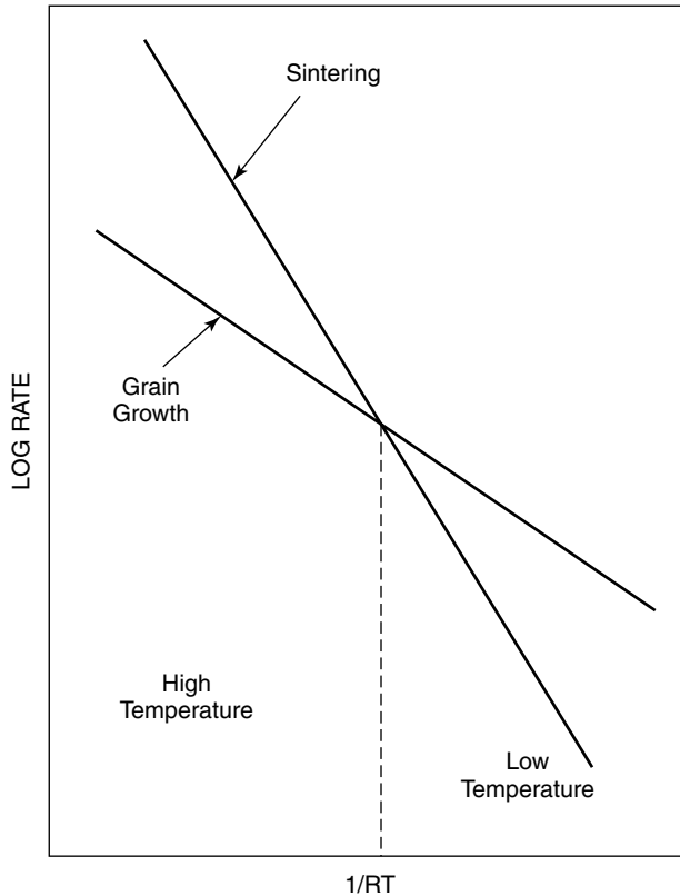
Figure 7.36 Temperature dependence of grain growth and sintering (densification) rates. The slope of each curve represents the activation energy. Adapted from J. S. Reed, Principles of Ceramics Processing , 2nd ed. Copyright © 1995 by John Wiley & Sons, Inc. This material is used by permission of John Wiley & Sons, Inc.
