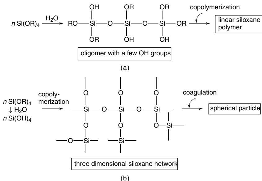
Figure 7.53 Hydrolysis and polymerization of a generic alkoxide \text{Si}(\text{OR})_4 involving both (a) acid and (b) basic routes. Reprinted, by permission, from H. Yanagida, K. Koumoto, and M. Miyayama, The Chemistry of Ceramics , p. 148. Copyright © 1996 by John Wiley & Sons, Inc.
