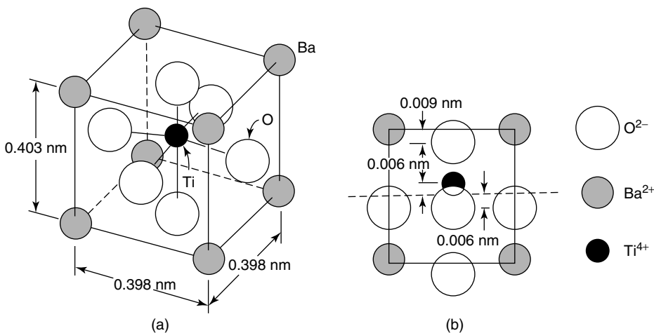
Figure 6.27 View of (a) the tetragonal unit cell of \text{BaTiO}_3 and (b) the ionic positions projected in a [100] direction onto a (100) face. From K. M. Ralls, T. H. Courtney, and J. Wulff, Introduction to Materials Science and Engineering . Copyright © 1976 by John Wiley & Sons, Inc. This material is used by permission John Wiley & Sons, Inc.
