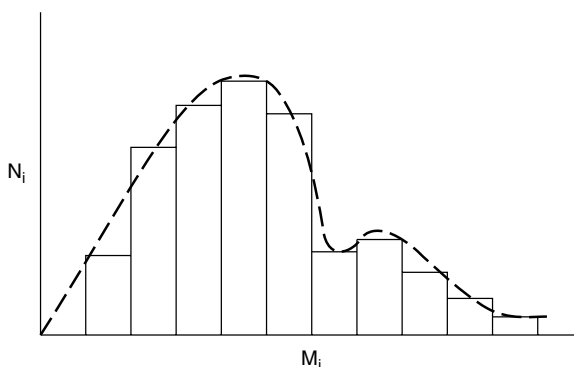
Figure 1.59 Histogram showing the number of molecules, N_i , having the molecular weight M_i . Reprinted, by permission, from P. Heimez, Polymer Chemistry: The Basic Concepts , p. 35. Copyright © 1984 by Marcel Dekker, Inc.
