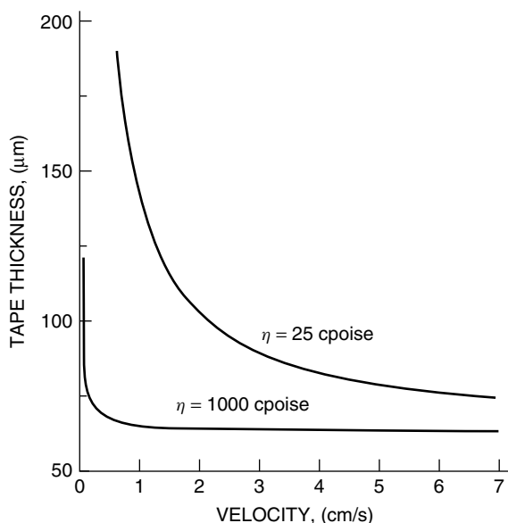
Figure 7.33 Variation of tape thickness with carrier velocity and slurry viscosity. Adapted from J. S. Reed, Principles of Ceramics Processing , 2nd ed. Copyright © 1995 by John Wiley & Sons, Inc. This material is used by permission of John Wiley & Sons, Inc.
