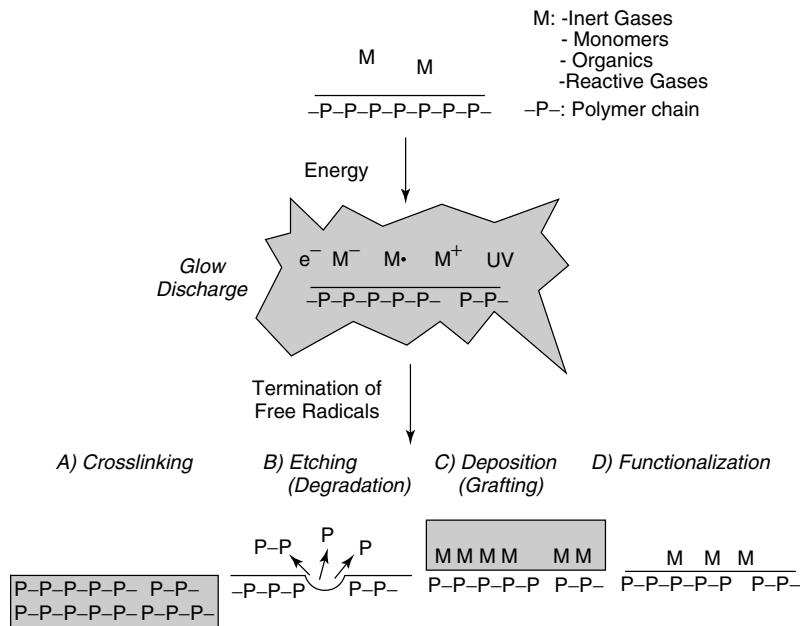
Figure 7.95 Schematic illustration of interactions of glow-discharge plasma with solid surfaces. Reprinted, by permission, from M. S. Sheu, D. M. Hudson, and I. H. Loh, in Encyclopedic Handbook of Biomaterials and Bioengineering , Part A: Materials, Vol. 1, p. 869. Copyright © 1995 by Marcel Dekker, Inc.
