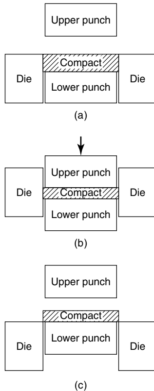
Figure 7.17 Schematic illustration of automated die-and-punch process in which (a) die is filled, (b) die is compacted, and (c) compact is ejected. Reprinted, by permission, from Encyclopedia of Materials Science & Engineering , Vol. 11, p. 3875. Copyright © 1986 by Pergamon Press.
