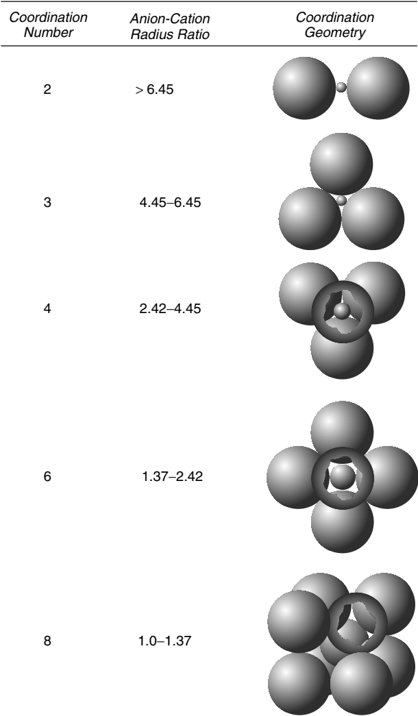
Figure 1.37 Critical radius ratios for various coordination numbers. Adapted, from W. Callister, Materials Science and Engineering: An Introduction , 5th ed., p. 384. Copyright © 2000 by John Wiley & Sons, Inc.
