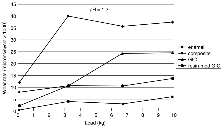
Figure 8.18 Wear rates for enamel and three dental restoration materials at different loads and pH 1.2. Reprinted from M. Shabanian and L. C. Richards, In vitro wear rates of materials under different loads and varying pH, J. Prosth. Dent. , 87 (6), 655. Copyright © 2002, with permission from Elsevier.
