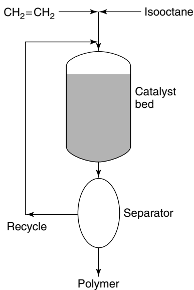
Figure 3.23 Schematic diagram of ethylene solution polymerization process.
