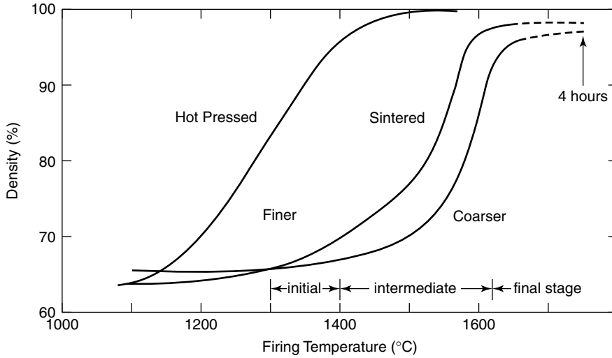
Figure 7.35 Densification behavior of compacts of two alumina powders (0.8- and 1.3- \mu\text{m} average particle size), with the sintering stages indicated for the coarser powder. A hot-pressed powder is shown for comparison. From J. S. Reed, Principles of Ceramics Processing , 2nd ed. Copyright © 1995 by John Wiley & Sons, Inc. This material is used by permission of John Wiley & Sons, Inc.
