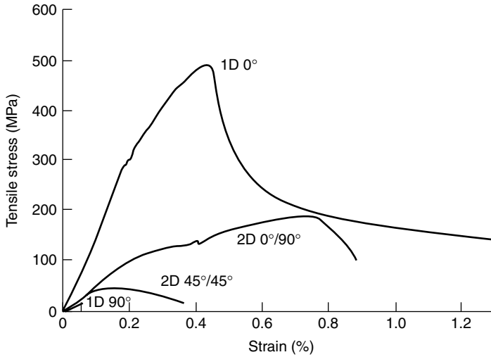
Figure 5.115 Stress-strain diagrams for lithiumaluminosilicate glass ceramic reinforced with 50% SiC fibers in various orientations. From Ceramic Microstructures , by W. E. Lee and W. M. Rainforth, p. 103. Copyright © 1994 by William E. Lee and W. Mark Rainforth, with kind permission of Kluwer Academic Publishers.
