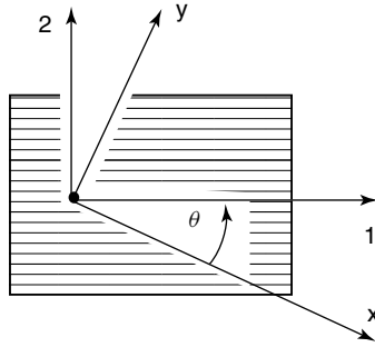
Figure 5.119 Cartesian coordinate system relative to principle fiber directions in unidirectional fiber composite. Reprinted, by permission, from P. C. Powell and A. J. I. Housz, Engineering with Polymers , p. 215. Copyright © 1998 by Stanley Thorned Publishers.
