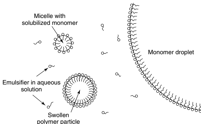
Figure 3.26 Schematic representation of micelle formation in emulsion polymerization.
