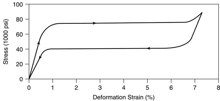
Figure 5.34 Example of superelasticity in an Ni–Ti alloy. A deformation of 7% is fully recovered. (ShapeMemory Applications, Inc.).
