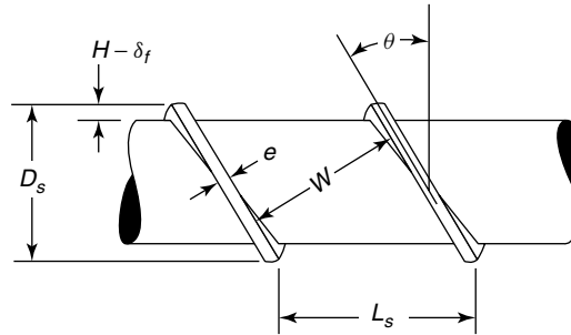
Figure 7.58 Characteristic dimensions of an extrusion screw. From Z. Tadmor and C. G. Gogos, Principles of Polymer Processing . Copyright © 1979 by John Wiley & Sons, Inc. This material is used by permission of John Wiley & Sons, Inc.
