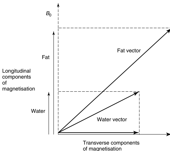
Figure 6.81 Magnitude of transverse and longitudinal magnetization for fat and water. Reprinted, by permission, from C. Westbrook and C. Kaur, MRI in Practice , 2nd ed., p. 18. Copyright © 1998 by Blackwell Science Ltd.
