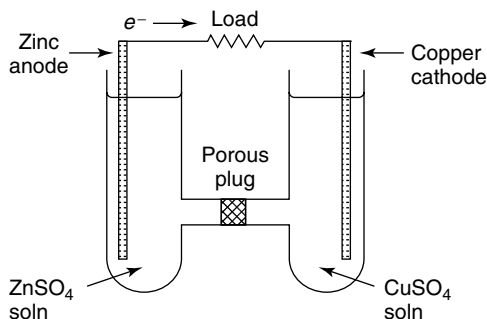
Figure 3.8 Schematic diagram of an electrochemical cell.
