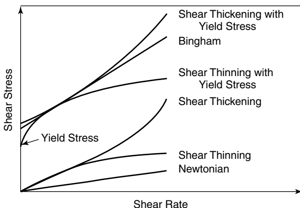
Figure 4.5 Variation of shear stress with shear rate for different models of flow behavior. From J. S. Reed, Principles of Ceramics Processing , 2nd ed. Copyright © 1995 by John Wiley & Sons, Inc. This material is used by permission of John Wiley & Sons, Inc.
