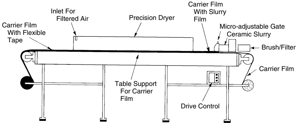
Figure 7.31 Schematic diagram of a typical tape-casting process. From Principles of Ceramics Processing , 2nd edition, by J. S. Reed; Copyright © 1995 by John Wiley & Sons, Inc. This material is used by permission of John Wiley & Sons, Inc.
