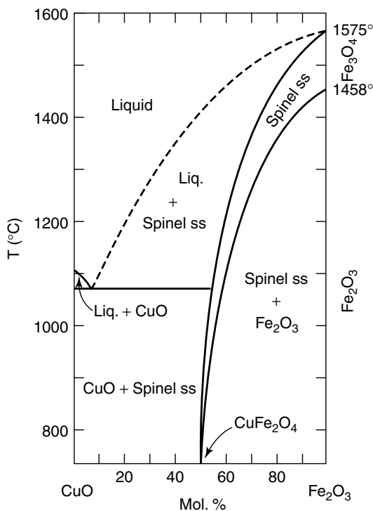
Figure 2.22 Binary component phase diagram for the system \text{CuO-Fe}_2\text{O}_3 . Reprinted, by permission, from Phase Diagrams for Ceramists , p. 31, Fig. 2140, 1969 Supplement. Copyright © 1969 by The American Ceramic Society.
