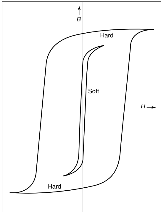
Figure 6.55 Comparison of hysteresis loops for soft and hard magnetic materials. From K. M. Ralls, T. H. Courtney, and J. Wulff, Introduction to Materials Science and Engineering . Copyright © 1976 by John Wiley & Sons, Inc. This material is used by permission John Wiley & Sons, Inc.
