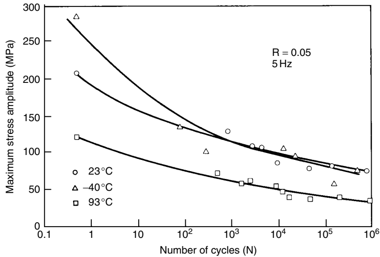
Figure 5.104 Fatigue S - N diagram for SMC-R65 composite. Reprinted, by permission, from Composite Materials Technology , P. K. Mallick and S. Newman, eds., p. 52. Copyright © 1990 by Carl Hanser Verlag.
