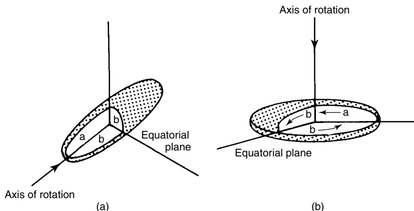
Figure 4.17 (a) Prolate and (b) oblate ellipsoids of revolution, showing the relationship between the semi-axes and the axis of revolution. Reprinted, by permission, from P. Hiemenz, Principles of Colloid and Surface Chemistry , 2nd ed., p. 26. Copyright © 1986 by Marcel Dekker, Inc.
