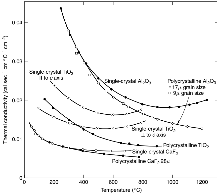
Figure 4.29 Thermal conductivity of single-crystal and polycrystalline \text{Al}_2\text{O}_3 , \text{TiO}_2 , and \text{CaF} . Multiply by 418.7 to obtain k in units of \text{W/m}\cdot\text{K} . From W. D. Kingery, H. K. Bowen, and D. R. Uhlmann, Introduction to Ceramics . Copyright © 1976 by John Wiley & Sons, Inc. This material is used by permission of John Wiley & Sons, Inc.
