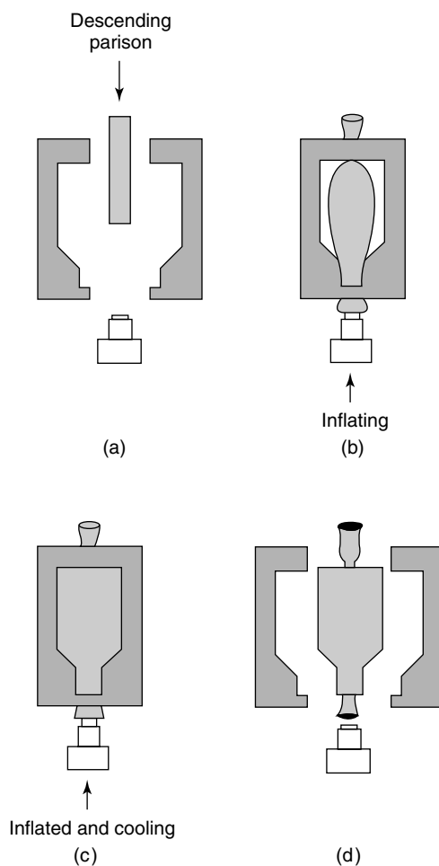
Figure 7.80 Schematic illustration of blow molding process. From Z. Tadmor and C. G. Gogos, Principles of Polymer Processing , Copyright © 1979 by John Wiley & Sons, Inc. This material is used by permission of John Wiley & Sons, Inc.
