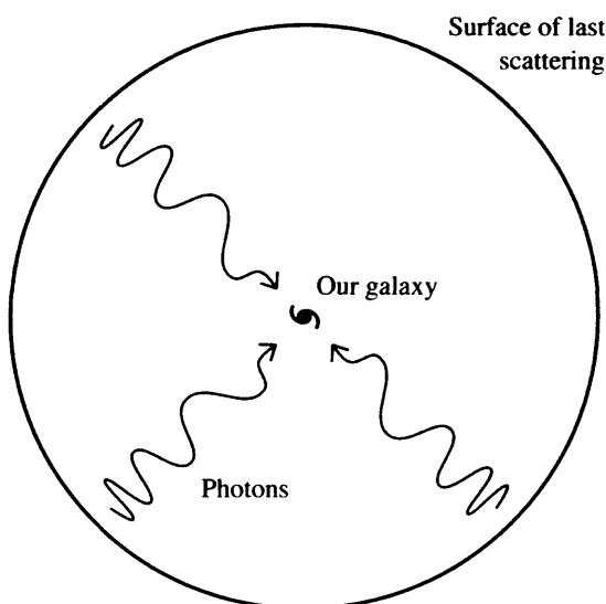
Figure 10.2 Because they have travelled towards us uninterrupted since the Universe was at 3000 K, the photons making up our microwave background originated on the surface of a sphere, known as the surface of last scattering, a considerable distance away from our own galaxy. If observers exist in other galaxies, they will see microwaves coming from the surface of a different sphere centred around their location. At the last-scattering surface, the photons had a much higher frequency, which has been redshifted as the photons travel towards us.
