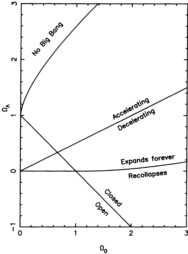
Figure 7.1 Different models for the Universe can be identified by their location in the plane showing the densities of matter and \Lambda . This figure indicates the main properties in different regions, with the labels indicating the behaviour on each side of the dividing lines.
