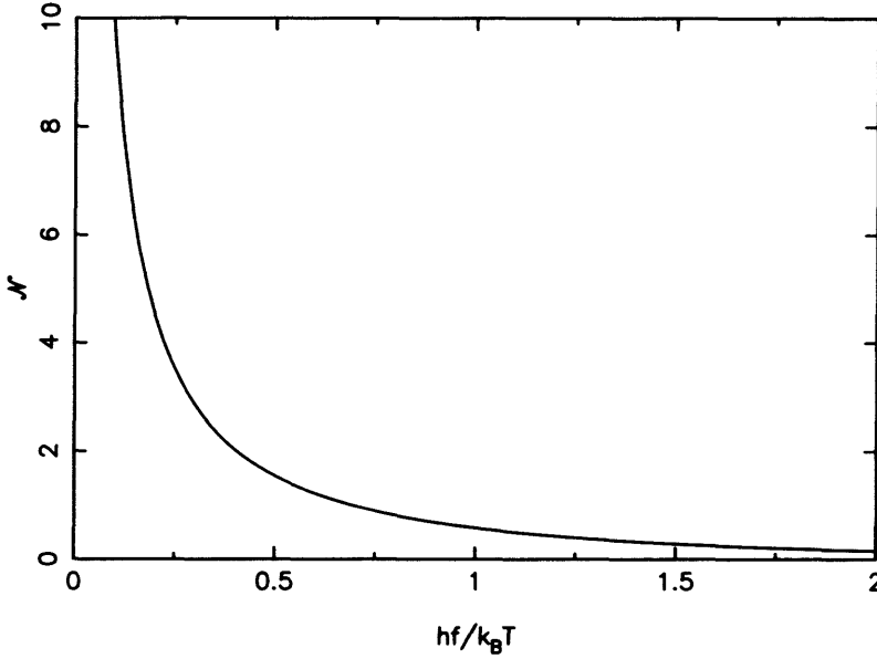
Figure 2.7 The Planck function of equation (2.7). There are far more photons with very low energy than very high energy.
