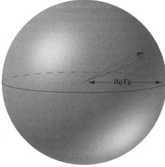
Figure A2.2 We receive light a distance a_0 r_0 from the source. The surface area of the sphere at that distance is 4\pi a_0^2 r_0^2 , and so our detector of unit area intercepts a fraction 1/4\pi a_0^2 r_0^2 of the total light output 4\pi L .
