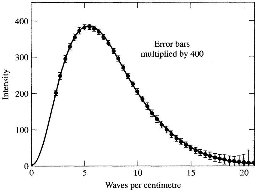
Figure 2.4 The cosmic microwave background spectrum as measured by the FIRAS experiment on the COBE satellite. The error bars are so small that they have been multiplied by 400 to make them visible on this plot, and the best-fit black-body spectrum at T = 2.725 Kelvin, shown by the line, is an excellent fit.
