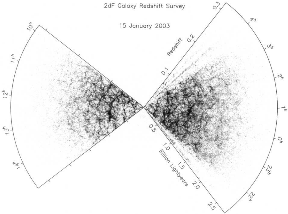
Figure A5.2 The completed 2dF galaxy redshift survey, with our galaxy located at the centre. The three-dimensional survey volume has been flattened to make this image, and the sudden angular variations indicate regions which were not surveyed. The number of galaxies is so large that projection effects make it difficult to see the structures. The radial distance indicates the redshift to the galaxy, which is independent of the underlying cosmological model, while the scale indicating distance makes particular assumptions about the cosmological model. For comparison, the CfA galaxy survey extends only to a redshift of around 0.02. [Figure courtesy Matthew Colless and the 2dFGRS Team.]
