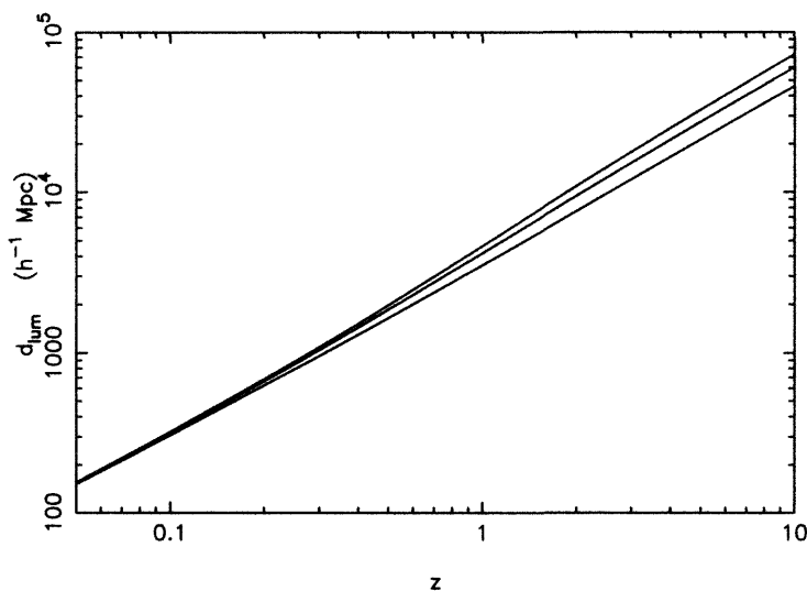
Figure A2.3 The luminosity distance as a function of redshift is plotted for three different spatially-flat cosmologies with a cosmological constant. From bottom to top, the lines are \Omega_0 = 1, 0.5 and 0.3 respectively. Notice how weak the dependence on cosmology is even to high redshift. It turns out that open Universe models with no cosmological constant have an even weaker dependence.
