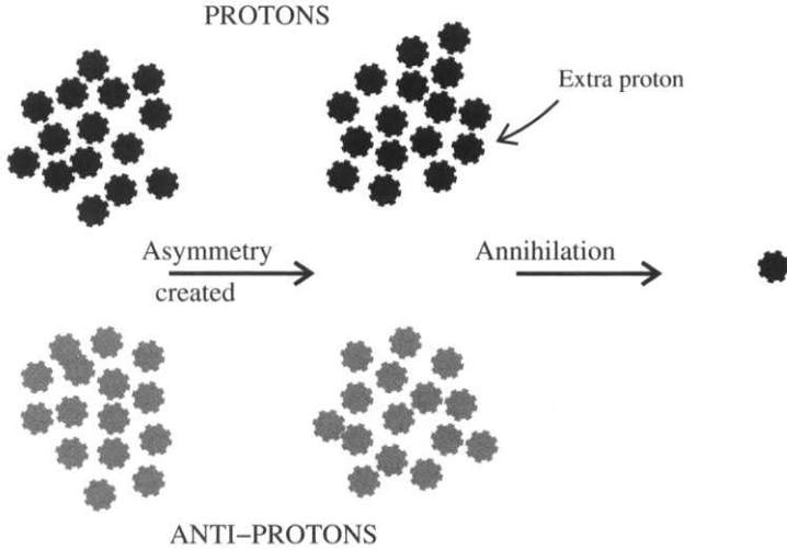
Figure A4.1 The favourite way to make a matter–anti-matter asymmetry is to do so very early, when the Universe was full of baryons and anti-baryons, by making a small excess of baryons. (I’ve contented myself with drawing fifteen rather than a billion!) Later, when the baryons and anti-baryons annihilate, the small excess is left over.
