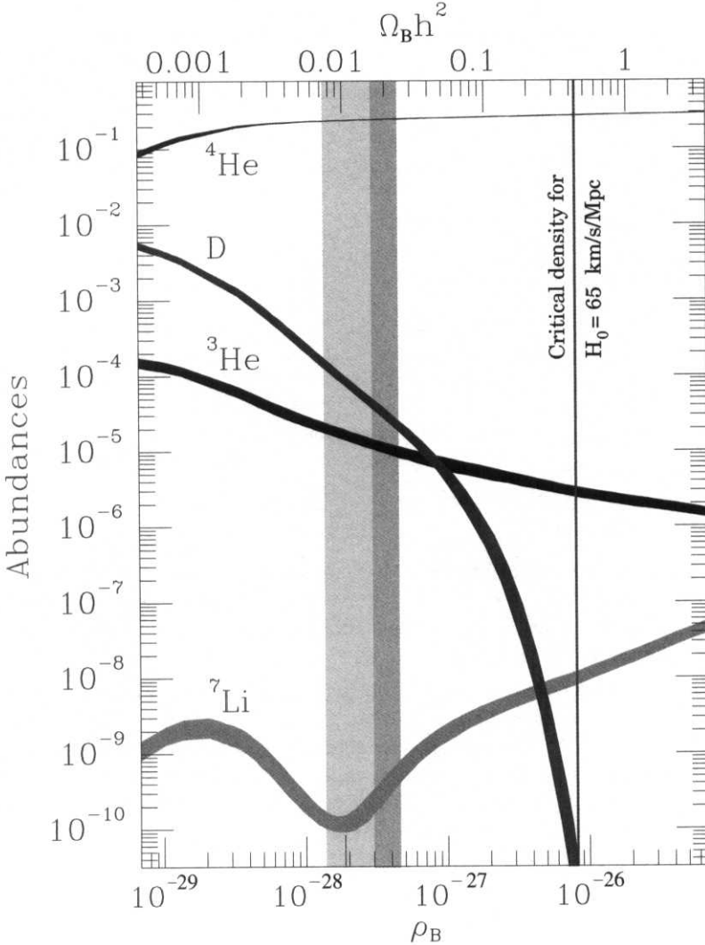
Figure 12.1 The predicted abundances of light nuclei, as a function of the absolute baryon density along the bottom or \Omega_B h^2 along the top. The width of the bands indicates the uncertainty in the predictions. The vertical bands show the range compatible with observations, while the vertical line shows the critical density. [From Schramm & Turner, Rev. Mod. Phys. 70 , 303 (1998), courtesy Michael Turner].
