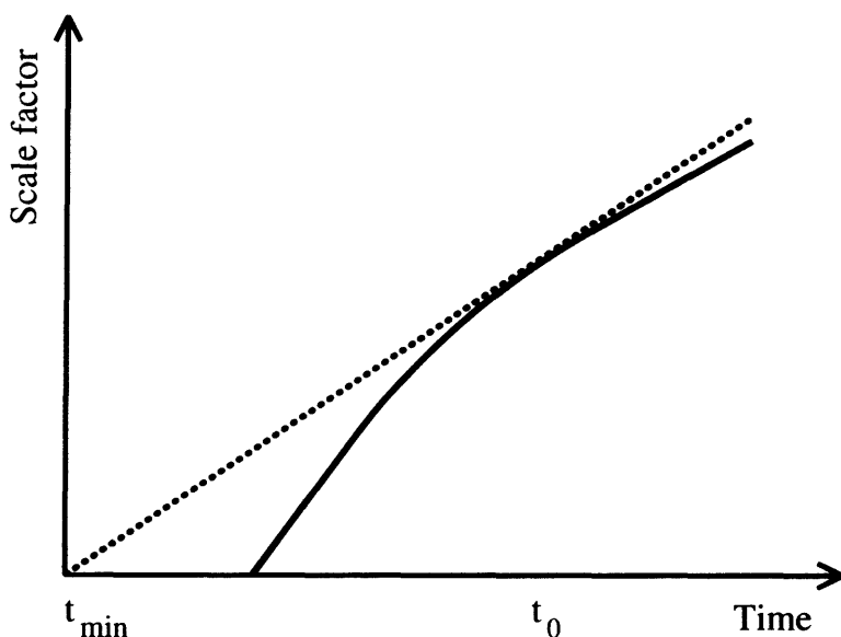
Figure 14.1 The solid line shows the true (decelerating) scale factor. The dotted line extrapolated back from the present shows the earliest possible time that the scale factor can have been zero.
