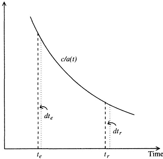
Figure A2.1 A graph of c/a(t) illustrates how the redshift law can be derived.
