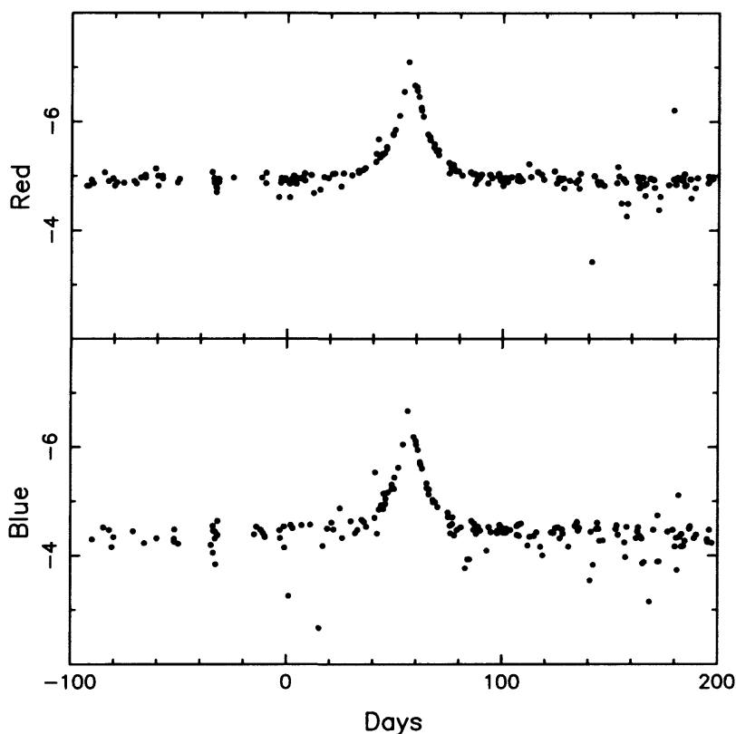
Figure 9.4 Light curves for a star in the LMC, obtained by the MACHO collaboration. The x -axis is in days with an arbitrary origin, while the y -axis shows the brightness of the star in red light and in blue light (the vertical units are a magnitude scale).
