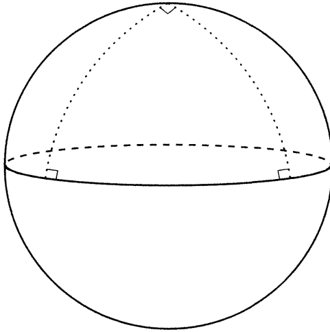
Figure 4.1 A sketch of a spherical surface, representing positive k . A triangle is shown which has three right angles!
