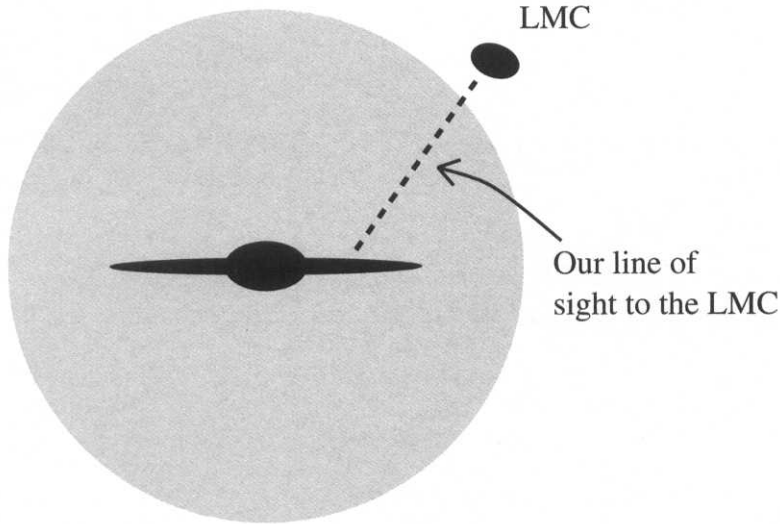
Figure 9.3 An illustration of the MACHO search strategy. We look from our position in the disk of the galaxy towards stars in the Large Magellanic Cloud. The line-of-sight passes through the dark matter halo, and if there are invisible compact objects there, and they pass extremely close to the line-of-sight, then gravitational lensing of the LMC star can occur.
