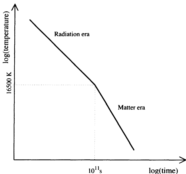
Figure 11.1 A schematic illustration of the temperature–time relation, assuming \Omega_0 = 1 and h = 0.5 . When the radiation era ends the expansion rate increases and the temperature cools more quickly.
