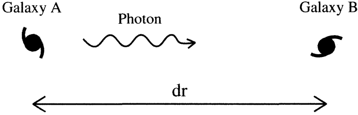
Figure 5.1 A photon travels a distance dr between two galaxies A and B.
