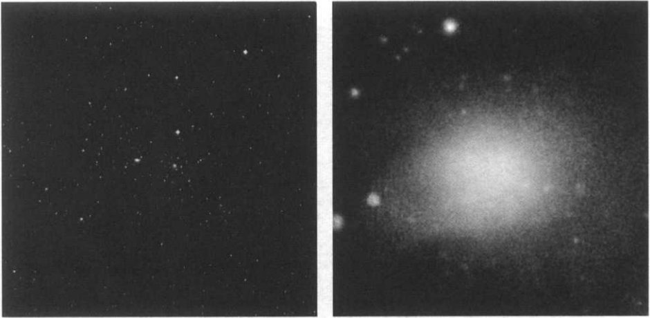
Figure 2.3 Images of the Coma cluster of galaxies in visible light (left) and in X-rays (right), on the same scale. Colour versions can be found on the book's WWW site. [Figures courtesy of the Digitized Sky Survey, ROSAT and SkyView ]
