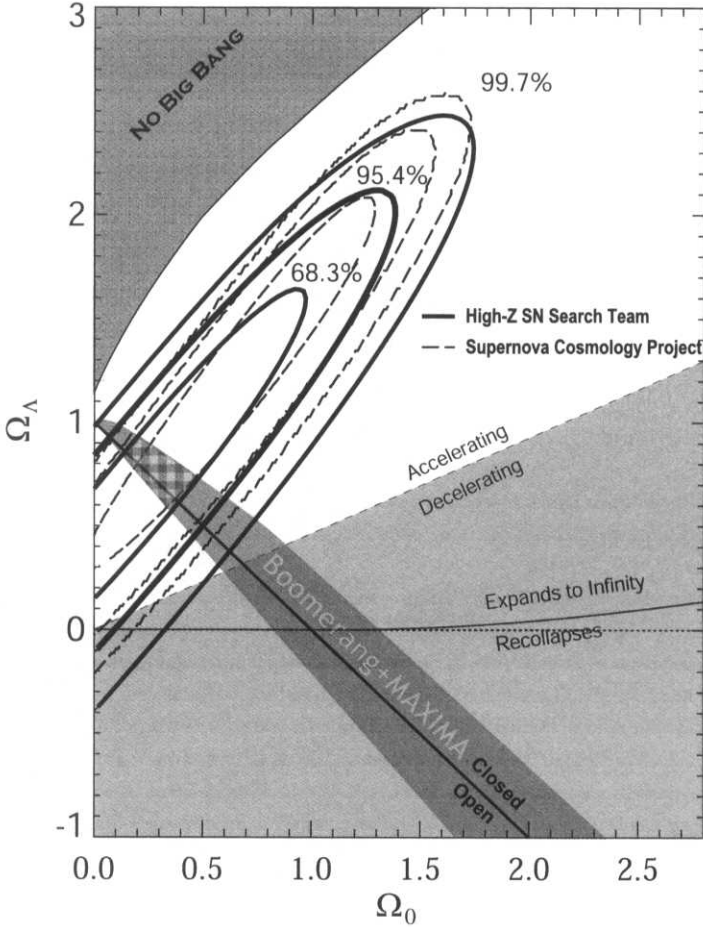
Figure A2.4 The contours show observational constraints from the supernova luminosity–redshift diagram, displayed in the \Omega_0 – \Omega_\Lambda plane as introduced in Section 7.3. Results from two separate observational programs are shown. In addition, the dark shaded region shows the part of the plane permitted by cosmic microwave background data obtained by the Boomerang and Maxima experiments, as described in Advanced Topic 5.4. Only a very small region, with \Omega_0 \simeq 0.3 and \Omega_\Lambda \simeq 0.7 , matches both data sets. [Figure courtesy Brian Schmidt.]
