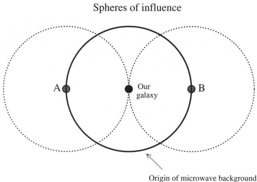
Figure 13.1 An illustration of the horizon problem. We receive microwave radiation from points A and B on opposite sides of the sky. These points are well separated and would not have been able to interact at all since the Big Bang — the dotted lines indicate the extent of regions able to influence points A and B by the present — far less manage to interact by the time the microwave radiation was released. So in the Hot Big Bang model it is impossible to explain why they have the same temperature to such accuracy.
