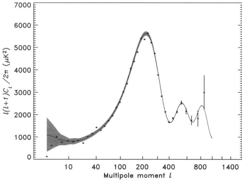
Figure A5.4 The radiation angular power spectrum as measured by the WMAP satellite, shown as the black dots. The solid line shows a theoretical prediction from their best-fit cosmological model, which fits the data extremely well. They define C_\ell using the multipoles of \Delta T itself rather than \Delta T/T , so their scale is T_0^2 = (2.725 \text{ K})^2 times that of Figure A5.3. I've drawn the figures so that their vertical axes match, but note that while Figure A5.3 uses a logarithmic \ell -axis, this plot uses a non-standard scaling along the \ell -axis chosen to display the observations evenly. [Figure courtesy NASA/WMAP Science Team.]
