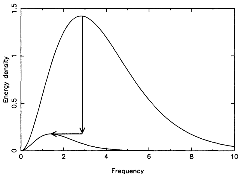
Figure 10.1 The evolution of the black-body spectrum as the Universe expands. The expansion reduces the number density of photons, while the redshifting reduces their frequency. In combination, these two effects map the spectrum onto a new black-body at a lower temperature. [The axes match Figure 2.8, using the higher temperature for each curve. The cooling is by a factor two.]
