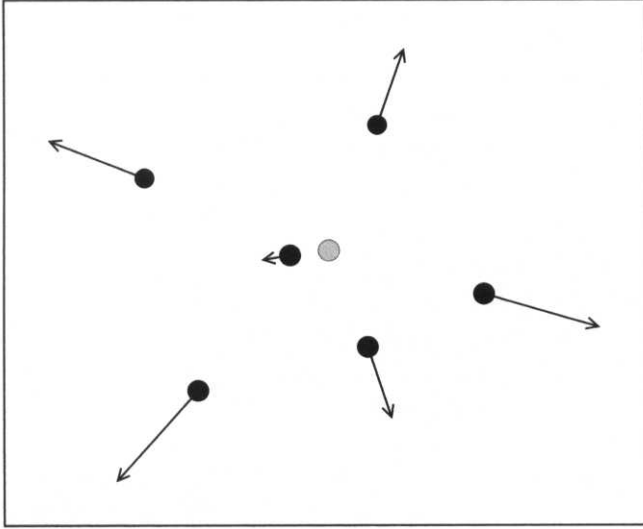
Figure 2.6 According to Hubble's law, the further away from us a galaxy is, the faster it is receding.
