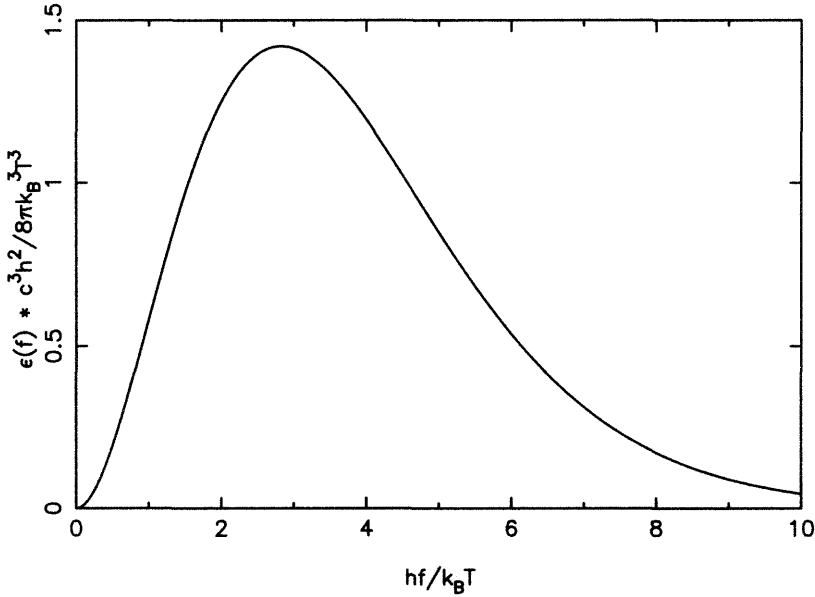
Figure 2.8 The energy density distribution of a black-body spectrum, given by equation (2.8). Most of the energy is contributed by photons of energy hf \sim k_B T .
