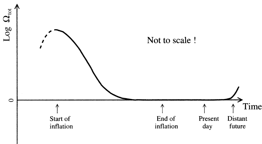
Figure 13.2 Possible evolution of the density parameter \Omega_{\text{tot}} . There might or might not be a period before inflation, indicated by the dashed line. Inflation then drives \log \Omega_{\text{tot}} towards zero (i.e. \Omega_{\text{tot}} towards 1), either from above or below. By the time inflation ends \Omega_{\text{tot}} is so close to one that all the evolution after inflation up to the present day is not enough to pull it away again. Only some time in the very distant future would it start to move away from one again.
