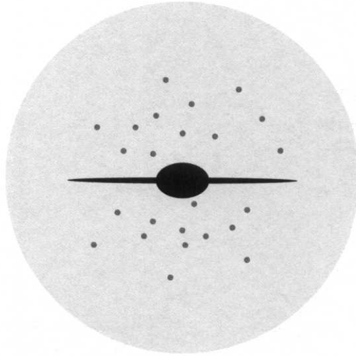
Figure 9.2 A schematic illustration of a galactic disk, with a few globular clusters, embedded in a spherical halo of dark matter.
