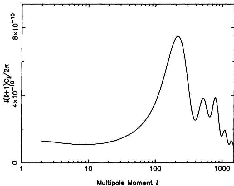
Figure A5.3 A typical prediction of cosmic microwave anisotropies, in this case for the Standard Cosmological Model. The predicted curve is calculated to better than one percent accuracy.
