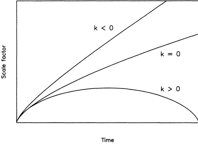
Figure 5.3 Three possible evolutions for the Universe, corresponding to the different signs of k . The middle line corresponds to the k = 0 case where the expansion rate approaches zero in the infinite future. During the early phases of the expansion the lines are very close and so observationally it can be difficult to distinguish which path the actual Universe will follow.
