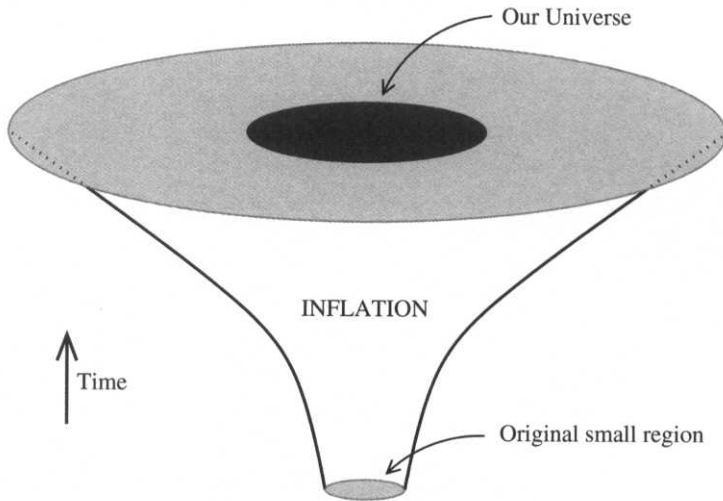
Figure 13.3 A schematic illustration of the inflationary solution to the horizon problem, with a small initial thermalized region blown up to encompass our entire observable Universe.
