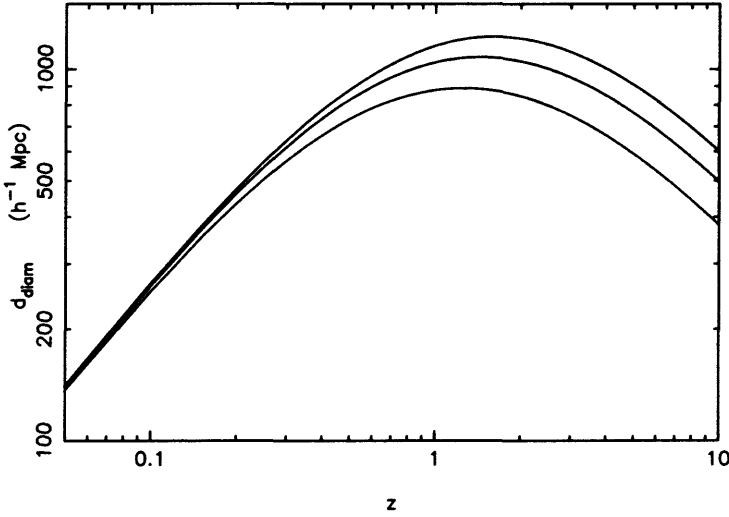
Figure A2.5 The angular diameter distance as a function of redshift is plotted for three different spatially-flat cosmologies with a cosmological constant. From bottom to top, the lines are \Omega_0 = 1, 0.5 and 0.3 respectively. For nearby objects d_{\text{diam}} and d_{\text{lum}} are very similar, but at large redshifts the angular diameter distance begins to decrease.
