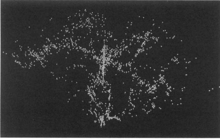
Figure 2.2 A map of galaxy positions in a narrow slice of the Universe, as identified by the CfA (Center for Astrophysics) redshift survey. Our galaxy is located at the apex, and the radius is around 200 Mpc. The galaxy positions were obtained by measurement of the shift of spectral lines, as described in Section 2.4. While more modern and extensive galaxy redshift surveys exist, this survey still gives one of the best impressions of structure in the Universe. [Figure courtesy Lars Christensen]
