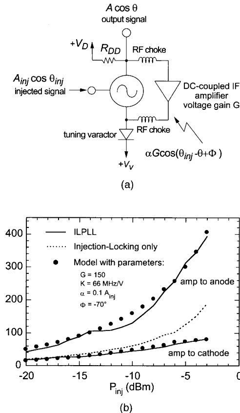
FIGURE 7.19 (a) A simplified schematic of an injection-locked phase-locked-loop (ILPLL) system using a conventional VCO with an active lowpass feedback element. (b) Measured locking characteristics for an experimental prototype at X-band.
