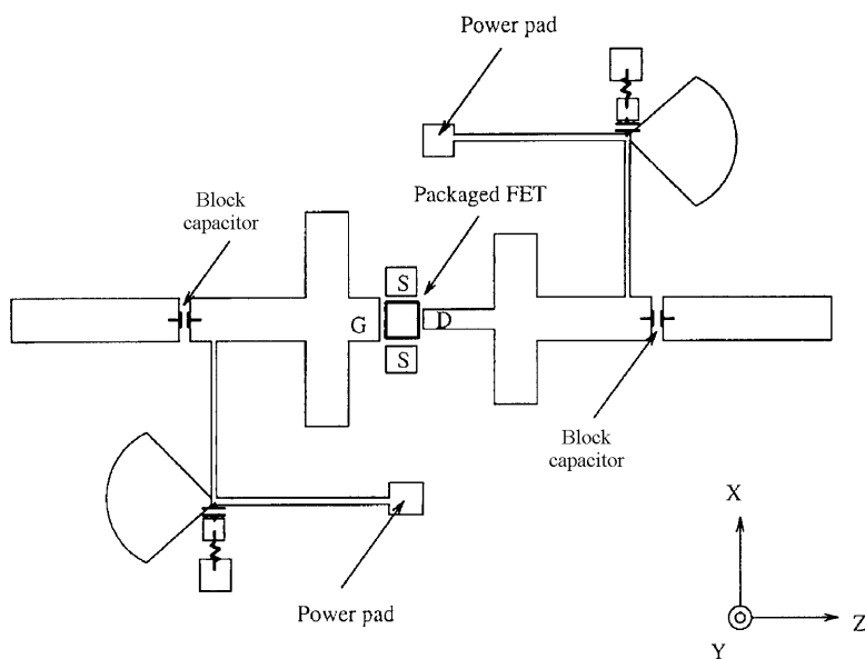
FIGURE 6.16 The layout of a microwave amplifier simulated by the extended FDTD algorithm. (From [43], copyright © 1995 by IEEE.)
