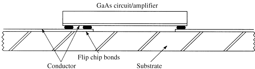
FIGURE 9.11 Flip chip mounting of power GaAs FET.
