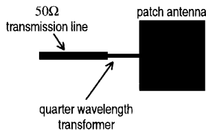
FIGURE 10.22 Simulated structure with Prelude.
