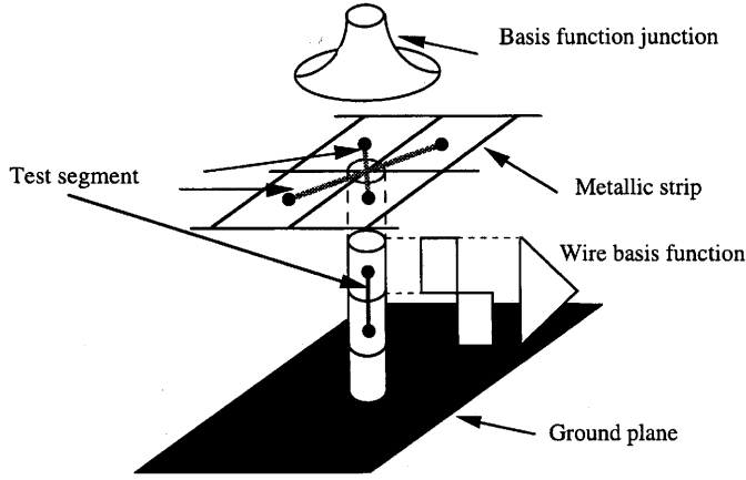
FIGURE 5.7 Strip-wire junction.
