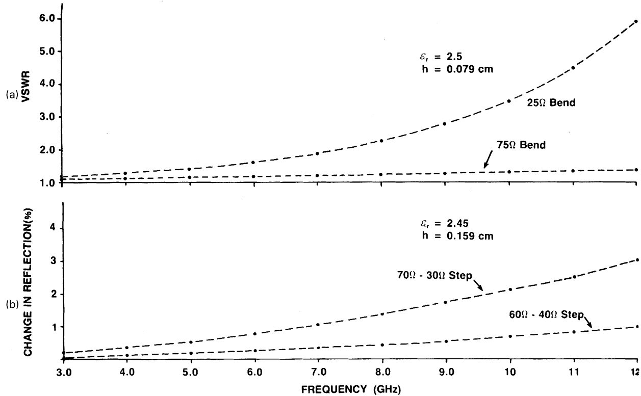
FIGURE 2.5 (a) Frequency variations of VSWR introduced by right-angled bends in 25- \Omega and 75- \Omega microstrip lines. (b) Frequency variations of the percentage changes in reflection coefficients introduced by two step discontinuities in microwave circuits. (From [16], copyright © 1988 by John Wiley & Sons; reprinted with permission.)
