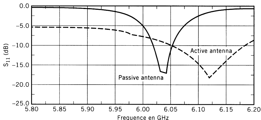
FIGURE 5.44 Input return loss.
