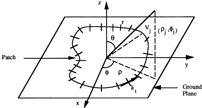
FIGURE 4.34 Patch geometry for far-field calculations.
