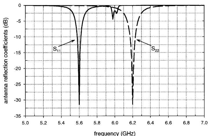
FIGURE 10.39 Reflection coefficients of the patch antenna transmit and receive ports.
