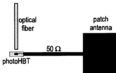
FIGURE 10.35 PhotoHBT-patch antenna integration.
