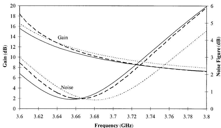
FIGURE 3.18 Gain and noise figure for three active LNA patch geometries. Insert: 9 mm (···), 7 mm (—), and 5 mm (- - -).
