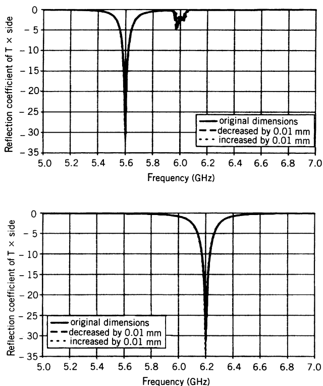
FIGURE 10.46 Fabrication tolerances on the performance of the full-duplex patch antenna.
