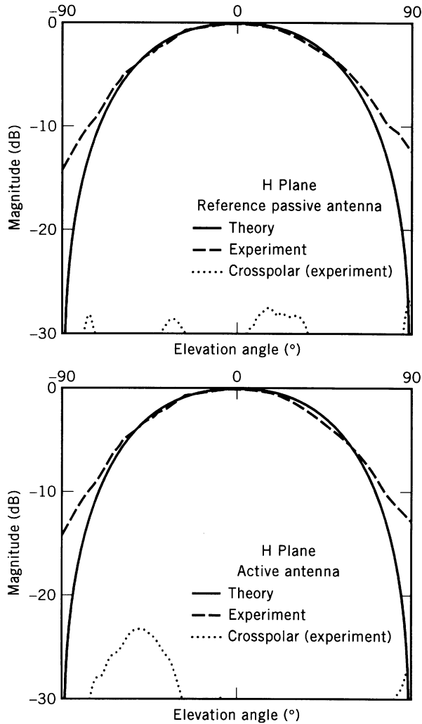
FIGURE 5.37 Radiation patterns ( H -plane).
