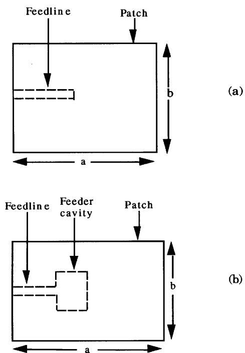
FIGURE 4.29 Feed structures for patch excitation.
