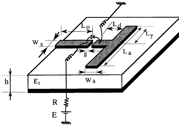
FIGURE 5.42 Active microstrip antenna loaded with a diode. ( W_s = 2.4 mm, L_0 = 47.7 mm, L_d = 2.0 mm, L_y = 8.0 mm, g = 0.3 mm, L_a = 17.45 mm, W_a = 2.2 mm, h = 0.8 mm, \epsilon_r = 2.17 , R = 10 \Omega .)
