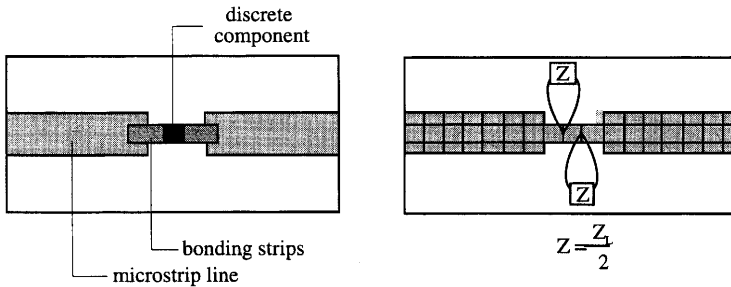
FIGURE 5.28 Discrete element with associated interconnections.
