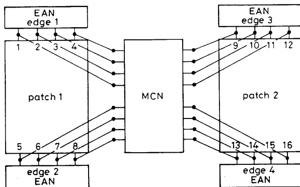
FIGURE 4.17 A mutual coupling network (MCN) representing the coupling between two adjacent patches in an array.
