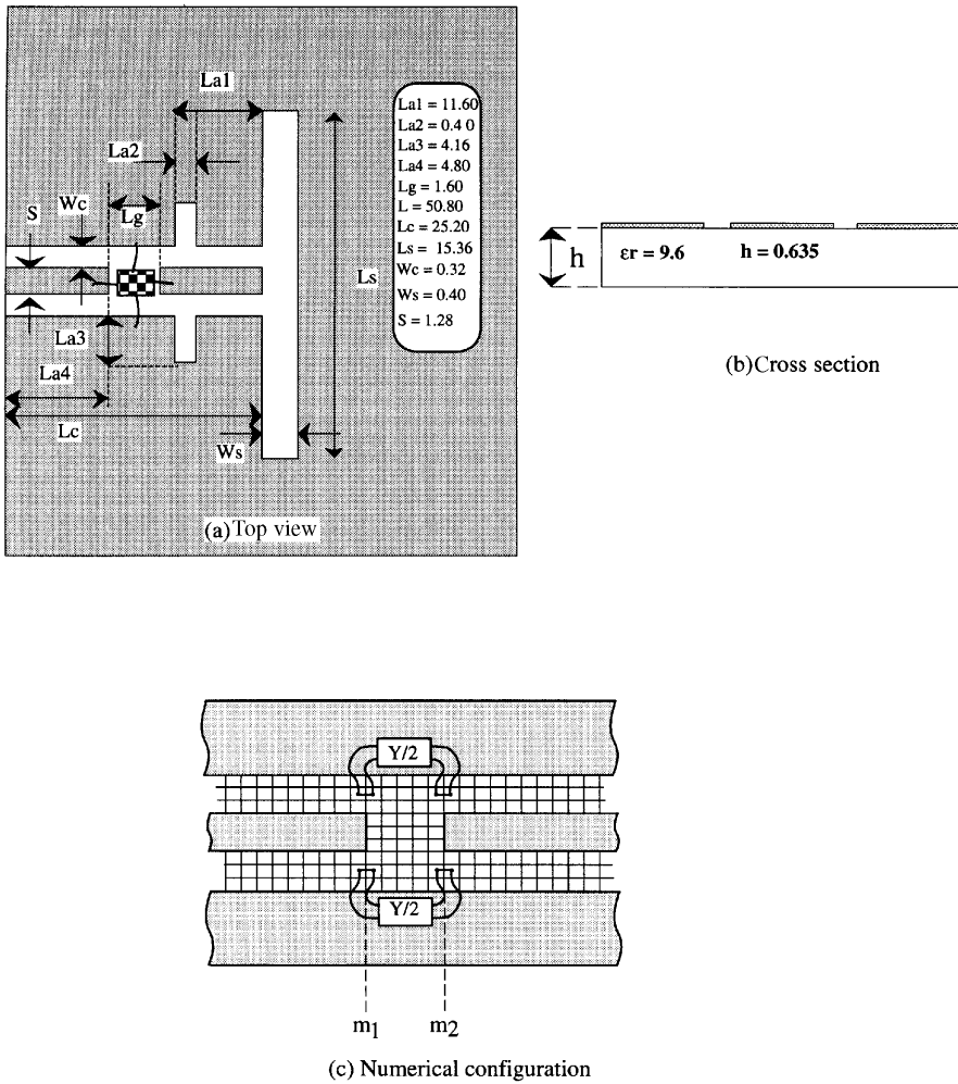
FIGURE 5.40 Uniplanar active antenna. ( L_{a1} = 11.60 mm, L_{a2} = 0.40 mm, L_{a3} = 4.16 mm, L_{a4} = 4.80 mm, L_g = 1.60 mm, L = 50.80 mm, L_c = 25.20 mm, L_s = 15.36 mm, W_c = 0.32 mm, W_s = 0.40 mm, S = 1.28 mm, \epsilon_r = 9.6 , h = 0.635 mm.)
