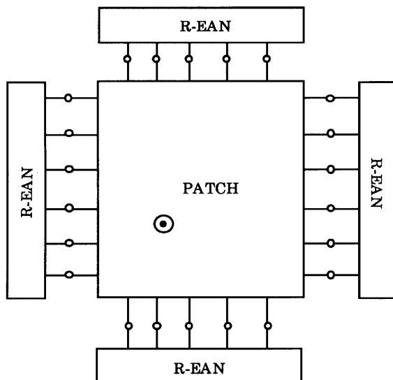
FIGURE 4.3 Edge admittance networks (EANs) connected to the multiport representation of a rectangular patch.
