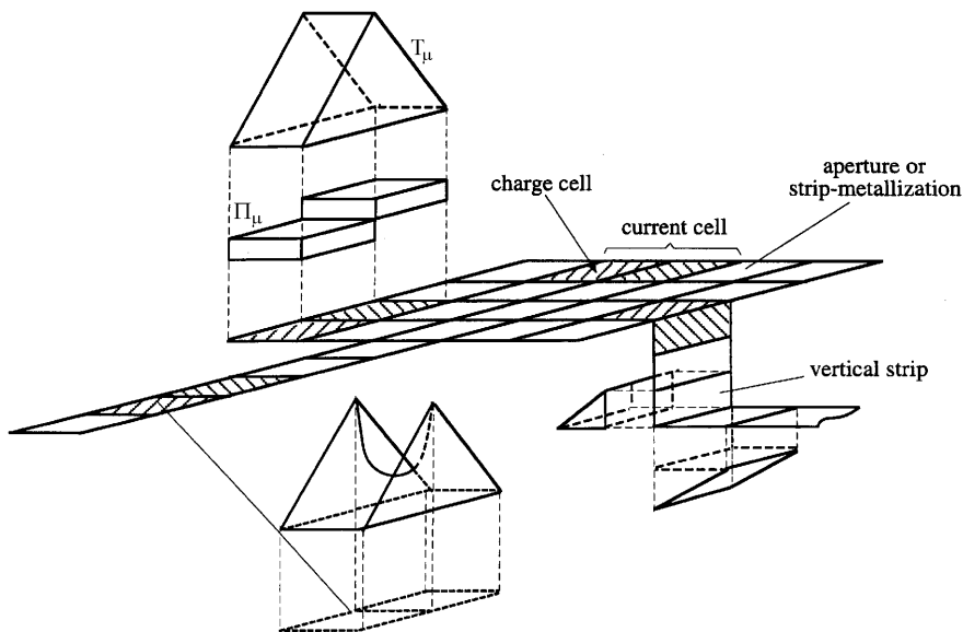
FIGURE 5.6 Current discretization and basis functions.
