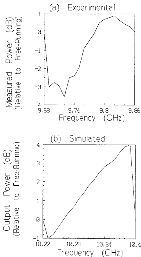
FIGURE 3.38 Injection locked active antenna output power. Bias tee input level = -2\ \text{dBm} . (From [50], reprinted with permission of John Wiley & Sons.)
