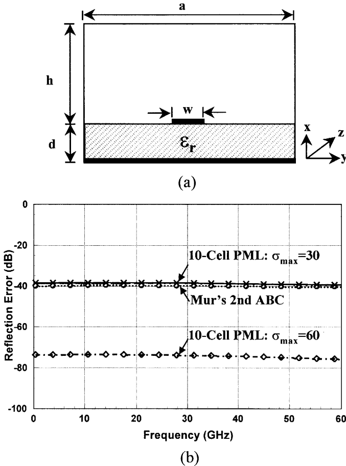
FIGURE 6.6 (a) FDTD simulation model of a shielded microstrip line and (b) reflection errors caused by Mur's second-order ABC and PML with two different conductivity values.
