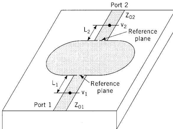
FIGURE 6.7 A general two-port microwave circuit.
