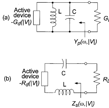
FIGURE 7.3 (a) Parallel-equivalent oscillator model; (b) series-equivalent oscillator model.
