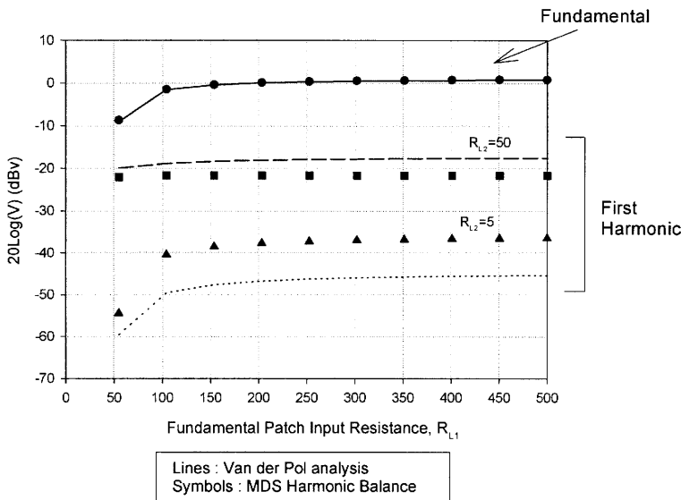
FIGURE 3.37 Output voltages of microstrip patch oscillator using dual LCR circuit (Fig. 3.35b). Values as in Fig. 3.36; L_1 = 0.2 \text{ nH} , C_2 = 20 \text{ pF} , L_2 = 0.05 \text{ nH} , and R_{Li} = 1/G_{Li} .
