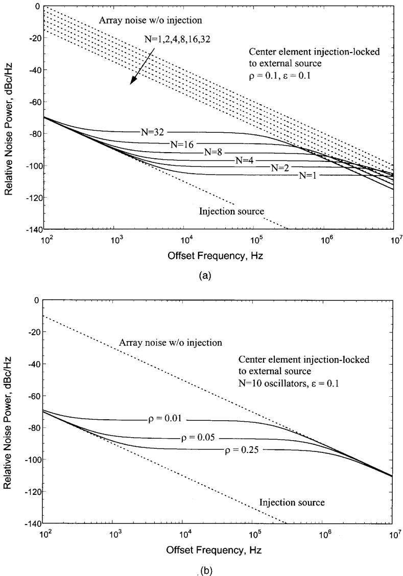
FIGURE 7.16 Spectral characteristics of the phase noise in an array with the center element injection-locked (Fig. 7.13b) for (a) Several array sizes, both with (solid lines) and without (dotted lines) the injected signal (the noise characteristics degrade with increasing array size); and (b) Several injection strengths, for the specific case of N = 10 .
