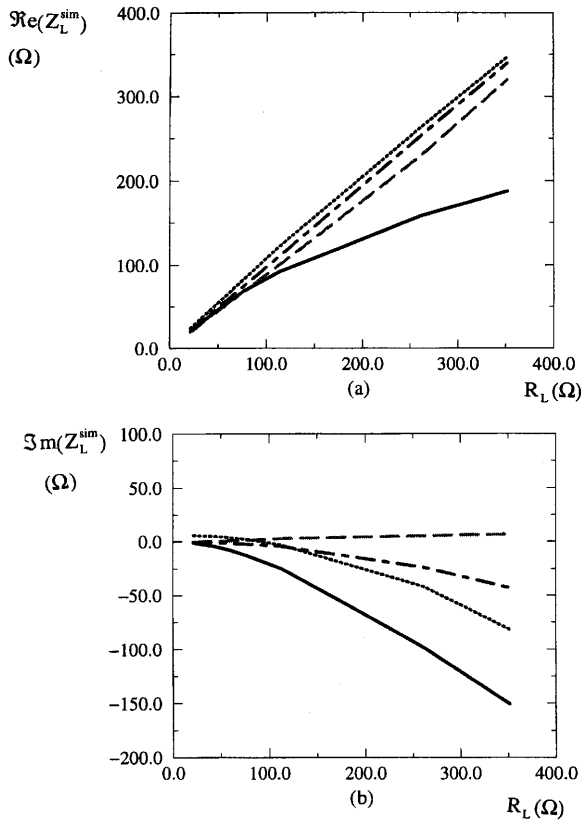
FIGURE 5.26 Simulated impedance versus inserted impedance: —, noncorrected results; - - -, corrected results (first modeling); - · -, corrected results (second modeling); · · ·, HP-EEsof results. From [43], copyright © 1998, reprinted with permission of IEEE.
