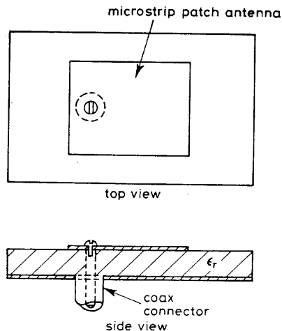
FIGURE 4.8 Microstrip patch antenna with a probe feed perpendicular to the substrate.
