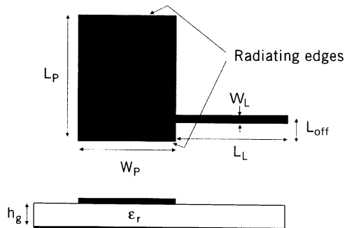
FIGURE 3.9 Nonradiating edge-fed microstrip patch antenna. L_p = 24.0 mm, W_p = 20.0 mm, L_{\text{off}} = 5.0 mm, W_L = 1.57 mm, h = 0.508 mm and \epsilon_r = 2.2 .
