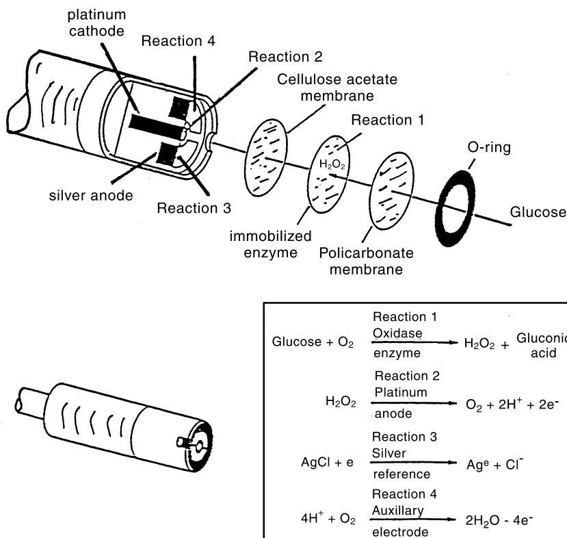
FIGURE 6-4 Schematic of a “first-generation” glucose biosensor (based on a probe manufactured by YSI Inc.).
