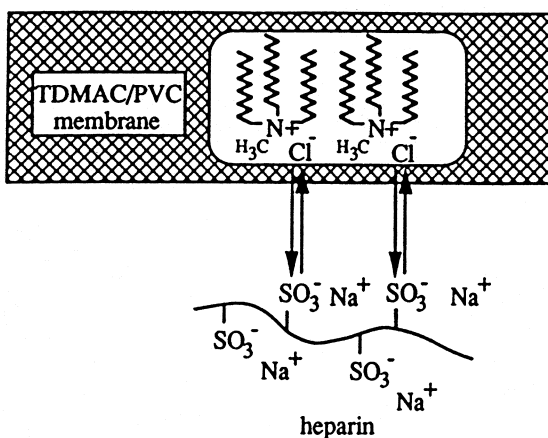
FIGURE 5-11 The recognition process occurring at the TDMAC/PVC membrane/sample interface used for measurements of heparin. (Reproduced with permission from reference 26.)
