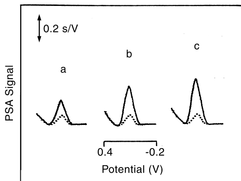
FIGURE 6-14 DNA hybridization biosensors: detection of DNA sequences from the E. coli pathogen. Chronopotentiometric response of the redox indicator upon increasing the target concentration in 1.0 µg/ml steps (a–c), in connection with a 2 min hybridization time. (Reproduced with permission from reference 46.)
