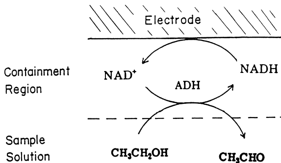
FIGURE 6-10 Reagentless ethanol bioelectrode.
