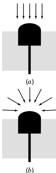
FIGURE 1-3 Planar (a) and spherical (b) diffusional fields at spherical electrodes.
