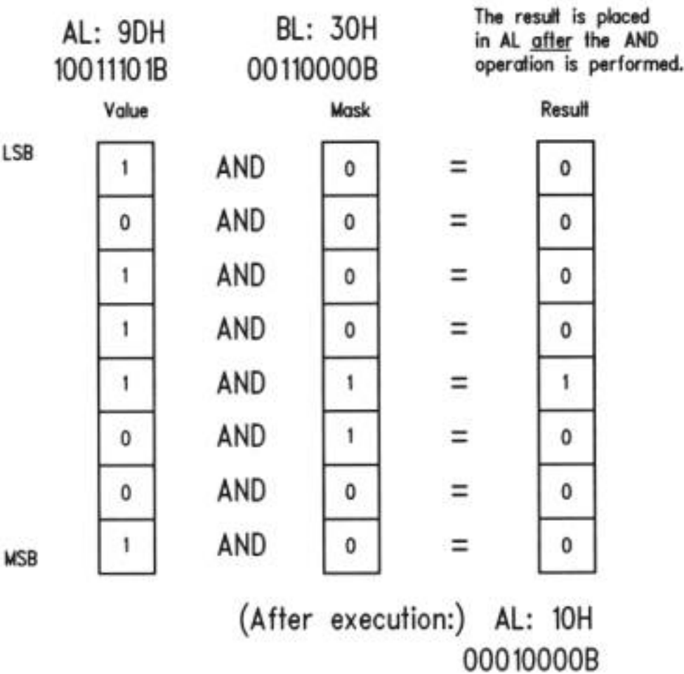
Figure 9.2. The Anatomy of an AND instruction AND AL,BL
