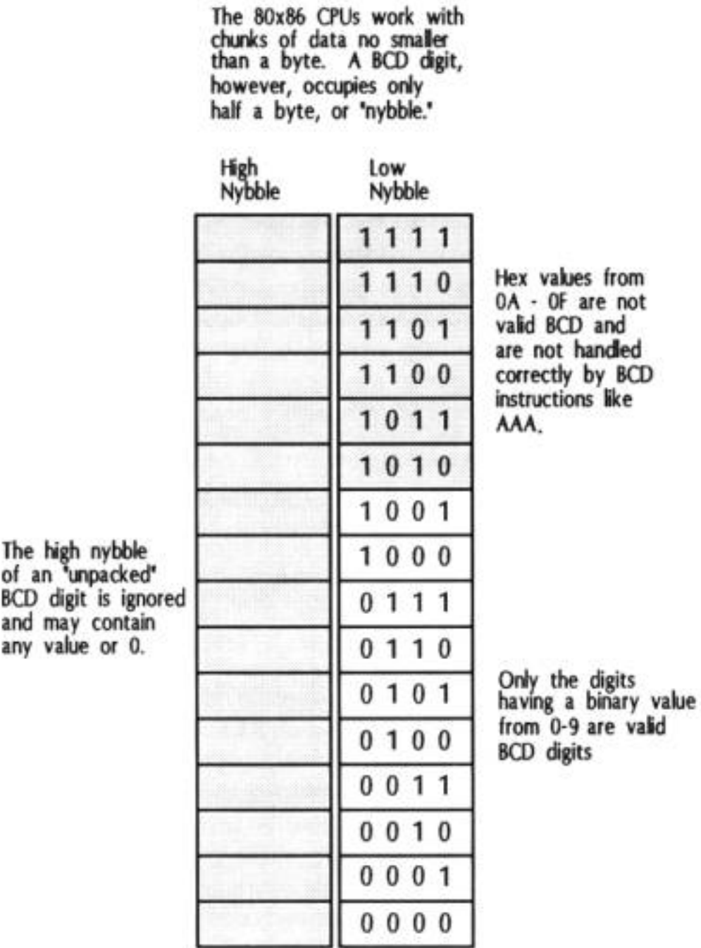
Figure 10.1. Unpacked BCD digits
