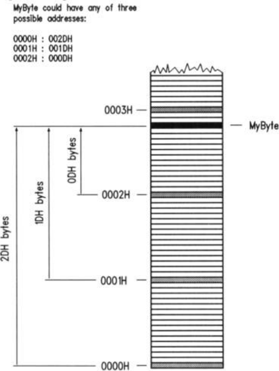
Figure 5.3. Segments and offsets
