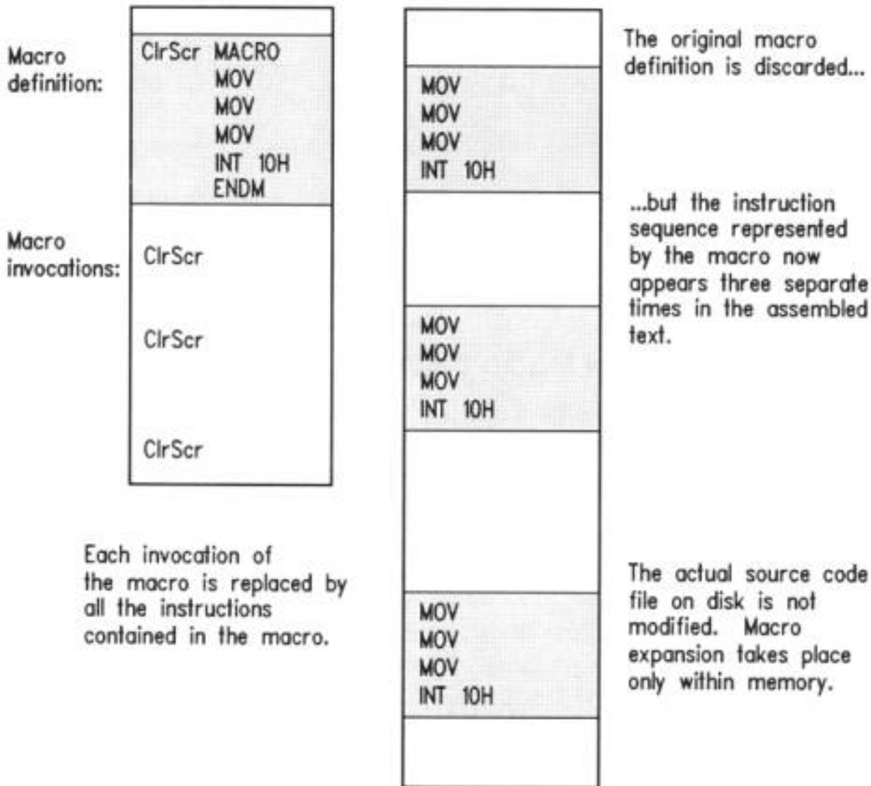
Figure 8.3. How macros work The source code file presented to the assembler:
