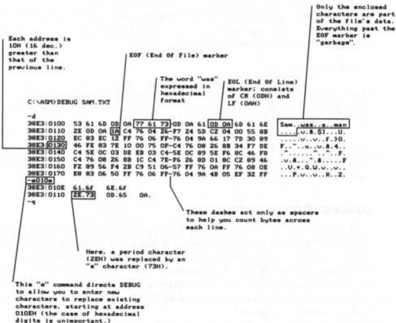
Figure 3.6. Hex dump of SAM.TXT
