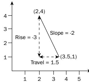
Figure 18-10: A line with a negative slope.
