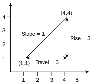
Figure 18-9: A line with a slope of 1.
