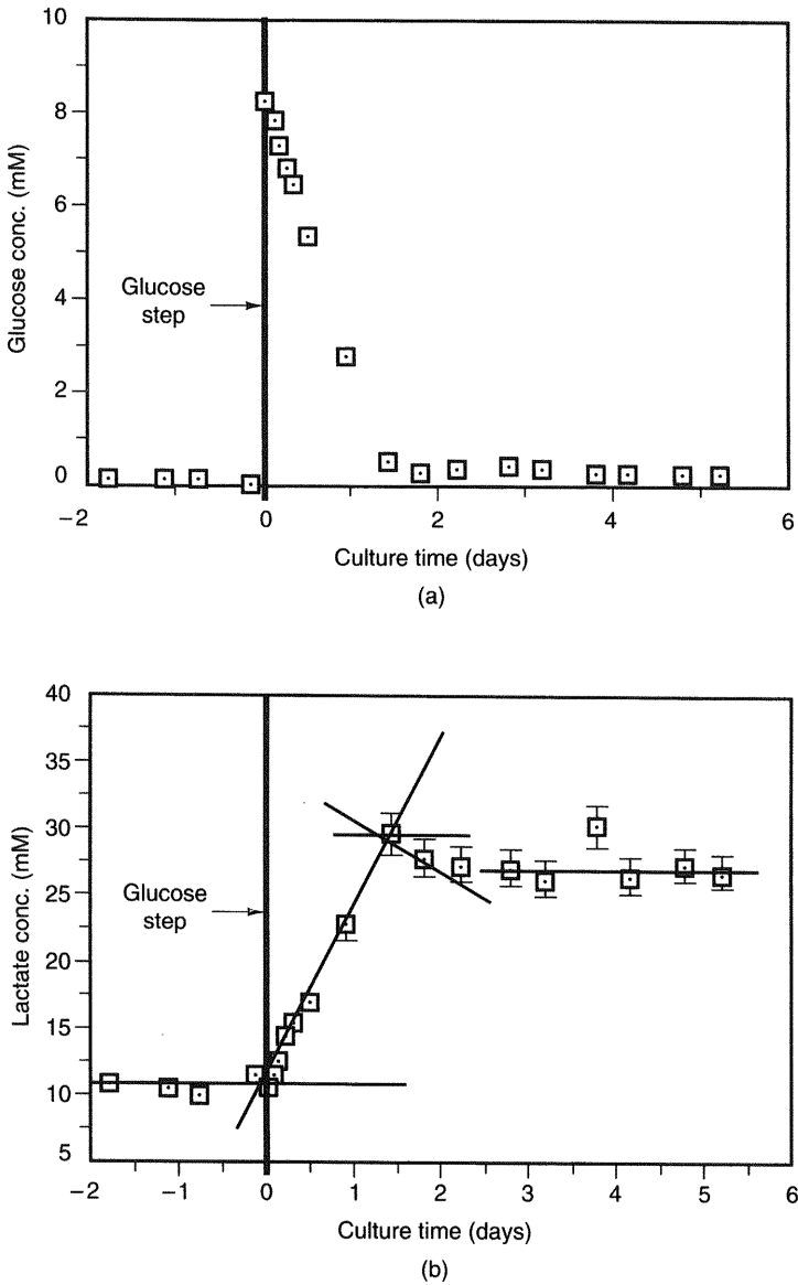
Figure 4.2.5 Glucose step change continuous culture experiment. Initial feed glucose concentration was 5.2 mM. At time zero the feed glucose concentration was increased to 13.8 mM and the reactor glucose concentration was increased to 8.3 mM. The reactor dilution rate was maintained at 0.54 day -1 throughout the experiment. (a) Glucose concentration (mM) as a function of culture time. The estimated error is \pm 0.02 g l -1 based on the variability of a 2 g l -1 glucose standard and phosphate-buffered saline (PBS) control. (b) Lactate concentration (mM) as a function of culture time. Tangent lines are shown for slope determination. Error bars represent the standard deviation based on a standard curve. Adapted from Miller et al. (1989) by permission of Biotechnology and Bioengineering .
