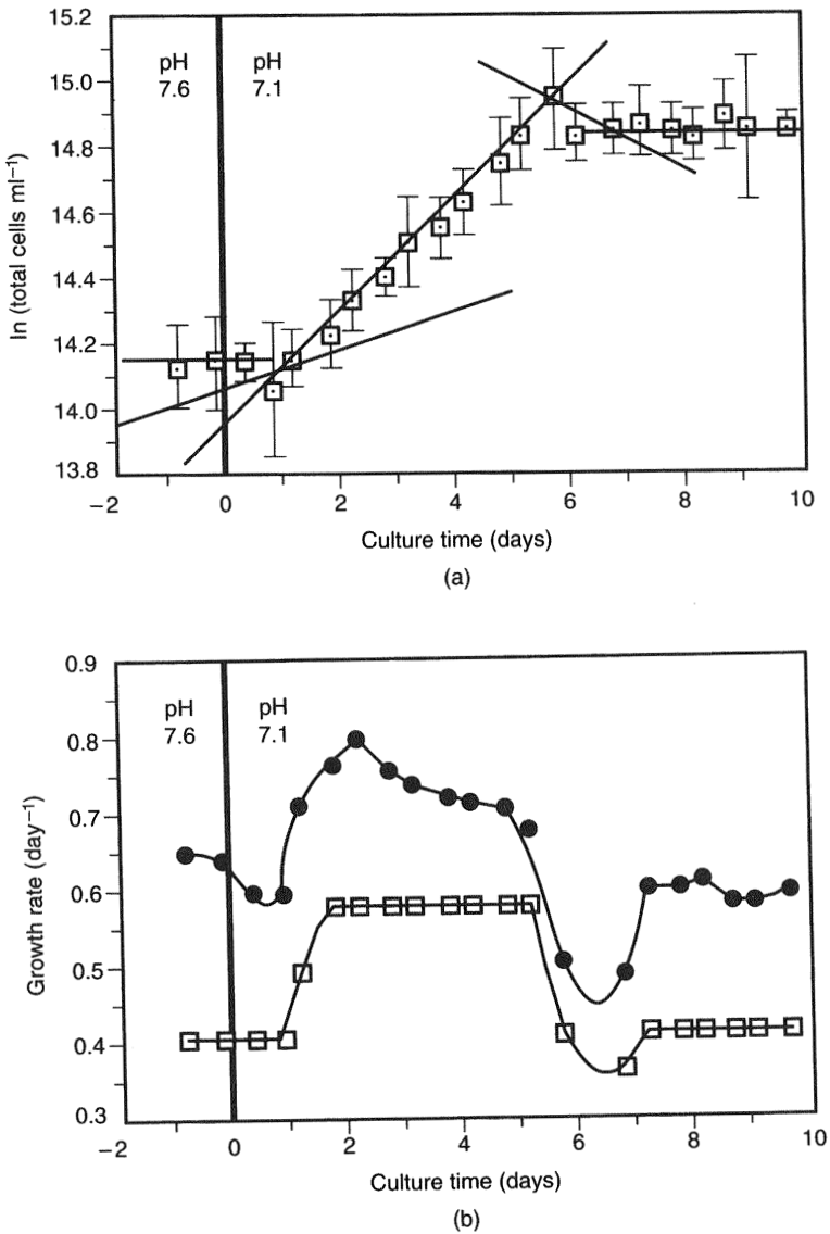
Figure 4.2.2 A pH step change continuous culture experiment. The reactor pH was decreased from 7.6 to 7.1 at time zero. The dilution rate was maintained at 0.41 \text{ day}^{-1} throughout the experiment. (a) Natural logarithm of total cell concentration versus culture time. Tangent lines are shown for slope determination. Error bars represent the standard deviation based on four replicate cell counts. (b) Apparent ( \mu_{app} , \square ) and true ( \mu , \bullet ) specific growth rates calculated from (a) and Equations 4.2.7 and 4.2.8. Adapted from Miller et al. (1988) by permission of Biotechnology and Bioengineering .
