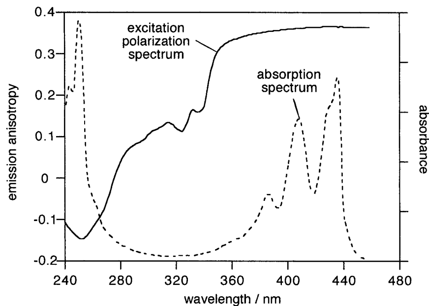
Fig. 5.8. Excitation polarization spectrum of perylene in propane-1,2-diol at -60^{\circ}\text{C} .
