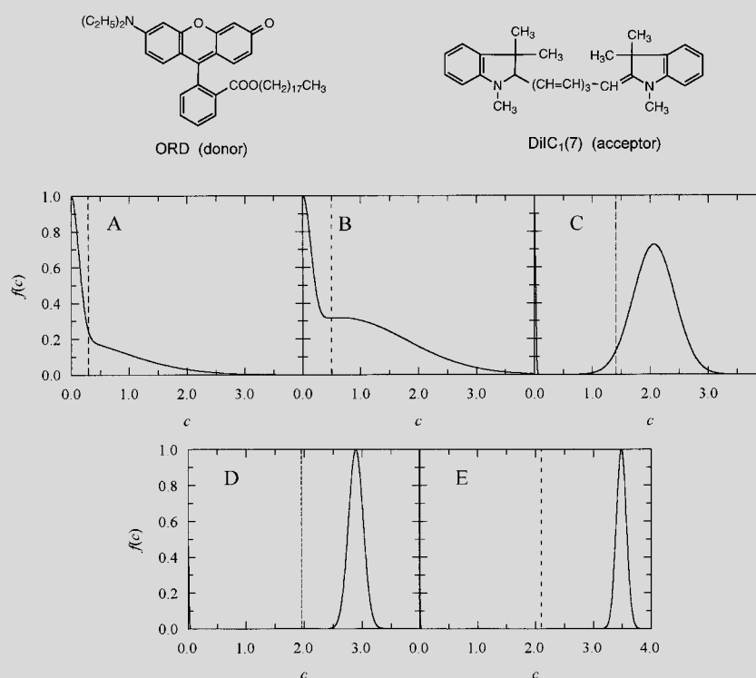
Fig. B9.2.1. Concentration distributions of acceptor [DiIC 1 (7)] obtained from the analysis of the donor (ORD) decay curves in the gel phase DPPC LUV (25 °C) in the presence of different amounts of acceptor (ratio DiIC 1 (7) to outer leaflet DPPC: A, 0.0022; B, 0.0044; C, 0.0082; D, 0.0126; E, 0.0171). The vertical broken lines represent the concentration values recovered with a model of discrete exponentials. C_2 is set at 0 (isolated donors). (Reproduced with permission from Lova et al. 3) )
