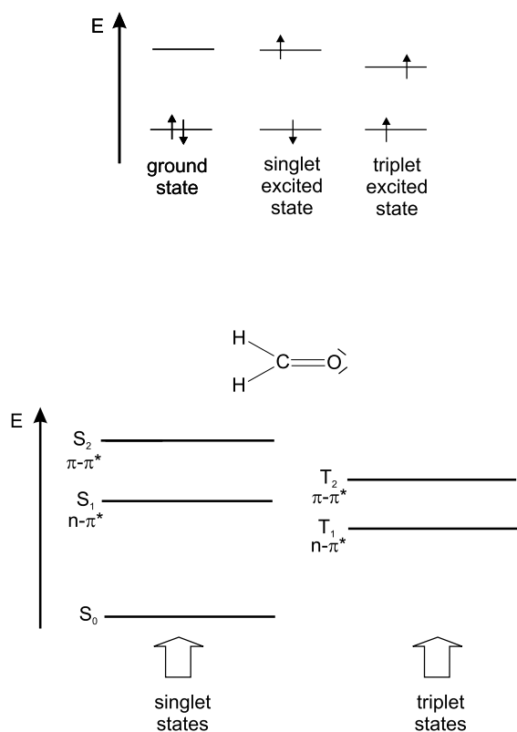
Fig. 2.2. Distinction between singlet and triplet states, using formaldehyde as an example.
