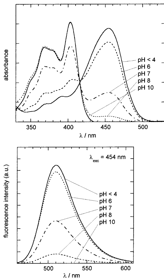
Fig. 10.4. pH dependence of the excitation and emission spectra of pyranine around neutral pH.
