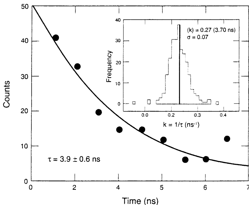
Fig. 11.15. Fluorescence decay of a single molecule of rhodamine 110. The estimated lifetime is 3.9 \pm 0.6 \text{ ns} . Repetitive measurements on several hundreds of single molecules lead to a value of 3.7 \pm 0.1 \text{ ns} , in
