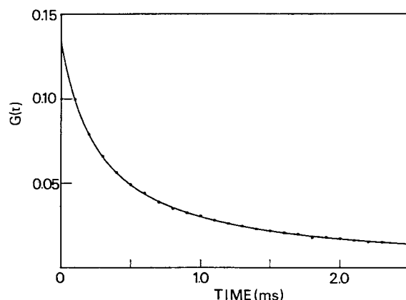
Fig. 11.12. Autocorrelation function for rhodamine 6G 10^{-9} M in ethanol. The best fit (solid line) yields D_t \cong 3 \times 10^{-6} \text{ cm}^2 \text{ s}^{-1} (reproduced with permission from Thompson, 1991).
