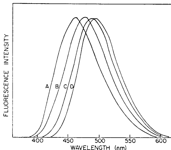
Fig. 7.3. Time-resolved fluorescence spectrum of 4-aminophthalimide at -70^{\circ}\text{C} in n -propanol. A: 4 ns; B: 8 ns; C: 15 ns; D: 23 ns (from Ware, 1971).
