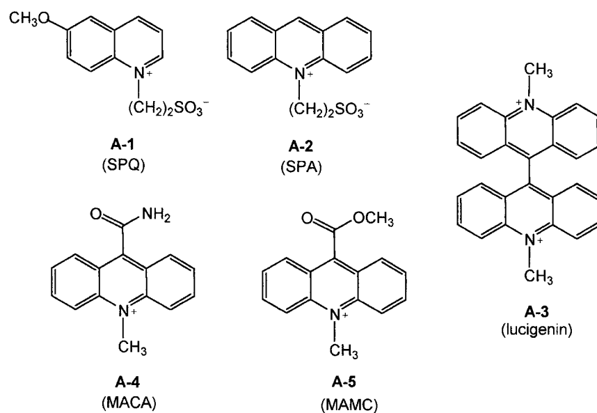
Fig. 10.29. Halide ion sensors (A-1 to A-5: Biwersi J. et al. (1994) Anal. Biochem. 219 , 139.
