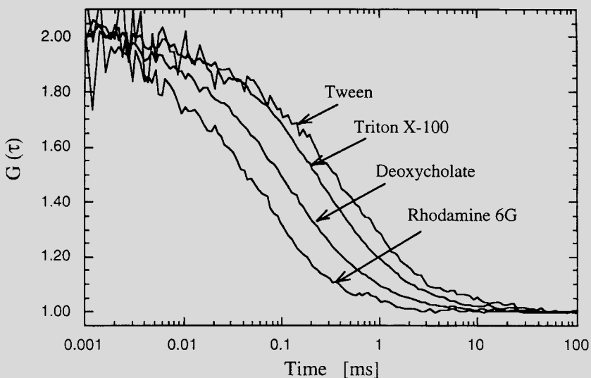
Fig. B11.2.1. Autocorrelation curves for Rhodamine 6G and various micelles loaded with ODBR (reproduced with permission from Hink and Visser a ).
