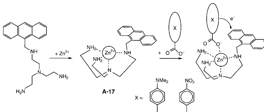
Fig. 10.35. Recognition of carboxylate ions by a complex of an anthrylamine with \text{Zn}^{\text{II}} (De Santis G. et al. (1996) Angew. Chem. Int. Ed. 35 , 202).
