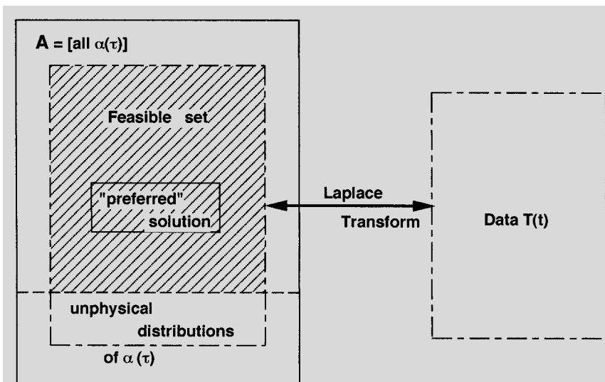
Fig. B6.1.1. The feasible set (hatched) in which MEM will choose a 'preferred' solution (redrawn from Livesey and Brochon 91 ).
