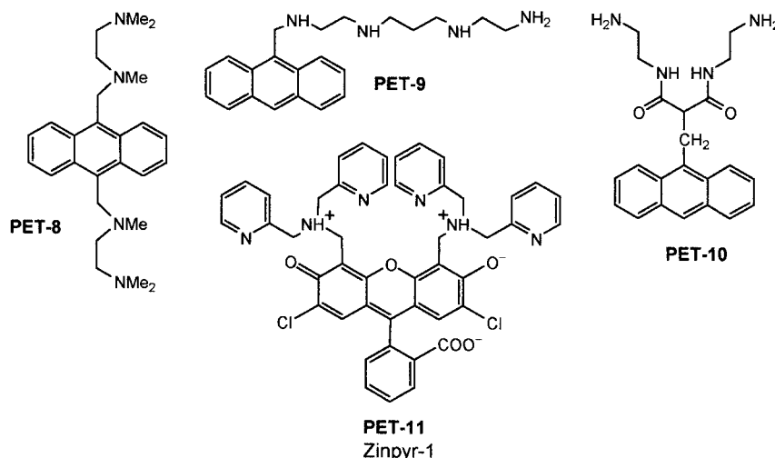
Fig. 10.13. Polyamine-based PET sensors (PET-8: Huston M. E. et al. (1988) J. Am. Chem. Soc. 110 , 4460. PET-9: Fabbri L. et al. (1996) Inorg. Chem. 35 , 1733. PET-10: Fabbri L. et al. (1994) Angew. Chem., Int. Ed. Engl. 33 , 1975. PET-11: Walkup G. K. et al. (2000) J. Am. Chem. Soc. 122 , 5644).
