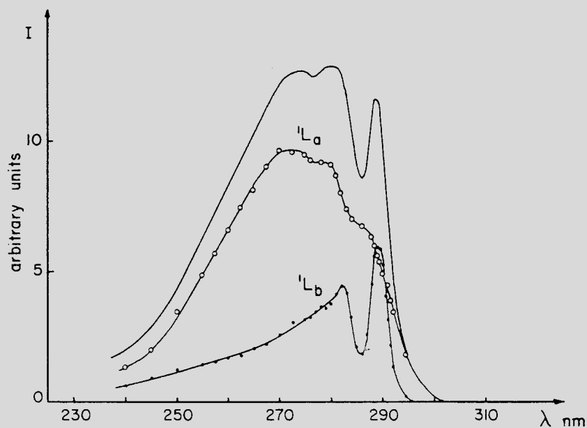
Fig. B5.2.2. Resolution of the excitation spectrum of indole (reproduced with permission from Valeur and Weber 41 ).
