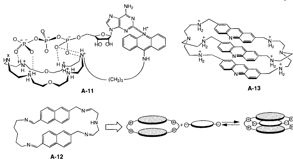
Fig. 10.33. Anion sensors based on protonated polyazamacrocycles and polyazamacrobicycles (A-11: Hosseini M. W. et al. (1988) J. Chem. Soc., Chem. Commun. 596. A-12: Dhaenens M. et al. (1993) J. Chem. Soc., Perkin Trans. 2 , 1379. A-12: Teulade-Fichou M.-P. et al. (1996) J. Chem. Soc., Perkin Trans. 2 , 2169).
