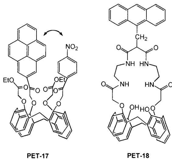
Fig. 10.15. Calixarene-based PET sensors (PET-17: Aoki I. et al. (1992) J. Chem. Soc., Chem. Commun. 730. PET-18: Unob F. et al. (1998) Tetrahedron Lett. 39 , 2951).
