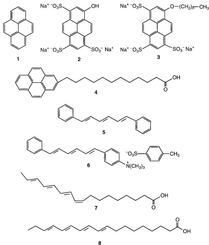
Fig. 1.5. Examples of hydrophobic, hydrophilic and amphiphilic probes. 1: pyrene. 2: 8-hydroxypyrene-1,3,6-trisulfonic acid, trisodium salt (pyranine). 3: 1-alkoxypyrene-1,3,6-trisulfonic acid, trisodium salt. 4: 1-pyrenedodecanoic acid. 5: 1,6-diphenyl-1,2,5-hexatriene (DPH). 6: 1-(4-trimethylammoniumphenyl)-6-phenyl-1,3,5-hexatriene, p -toluenesulfonate (TMA-DPH). 7: cis -parinaric acid. 8: trans -parinaric acid.
