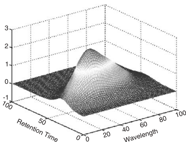
Figure 3.2. Plot of the synthetic 2D data matrix of three chemical components with white noises (see Fig. 3.3 for details).
