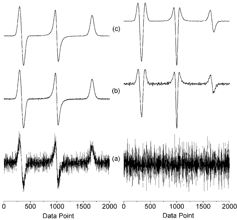
Figure 5.41. The first- (left column) and second- (right column) order derivatives of the simulated noisy signal calculated by CWT with the Haar wavelet and the scale parameter a = 1 (a), 20 (b), and 50 (c).
