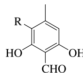
R = H: atranol R = Cl: chloroatranol
