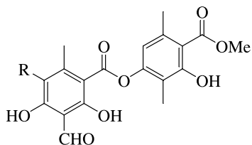
R = H: atranorin R = Cl: chloroatranorin
