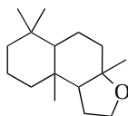
3a,6,6,9a-Tetramethyldodecahydronaphtho[2,1-b]furan [6790-58-5] (odor: ambergris)
