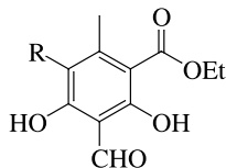
R = H: ethyl hematommate R = Cl: ethyl chlorohematommate
