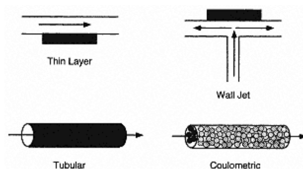
Fig. 5.1. Amperometric cells for flow analysis.
