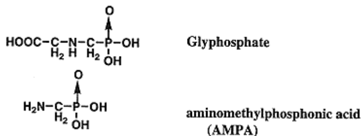
Fig. 2.15. Glyphosate and its metabolite, AMPA.
