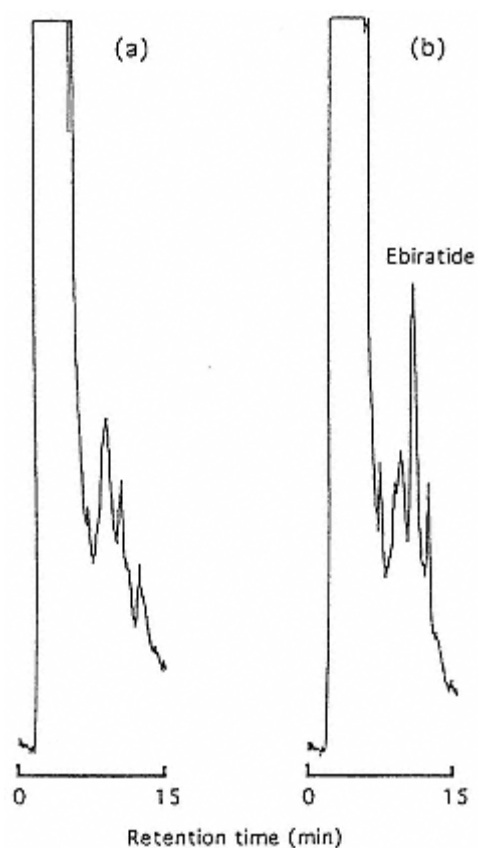
Fig. 3.15. Chromatograms obtained with: (a) rat plasma; and (b) ebiratide-spiked rat plasma (1 nmol /ml). Column: Vydac protein and peptide column 5C18 (5 \mu m; 150 \times 4.6 mm I.D.). Mobile phase: 50 mM Na 2 HP0 4 acetonitrile (3:2, v/v). Flow-rate: 1 ml/min. [Reproduced from ref. 68, p. 219, Fig. 7.].
