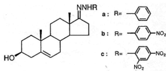
Fig. 5.15. Structures of DHEA derivatives.
