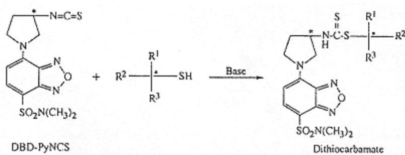
Fig. 6.43. Derivatization reaction of racemic thiols with R(-)-DBD-PyNCS. [Reproduced from ref. 219, p. 114, Fig. 2.].
