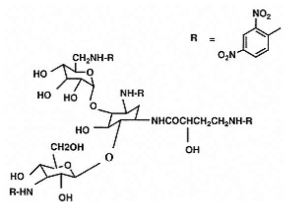
Fig. 2.1. 2,4-Dinitrophenyl derivative of amikacin.
