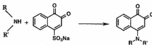
Fig. 2.10. The reaction of sodium NQS with amines.
