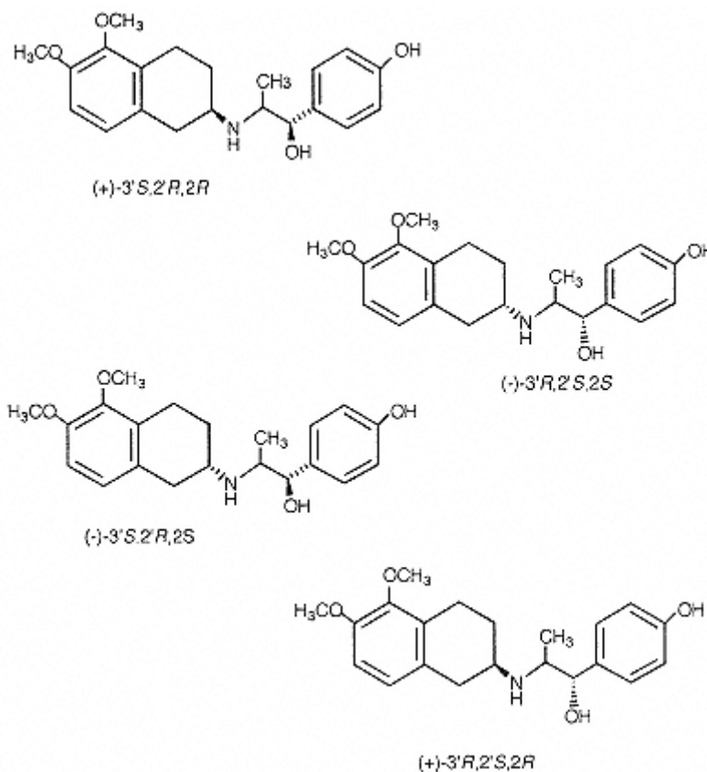
Fig. 5.7. Structures of stereoisomers of aminotetralin.
