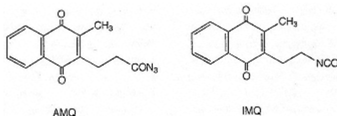
Fig. 5.14. Structures of AMQ and IMQ.
