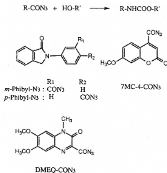
Fig. 3.44. Fluorescence labeling reagents with azide and their reaction with alcohols.
