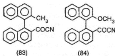
Fig. 6.39. Chiral axis reagents for alcohols by HPLC: (83) (aS)-2'-methyl-1,1'-binaphthalene - 2-carbonyl cyanide (methyl-BNCC); (84) (aS)-2'-methoxy -1,1'-binaphthalene- 2-carbonyl cyanide (methoxy-BNCC).
