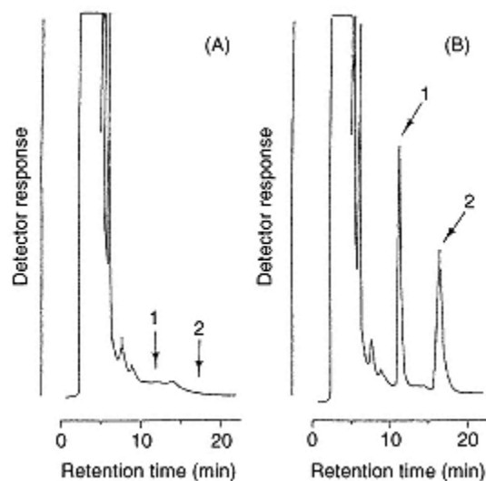
Fig. 3.11. Chromatograms obtained from: (A) drug-free plasma; and (B) plasma spiked with amantadine. Peaks: 1 = amantadine; 2 = (1-adamantyl)ethylamine (IS). Column: YMC-PackC8 (5 \mu m; 250 \times 4.6 mm I.D.). Mobile phase: methanol-acetonitrile-water (35:35:30, v/v). Flow-rate: 1 ml/min. [Reproduced from ref. 49, p. 470, Fig. 4].
