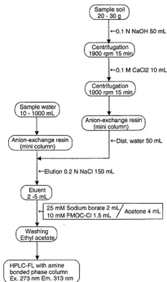
Fig. 1.3.13. Procedures for determination of glyphosate and aminomethyl phosphoric acid in soil and water developed by Glass et al. [39].
