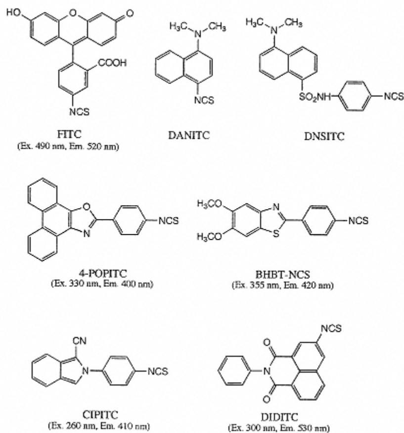
Fig. 3.12. Edman's reagents.
