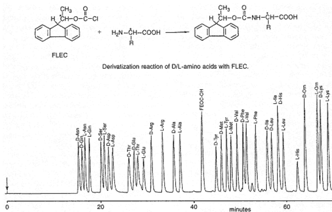
Fig. 6.30. Separation of standard L- and D- amino acids derived from (+)-FLEC. [Reproduced from ref. 154, p. 1194, Fig. 5.].
