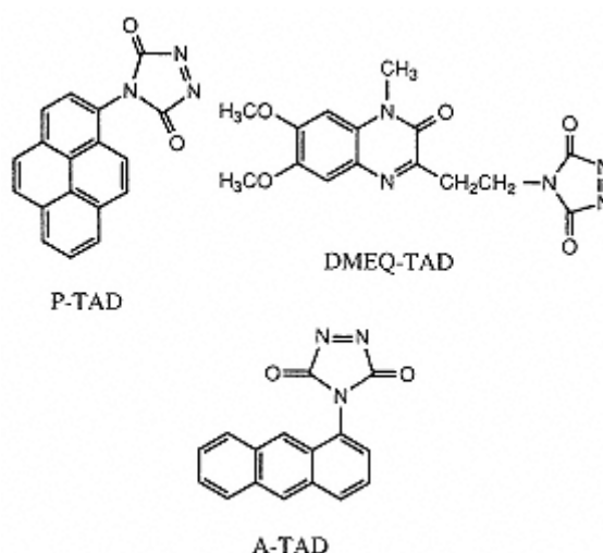
Fig. 3.61. Cookson-type fluorescence labeling reagents for dienes.
