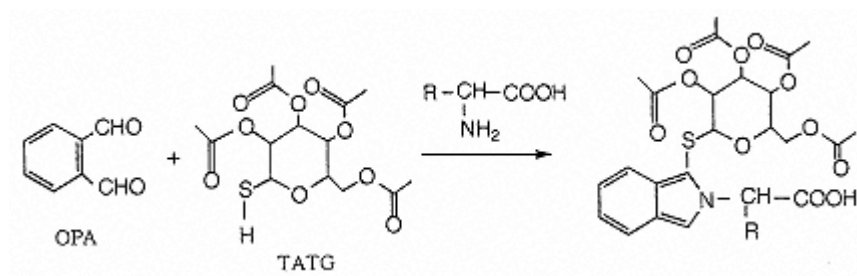
Fig. 5.3. Reaction of amino acid and OPA/TATG.
