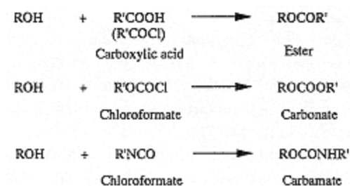
Fig. 6.11. Derivatization reactions for diastereomer formation of optically active hydroxyls.
