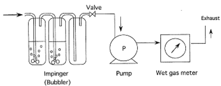
Fig. 1.3.2. Scheme of sampling device for solution-trapping method.
