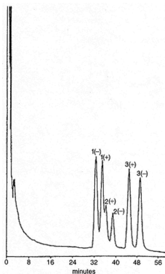
Fig. 6.14. GC separation of \pm -fenchyl alcohol (1); (\pm) -neomenthol (2); and (\pm) -menthol (3). [Reproduced from ref. 10, p. 898, Fig. 4.].
