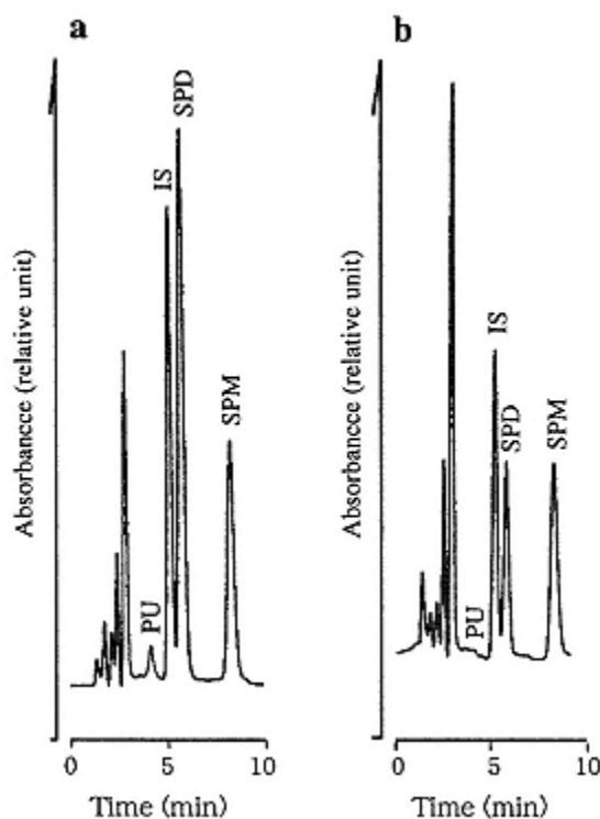
Fig. 2.11. Chromatograms of benzoylated polyamines from PC-93 tumour tissue grown in nude mice, monitored by their absorbance at 229 nm. Elution with
