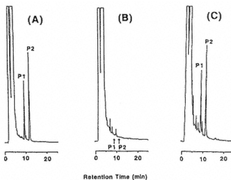
Fig. 1.2.11. High-performance liquid chromatograms of progesterone standard 2 ng (A), beef (B) and fortified beef as 20 ppb progesterone (C). (Reproduced from ref. 203: J. Food Hyg. Soc. Japan, (1995) 36, p. 599, Fig. 6.).
