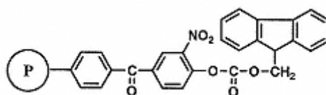
Fig. 2.22. Polymeric 3-nitro-4-[[9-fluorenylmethoxy)carbonyl] oxy]benzophenone.
