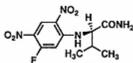
Fig. 2.4. Na-(2,4-Dinitro-5-fluorophenyl) -L-alanineamide (FDAA).
