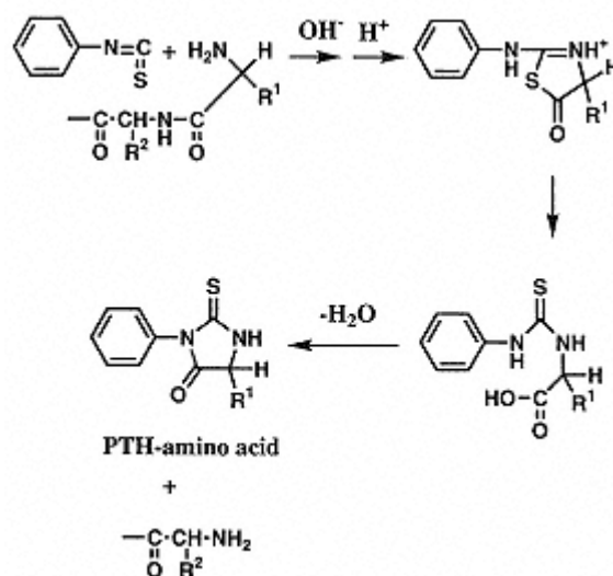
Fig. 2.6. Analysis of sequential N-terminal amino acid analysis using phenyl isothiocyanate (Edman degradation).
