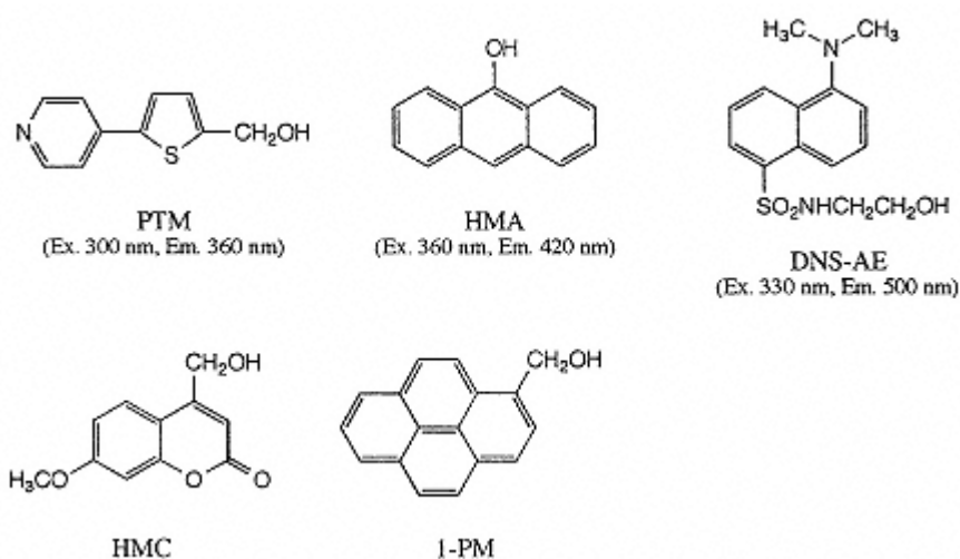
Fig. 3.34. Sulfonate reagents.
