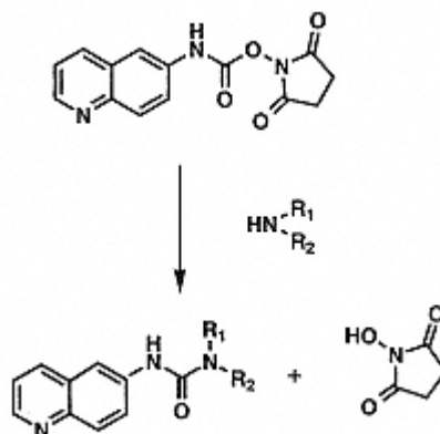
Fig. 2.17. The reaction of AQC with amines.
