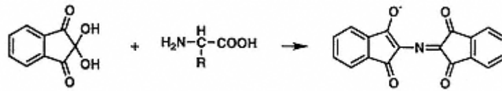
Fig. 2.14. The reaction of ninhydrin with amino acids.
