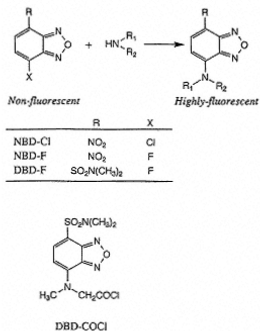
Fig. 3.14. Benzofurazan reagents.
