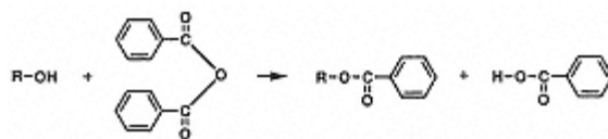
Fig. 2.30. The reaction of hydroxyl group and benzoic anhydride.
