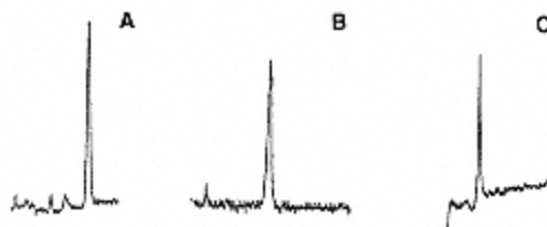
Fig. 1.1.4. Comparison of the detection limit of N-dansyl-ethylenediamine derivative of pravastatin sodium by three different detectors in HPLC. A; UV (239 nm) detection with 10 ng/injection, B; conventional fluorescence detection (Ex. 350 nm and Em. 530 nm) with 50 pg/injection and C; laser-induced fluorescence detection with 15 pg/injection. [Reproduced from ref. 3, p. 1634, Fig. 5.].
