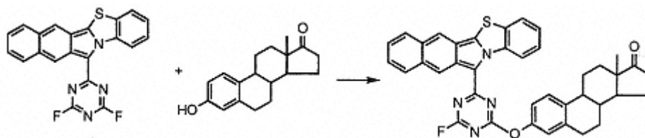
Fig. 3.48. Fluorescence labeling reaction of estron with FBIBT.
