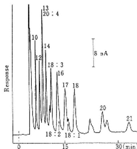
Fig. 5.12. Chromatogram of p-hydroxyanilides of fatty acids [71]. The numbers in the figure present the ratio (number of carbon atoms): (number of double bonds) for fatty acids. Reprinted from Chemical & Pharmaceutical Bulletin , 28, S. Ikenoya et al., Chromatogram of p-Hydroxyanilides, 2945, 1980, with kind permission of The Pharmaceutical Society of Japan.
