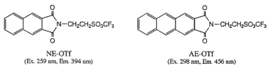
Fig. 3.33 Alcohol reagents.
