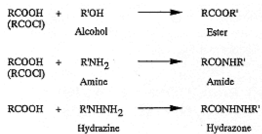
Fig. 6.10. Derivatization reactions for diastereomer formation of optically active carboxyls.
