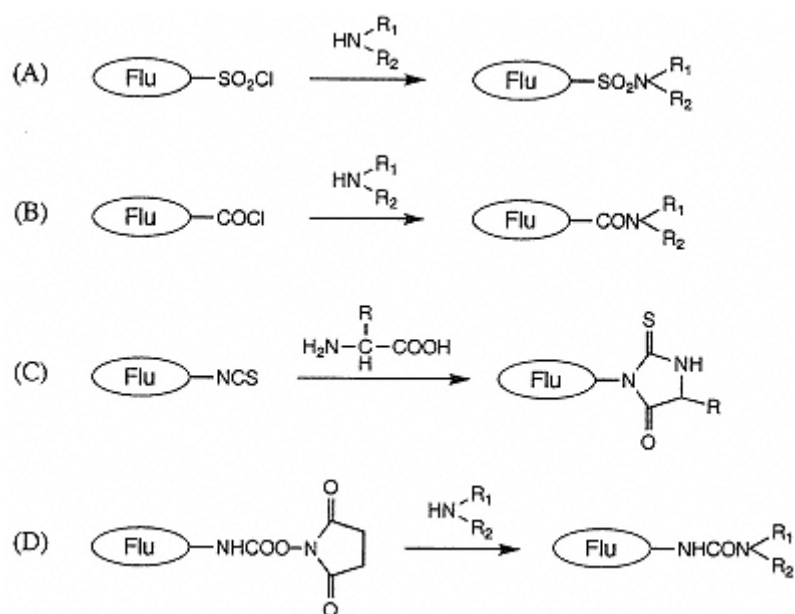
Fig. 3.5. Fluorescence labeling reagents for amines.
