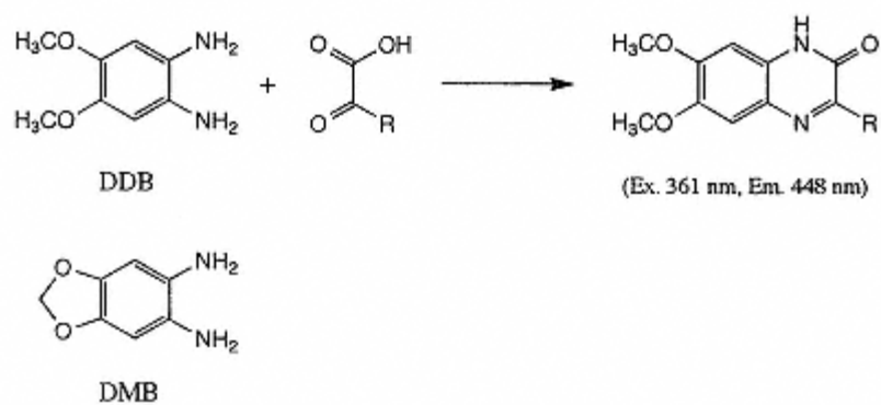
Fig. 3.40. Fluorogenic reaction of \alpha -keto acids with DDB (or DMB).
