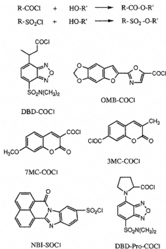
Fig. 3.43. Fluorescence labeling reagents with carbonyl and sulfonyl chloride and their reaction with alcohols.
