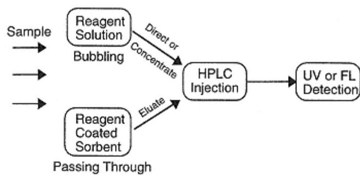
Fig. 1.3.6. Scheme of trapping methods with derivatization for the aldehydes and ketones.
