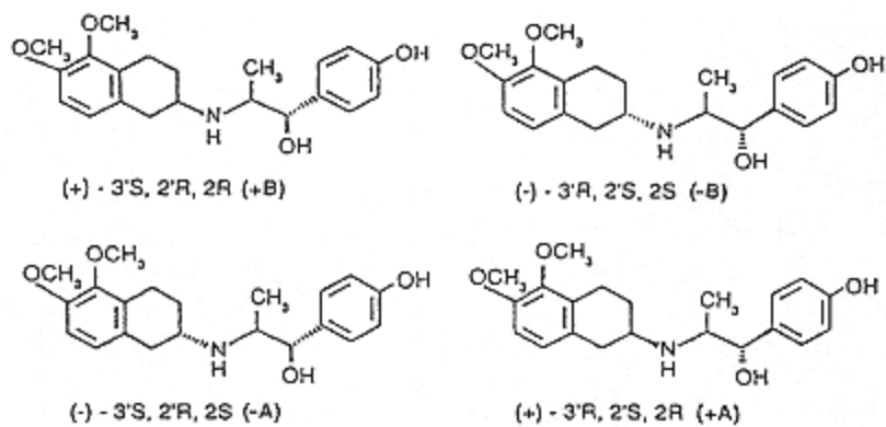
Structures of the stereoisomers of I.
