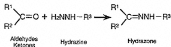
Fig. 1.3.5. Reaction of aldehydes and ketones with hydradine compound.
