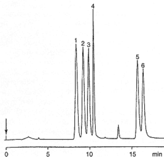
Fig. 6.31. Separation of proline derivatives obtained from racemic FLEC reagents. Peaks: (1) trans-4-hydroxy-L-proline; (2) trans-4-hydroxy-D-proline; (3) cis-4-hydroxy-L-proline; (4) cis-4-hydroxy-D-proline; (5) L-proline; and (6) D-proline. [Reproduced from ref. 154, p. 1193, Fig. 2.].
