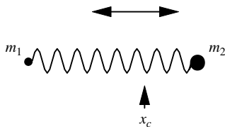
Figure 4-2 Two Masses Vibrating Harmonically with Respect to their Center of Mass. The center of mass may be stationary or moving with respect to an external coordinate system.
