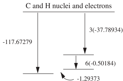
Figure 10-4 The Energy of Formation of \text{C}_3\text{H}_6(\text{g}) from 3 \text{C}(\text{g}) and 6 \text{H}(\text{g}) .
