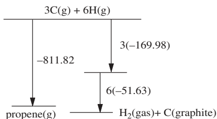
Figure 10-6 Energies Leading to the Energy of Formation of Propene ( \text{g} ).
