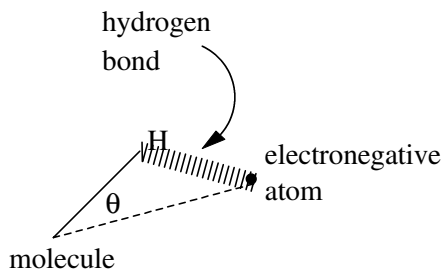
Figure 4-17 Hydrogen Bonding.
