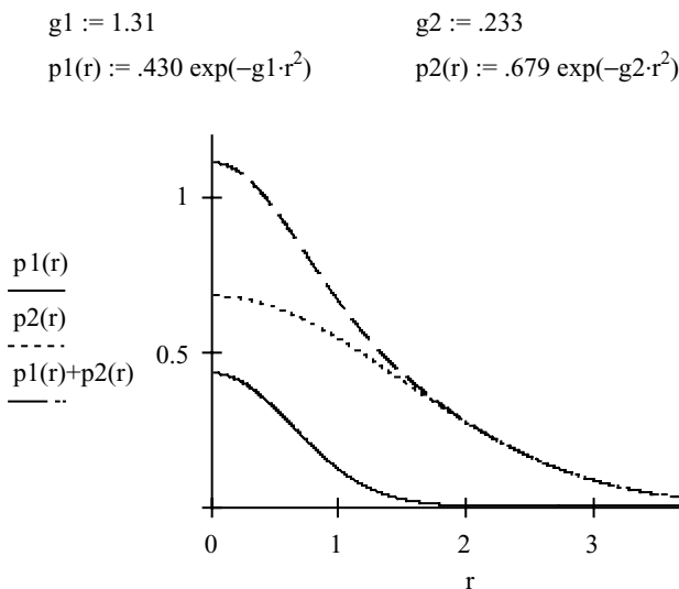
Figure 8-3 Approximation to the 1s Orbital of Hydrogen by 2 Gaussians. The upper curve is the sum of the lower two curves.
