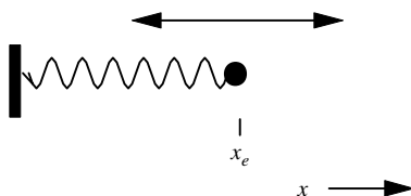
Figure 4-1 A Harmonic Oscillator in One Dimension.
