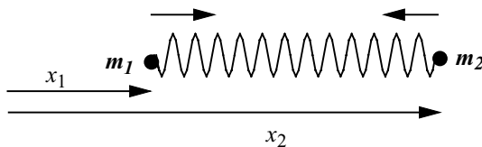
Figure 9-5 A Diatomic Molecule. The molecule can undergo translation without changing the distance ( x_2 - x_1 ), or it can undergo vibration, in which ( x_2 - x_1 ) changes, or it can undergo translation while vibrating.
