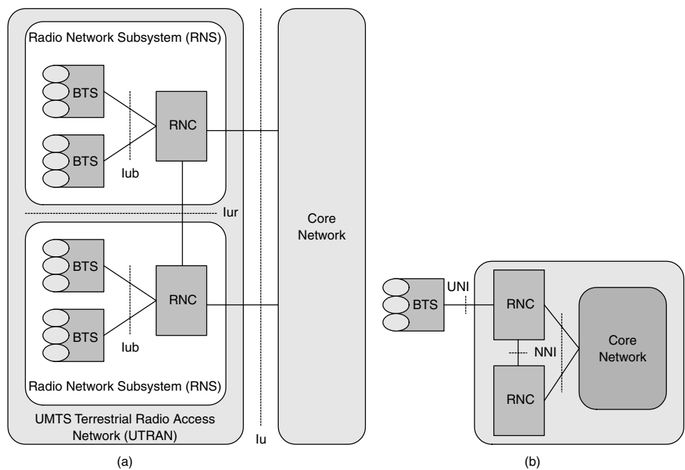
Figure 6.7 UTRAN architecture
