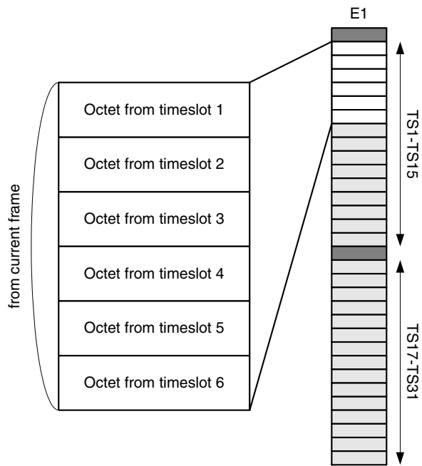
Figure 7.25 n \times 64 kbps block
