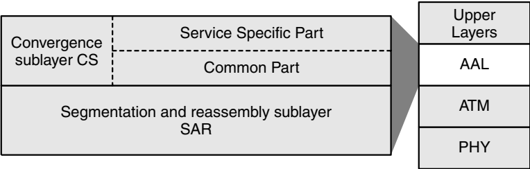
Figure 7.19 AAL sublayers
