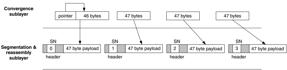
Figure 7.22 AAL1 structured data
