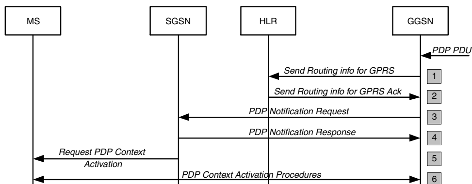
Figure 4.44 GGSN-originated PDP context activation
