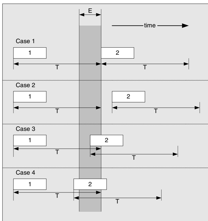
Figure 7.51 Generic cell rate algorithm
