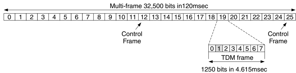
Figure 3.13 GSM multiframe
