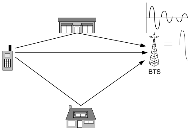
Figure 2.21 Multipath propagation
