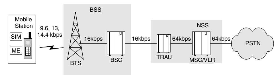
Figure 3.4 Transcoding
