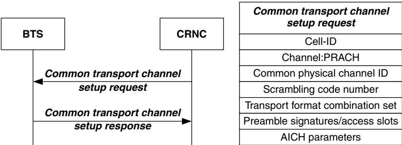
Figure 6.101 NBAP common channel setup
