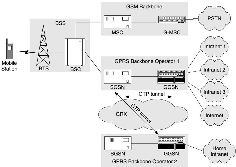
Figure 4.41 GTP tunnel
