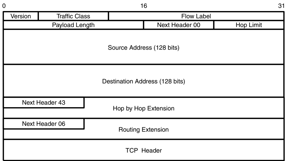
Figure 5.56 Example header extensions
