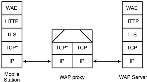
Figure 5.45 WAP 2.0 security
