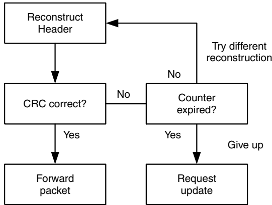
Figure 5.34 ROHC decompressor
