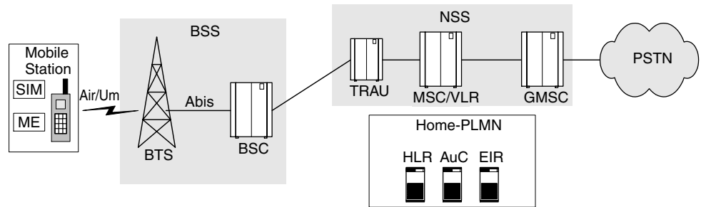
Figure 3.1 GSM general architecture
