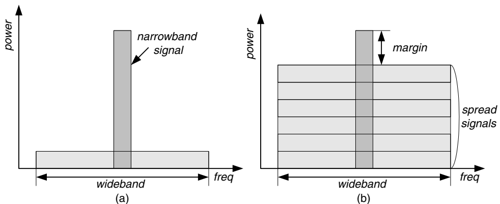
Figure 2.10 Signal spreading
