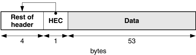
Figure 7.13 Header checking
