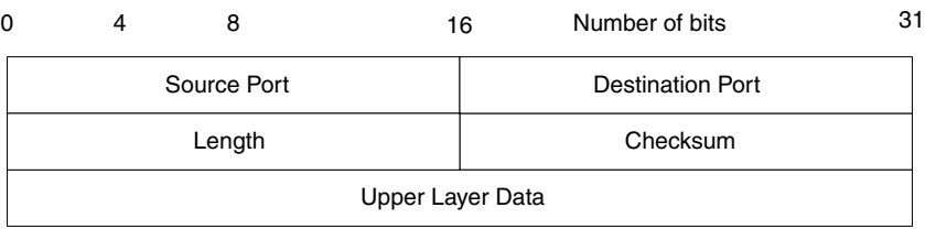
Figure 5.7 UDP header
