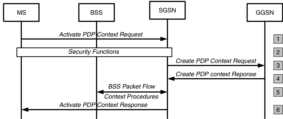
Figure 4.43 UE-originated PDP context activation
