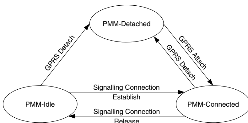
Figure 6.118 Mobility management
