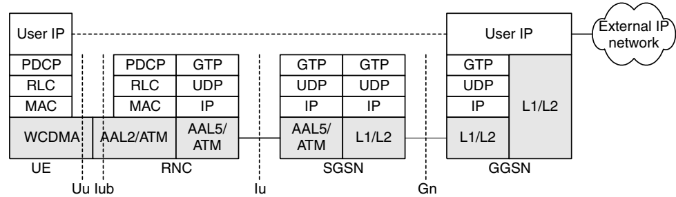
Figure 5.28 GTP tunnelling for user IP (release 99)
