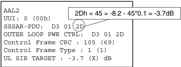
Figure 6.82 Sample trace of outer loop power control
