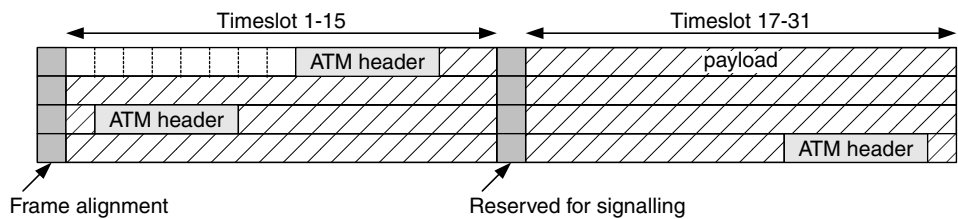
Figure 7.10 Framing of ATM cells in 2 Mbps PDH frame
