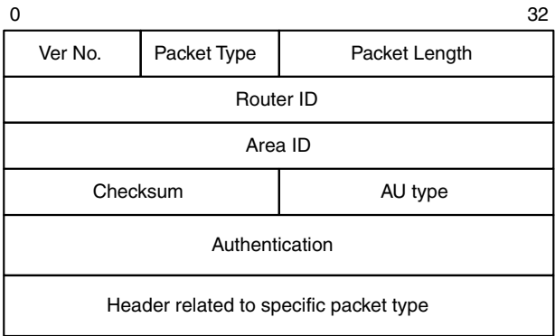
Figure 5.21 OSPF header structure
