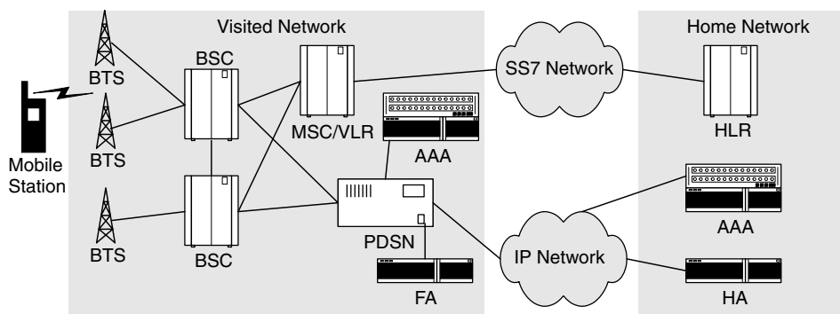
Figure 6.142 CDMA2000 example network
