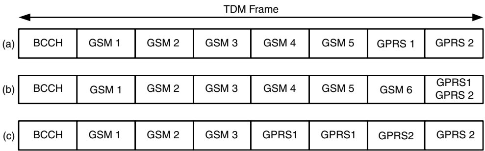
Figure 4.5 TDM frames
