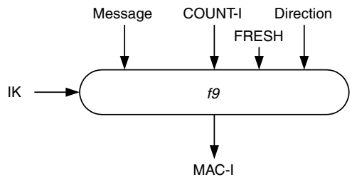
Figure 6.122 Message integrity check
