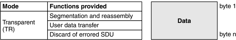
Figure 6.45 RLC transparent mode PDU
