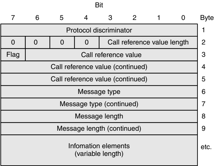
Figure 7.70 ATM signalling header
