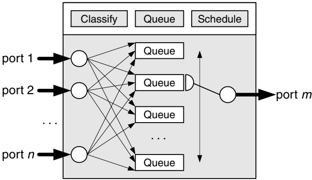
Figure 7.45 CQS architecture
