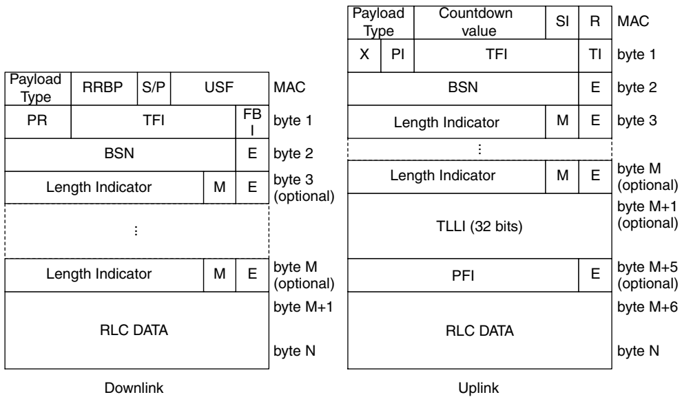
Figure 4.24 RLC/MAC data block
