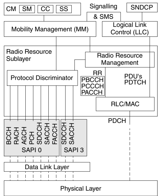
Figure 4.10 Mobile device layered architecture
