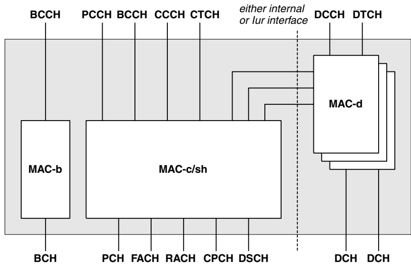
Figure 6.51 MAC architecture
