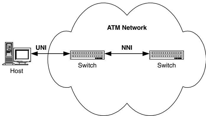
Figure 7.16 ATM interfaces
