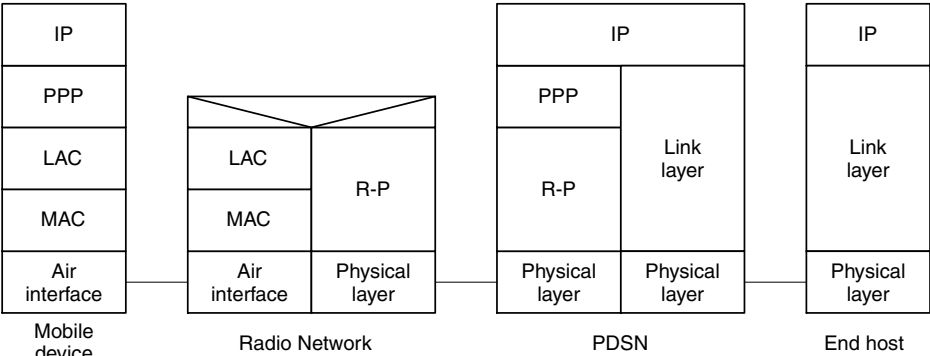
Figure 5.67 PPP for CDMA2000
