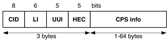
Figure 7.29 CPS packet format
