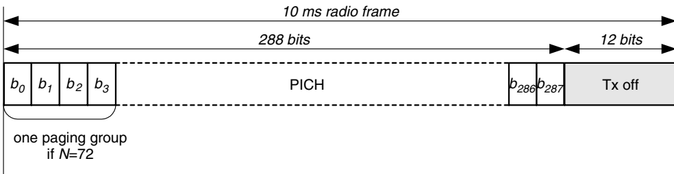
Figure 6.26 PICH structure
