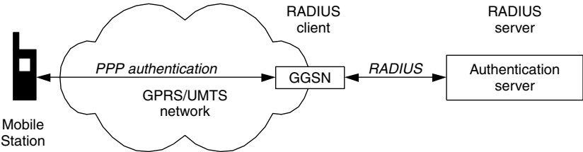
Figure 5.68 RADIUS configuration
