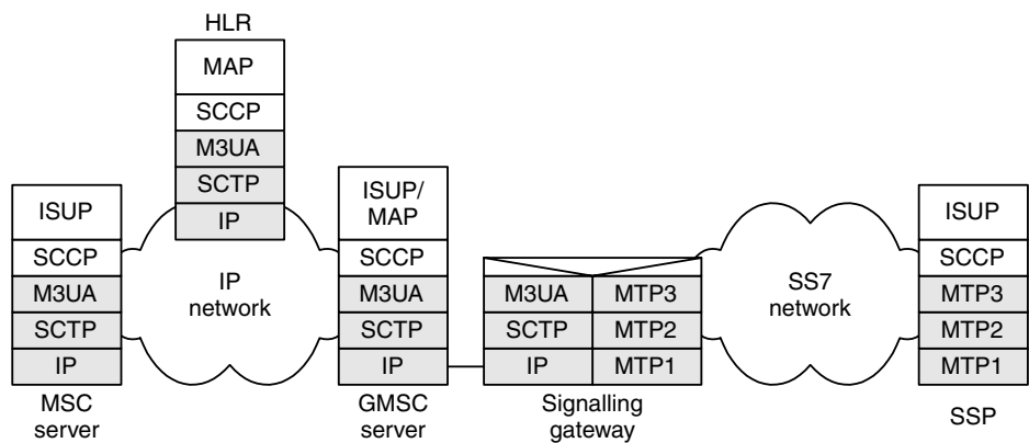
Figure 8.28 M3UA service
