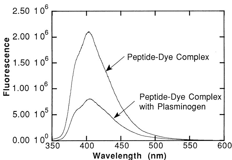
Figure 4.17 Fluorescence spectra of a fluorescently labeled peptide (Lys-Cys-Lys) free in solution (peptide—dye complex) and bound to the protein plasminogen. Note the significant quenching of the probe fluorescence upon peptide—plasminogen binding. [Data from Balciunas et al. (1993).]
