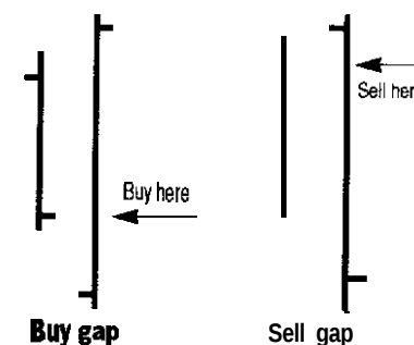
FIGURE 4.1 A standard gap buy-and-sell pattern.
