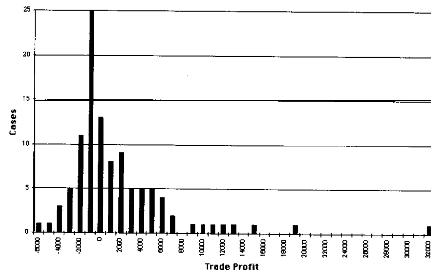
FIGURE 16.1 The distribution of trade profits for a standard channel breakout system on the Yen.
