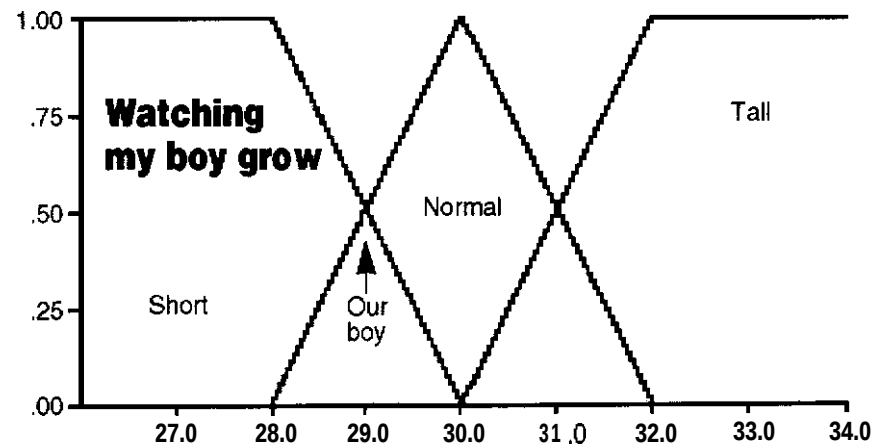
FIGURE 11.9 An example of a simple defuzzification function for height.
