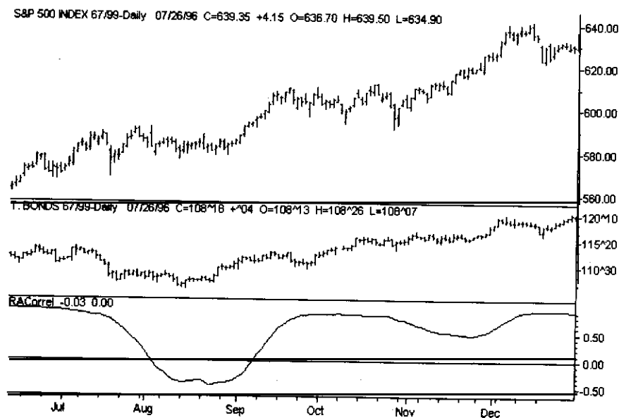
FIGURE 8.1 The correlation between the S&P500 and T-Bonds can predict when a market will trend. In 1995, as correlation rose, the S&P500 exploded and rose 57.55 points in only about 70 trending days
