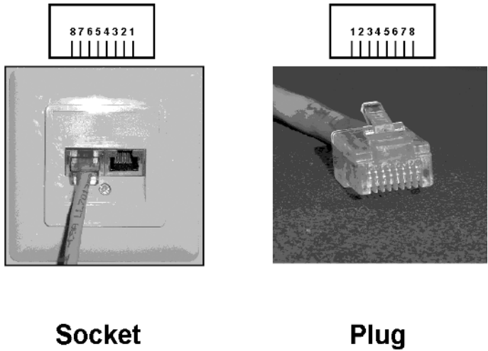
Figure A7.13 RJ-45 connector: 8-pole socket and plug and pin layout.
