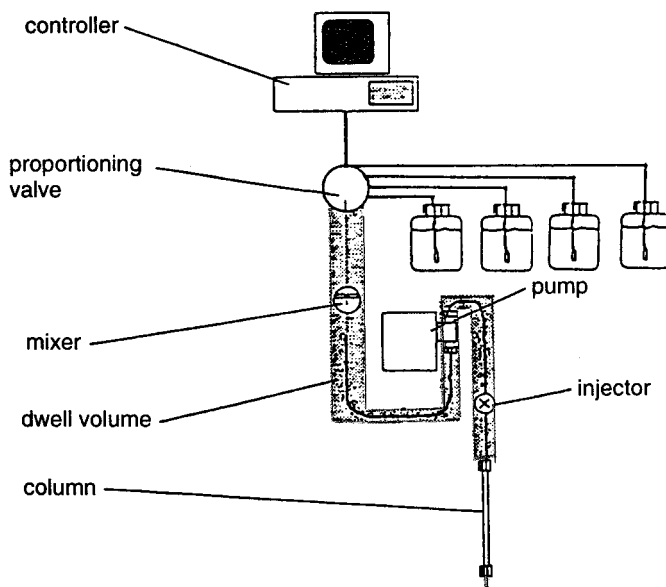
Figure 2.6. Low-pressure mixing systems use a single pump with a proportioning valve to control composition. Advantages of low pressure mixing are lower cost (single pump) and more versatile gradients (four solvents).
