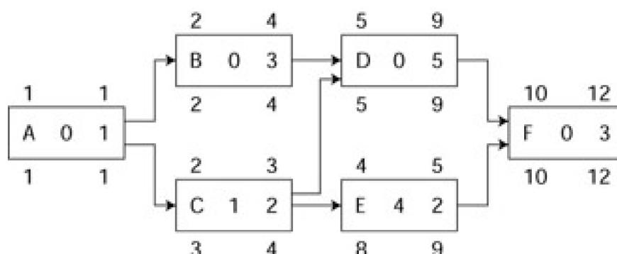
Figure 6.8: Critical path.
