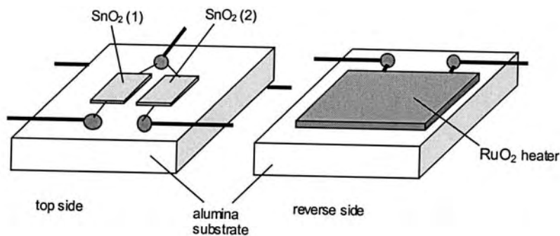
Fig. 4.49 Twin tin oxide-based sensors for monitoring \text{NO}_2 and CO in automobile passenger compartments. NB: alumina substrate size approximately 2 \times 2.6 \times 0.254 mm. (Adapted from Oto, K. et al. (2001), Sensors and Actuators , B77 , 525–8.)
