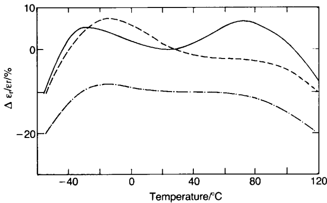
Fig. 5.48 Dependence of \epsilon_r on T and d.c. bias (—, 0; ---, 2 \text{ MV m}^{-1} ; - · - ·, 4 \text{ MV m}^{-1} ) for \text{Pb}_{0.85}\text{La}_{0.1}\text{Ti}_{0.2}\text{Zr}_{0.8}\text{O}_3 (PLZT). (After G.H. Maher (1983) 33rd Electron. Comp. Conf. (IEEE) 173–7.)
