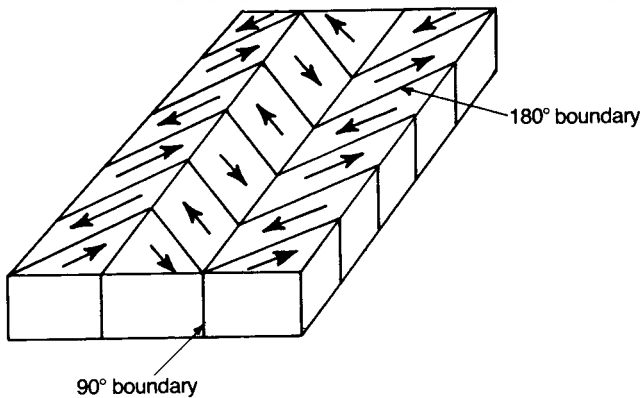
Fig. 2.45 (a) Polished and etched surface of unpoled ceramic; (b) schematic diagram of 180^\circ and 90^\circ domains in barium titanate.
