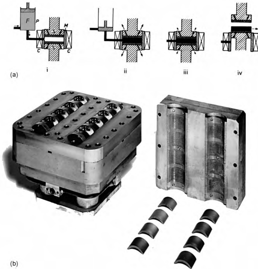
Fig. 9.42 (a) Diagram of the pressing cycle: M, Die; S, S', punches; P, injection pump; F, suspension; C, magnet coil. The punches contain filters and drainage channels for the water. (i) Before and (ii) after the material is injected into the compression space; the slurry is densified from 40% to 13% water content, and the particles are oriented by the magnetic field; (iii) after densification by slight upward movement of the lower punch, the amount of the movement depending on the thickness of the product; demagnetization; (iv) removal of the compacted product. (b) Die for simultaneous pressing of eight oriented magnet segments. (Courtesy of Philips Technical Review.)
