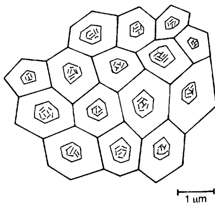
Fig. 5.45 Duplex microstructure of an X7R dielectric ceramic.
