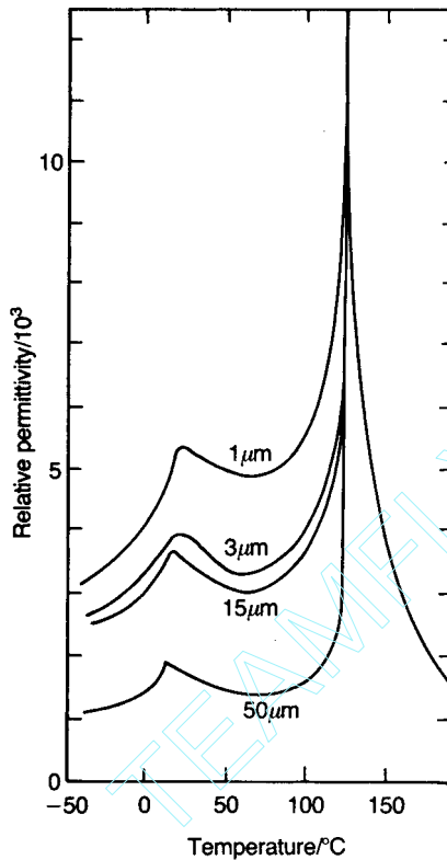
Fig. 2.48 The effect of grain size on the permittivity of a \text{BaTiO}_3 ceramic. (After K. Kinoshita and A. Yamaji (1976) J Appl. Phys. 47 , 371.)
