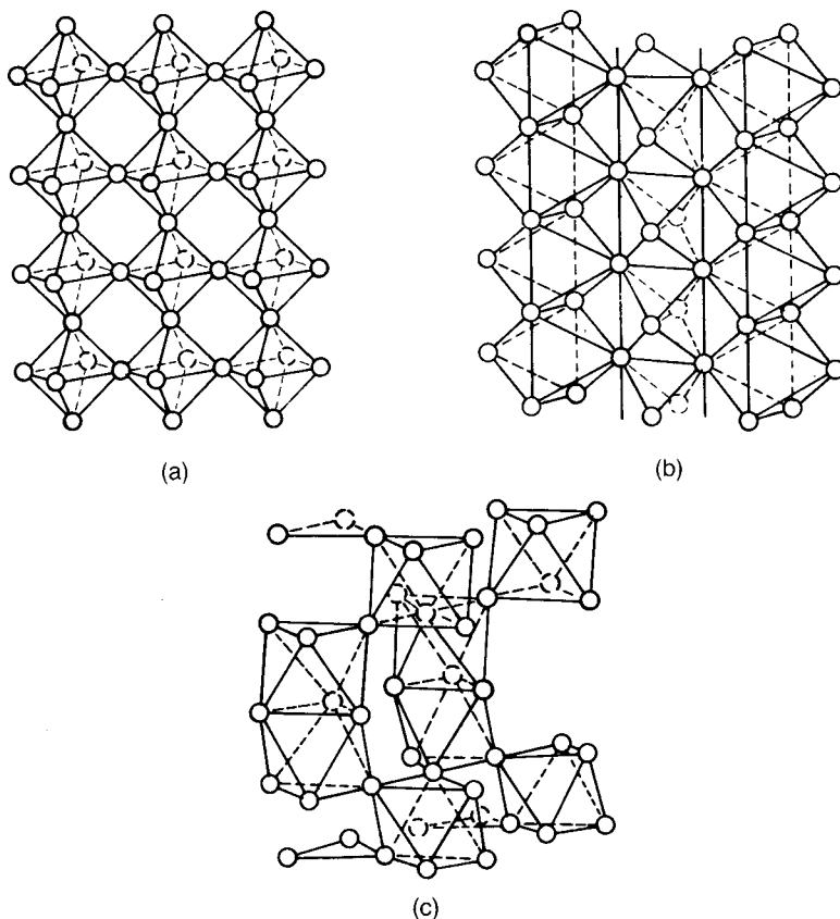
Fig. 2.2 \text{MO}_6 octahedra arrangements in (a) perovskite-type structures, (b) \text{TiO}_2 and (c) hexagonal \text{BaTiO}_3 .
