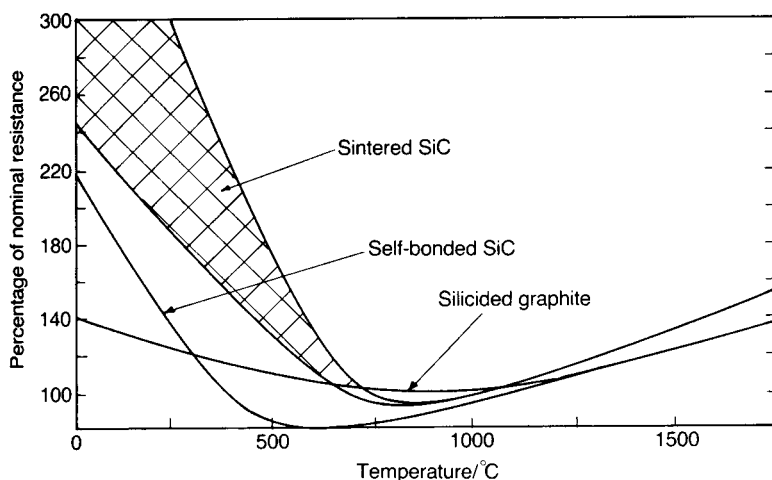
Fig. 4.2 Resistance-temperature characteristics of SiC elements prepared by various methods.
