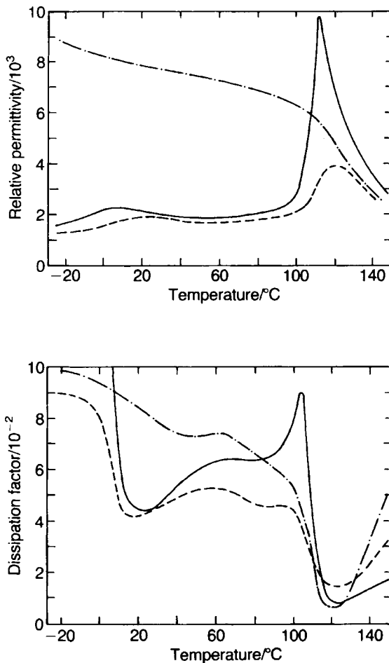
Fig. 5.43 Dielectric properties of technical grade BaTiO 3 ceramic under various field conditions: —, 15 kV m -1 peak and 1 kHz; ---, 15 kV m -1 peak and 1 kHz + 1.43 MV m -1 d.c.; — · —, 1.6 MV m -1 peak and 50 Hz.
