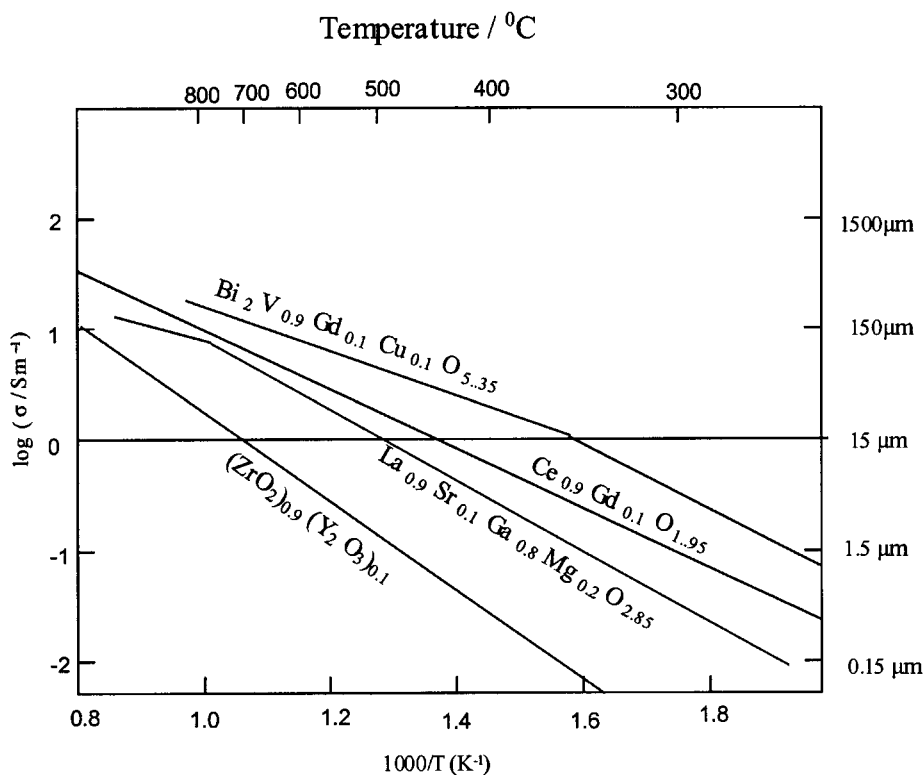
Fig. 4.31 Ionic conductivities for candidate electrolyte ceramics. The arbitrary assumption that for a planar cell format a resistance of <15 \mu\Omega \text{m}^{-2} is required places an upper limit on the permitted thickness of the electrolyte; lower values of conductivity demand thinner membranes whilst higher values permit correspondingly thicker membranes. Electrolyte thicknesses greater than approximately 150 \mu\text{m} are considered mechanically self-supporting. After B.C.H. Steele [11].
