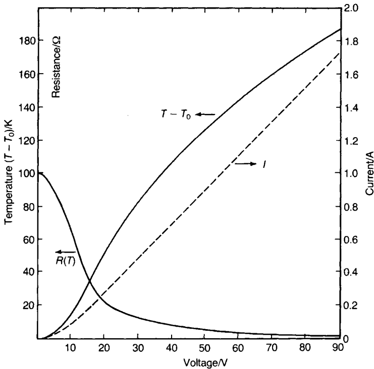
Fig. 4.19 Resistance, current and temperature versus voltage for an NTC thermistor with series load: P = (T - T_0)/30 \text{ W} .
