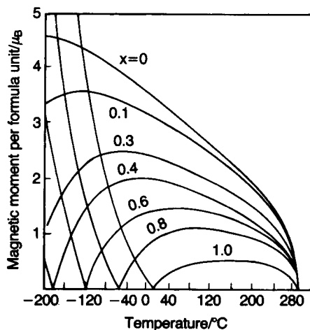
Fig. 9.16 Variation of saturation magnetization with temperature for \text{Y}_{3(1-x)}\text{Gd}_{3x}\text{Fe}_5\text{O}_{12} for various x values.
