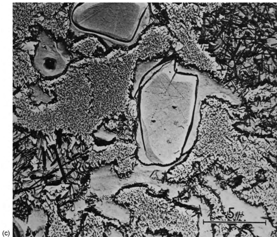
Fig. 5.20 Microstructures of (a) 99.9% \text{Al}_2\text{O}_3 (Courtesy of E.W. Roberts), (b) 95% \text{Al}_2\text{O}_3 (Courtesy of R. Morrell), (c) chemically etched electrical porcelain: note the partially dissolved quartz grains and mullite precipitates (Courtesy of S.T. Lundin).
