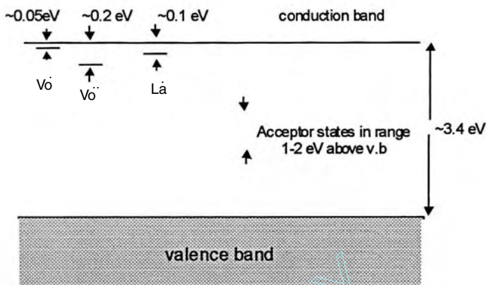
Fig. 2.15 Tentative band diagram for doped \text{BaTiO}_3 .
