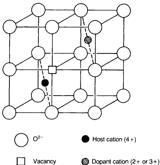
Fig. 4.29 The ideal fluorite structure showing half a unit cell including a dopant cation and a charge-compensating oxygen vacancy.
