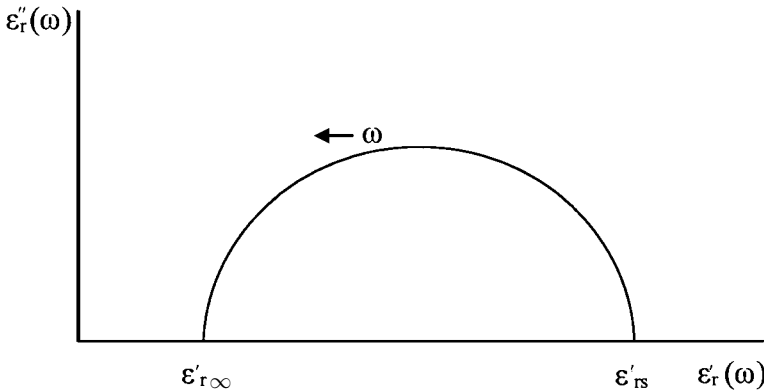
Fig. 2.52 Plot of the frequency response of the real and imaginary components of the relative permittivity of a dielectric satisfying the Debye equations.
