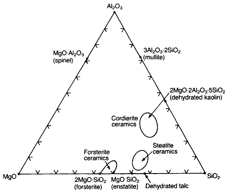
Fig. 5.18 Phases present in the \text{Al}_2\text{O}_3\text{--MgO--SiO}_2 system (in wt%).
