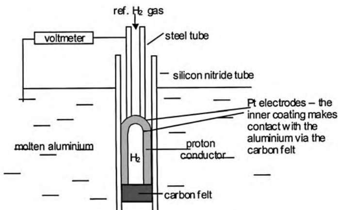
Fig. 4.43 A protonic electrolyte used for measuring the hydrogen content of molten aluminium (adapted from TYK Corporation (Japan) literature; see [23]).
