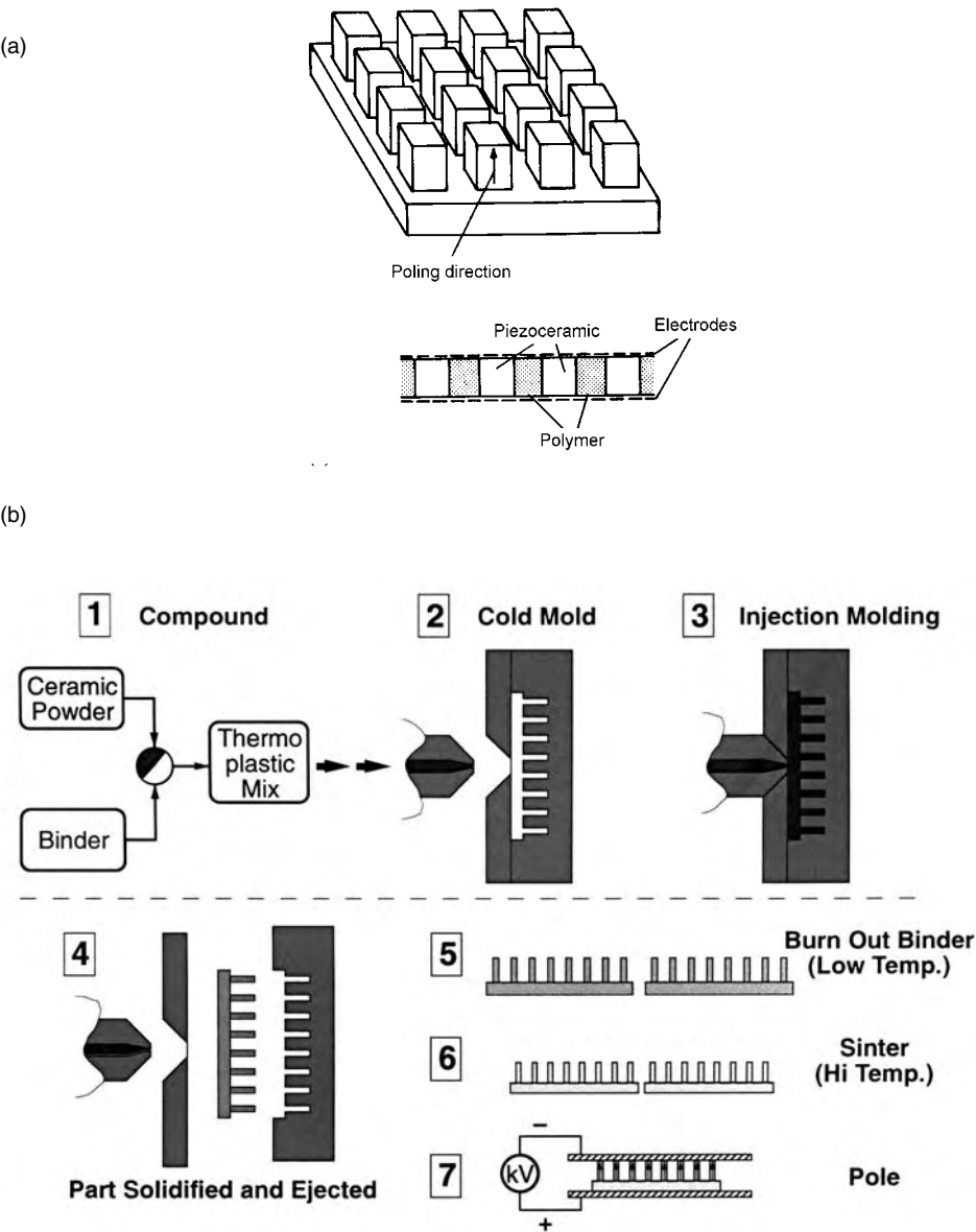
Fig. 6.19 (a) 1–3 piezoceramic–polymer composite. (b) Fabricating the rod array for a 1–3 piezoceramic–polymer composite by injection-moulding. (Courtesy of Materials Systems Inc. Littleton MA; the ‘MSI’ website: www.matsyinc.com is an excellent source of information.)
