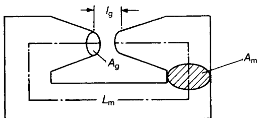
Fig. 9.36 Permanent magnet with an air gap.
