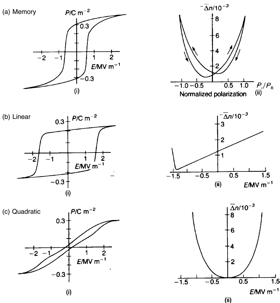
Fig. 8.11 Hysteresis and electro-optic characteristics of the three main types of PLZT: (a) memory; (b) linear; (c) quadratic (after G.H. Haertling (1971) J. Am. Ceram. Soc. , 54 , 303).
