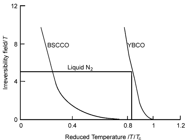
Fig. 4.57 Irreversibility curves for candidate HTS ceramics: at liquid N 2 temperature T/T_c (YBCO) \sim 0.83 and for Bi-2223 \sim 0.79 . (After D.A. Cardwell [41].)
