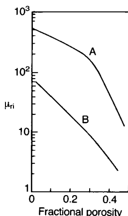
Fig. 9.21 Dependence of the initial relative permeability on porosity: curve A, \text{Ni}_{0.5}\text{Zn}_{0.5}\text{Fe}_2\text{O}_4 ; curve B, \text{NiFe}_2\text{O}_4 (after [6]).
