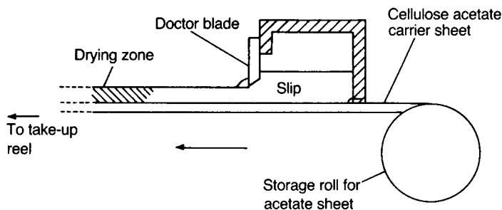
Fig. 3.6 Schematic diagram of the doctor-blade tape-casting process.
