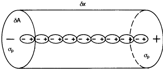
Fig. 2.26 Elementary prism of polarized material.
