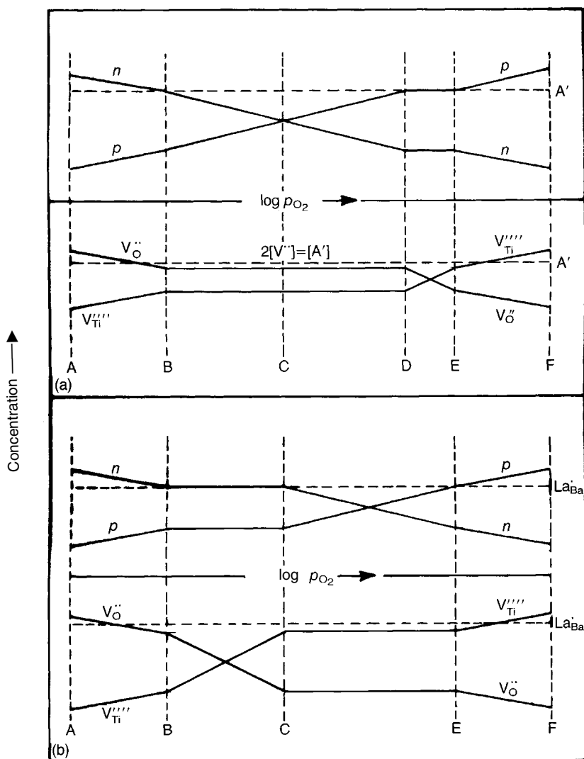
Fig. 2.13 Schematic representation of the dependence of n , p , [V_{Ti}^{\bullet\bullet\bullet\bullet}] and [V_O^{\bullet\bullet}] on p_{O_2} for (a) acceptor-doped and (b) donor-doped BaTiO_3 .
