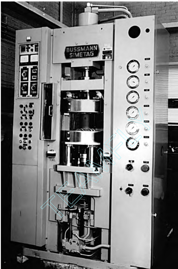
Fig. 9.43 Production press for oriented ferrite components. (Courtesy of Philips Technical Review.)
