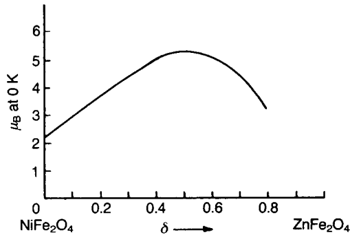
Fig. 9.14 Saturation magnetization per 'formula unit' for the ferrite (\text{Fe}_{1-\delta}^{3+}\text{Zn}_\delta^{2+})(\text{Fe}_{1+\delta}^{3+}\text{Ni}_{1-\delta}^{2+})\text{O}_4 as a function of \delta .
