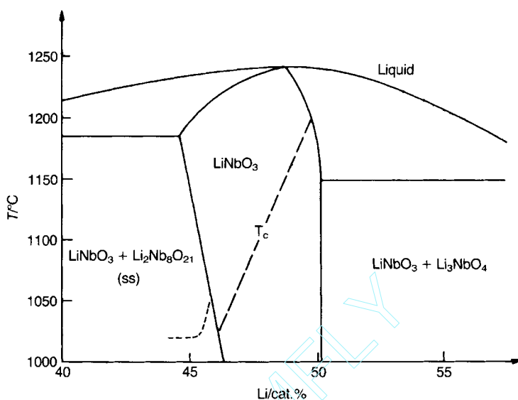
Fig. 6.18 Phase diagram for \text{LiNbO}_3 as determined for crystal growth.
