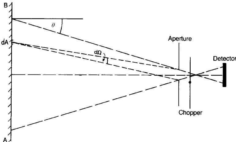
Fig. 7.8 Radiometer optics.
