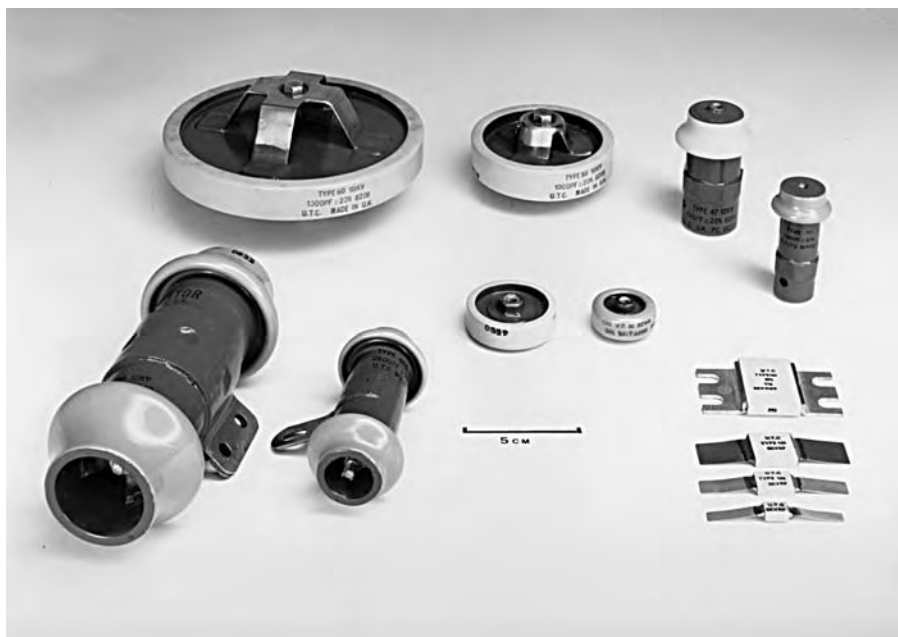
Fig. 5.16 A range of high-power transmitter capacitors (components supplied by Morgan Electro Ceramics).
