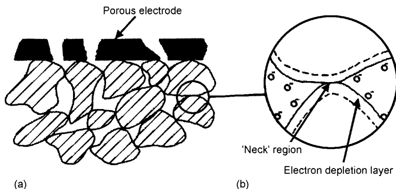
Fig. 4.46 (a) Schematic diagram of a section through a porous \text{SnO}_2 compact with a porous electrode; (b) detail of the 'neck' region between the grains showing the effect of adsorbed oxygen.
