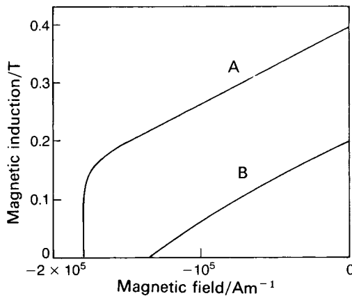
Fig. 9.34 Demagnetization curves for an oriented barium hexaferrite (curve A) and an isotropic hexaferrite (curve B).
