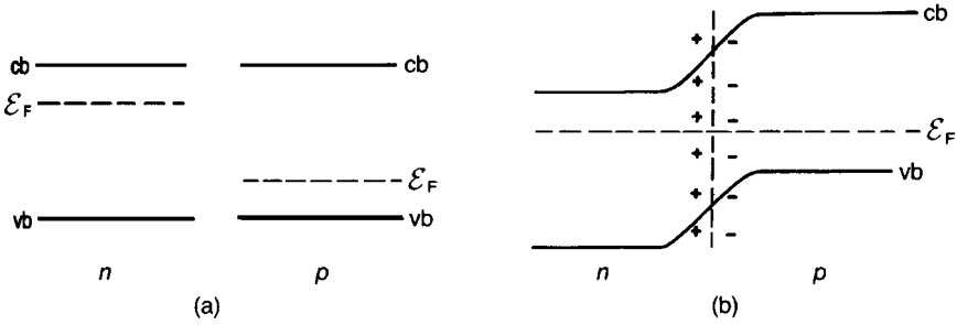
Fig. 2.23 Junction between an n-type and a p-type semiconductor (a) before contact and (b) after contact.
