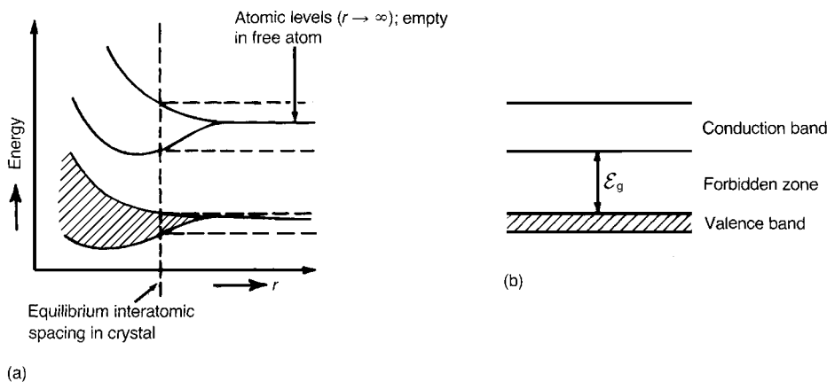
Fig. 2.7 (a) Atomic levels having identical energies merging to a broad band of levels differing slightly in energy as free atoms condense to form a crystal; (b) band structure at equilibrium interatomic spacing in a crystal.
