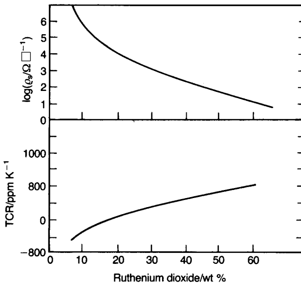
Fig. 4.6 Electrical characteristics of \text{RuO}_2 thick-film resistors.
