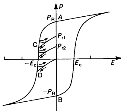
Fig. 8.12 Establishment of intermediate polarization states P_{r1} , P_{r2} etc.
