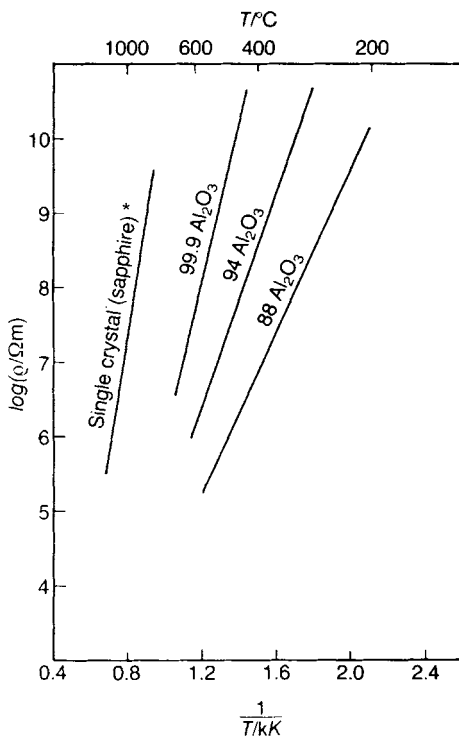
Fig. 5.21 Dependence of resistivity on temperature for various grades of \text{Al}_2\text{O}_3 . *[4]
