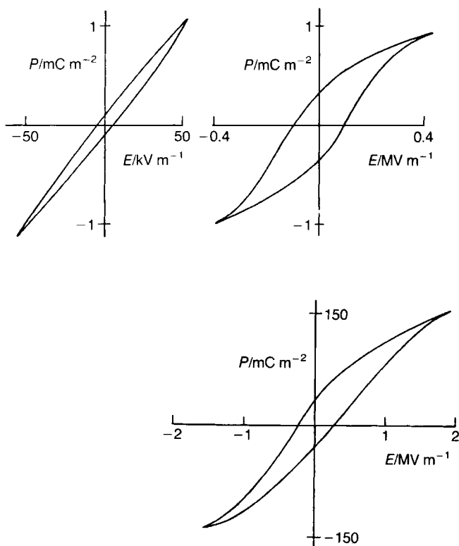
Fig. 6.9 P - E loops with increasing peak field strengths at 50 Hz for a ceramic ferroelectric.
