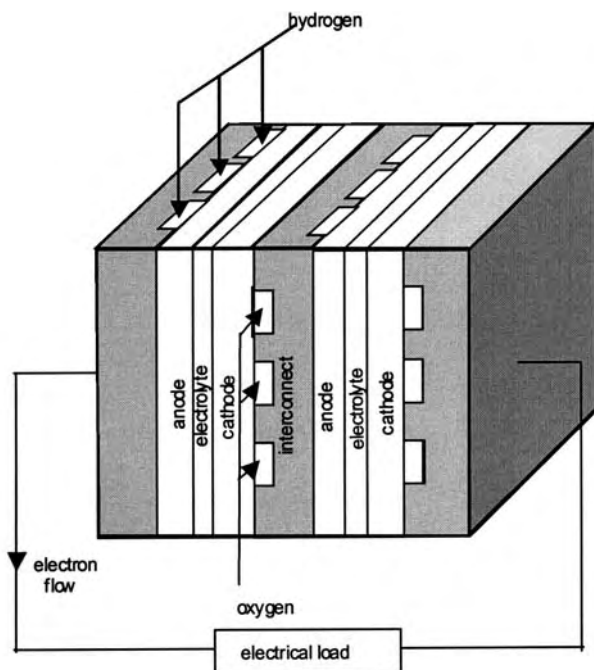
Fig. 4.27 Illustrating the connecting of two fuel cells via bipolar plates ('interconnects').
