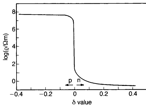
Fig. 9.23 Dependence of the resistivity of the ferrite \text{Ni}_{0.3}\text{Zn}_{0.7}\text{Fe}_{2+\delta}\text{O}_{4-x} on the iron content.
