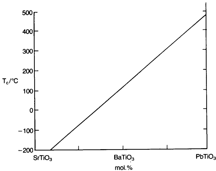
Fig. 2.47 The approximate effect on the Curie point of the substitution of either strontium or lead for barium in \text{BaTiO}_3 .
