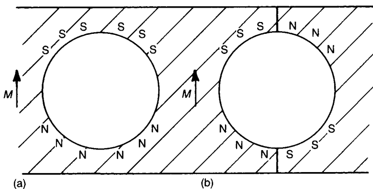
Fig. 9.30 Intersection of a Bloch wall by a pore.
