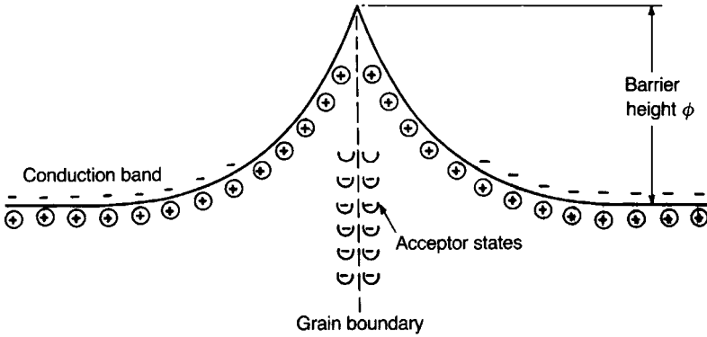
Fig. 4.21 Electrical double layer at a grain boundary.
