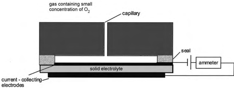
Fig. 4.40 Schematic illustrating the principle of the amperometric mode.
