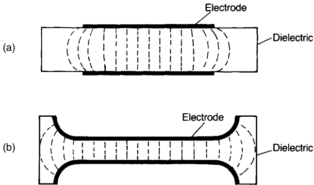
Fig. 5.14 (a) Converging lines of force at electrode edges; (b) dielectric shaping for high voltage capacitors.
