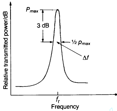
Fig. 5.34 Frequency response of a microwave resonator.
