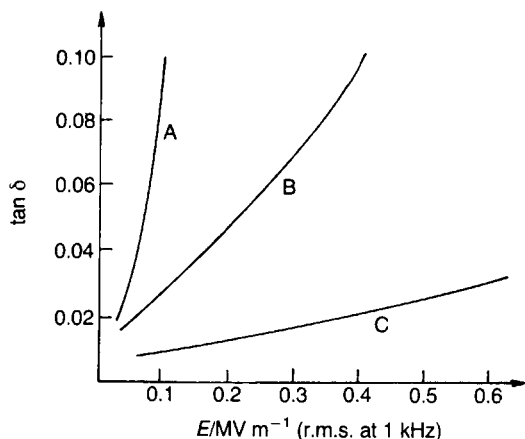
Fig. 6.12 Dependence of \tan \delta on the applied field strength for barium titanates: curve A, technically pure barium titanate; curve B, barium titanate containing lead and 1–2 at.% \text{Ti}^4 replaced by \text{Co}^{3+} , unpoled; curve C as B but poled.
