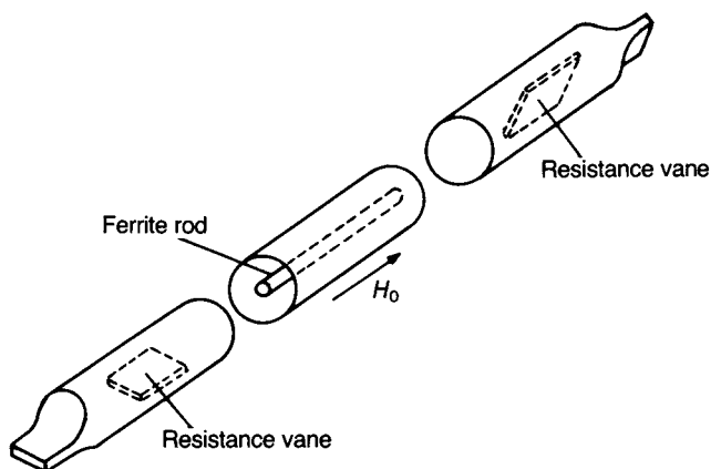
Fig. 9.53 Faraday rotation isolator.
