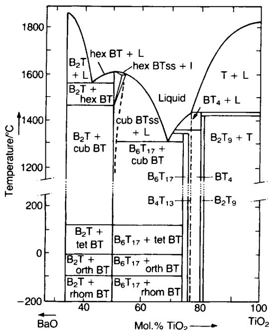
Fig. 5.41 Phase diagram of the \text{BaO} – \text{TiO}_2 system ( >34\ \text{mol.}\% \text{TiO}_2 ).
