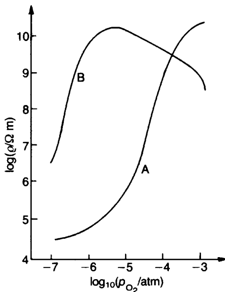
Fig. 5.50 Resistivity at room temperature as a function of oxygen pressure during sintering: curve A, undoped \text{Ba}_{0.85}\text{Zr}_{0.15}\text{O}_3 ; curve B, (\text{Ba}_{0.85}\text{Ca}_{0.15}\text{O})_{1.01}-(\text{Ti}_{0.9}\text{Zr}_{0.1})\text{O}_2 . (After [24])
