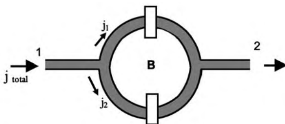
Fig. 4.61 Two Josephson junctions comprising a superconducting quantum interference device (SQUID).
