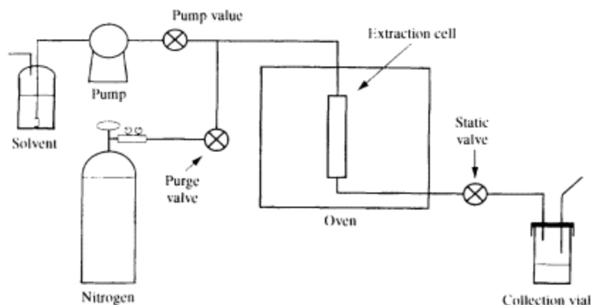
Figure 10.1 Schematic diagram of an accelerated solvent extraction system. Reproduced by permission of Dionex (UK) Ltd. Surrey
