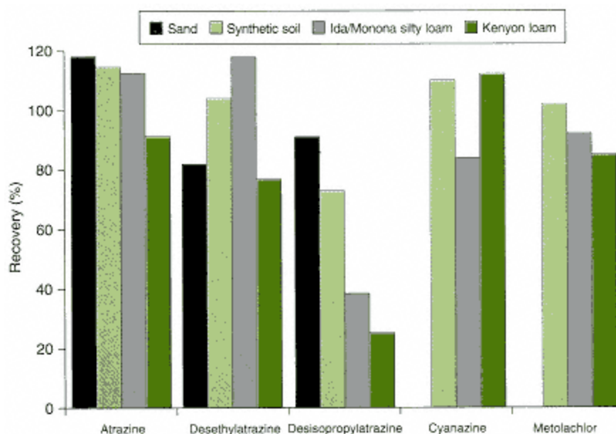
Figure 8.27 SFE of herbicides from fortified western cornbelt soils. From Steinheimer et al, Analytical Chemistry , 66 (1994) 645
