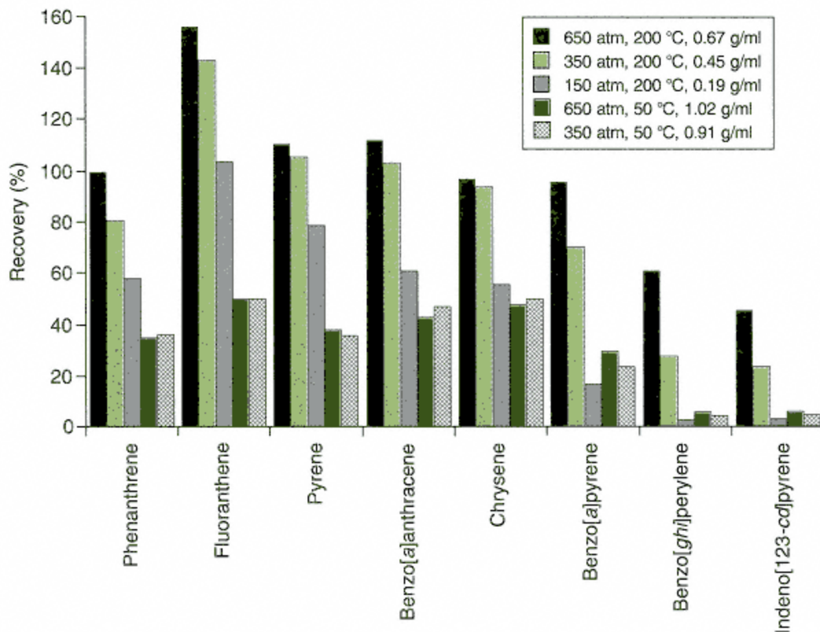
Figure 8.4 SFE of PAHs from marine sediment (SRM CRM 1941) at 80°C. From Yang et al. , Analytical Chemistry , 67 (1995) 641
