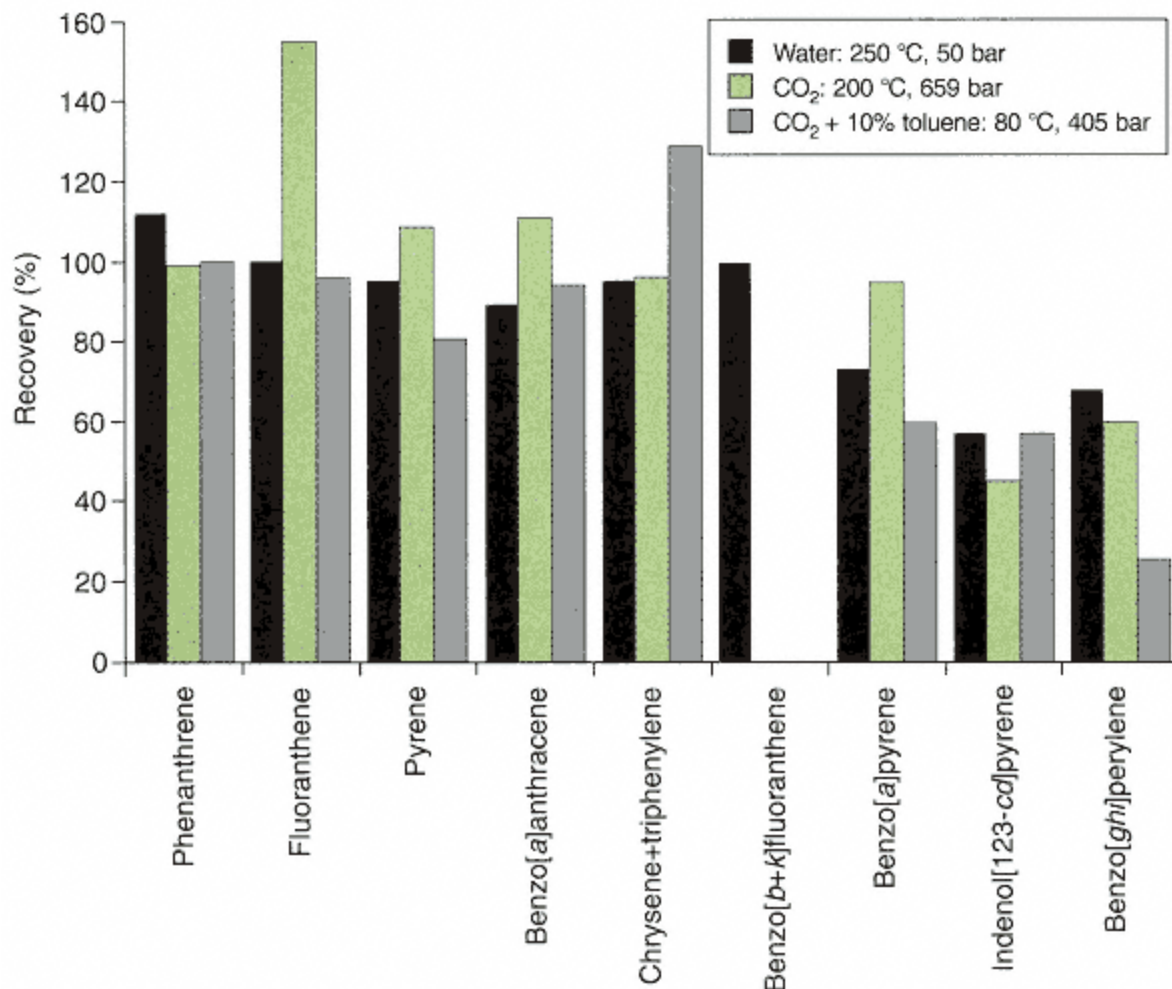
Figure 8.12 SFE of PAHs from urban air particulates (SRM CRM 1649). From Hawthorne et al. , Analytical Chemistry , 66 (1994) 2912
