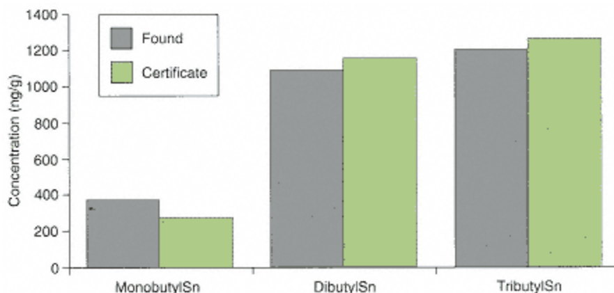
Figure 9.8 Atmospheric MAE of organotin compounds from PACS-1. From Donard et al. , Analytical Chemistry , 67 (1995) 4250
