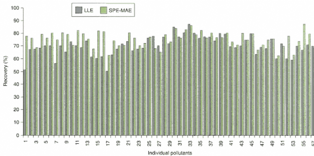
Figure 9.13 Comparison of SPE-MAE with LLE: recoveries obtained from reagent water. From Chee et al. , Analytica Chimica Acta , 330 (1996) 217
