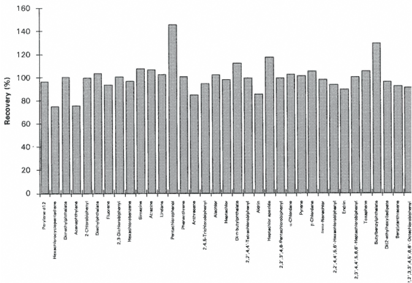
Figure 8.37 SPE-SFE using SDB disks (spike level 2 \text{ ng ml}^{-1} , n = 7 ). From Tang et al. , Journal of Chromatographic Science , 33 (1995) 1
