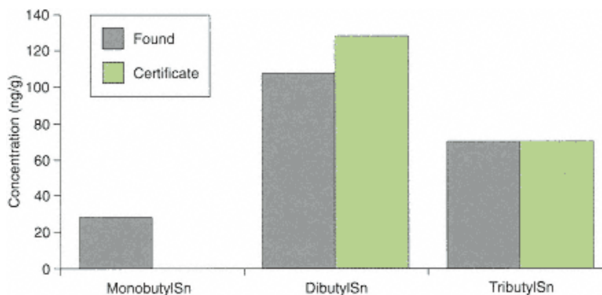
Figure 9.7 Atmospheric MAE of organotin compounds from CRM 462. From Donard et al. , Analytical Chemistry , 67 (1995) 4250
