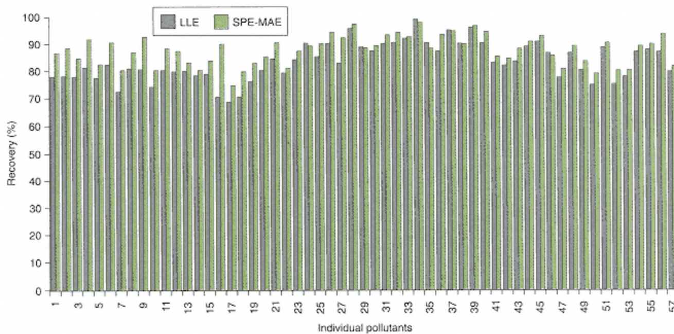
Figure 9.12 Comparison of SPE-MAE with LLE: recoveries obtained from sea water. From Chee et al. , Analytica Chimica Acta , 330 (1996) 217
