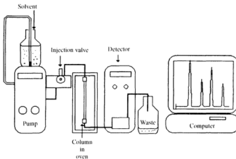
Figure 1.2 Schematic diagram of a high performance liquid chromatograph. Reproduced by permission of Mr E Ludkin, University of Northumbria at Newcastle
