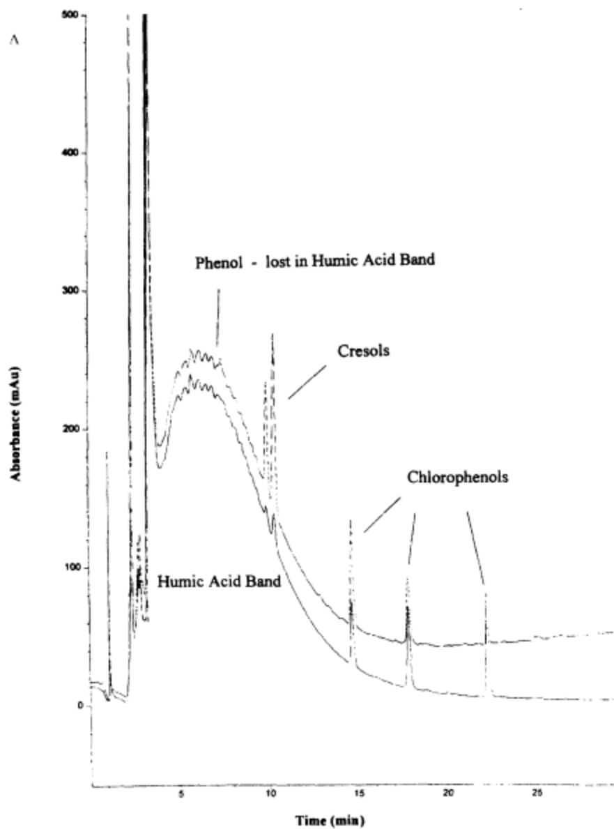
Figure 4.12 Automated SAMOS-HPLC determination of 1 ppb phenols in raw water using two pre-column system. Reproduced by permission of Dr I.A. Fowlis, Northumbrian Water
