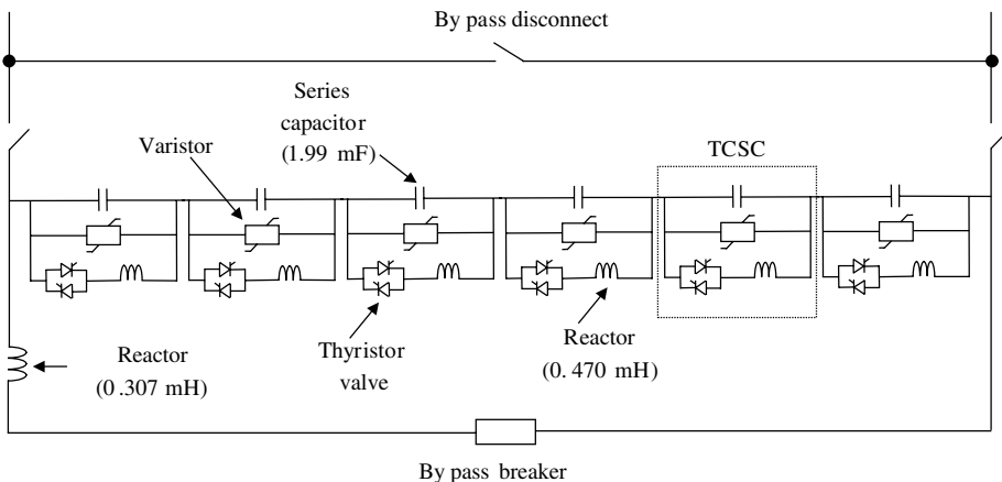
Figure 2.6 Physical structure of one phase of a thyristor-controlled series capacitor (TCSC). Reproduced, with permission, from S.J. Kinney, W.A. Mittelstadt, and R.W. Suhrbier, ‘Test Results and Initial Operating Experience for the BPA 500 kV Thyristor Controlled Series Capacitor: Design, Operation, and Fault Test Results, Northcon 95’, in IEEE Technical Conference and Workshops Northcon 95, Portland, Oregon, USA, October 1995 , pp. 268–273, © 1995 IEEE
