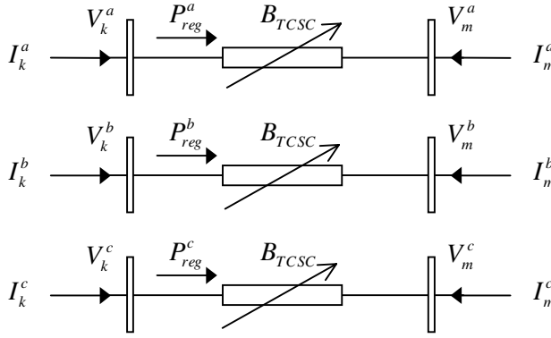
Figure 6.4 Three-phase variable series susceptance
