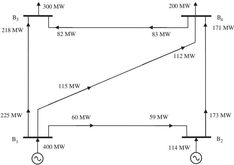
Figure 8.11 Power flows in a small, meshed network
