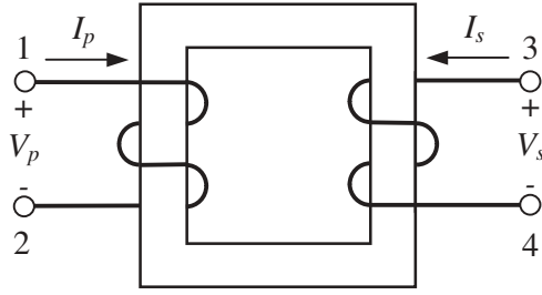
Figure 3.10 Two-winding transformer
