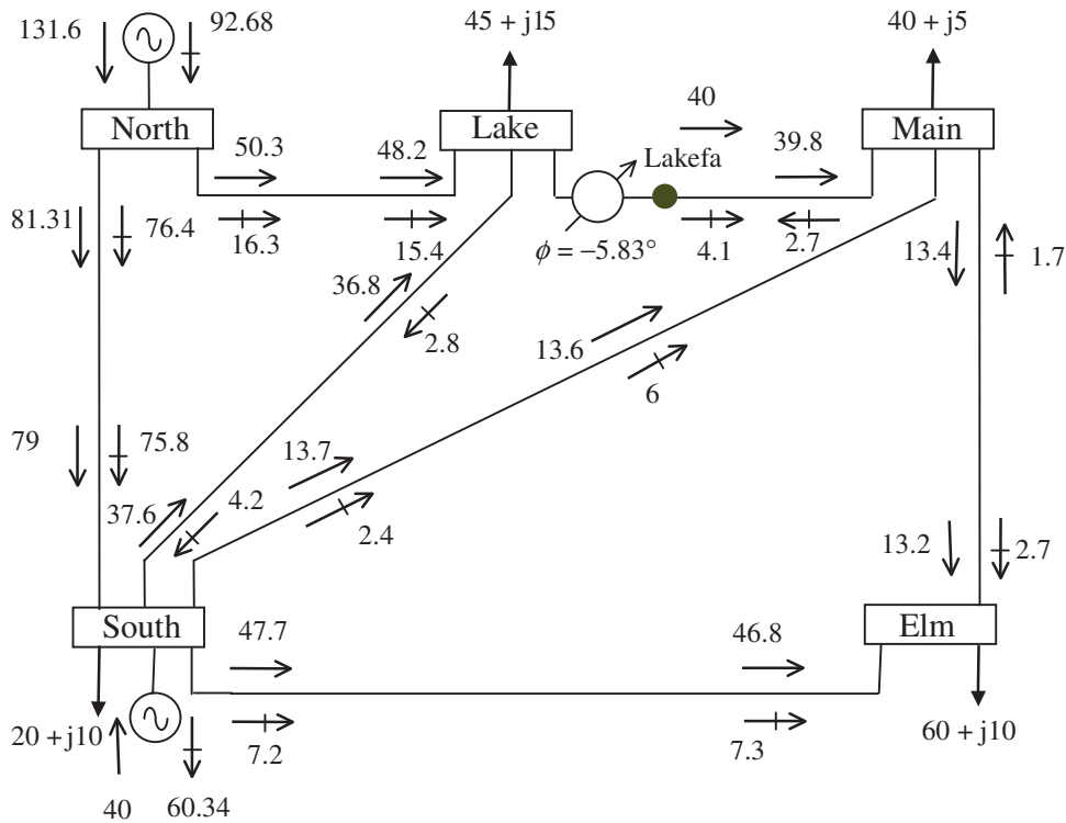
Figure 4.10 Modified test network and power flow results
