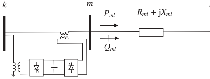
Figure 7.9 Unified power flow controller power flow constraint at bus m
