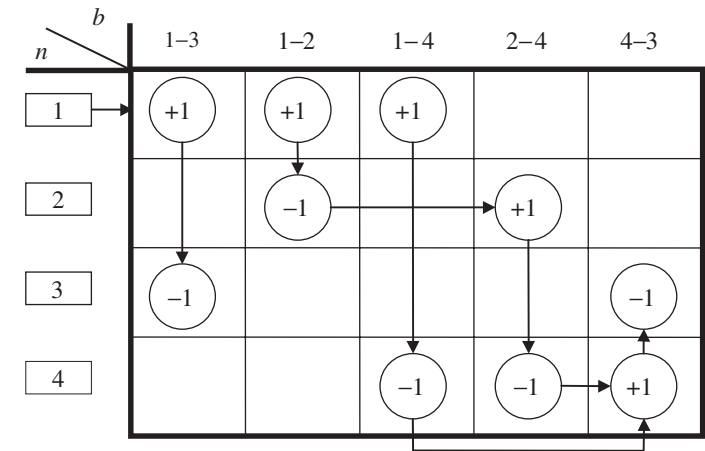
Figure 8.12 Branch–bus incidence matrix and branch search for the dominion of generator G_1
