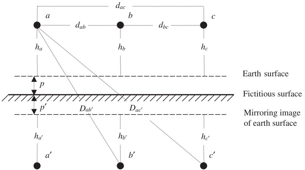
Figure 3.5 Line geometry showing the complex depth
