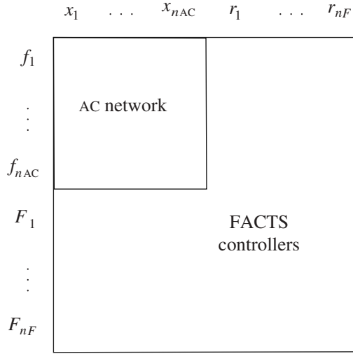
Figure 5.1 Augmented Jacobian
