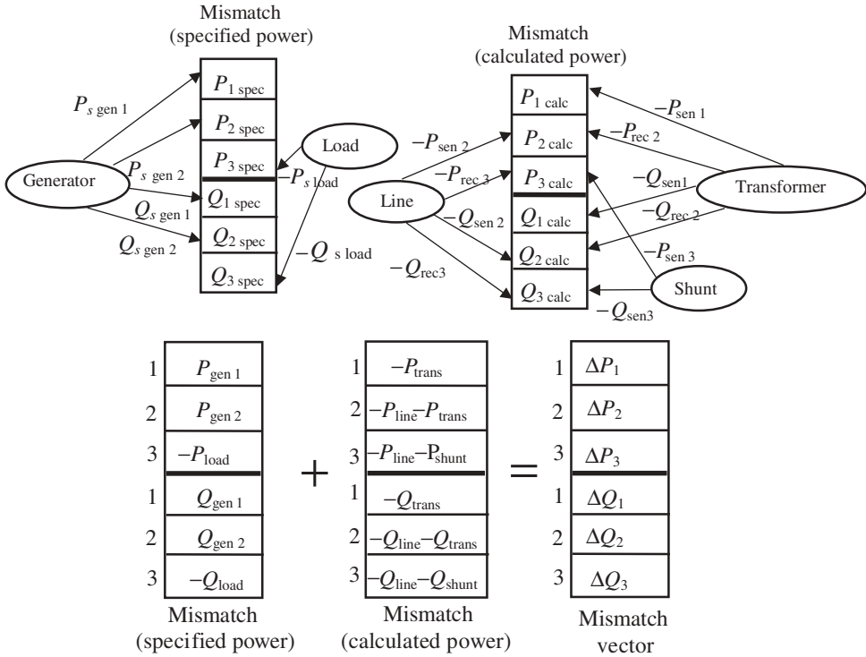
Figure 4.4 Power mismatch vector; subscripts 'sen' and 'rec' indicate the sending and receiving ends. Reproduced, with permission, from C.R. Fuente-Esquivel, E. Acha, S.G. Tan, and J.J. Rico, 'Efficient Object Oriented Power System Software for the Analysis of Large-scale Networks Containing FACTS Controlled Branches', IEEE Trans. Power Systems 3(2) 464–472, © 1998 IEEE
