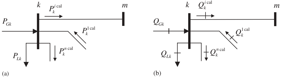
Figure 4.2 Power balance at bus k : (a) active power, and (b) reactive power
