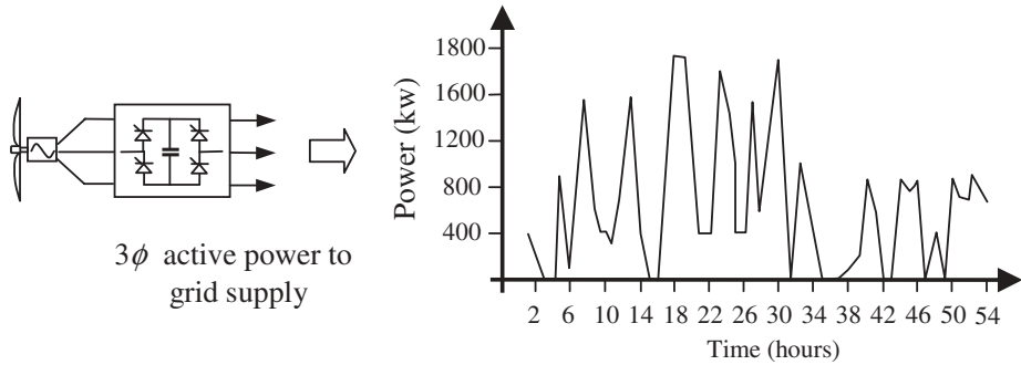
Figure 8.21 Wind generator model for power flow studies that caters for time dependency
