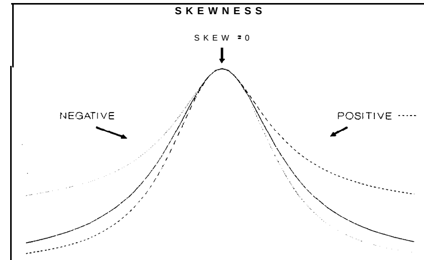
Figure 3-2 Skewness.
