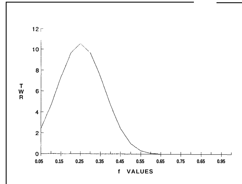
Figure 1-1 20 sequences of +2, -1.
