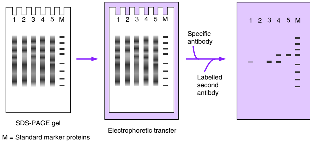
Figure 13.15 Western blotting
