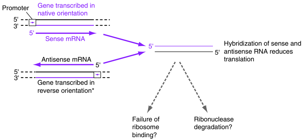
Figure 17.2 Antisense RNA
