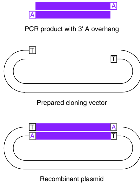
Figure 5.14 TA cloning
