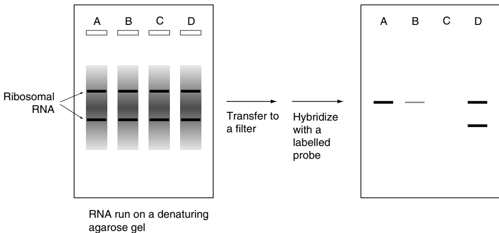
Figure 13.1 Northern blotting
