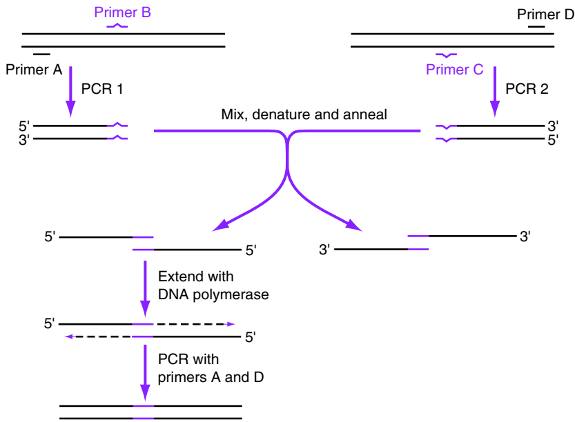
Figure 15.11 PCR-based mutagenesis
