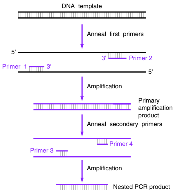
Figure 9.4 Nested PCR
