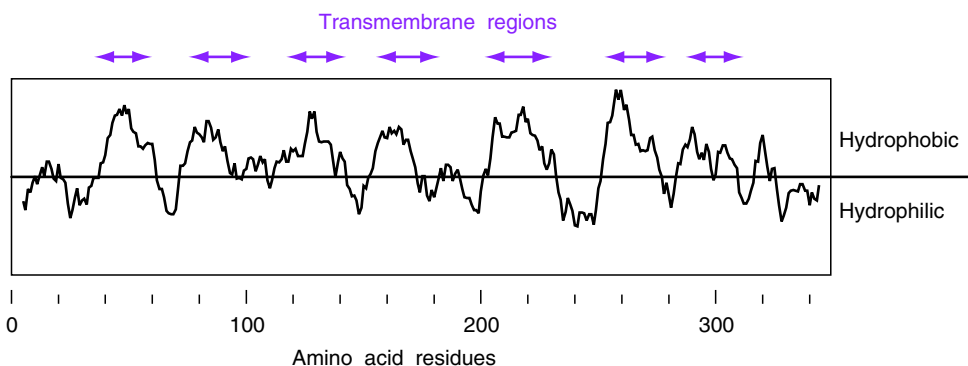
Figure 11.6 Hydrophobicity plot: the illustration shows a Kyte–Doolittle hydropathy plot for human rhodopsin (Swiss-Prot P08100); the hydrophobic regions represent transmembrane structures, with the intervening hydrophilic sequences alternating between cytoplasmic and external structures
