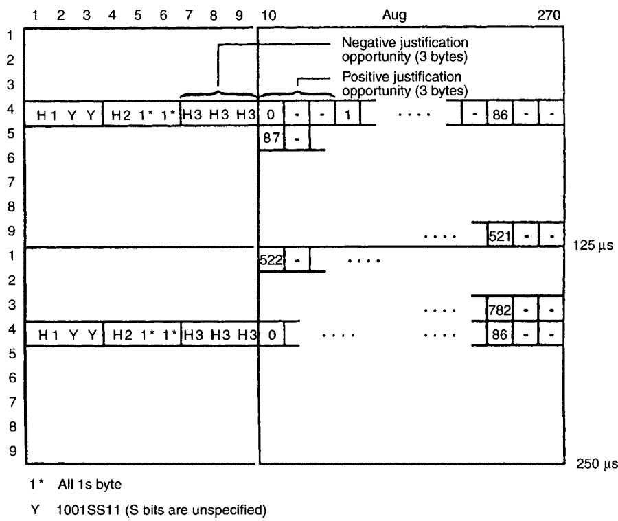
Figure 19.19 AU-4 pointer offset numbering. [From ITU-T Rec. G.709, Figure 3-1/G.709 (Ref. 7).]
