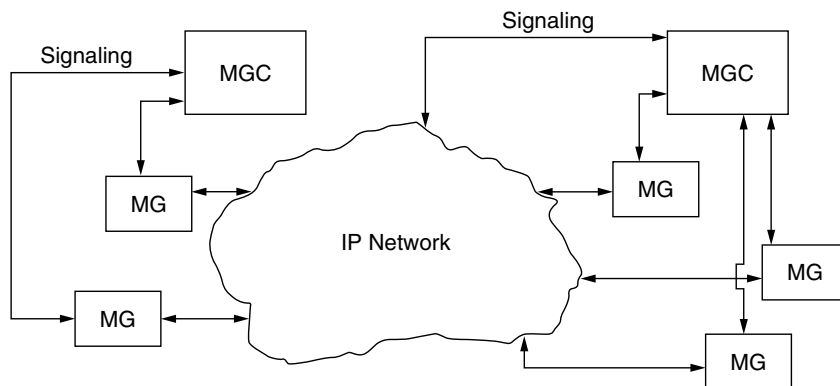
Figure 15.7 A media gateway controller (MGC) provides a signaling interface for media gateways (MG) and thence to the IP network.
