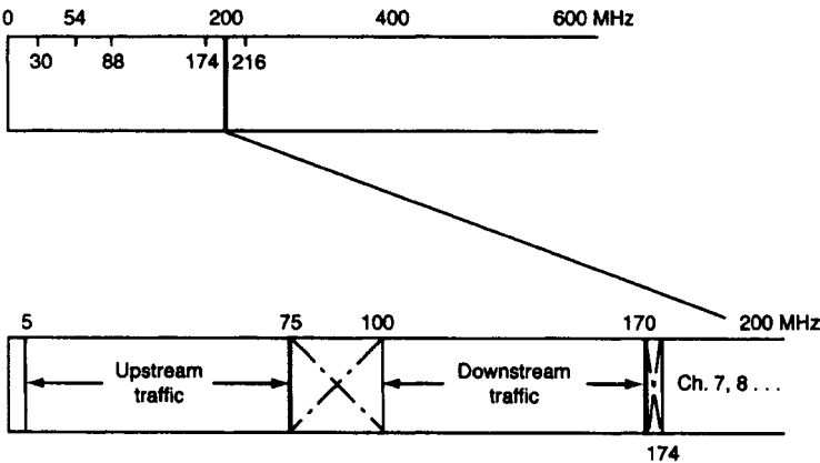
Figure 17.16b CATV spectrum with equal upstream and downstream bandwidth for other services.
