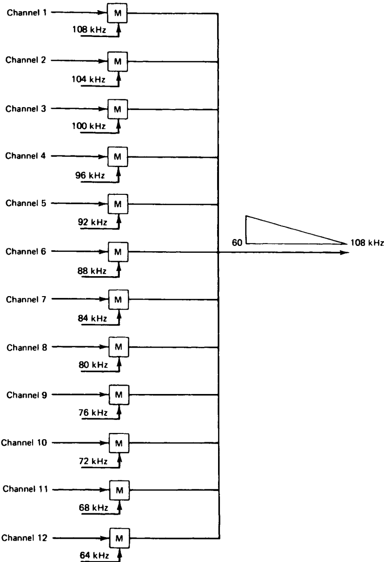
Figure 4.19 Formation of the standard CCITT group.
