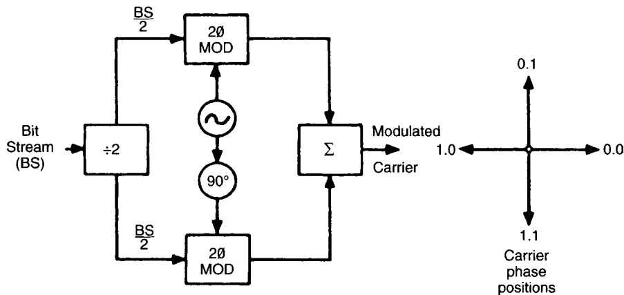
Figure 9.11 Conceptual block diagram of a QPSK modulator. Note that these are two BPSK modulators working jointly, and one modulator is 90^\circ out of phase with the other. The first bit in the bit stream is directed to the upper modulator, the second to the lower, the third to the upper, and so on.
