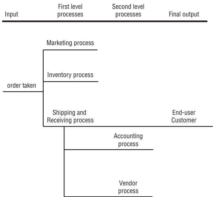
FIGURE 5.1 CTQ tree.
