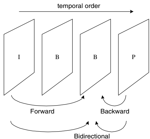
Figure 5.19 Prediction modes for B-VOP
