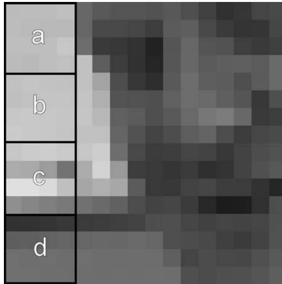
Figure 6.31 16 \times 16 luma macroblock showing block edges
