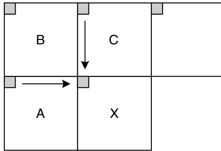
Figure 5.14 Prediction of DC coefficients
