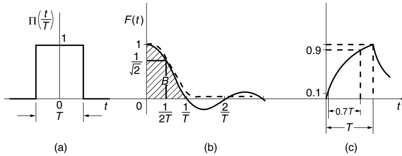
Figure 16.29 Relationship between NRZ pulse, its Fourier transform, and the output of an amplifier with B = 1/2T . (a) NRZ pulse in the time domain. (b) NRZ pulse in the frequency domain. (c) Output from an amplifier with B = 1/2T .
