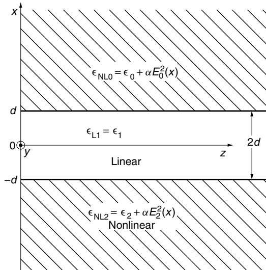
Figure 15.8 Geometry of a three-layer optical guide with a linear core and nonlinear identical claddings.
