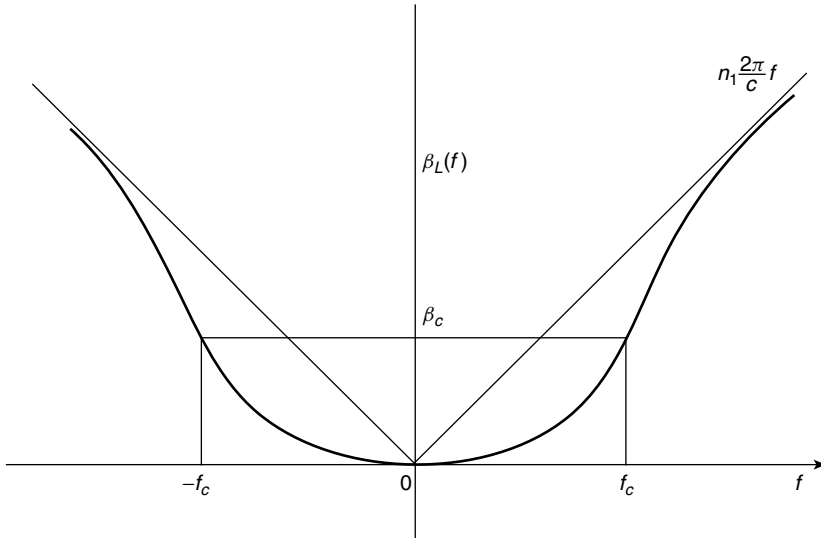
Figure 15.17 Propagation constant \beta(f) of the HE_{11} mode in a step index fiber.
