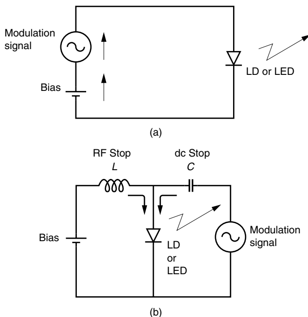
Figure 16.4 Amplitude modulation of a radiant diode. (a) Series circuit modulation. (b) Shunt circuit modulation.
