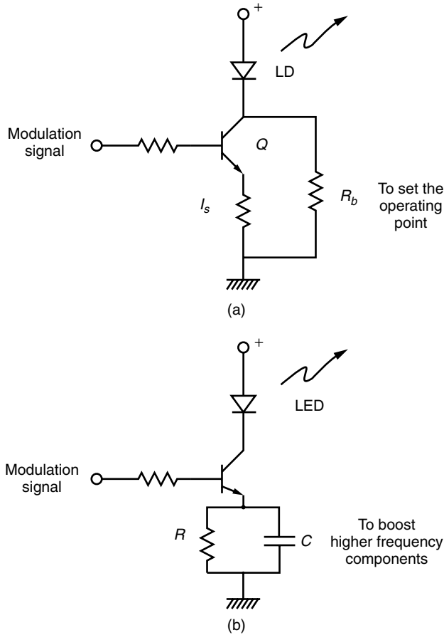
Figure 16.7 Drivers with pre-enhancement. (a) Driver with pre-biasing. (b) Driver with pre-emphasis.
