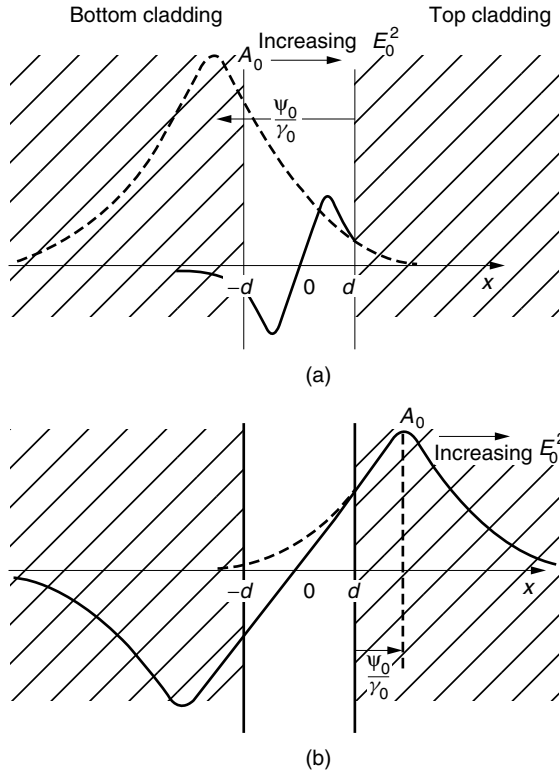
Figure 15.10 Change in the TE 1 mode field pattern with the field intensity E_0^2 . (a) TE 1 mode with lower field intensity. (b) TE 1 mode with higher field intensity.
