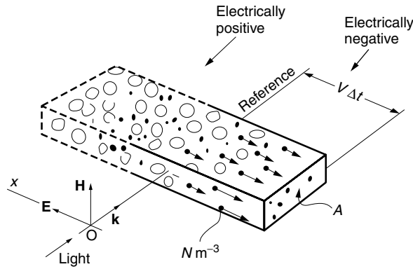
Figure 14.19 The movement of charge across a reference cross section is the plasma current.
