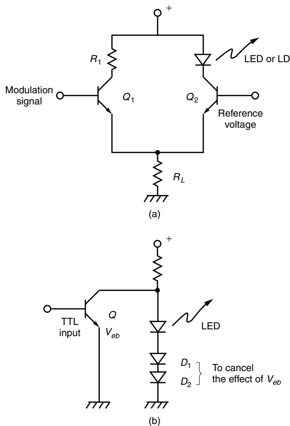
Figure 16.6 Circuits for modulating an LED. (a) Emitter coupled circuit. (b) Parallel switching.
