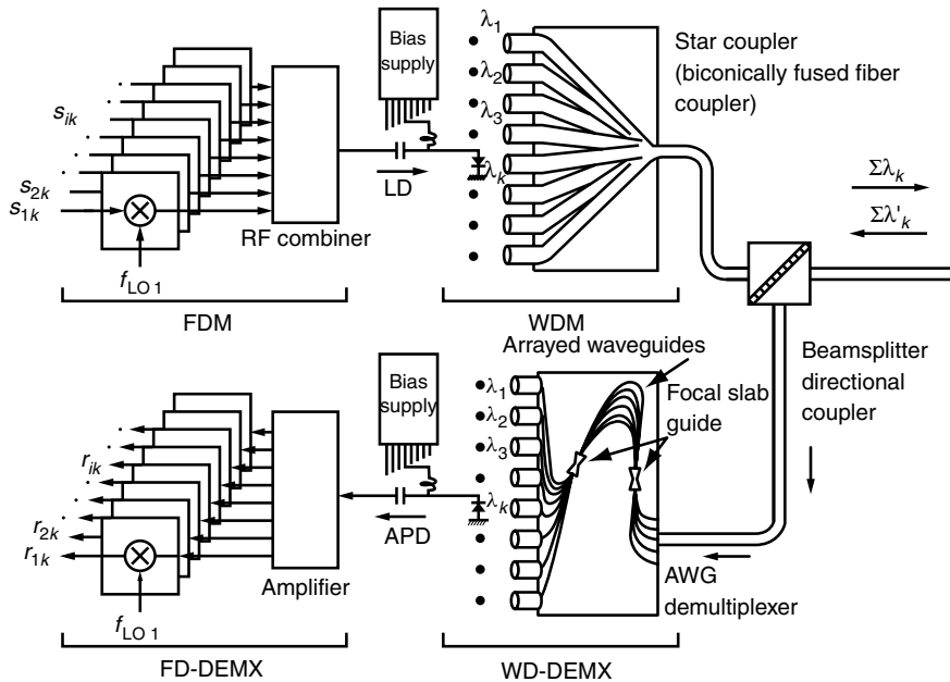
Figure 16.10 Bidirectional WDM combined with FDM.
