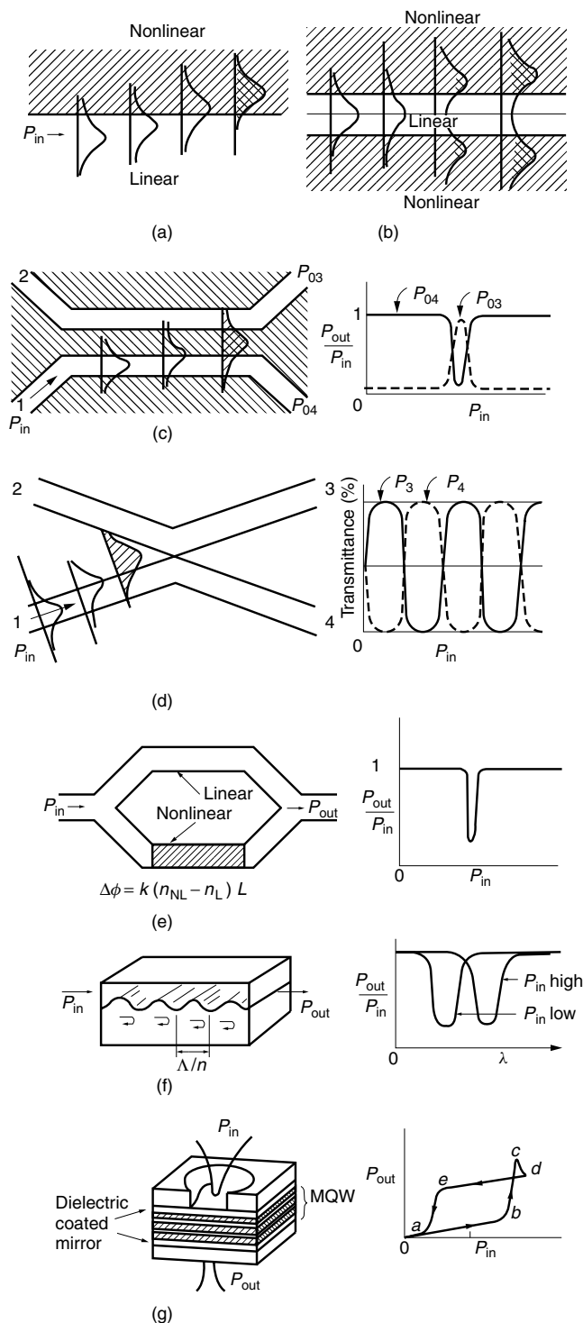
Figure 15.1 Devices based on Kerr nonlinear optics. (a) Guided nonlinear boundary wave. (b) Nonlinear guide. (c) Nonlinear directional coupler. (d) Nonlinear X junction. (e) Mach-Zehnder interferometer. (f) Nonlinear distributed feedback grating. (g) Optical bistability.
