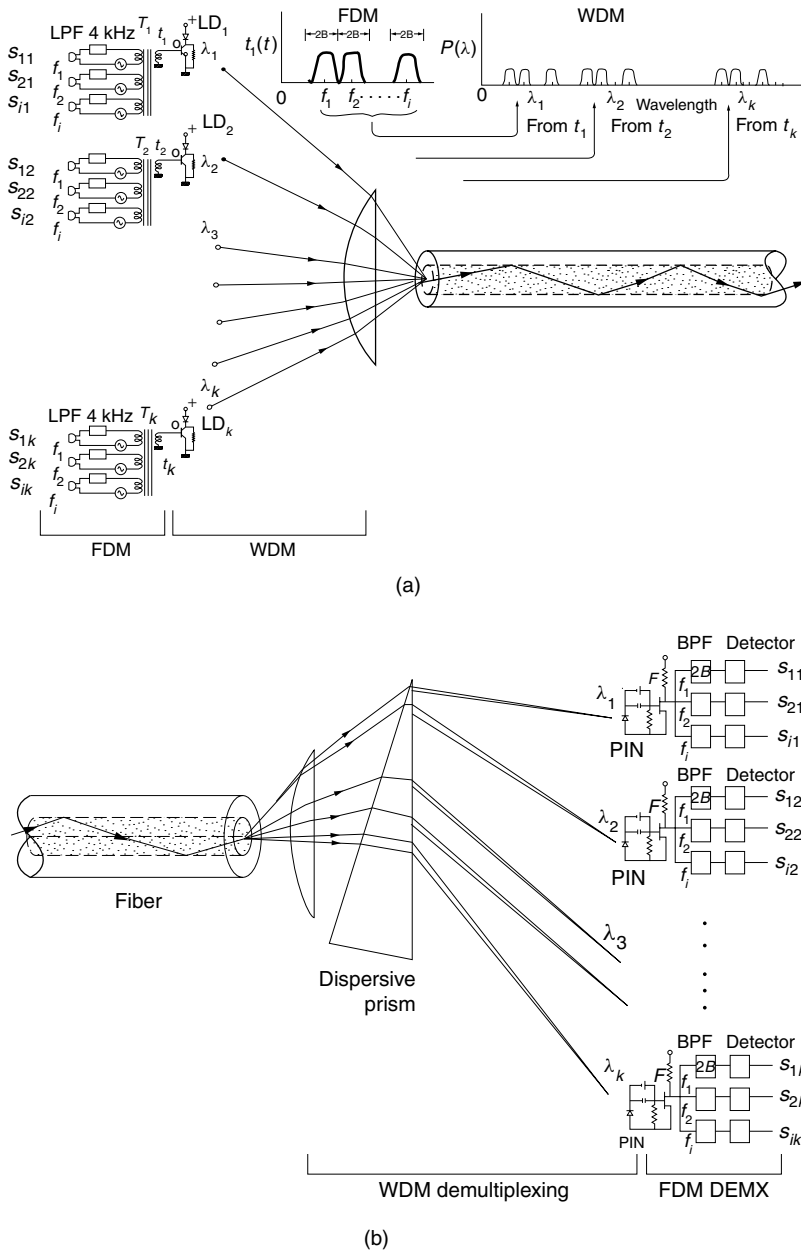
Figure 16.9 (a) WDM combined with FDM. (b) Demultiplexing of WDM combined with FDM.
