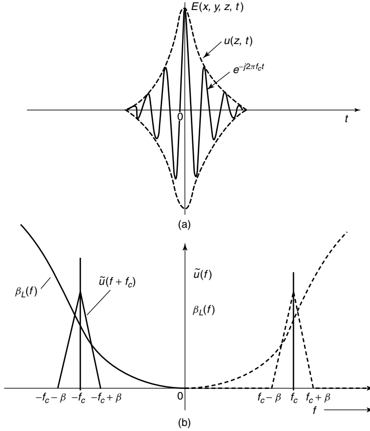
Figure 15.16 Soliton pulse in the time and frequency domains. (a) Soliton pulse E(x, y, z, t) . (b) Spectrum of the soliton pulse.
