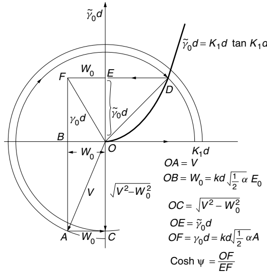
Figure 15.11 Graphically finding \gamma_0 d and \cosh \psi .
