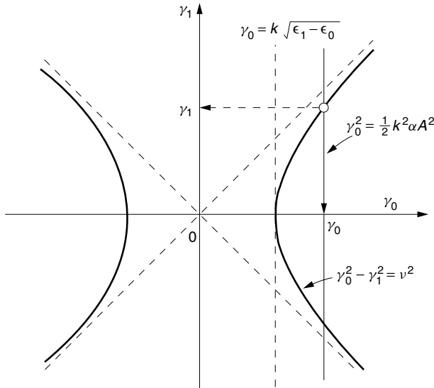
Figure 15.5 Plots of the characteristic equation of the guided nonlinear boundary wave.
