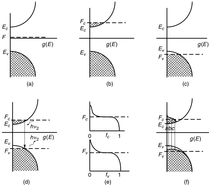
Figure 14.3 Density of state function g(E) and the Fermi-Dirac distribution. (a) T = 0 , J = 0 , pure semiconductor. (b) T = 0 , J = 0 , n-doped semiconductor. (c) T = 0 , J = 0 , p-doped semiconductor. (d) T = 0 , J = 0 , p-n junction. (e) Fermi-Dirac distribution. (f) T \neq 0 , J = 0 , p-n junction.
