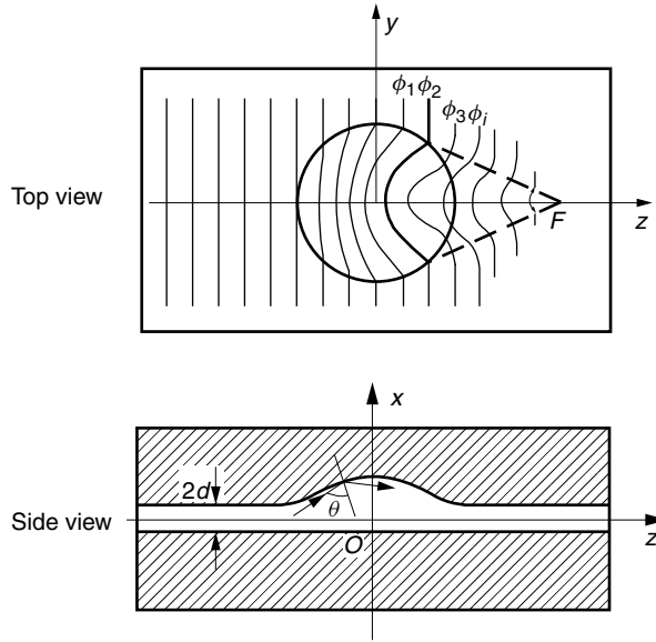
Figure 9.7 Mode-index lens used for integrated optics devices.
