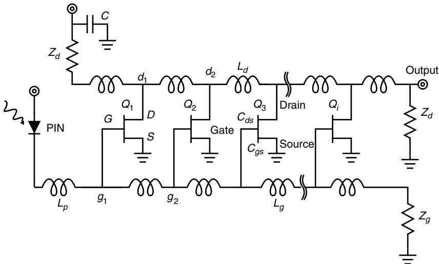
Figure 16.17 Diagram of distributed preamplifiers. (After A. P. Freundorfer and P. Lionais [25].)
