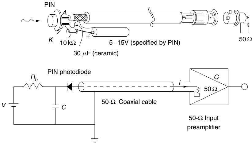
Figure 16.14 PIN photodiode connected to a 50-Ω input preamplifier.
