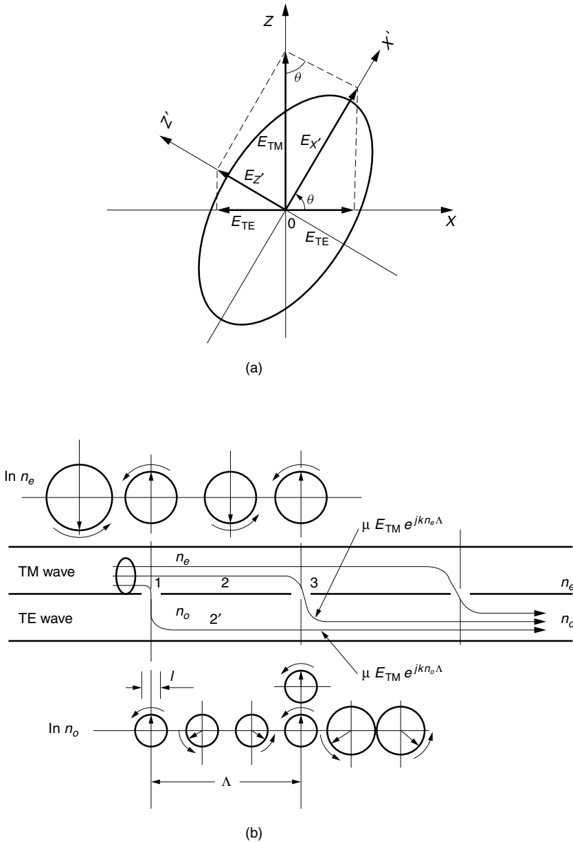
Figure 10.21 Mode converter principle. (a) Rotation of the elliptical cross section of the indicatrix due to \varepsilon_x . (b) Coupling from the TM wave to the TE wave.
