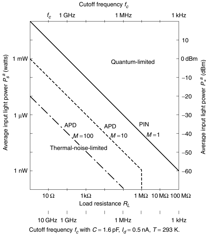
Figure 16.22 Borderline between quantum-limited and thermal-noise-limited cases of PIN and APD photodiodes.
