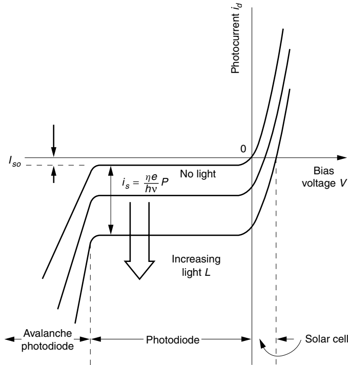
Figure 16.12 Current–voltage characteristic of a p-n junction.
