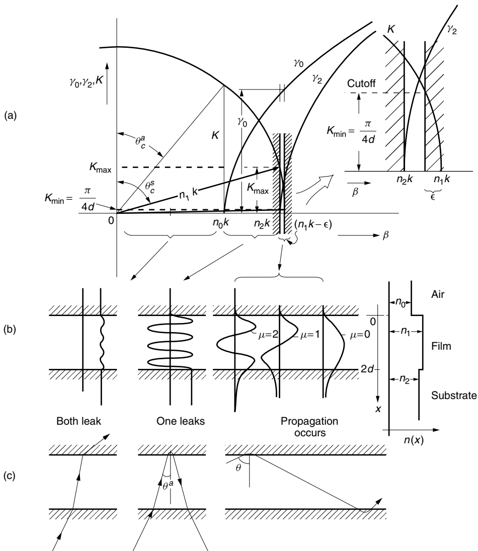
Figure 9.15 Combined chart of an asymmetric optical guide. (a) K - \beta diagram. (b) Amplitude distribution. (c) Ray path.
