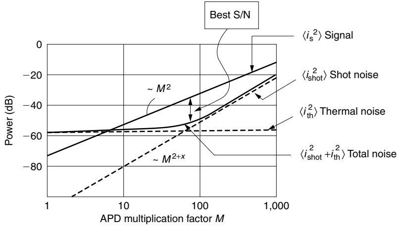
Figure 16.20 Dependence of signal and noise powers of an APD on the multiplication factor M .
