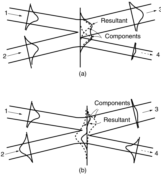
Figure 10.17 Optical magic T. (a) Arms 1 and 2 are fed in phase. (b) Arms 1 and 2 are fed out of phase.
