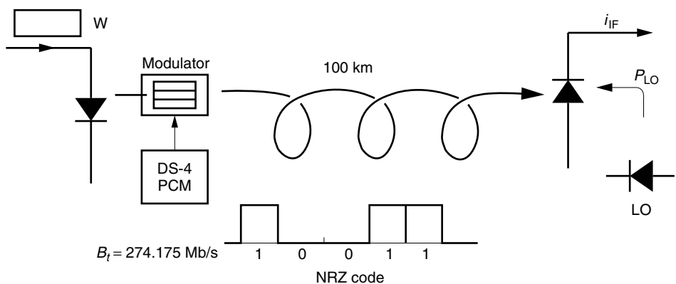
Figure 16.32 Layout of Example 16.5.
