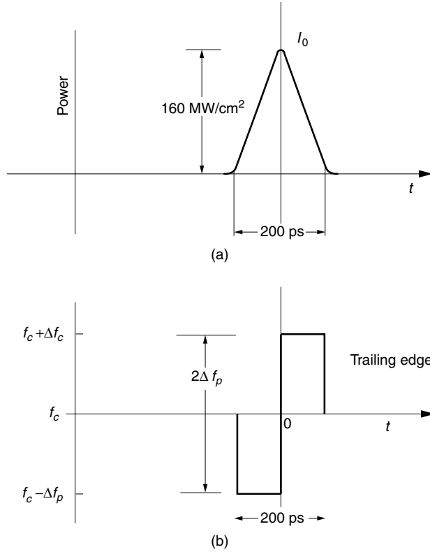
Figure 15.13 Frequency spread due to self-phase modulation (SPM) in a Kerr medium. (a) Triangular pulse with smooth edges. (b) Frequency spread due to SPM effect.
