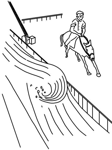
John Scott-Russell galloping after a solitary wave in a Scottish canal in 1838.
