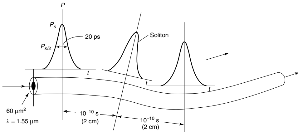
Figure 15.19 Soliton-based optical communication.
