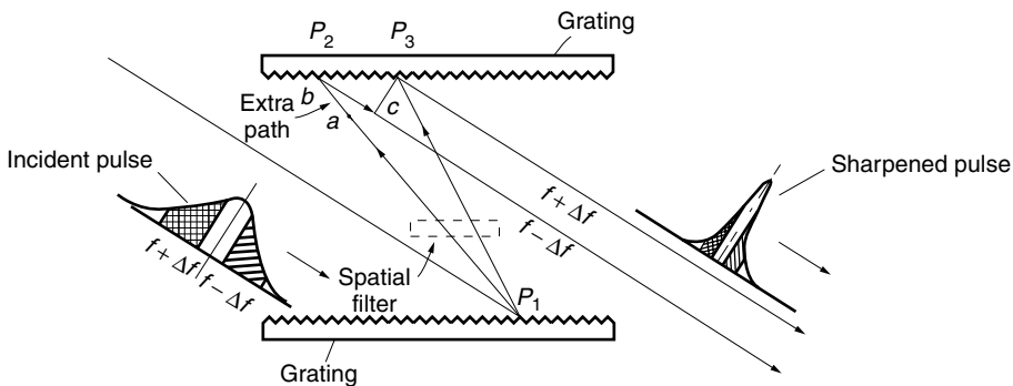
Figure 15.15 A diffraction grating used for sharpening a chirped pulse.
