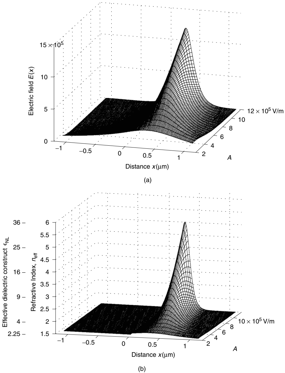
Figure 15.6 Field and refractive index distribution of the nonlinear boundary wave. (Calculations courtesy of D. Khomarlou.) (a) Electric field distribution as a function of x for values of A . (b) Refractive index as a function of x for values of A .
