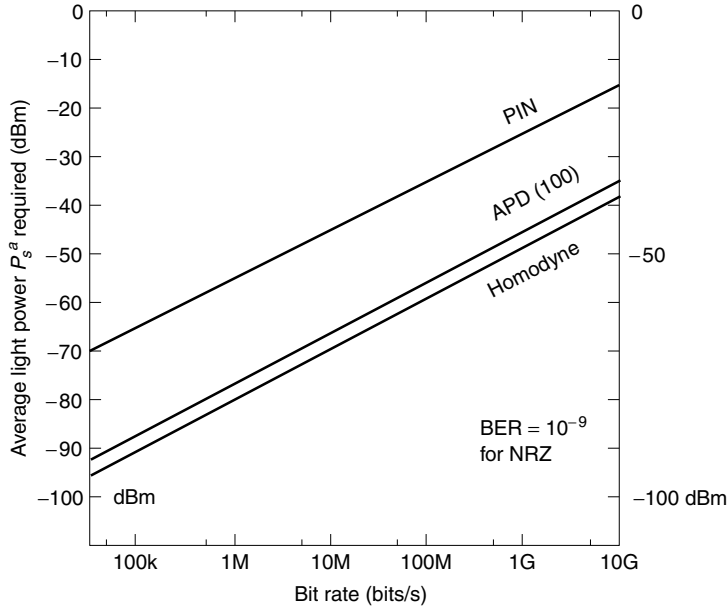
Figure 16.30 Input average light power P_s^a versus bit rate (bits/s) for NRZ code. For the value of the RZ code add 3 dB. The PIN photodiode and APD are thermal noise limited but the homodyne is quantum limited.
