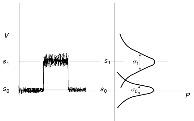
Figure P16.8 A pulse with different probability density function for “0” and “1” states.
