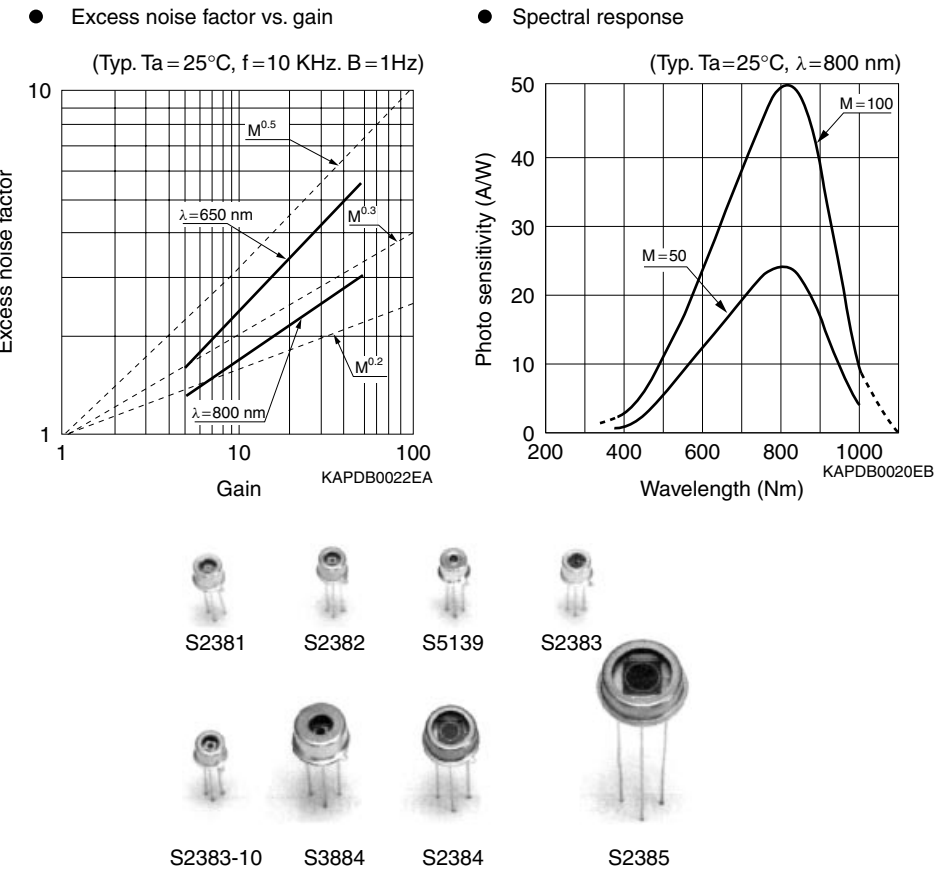
Figure 16.21 APD characteristics. (From Hamamatsu Photonics catalogue [19].)
