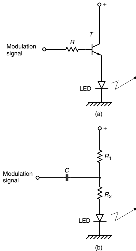
Figure 16.5 Simple circuits to modulate an LED. (a) Emitter follower (series connection). (b) RC coupling (shunt connection).
