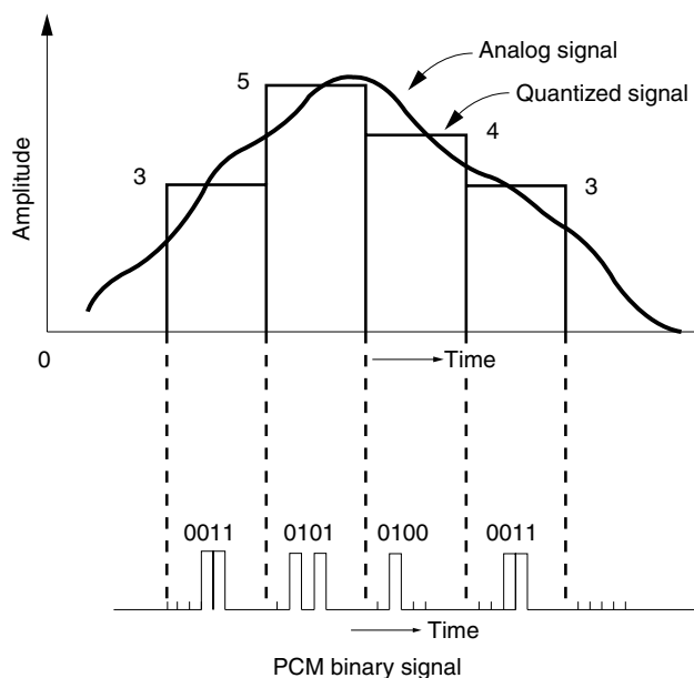
Figure 16.3 Principle of pulse code modulation (PCM).
