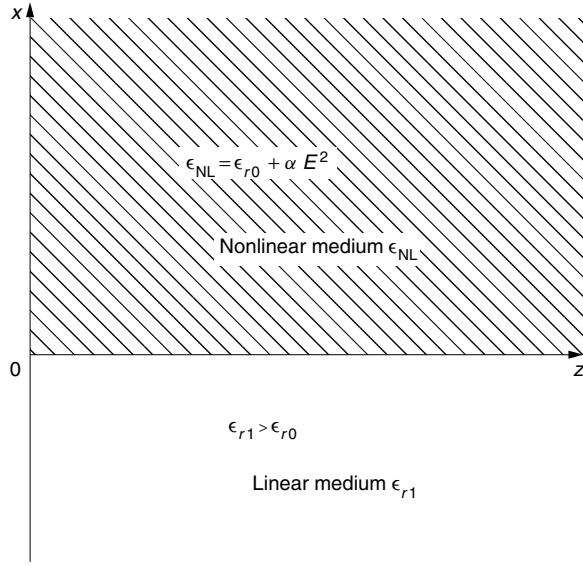
Figure 15.3 Combination of linear and nonlinear half-spaces.
