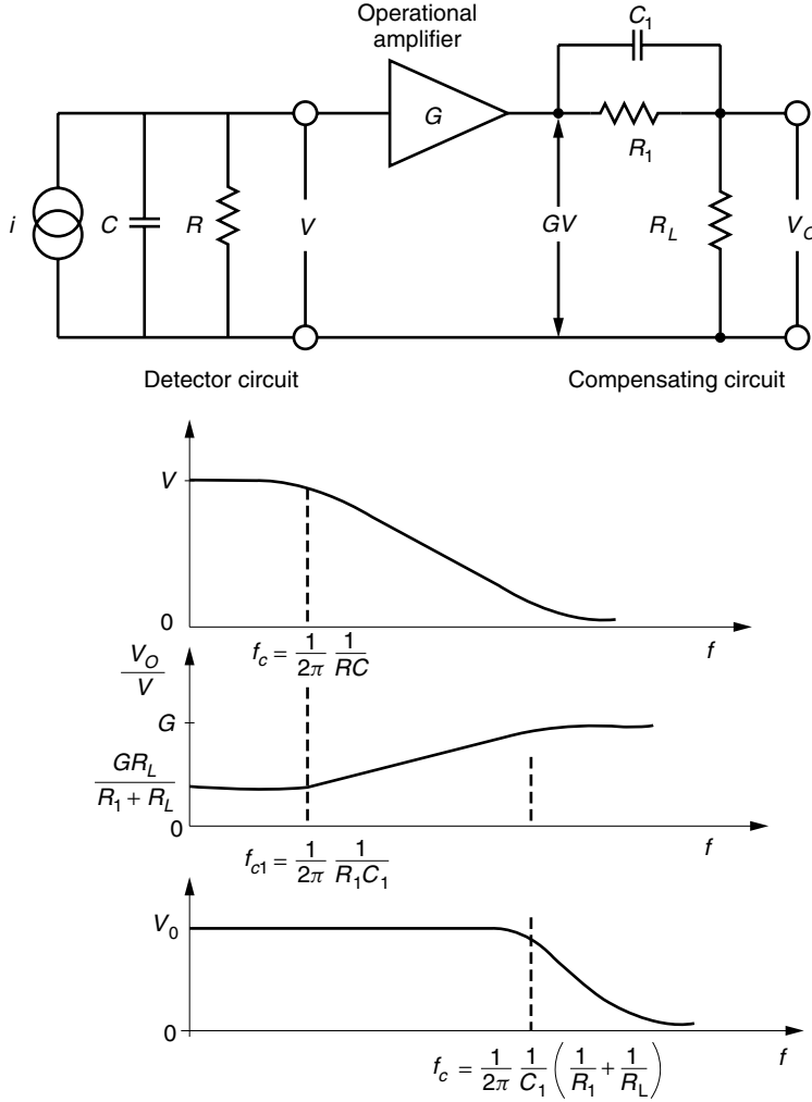
Figure 16.15 High impedance with a compensation circuit.
