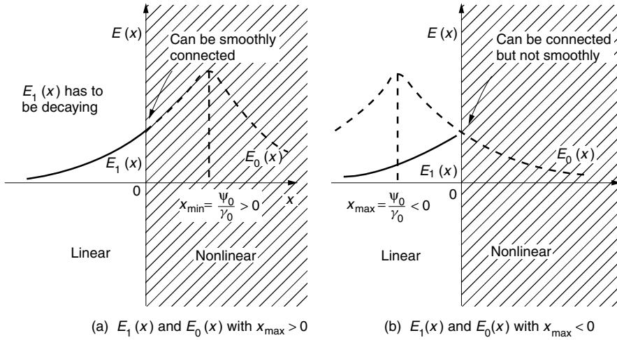
Figure 15.4 Possible combinations of solutions. Case (a) satisfies the boundary condition but case (b) does not.
