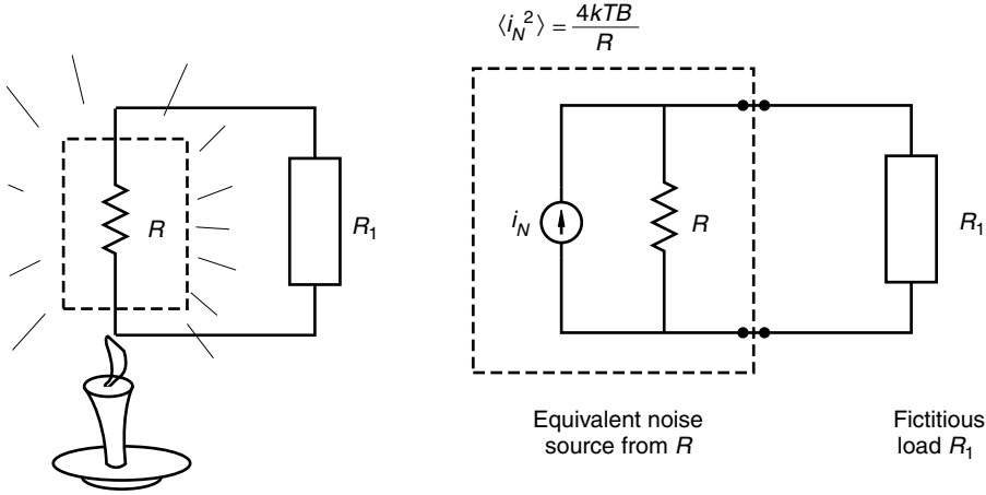
Figure 16.19 The equivalent circuit of noise from resistor R . \langle i_N^2 \rangle is determined such that the noise source delivers a noise power of kTB when R_1 is selected to be R .
