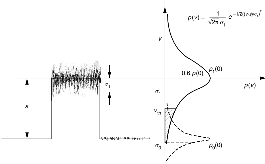
Figure 16.23 Pulse with Gaussian noise in “1.” The noise in “0” is suppressed for clarity.
