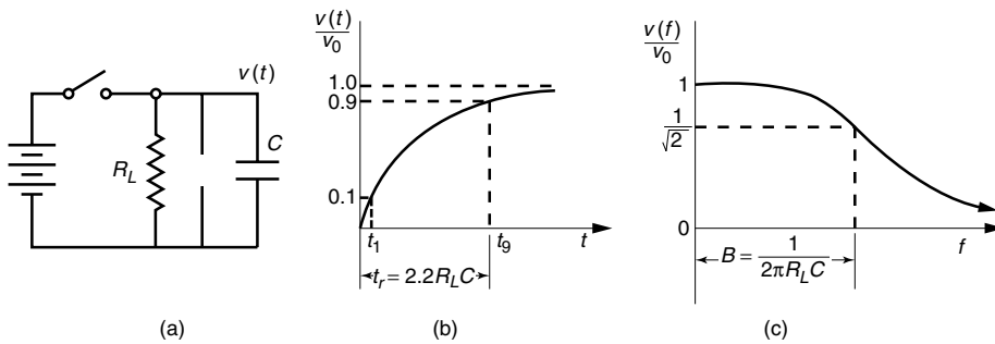
Figure 16.26 Relationship between rise time and frequency response of an RC circuit to show Bt_r = 0.35 by eliminating R_L C from the expressions. (a) RC circuit. (b) Rise time. (c) Frequency response.
