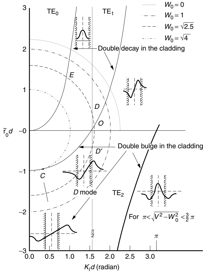
Figure 15.9 Solutions in a waveguide with V = \sqrt{5.0} : even and odd modes for both linear and nonlinear cases. (After Y. F. Li and K. Iizuka [11].)
