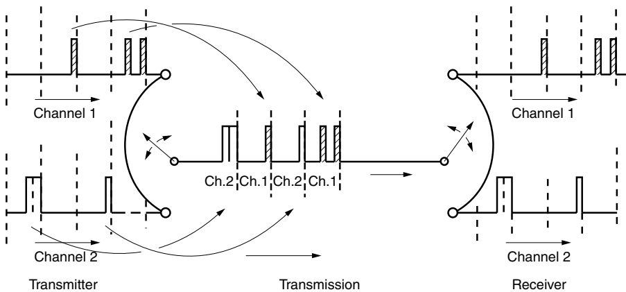
Figure 16.11 Time division multiplexing (TDM) and demultiplexing.
