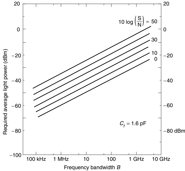
Figure 16.25 Required average light power of a PIN photodiode as a function of frequency bandwidth B with S/N as a parameter. The modulation is analog and the S/N is thermal noise limited. C_f = 1.6 pF.
