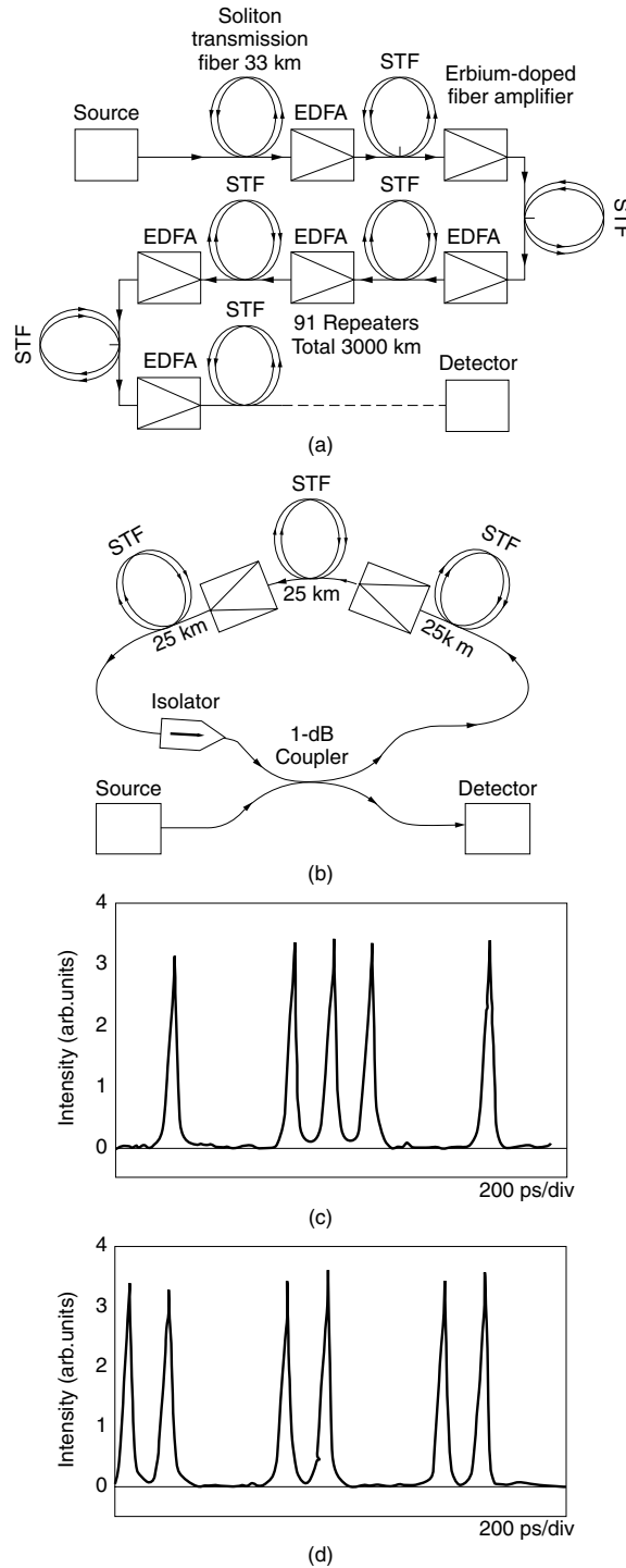
Figure 15.20 Arrangements for soliton experiments. (a) A 3000-km soliton transmission. (b) A loop to simulate long-distance transmission of a soliton. (c) Transmitted data pattern at 10 Gbs over 50 million kilometers of simulated length coded as (0100111001). (d) Transmitted data pattern at 10 Gbs over 180 million kilometers of simulated length coded as (1100110011). (After M. Nakazawa [16].)
