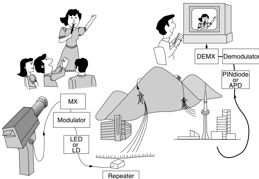
Figure 16.1 Pictorial block diagram of fiber-optic communication system. MX: Multiplexer. DEMX: Demultiplexer. LED: Light emitting diode. LD: Laser diode. APD: Avalanche photodiode.
