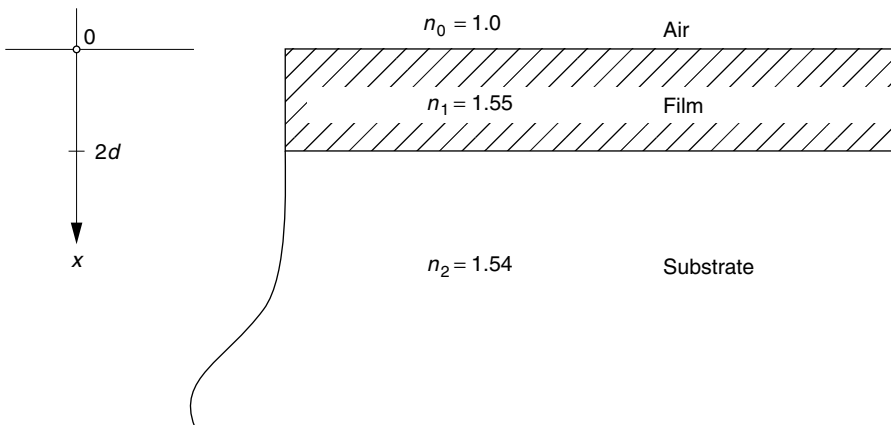
Figure 9.14 Geometry of an asymmetric slab optical guide.
