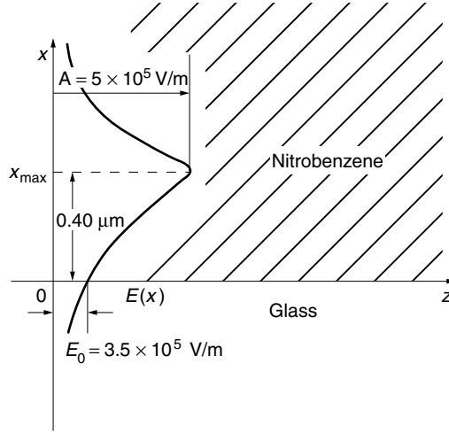
Figure 15.7 Guided wave excitation at the interface between linear and nonlinear media: the results of Example 15.1.
