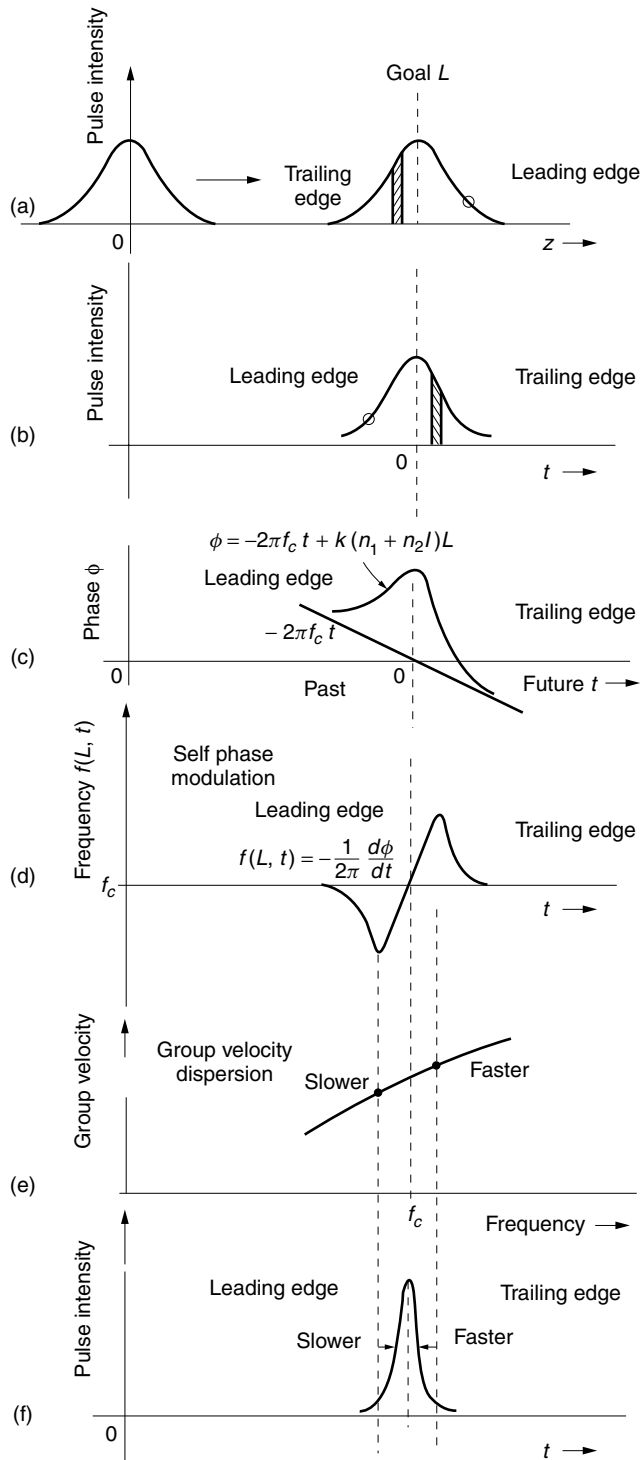
Figure 15.12 Explanation of the formation of a soliton wave.
