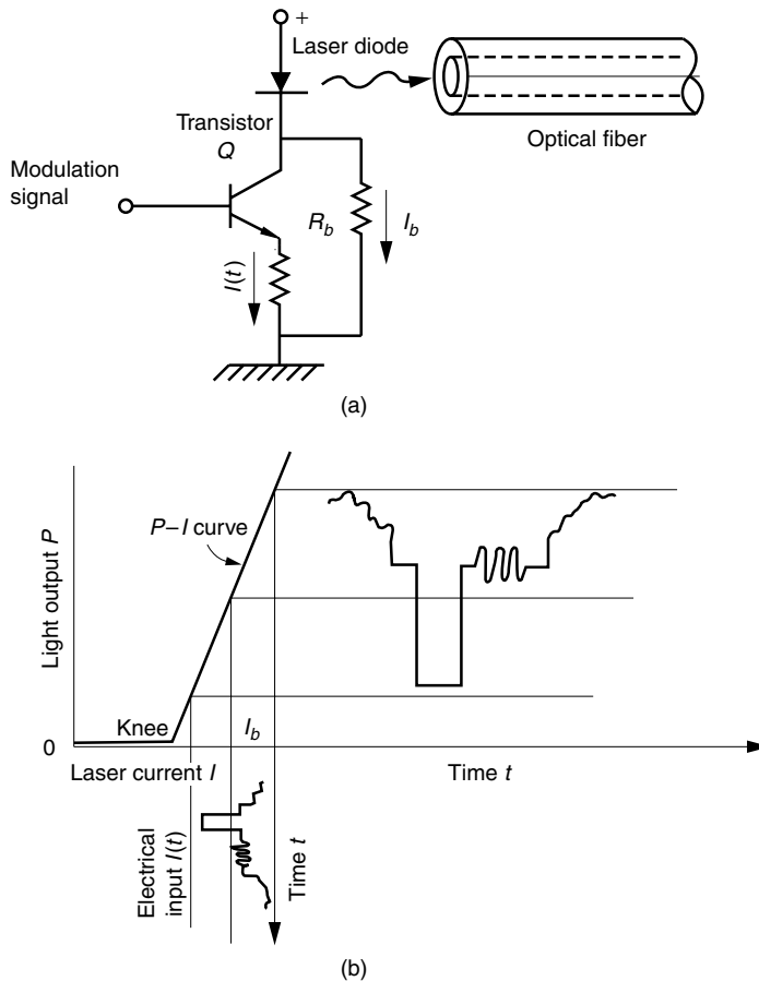
Figure 16.2 Modulation of laser light by an electrical signal. (a) Circuit for modulating a laser diode. (b) Light output versus injection current ( P – I curve).
