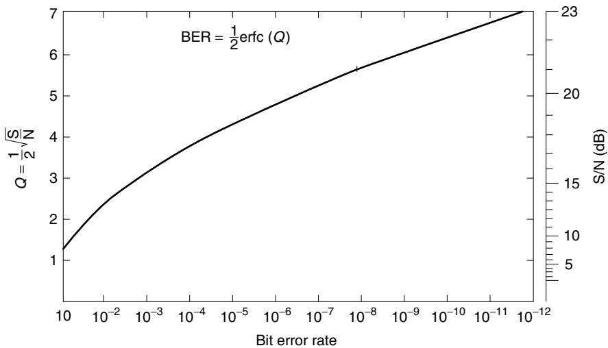
Figure 16.24 Bit error rate versus Q and S/N in dB.
