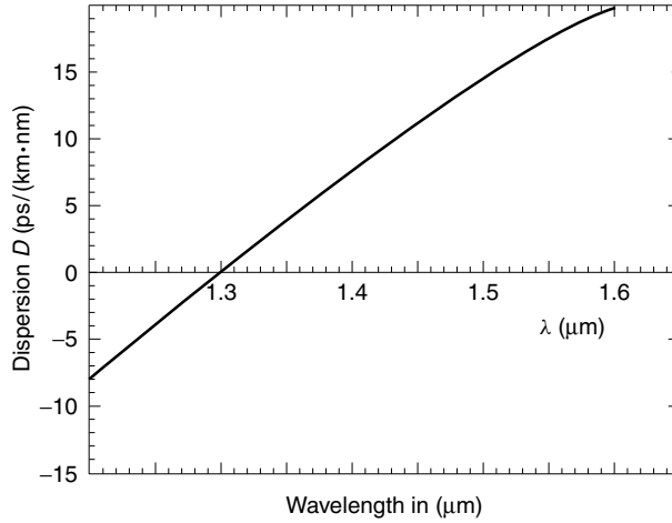
Figure 15.14 Dispersion parameter for calculating group velocity dispersion (GVD) of a single-mode optical fiber.
