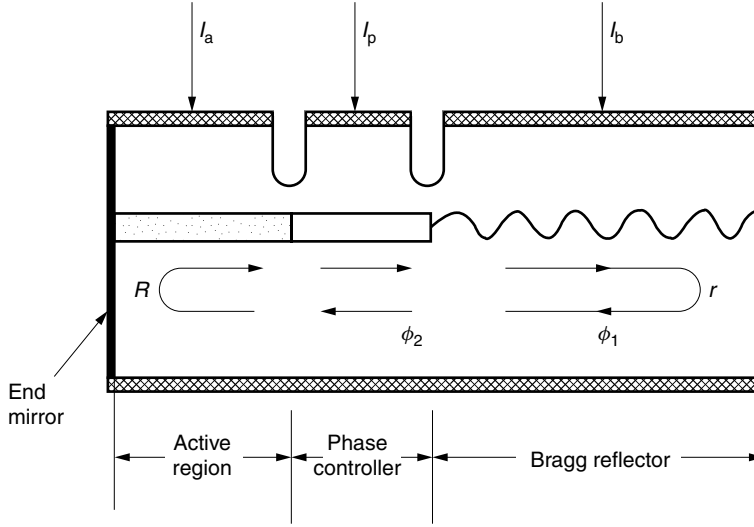
Figure 14.41 Structure of the DFB laser.
