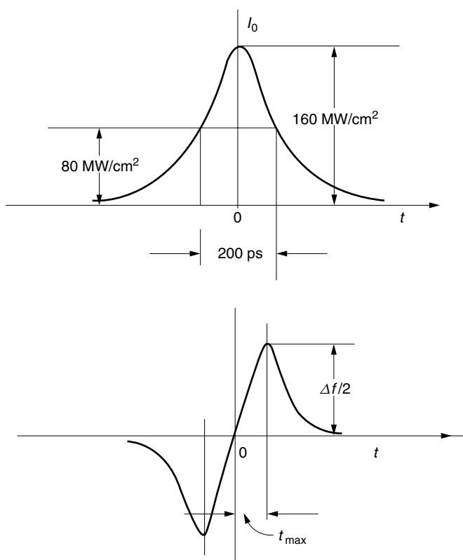
Figure P15.3 Gaussian pulse (top) and self-phase modulation (bottom) due to nonlinearity.
