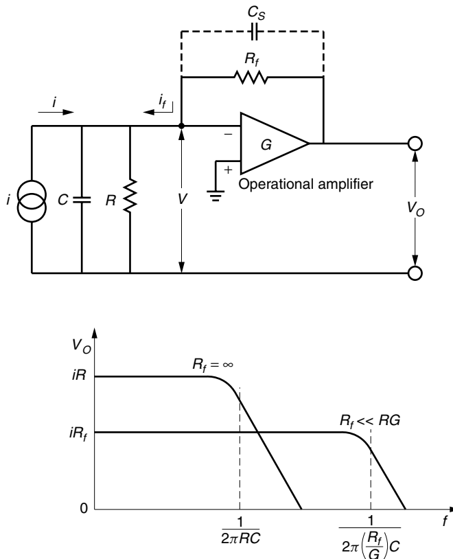
Figure 16.16 Transimpedance coupling.
