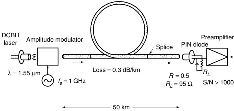
Figure 16.27 Another example of an analog system design.
