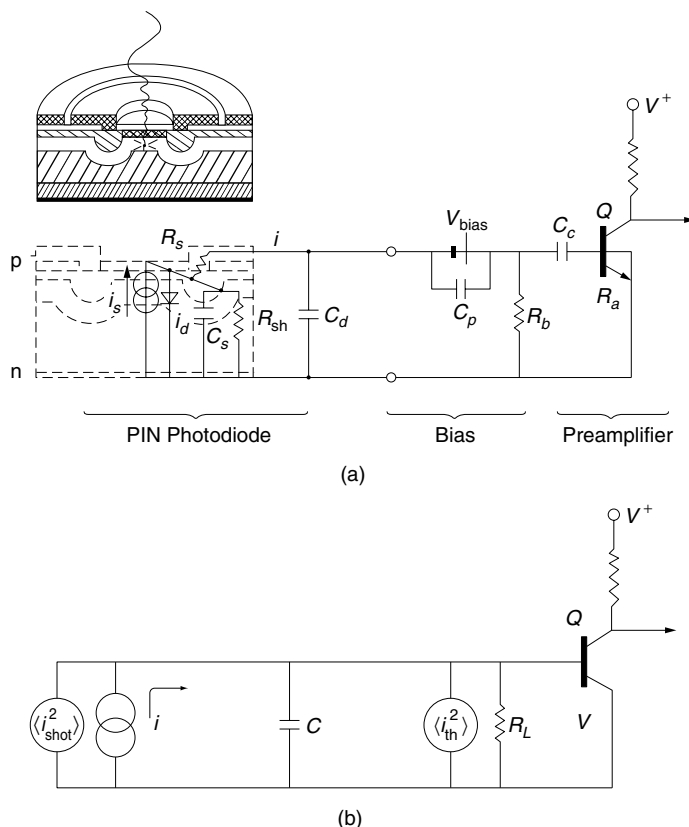
Figure 16.13 Equivalent circuits of a PIN diode. (a) Connection diagram of PIN photodiode. (b) Simplified equivalent circuit including noise sources.
