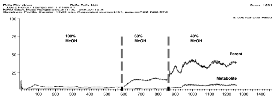
Figure 8.3. Systematic method development: mobile-phase choice using infusion experiment.
