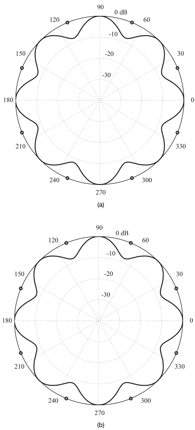
Figure 2.13. Omnidirectional patterns with N = 8 and d/\lambda = 0.65 . (a) Computed from a summation over all elements; (b) directly from a summation of three phase modes (cf. Figure 2.7).
