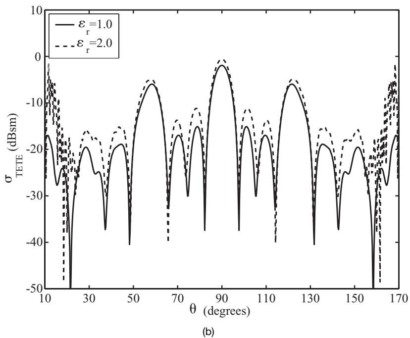
Figure 11.22. The H -plane RCS for a 4 \times 32 element array with a dielectric coating (dashed line). The noncoated case is included as reference (solid line). (a) 4.3 GHz. (b) 6.8 GHz.
