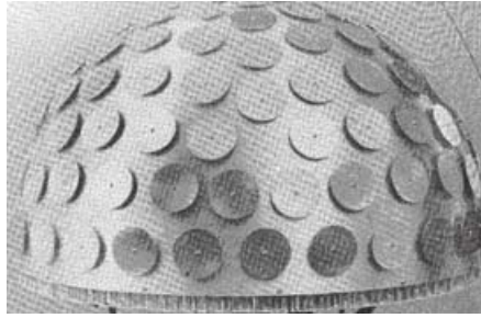
Figure 8.55. The ESSA hemispherical array with patch elements (electronically switched spherical array) [Stockton and Hockensmith 1977, 1979; Mailloux et al. 1981].
