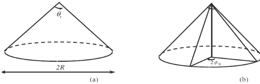
Figure 3.14. Cone parameters. (a) cone angle \theta_t and (b) active sector 2\phi_0 .
