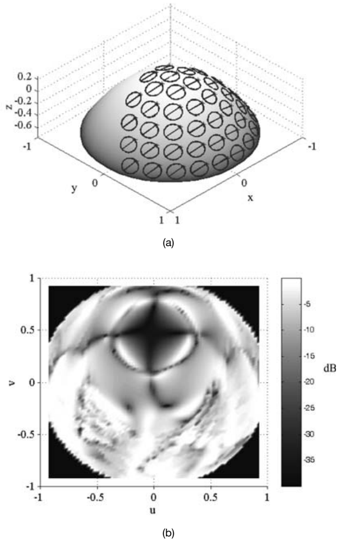
Figure 8.43. (a) The array configuration (first set of dipoles). (b) Shows the cross polarization expressed as isolation (in decibels) between the two fields that result from, respectively, the first set of dipoles and a second set of dipoles. The second set consists of dipoles that are orthogonal to the respective dipoles of the first set at each element location.
