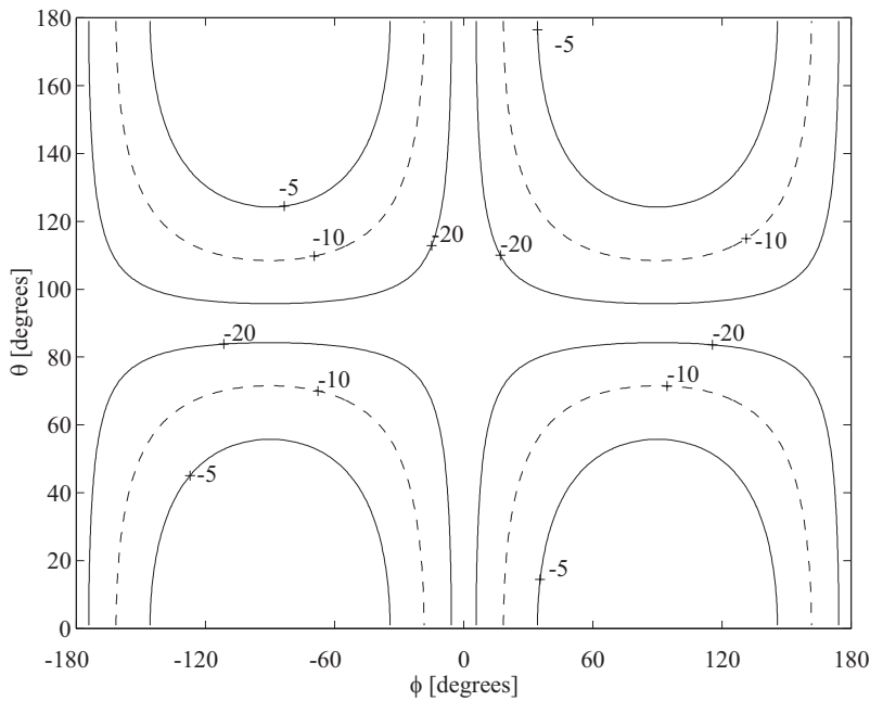
Figure 8.29. Cross polarization levels for the horizontal dipole when the polarization reference axis is vertical. Contour lines at -5 , -10 , and -20 dB levels.
