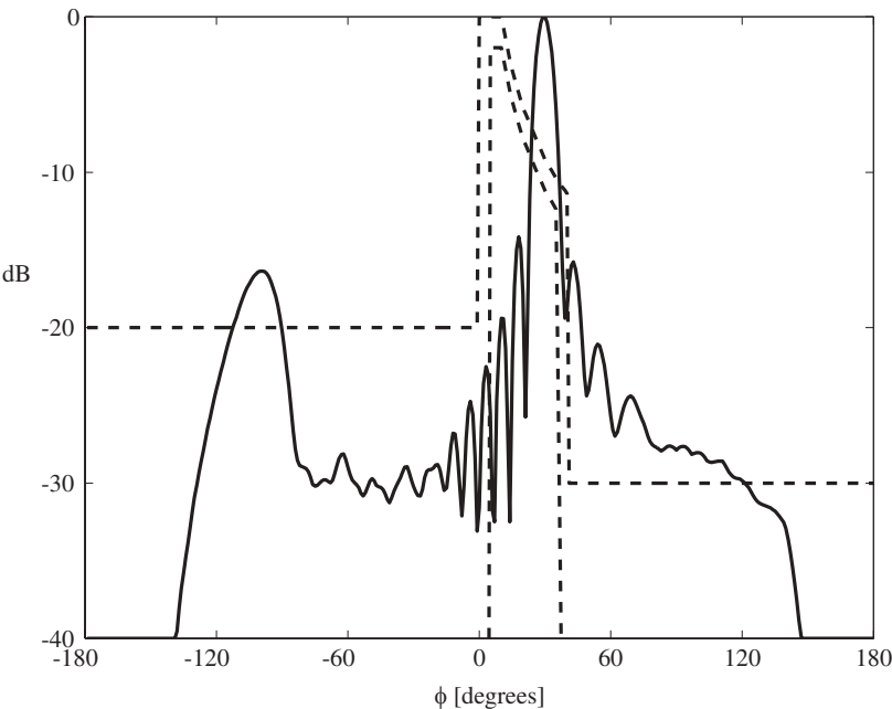
Figure 10.11. Starting case: Equal amplitude excitation with the main beam directed at 30 degrees. Dashed lines represent the requirement template.
