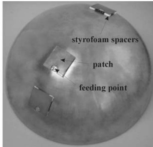
Figure 7.31. The experimental microstrip patch antenna [Burum et al. 2004]. Copyright (2003) Wiley Periodicals, Inc. Reprinted by permission of John Wiley & Sons, Inc.
