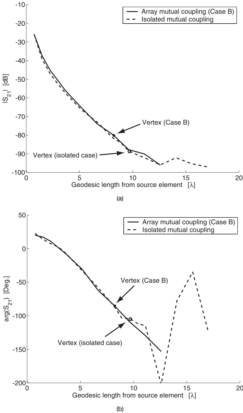
Figure 7.23. Comparison between the array and isolated H -plane mutual coupling along the y axis of the experimental antenna ( f = 8.975 GHz). Note that the array mutual coupling shown is measured from element -y_{11} , whereas the isolated coupling is measured from element -y_{13} [Lanne and Josefsson 2002]. (a) Amplitude. (b) Phase.
