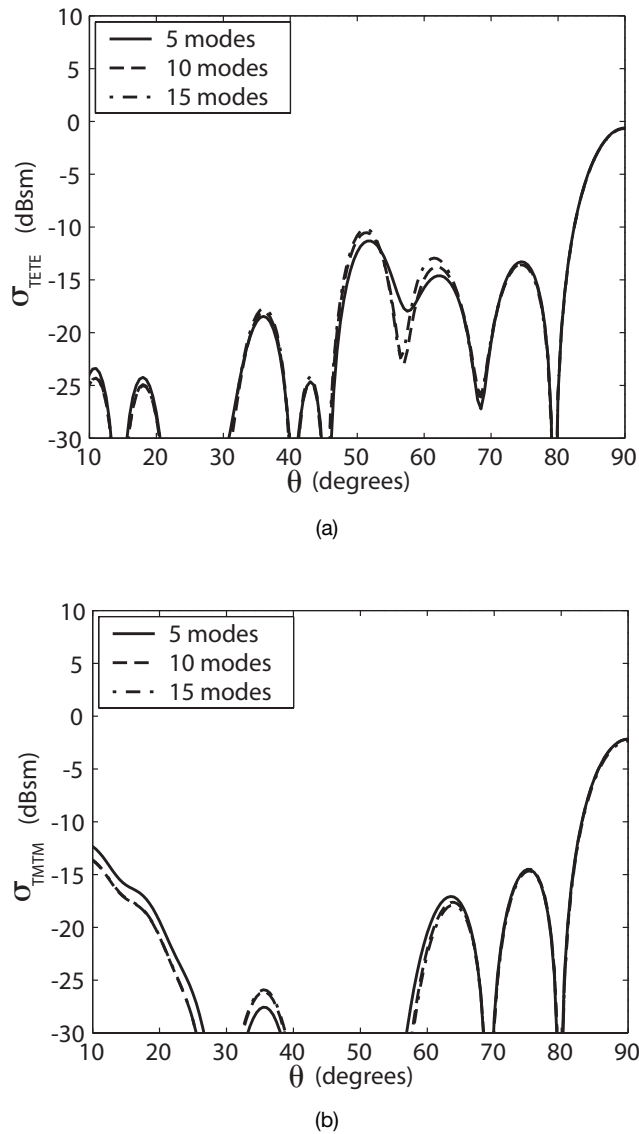
Figure 11.10. H -plane results for 6.8 GHz with up to 15 waveguide modes. (a) \sigma_{TETE} . (b) \sigma_{TM_{TM}} .
