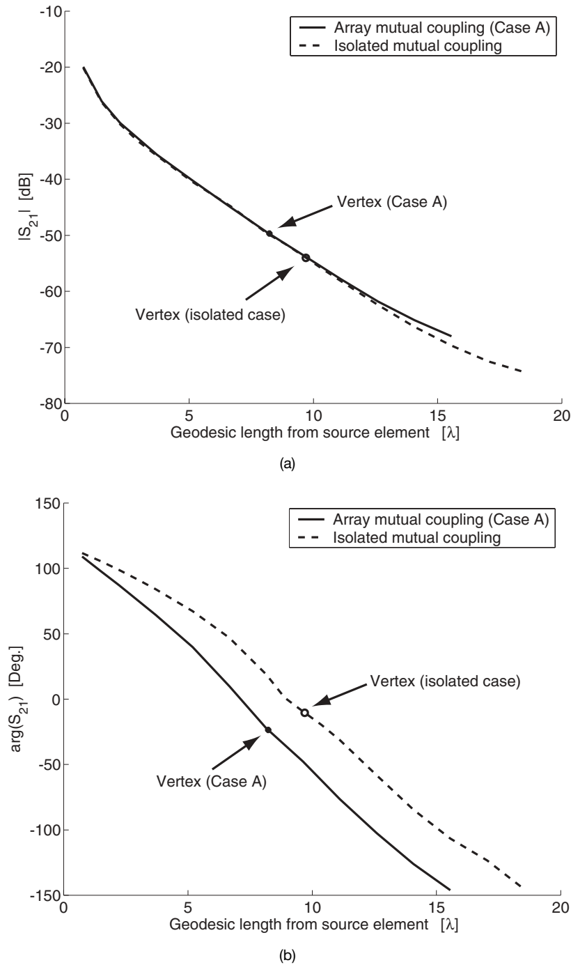
Figure 7.22. Comparison between the array and isolated E -plane mutual coupling along the y axis of the experimental antenna ( f = 8.975 GHz). Note that the array mutual coupling shown is measured from element -y_{11} , whereas the isolated coupling is measured from element -y_{13} [Lanne and Josefsson 2002]. (a) Amplitude. (b) Phase.
