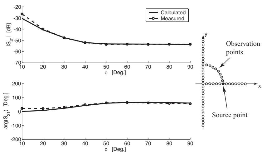
Figure 7.6. Isolated coupling along the circle arc, [R, R] polarization. The source point is element +x_6 . Solid line: calculated; dashed line: measured.
