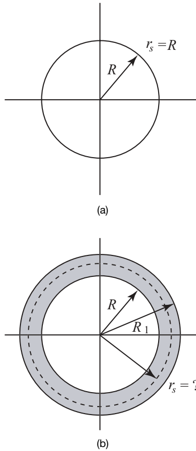
Figure 4A.1. The interpretation of r_s for (a) the noncoated PEC circular cylinder, (b) the coated PEC circular cylinder.
