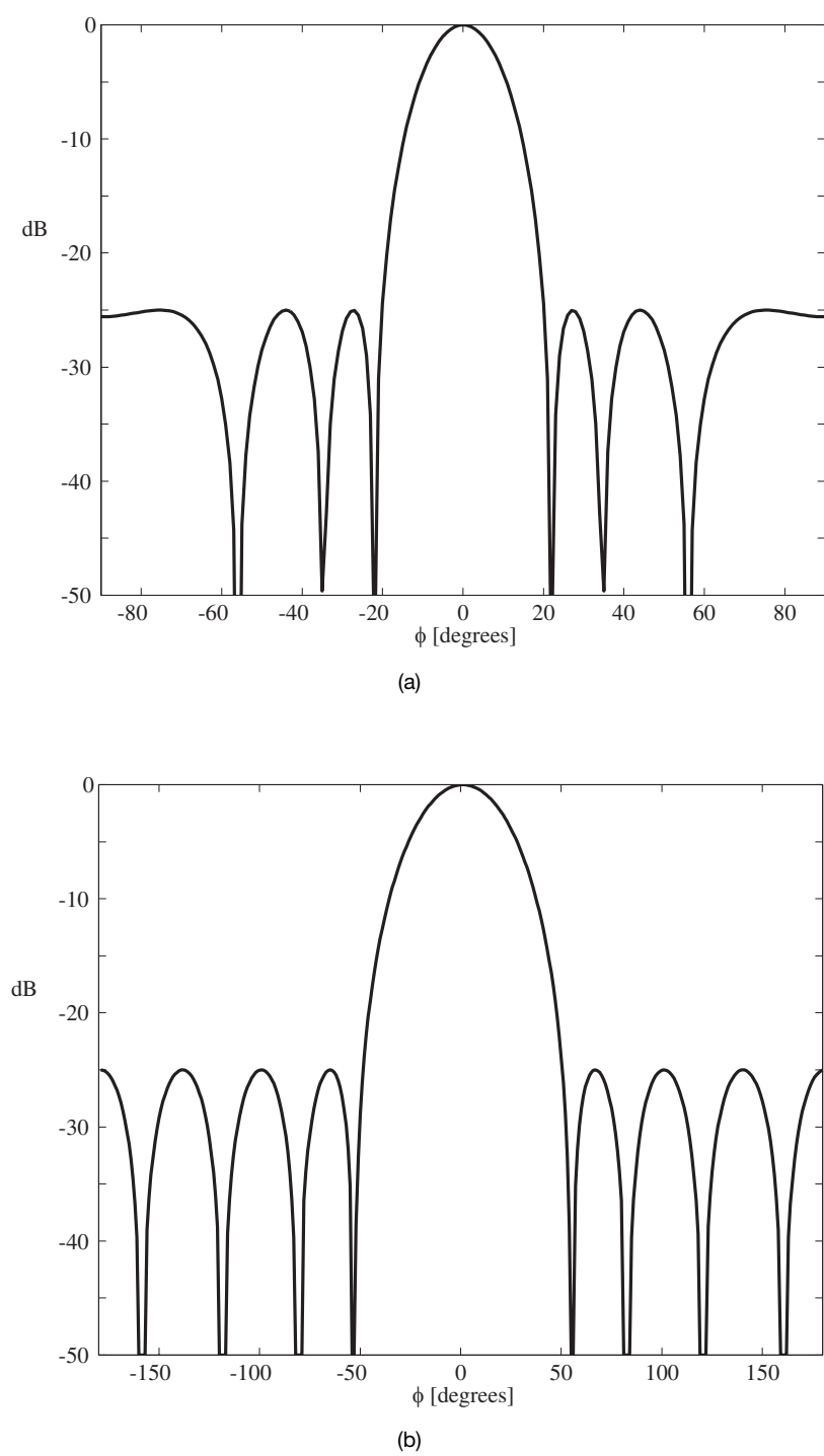
Figure 10.1. Chebyshev patterns: (a) Linear array with 9 elements, (b) Circular array with 9 phase modes (and 10 elements). Both cases have isotropic elements spaced 0.4 \lambda .
