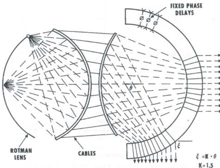
Figure 9.18. A broadband multiple array feed using a two-dimensional dome output lens [Thomas 1979].
