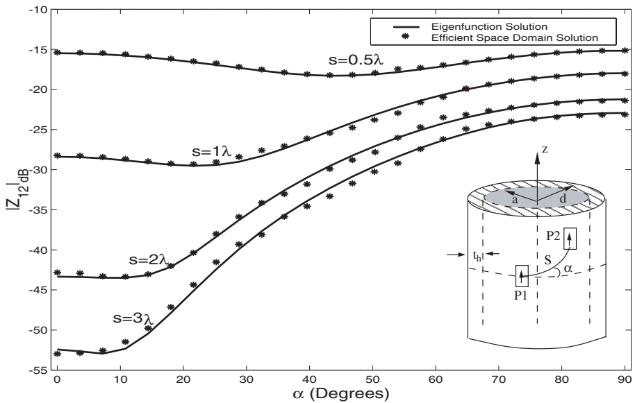
Figure 6.62. Mutual coupling, Z_{12} , between two identical z -directed current modes for a coated cylinder with R = 3\lambda_0 , t = 0.06\lambda_0 , and \epsilon_r = 3.25 [Ertürk 2000]. a = R and d = R + t .
