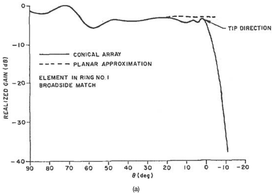
Figure 6.82. Embedded-element patterns (axial cut and E plane) for elements in different rings [Balzano and Dowling 1974]. (a) Element in ring No. 1. (continued)
