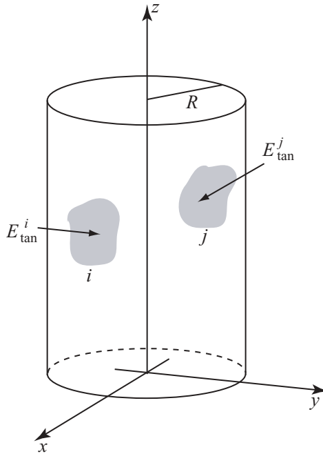
Figure 4.2. Two apertures ( i and j ) in a conducting circular cylinder.
