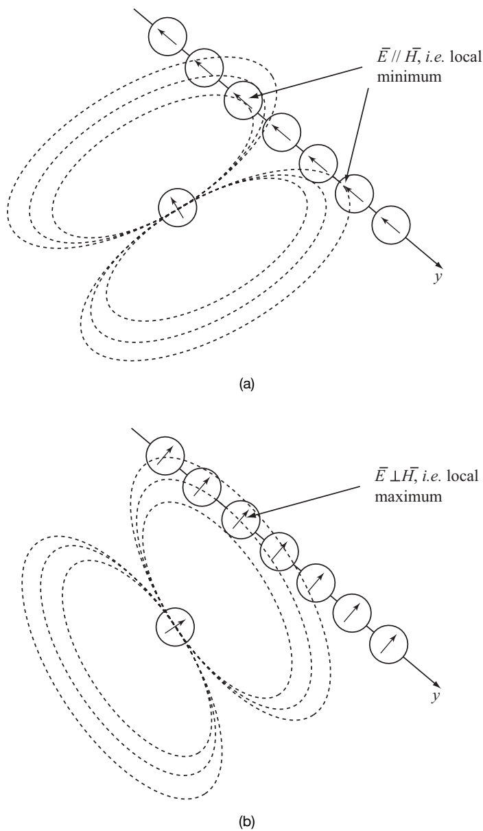
Figure 7.16. A sketch of the magnetic field for the planar case. (a) [R, R] polarization case; see also Figure 7.12. (b) [\varphi, \varphi] polarization case; see also Figure 7.13.
