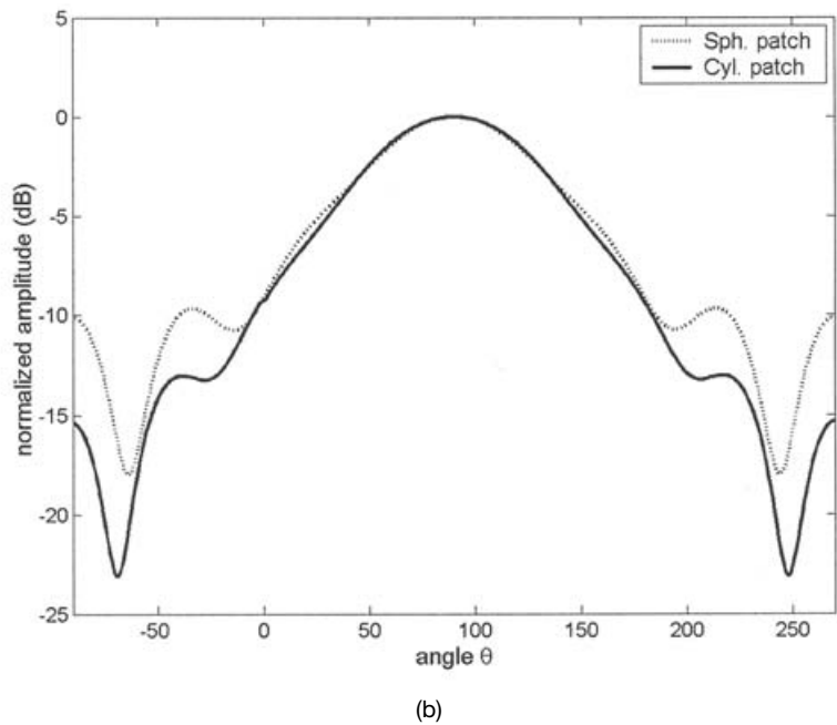
Figure 7.34. Comparison between radiation patterns of spherical patch antenna (dotted line) and \phi -polarized cylindrical patch antenna (solid line) [Burum and Sipus 2002b]. (a) H plane. (b) E plane.
