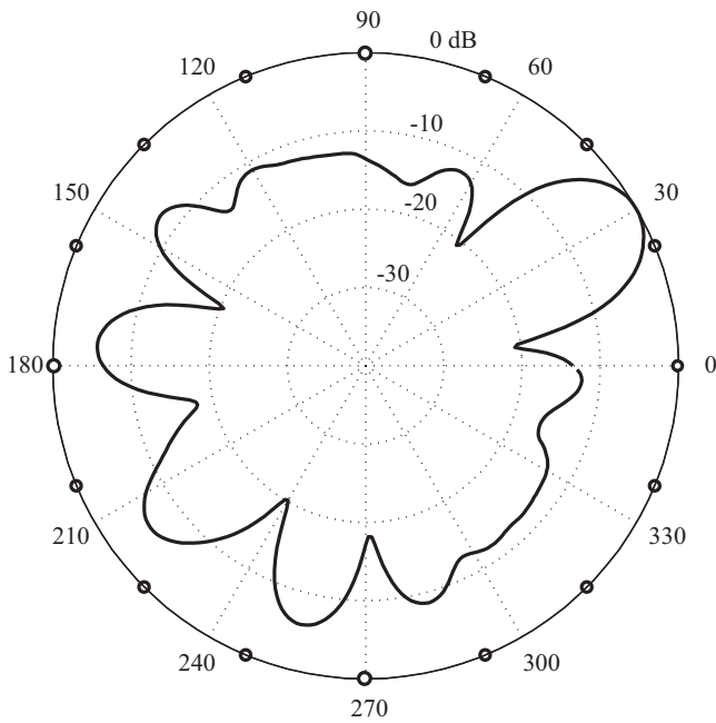
Figure 8.9. Computed pattern with 16 elements and 30° scan angle. All 16 elements are used; the element spacing is 0.5 \lambda (10 dB between circles).
