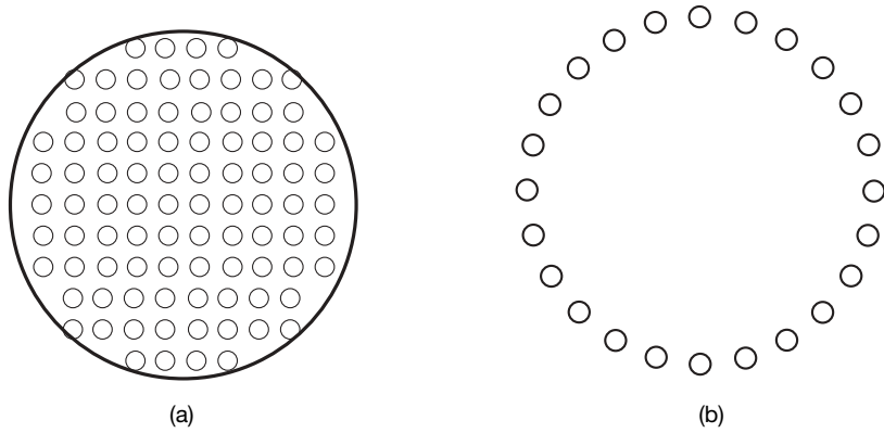
Figure 2.1. A circular planar array (a), and a circular (ring) array (b).
