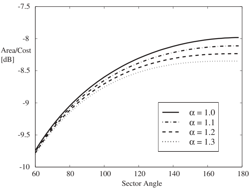
Figure 3.8. Normalized performance (effective area/cost) versus sector angle for omnidirectional coverage (360°).
