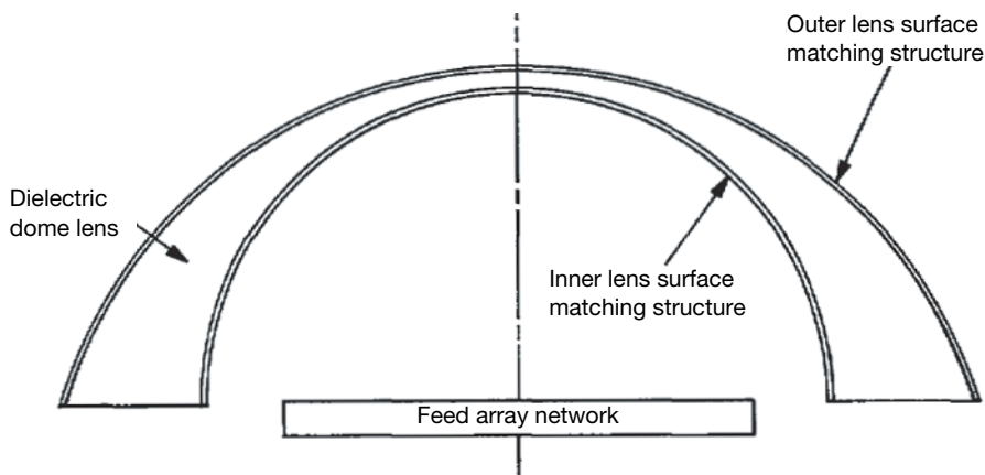
Figure 9.17. A dielectric dome lens antenna [Valentino et al. 1980].
