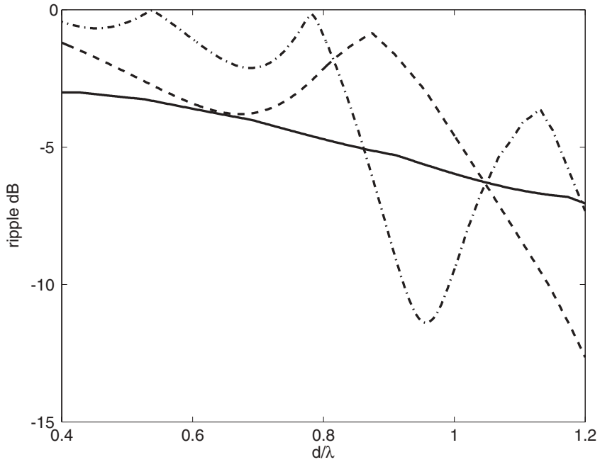
Figure 2.25. The ripple amplitude for circular arrays with \cos \phi element patterns. Compare Figure 2.17. Four elements = solid line, eight elements = dashed line, and 16 elements = dash-dotted line.
