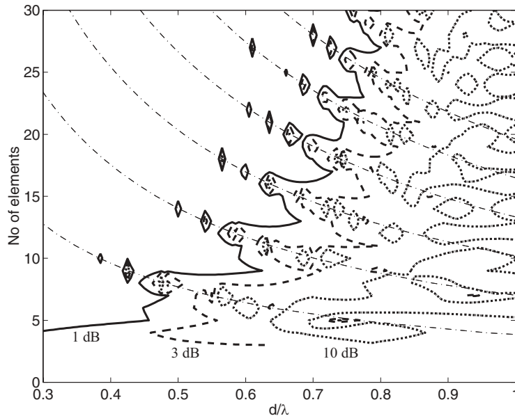
Figure 2.21. Ripple amplitude contour lines (1 dB solid, 3 dB dashed, and 10 dB dotted) for ring arrays with isotropic elements and m = 1 mode excitation. Along the dash-dotted lines, J_1(kR) = 0 .
