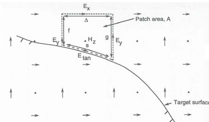
Figure 4.5. The CP FDTD methodology for a perfectly conducting surface [Jurgens et al. 1992].
