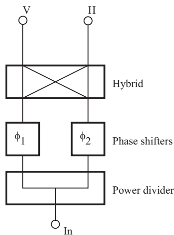
Figure 8.47. Variable power divider (VPD).
