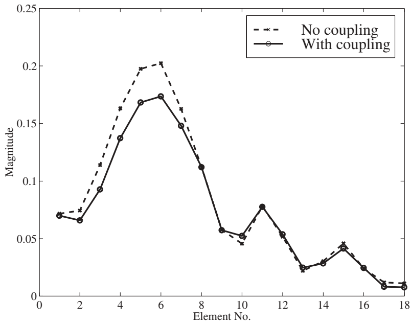
Figure 10.16. The mutual coupling effect on the synthesized excitation amplitude.
