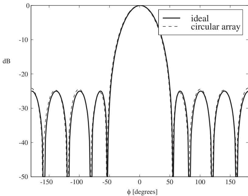
Figure 10.4. Pattern from an 11 element circular array, nine phase modes, and 0.4 \lambda element spacing (dashed line), compared with the desired Chebyshev pattern (solid line).
