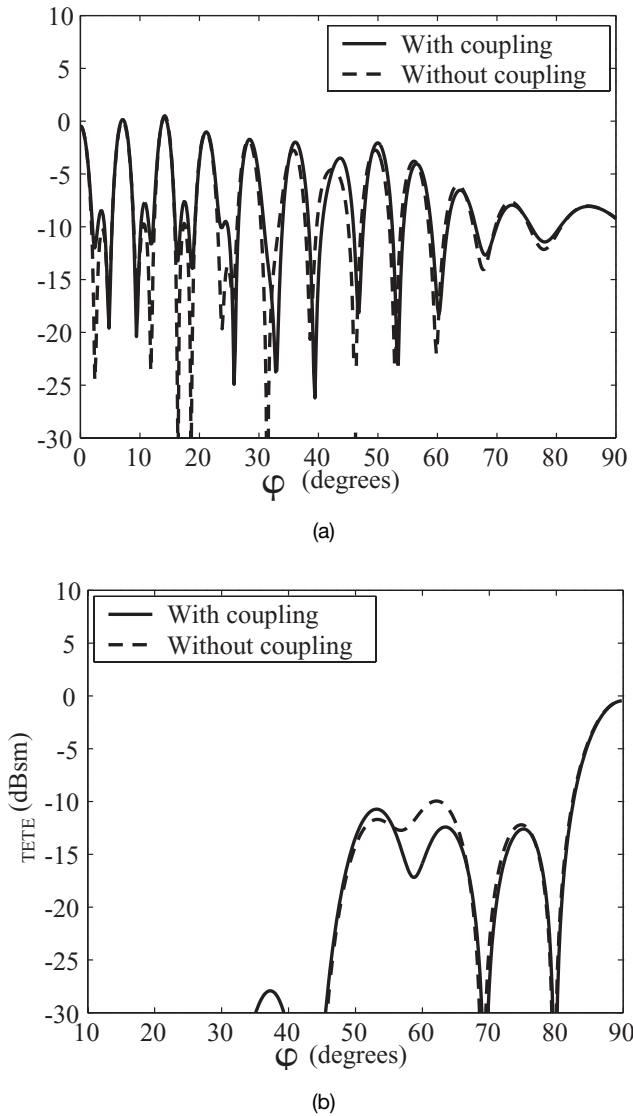
Figure 11.4. Calculated results for \sigma_{TETE} at 6.8 GHz with one waveguide mode, with mutual coupling (solid line) and without mutual coupling (dashed line). (a) E plane. (b) H plane.
