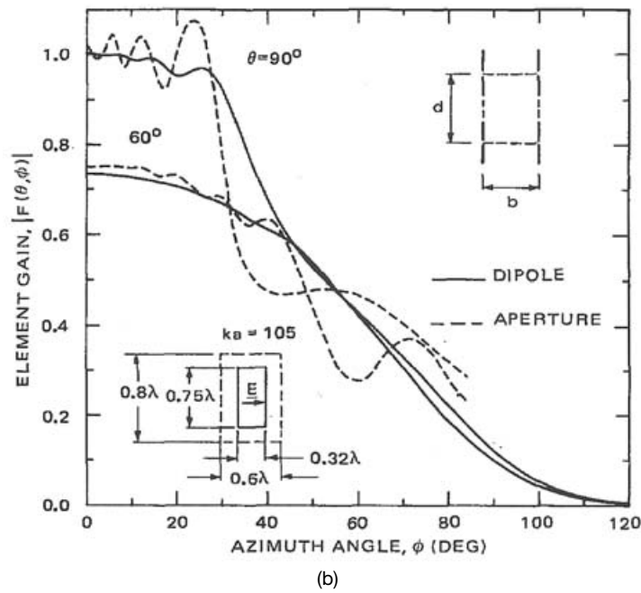
Figure 6.26. (a) Geometry of the circular cylindrical array of dipoles in a rectangular lattice. (b) Voltage element gain patterns between dipole and rectangular aperture radiators. ka = 105 , b = 0.6\lambda , and d = 0.8\lambda [Herper et al. 1985a].
