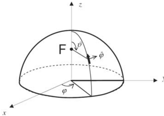
Figure 8.36. Dipole element at coordinates (\vartheta, \varphi) . F is the focal point of the parabolic surface.
