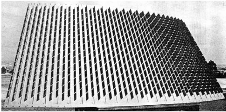
Figure 8.50. A sector of a conical array with 700 dipole elements [Munger et al. 1974].
