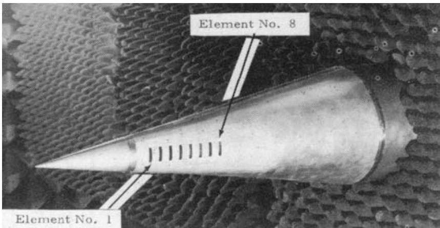
Figure 8.49. Linear slot array on a metallic cone [Villeneuve et al. 1974].
