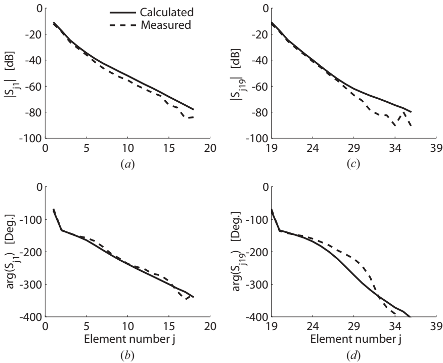
Figure 6.14. The array mutual coupling in the E plane for the first row (elements 1 \rightarrow 18) and the second row (elements 19 \rightarrow 36). Single-mode approximation, f = 5.65 GHz. Solid line: calculated, dashed line: measured. (a) Amplitude, first row. (b) Phase, first row. (c) Amplitude, second row. (d) Phase, second row [Persson and Josefsson 2001].
