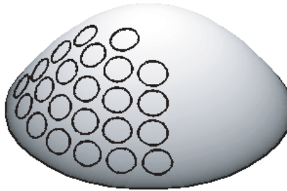
Figure 8.35. Active region for 60° scan angle (from zenith) and max 45° element scan angle.
