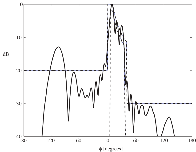
Figure 10.12. Result after three iterations.
