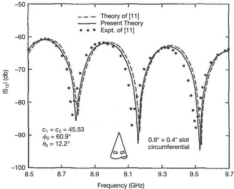
Figure 6.72. Coupling coefficient S_{12} between two circumferential slots on a cone as a function of frequency [Lee 1978]. Reference [11] is [Golden et al. 1974].
