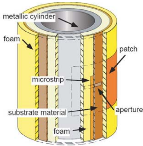
Figure 8.6. Aperture-coupled microstrip patch on a cylindrical structure [Löffler et al. 1999].
