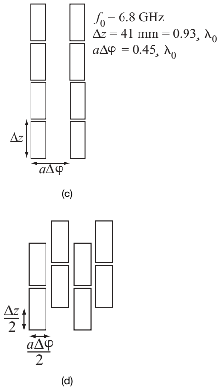
Figure 11.25. (cont.) (c) Rectangular grid array with 4 \times 2 elements. (d) Triangular grid array with 4 \times 2 elements.
