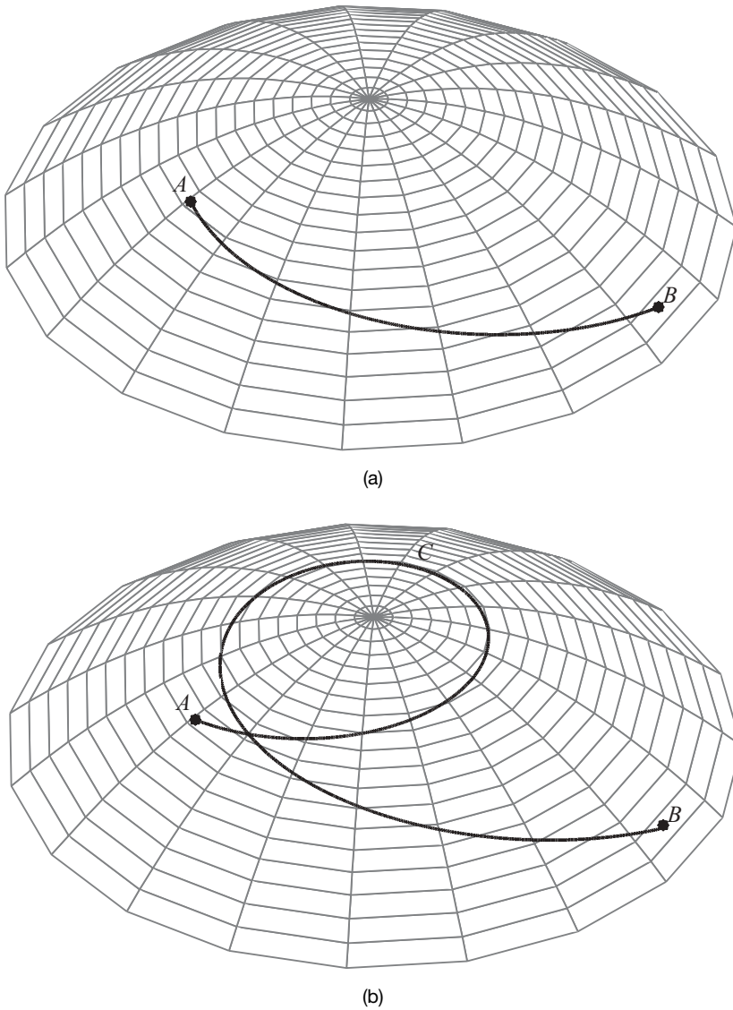
Figure 5.12. A GPOR in which a = 1.6 ( u_A = 4 , \varphi_A = 20^\circ ; u_B = 6.5 , \varphi_B = 140^\circ ). (a) The first-order geodesic in the positive \varphi direction; \alpha = 4.4851 and \beta = -165.218^\circ . (b) The nontrivial second-order geodesic in the positive \varphi direction; \alpha = 3.4 and \beta = -217.4338^\circ .
