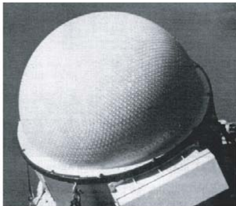
Figure 9.16. The dome array antenna with 3636 passive lens elements fed by a planar array with 805 elements and phase shifters [Fowler 1998].
