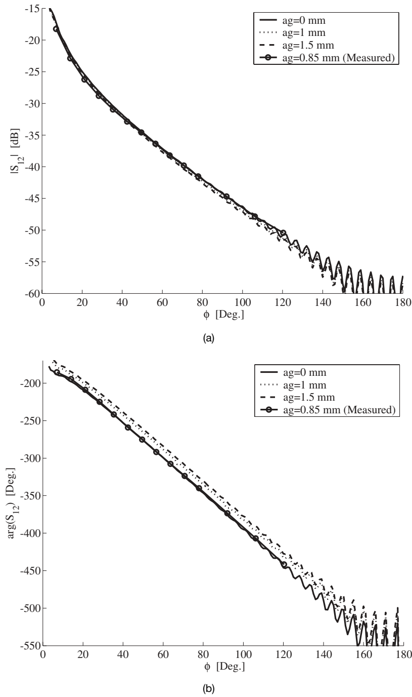
Figure 6.50. Isolated E -plane coupling along the cylindrical surface in the azimuth ( \alpha = 0^\circ ). Here, the coupling is studied with respect to the thickness of the air gap ( ag ) between the PEC surface and the coating. Measured data are also included (line with circles). (a) The amplitude. (b) The phase with the free-space contribution subtracted. (continued)
