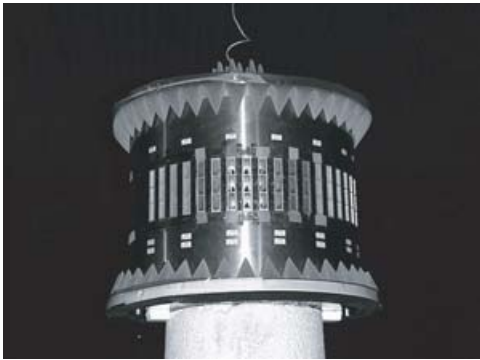
Figure 11.5. The experimental antenna prepared for RCS measurements. (Courtesy of Ericsson Microwave Systems AB, Göteborg, Sweden.)
