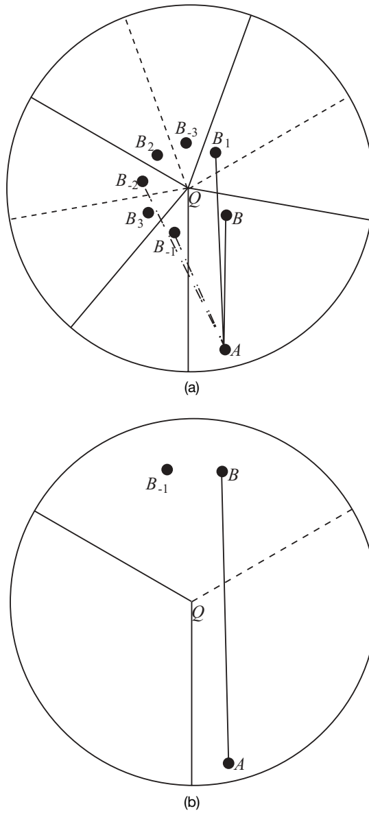
Figure 5.9. The unrolled cone for two different values of the half-cone angle \theta_0 . (a) \theta_0 < 45^\circ . (b) \theta_0 > 45^\circ .
