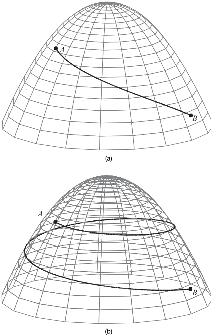
Figure 5.11. Geodesics in the positive \varphi direction of a GPOR with a = 0.4 . (a) The first-order geodesic; \alpha = 0.33981 and \beta = -529.5008^\circ . (b) The second-order geodesic; \alpha = 1.1303 and \beta = -696.0058^\circ . (continued)
