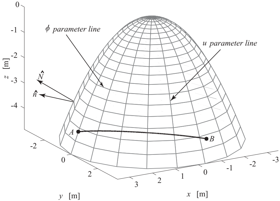
Figure 5.13. An example of a geodesic when u_A = u_B but no geodesic splitting occurs. Furthermore, for the \varphi parameter lines the normal direction and the surface normal direction are indicated. This shows that the \varphi parameter lines are not geodesics.
