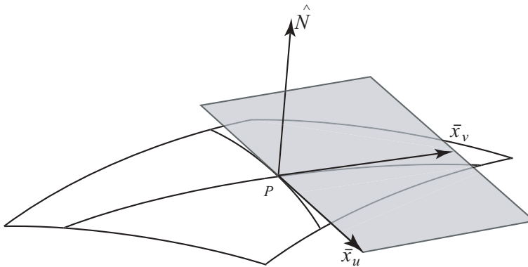
Figure 5.1. The u and v parameter lines with the tangent plane and the surface unit normal vector \hat{N} .
