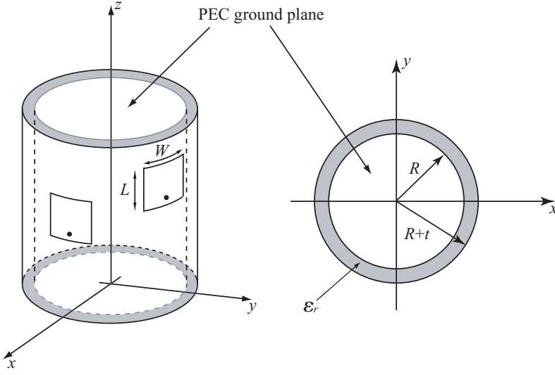
Figure 6.60. Geometry of two probe-fed rectangular microstrip antennas located on a circular cylinder.
