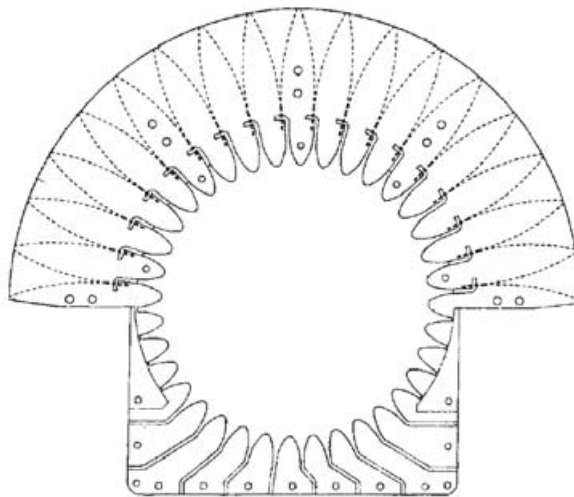
Figure 9.11. A broadband semicircular array with microstrip R-kR lens feed in printed circuit technology [Sierra and Bernal 1989].
