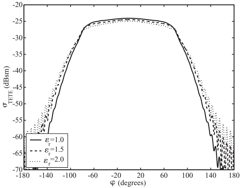
Figure 11.17. The E -plane RCS at 4.3 GHz for a single waveguide element on a cylinder with different dielectric coatings.
