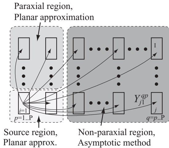
Figure 6.55. The admittance values are calculated with the source aperture in the lower-left corner of the array. For computational purposes, the rectangular grid array is divided into three regions: source region, paraxial region, and nonparaxial region [Thors et al. 2003].
