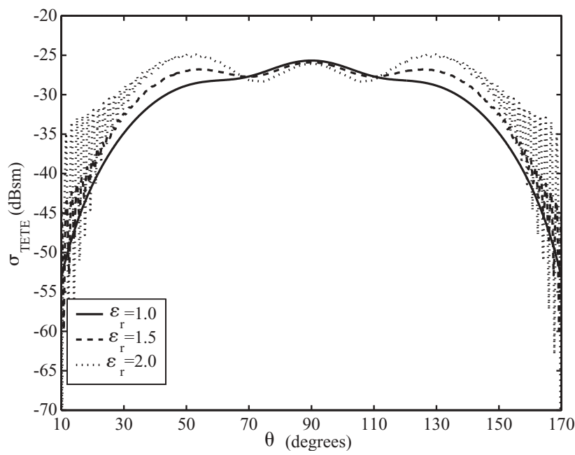
Figure 11.20. The H -plane RCS at 6.8 GHz for a single waveguide element on a cylinder with different dielectric coatings.
