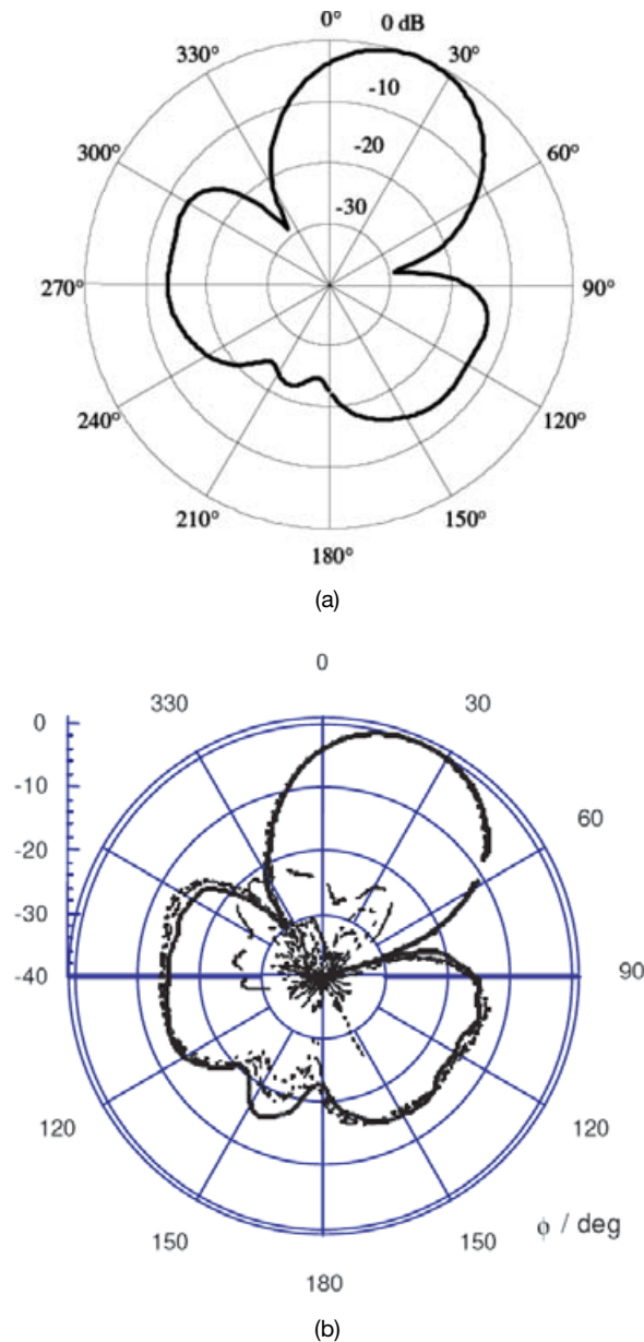
Figure 8.20. Computed pattern using the slot model (a). Measured (co- and cross polar) results at 5.0–5.4 GHz (b), and cylindrical array (c) [Löffler et al. 1999]. (continued)
