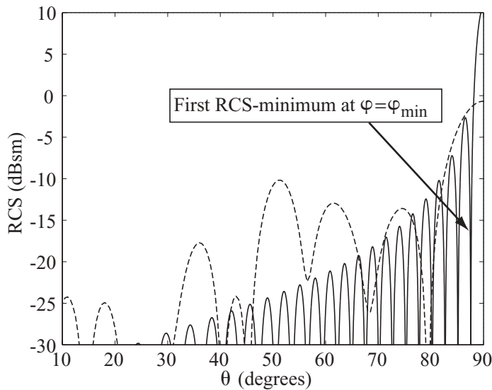
Figure 11.6. Comparison between the backscattered cross section from a finite cylinder without apertures (solid line) and the predicted array scattered cross section (dashed line) in the H plane.
