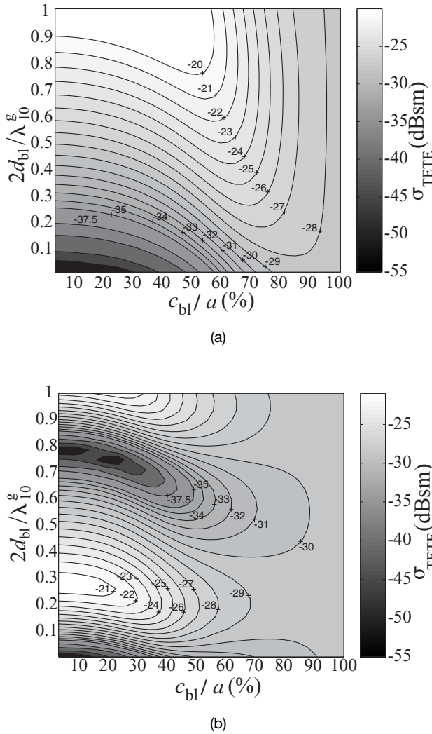
Figure 11.29. RCS as a function of iris gap and iris position ( \theta = 90^\circ , \varphi = 0^\circ ). (a) f = 4.3 GHz, (b) f = 8.0 GHz.
