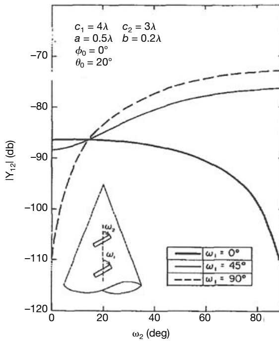
Figure 6.76. The mutual admittance between two arbitrarily oriented slots on a cone [Lee 1978].
