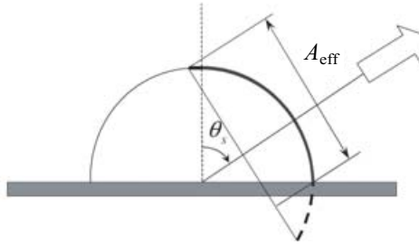
Figure 3.4. Effective (projected) area of a curved half-sphere or half-cylinder array antenna.
