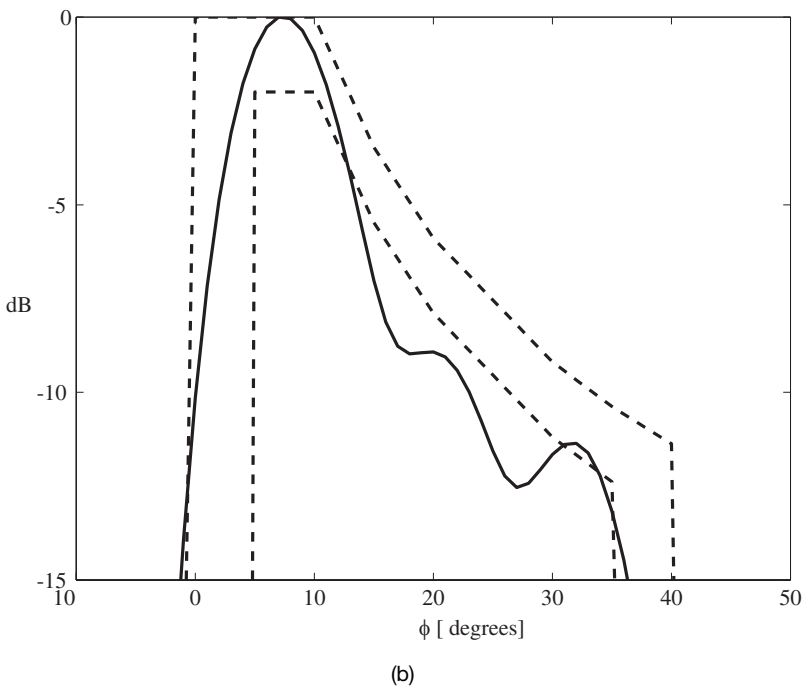
Figure 10.15. Pattern synthesis with coupling (a). The pattern in (b) demonstrates the effect of the mutual coupling if not included in the synthesis.
