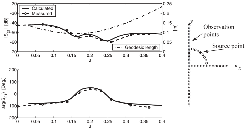
Figure 7.12. Isolated coupling, [R, R] polarization. The source point is element c_5 . Solid line: calculated; dashed line: measured, dashed-dotted line: geodesic length.
