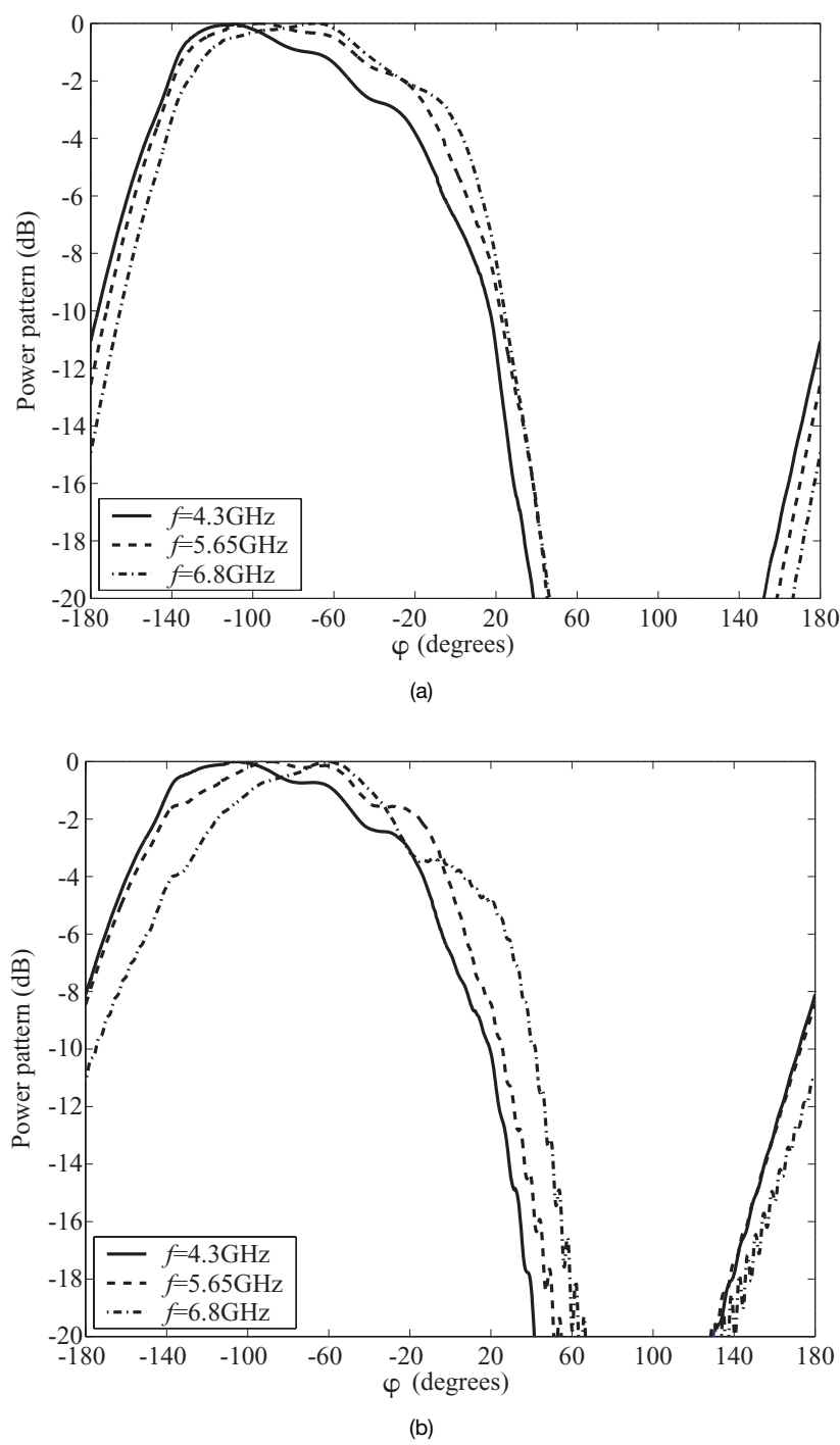
Figure 6.58. Normalized E -plane embedded-element patterns for the first element of the second row of the 4 \times 32 elements array. The results are shown versus the frequency. (a) Without dielectric coating. (b) With dielectric coating ( \epsilon_r = 2.0 , d = 2.4\text{ mm} ) [Thors et al. 2003].
