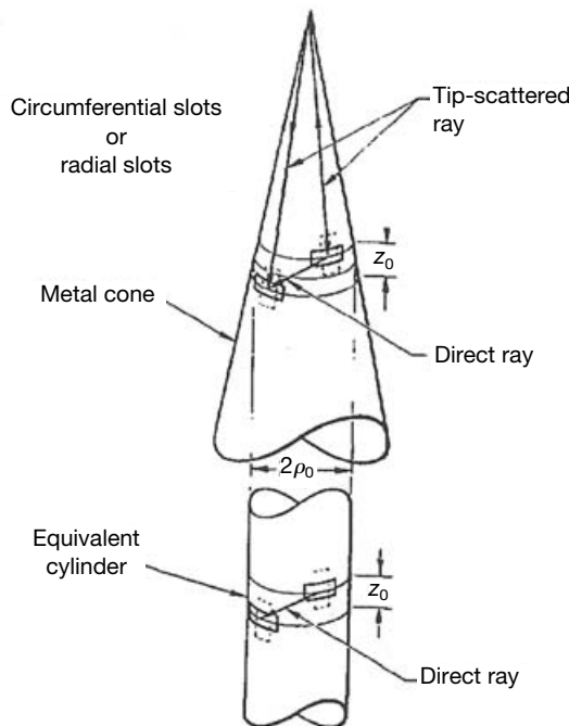
Figure 6.71. Slotted cone and equivalent cylinder [Golden et al. 1974].
