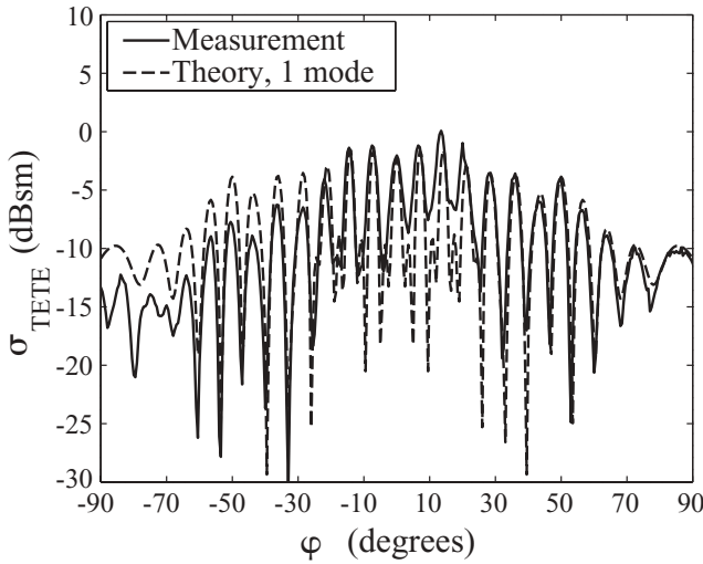
Figure 11.7. Comparison between the measured (solid line) and the calculated (dashed line) RCS at 6.8 GHz and \theta = 86.3^\circ . The calculations included one waveguide mode and mutual coupling.
