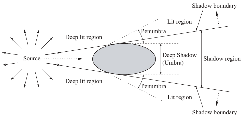
Figure 4.11. Definition of the different regions in space when a source is illuminating a smooth cylindrical surface. If the source is moving toward the surface (dotted arrow) the lit region will be concentrated to the “left” since the shadow boundary will move as well (dotted arrows). After [McNamara et al. 1990.]
