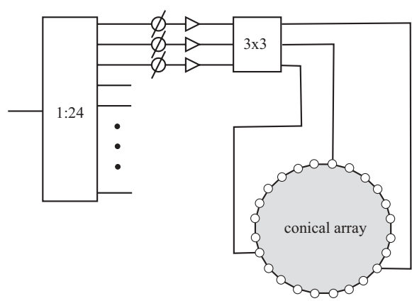
Figure 9.7. A “semiactive” phase-commutating feed system, after [Martín Polegre et al. 2001].
