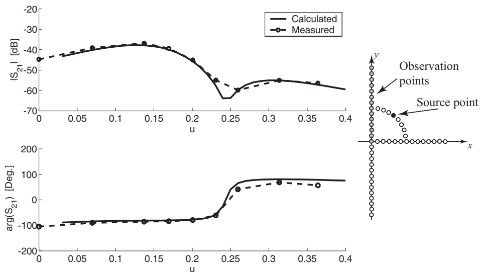
Figure 7.15. Isolated coupling, [\varphi, R] polarization. The source point is element c_5 . Solid line: calculated; dashed line: measured.
