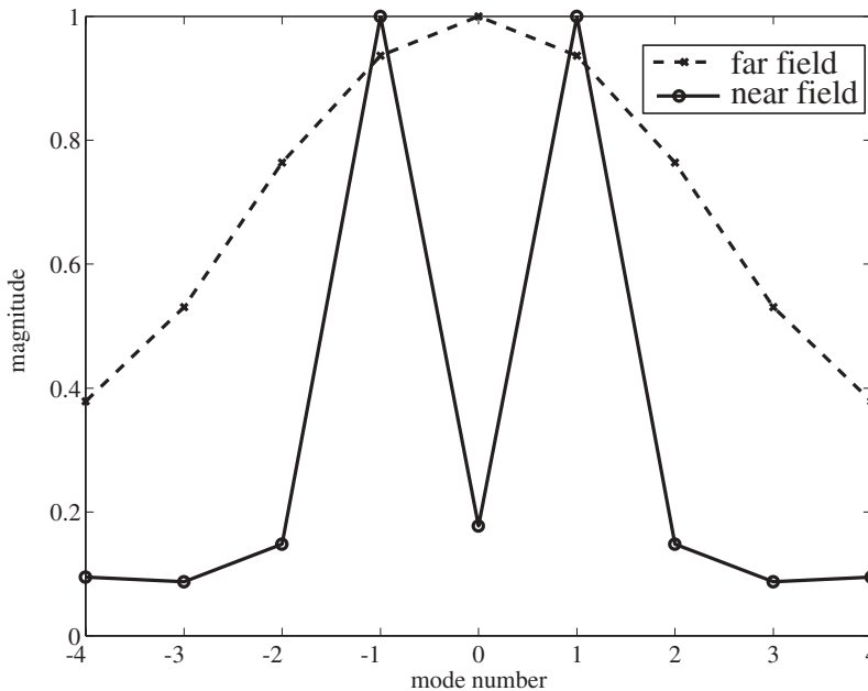
Figure 10.2. Far field mode (dashed line) and excitation mode (solid line) amplitudes for the circular array case in Figure 10.1 (b).
