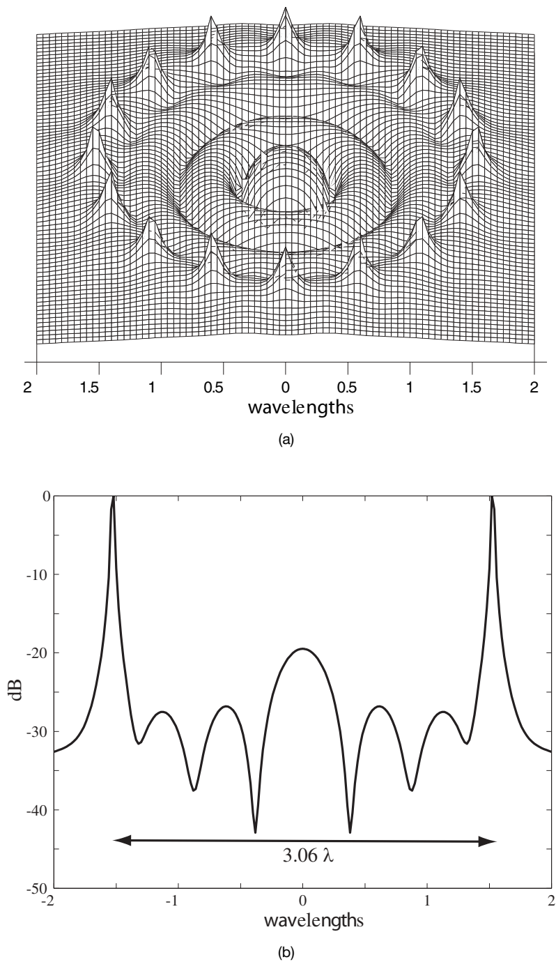
Figure 2.22. (a) The near field of a circular array. (b) Shows a cut through the array center. 16 isotropic elements spaced at 0.6 wavelengths. The array diameter 2R is 3.06 \lambda .
