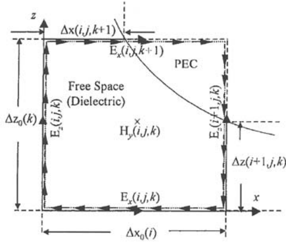
Figure 4.6. The contour path of the conformal FDTD in a deformed cell [Yu and Mittra 2000].
