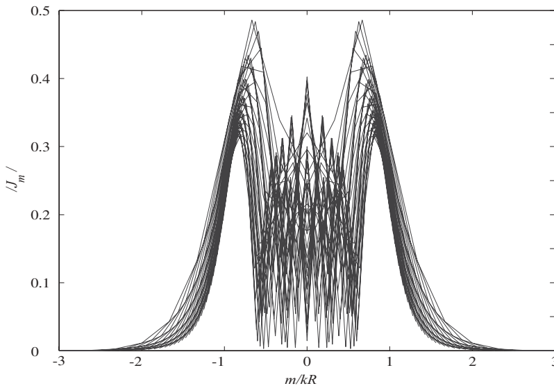
Figure 2.12. Bessel windowing function versus normalized order m/kR .
