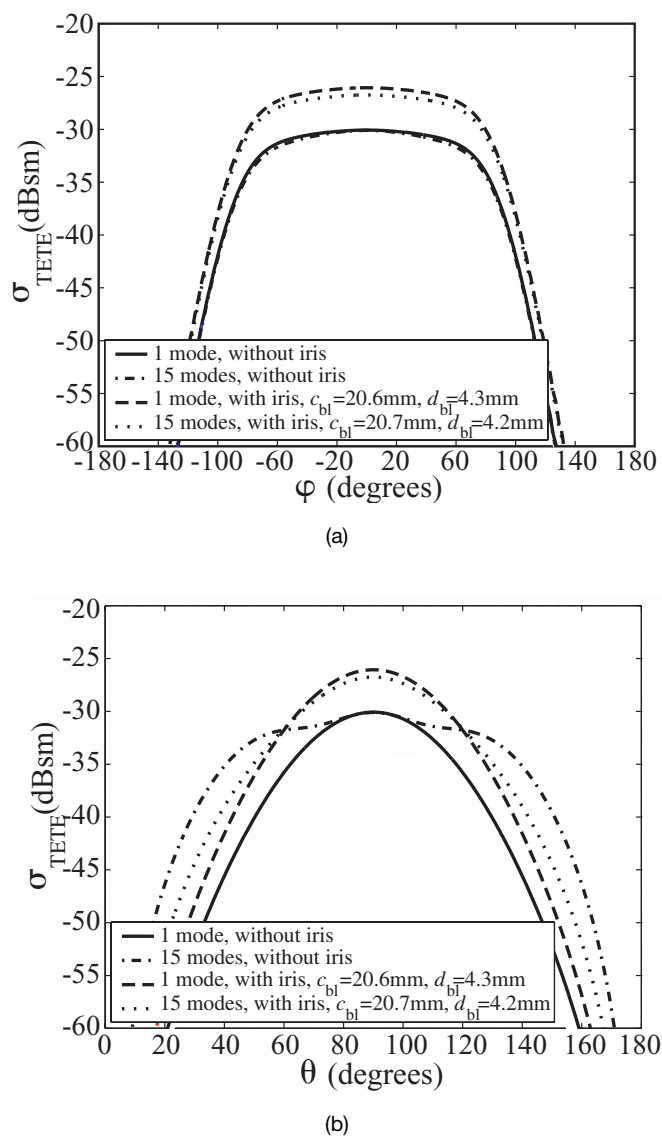
Figure 11.26. RCS at 6.8 GHz with and without iris (effect of higher-order modes). Solid line: one mode, no iris. Dash-dotted line: 15 modes, no iris. Dashed line: One mode, iris matched. Dotted line: 15 modes, iris matched. (a) E plane. (b) H plane.
