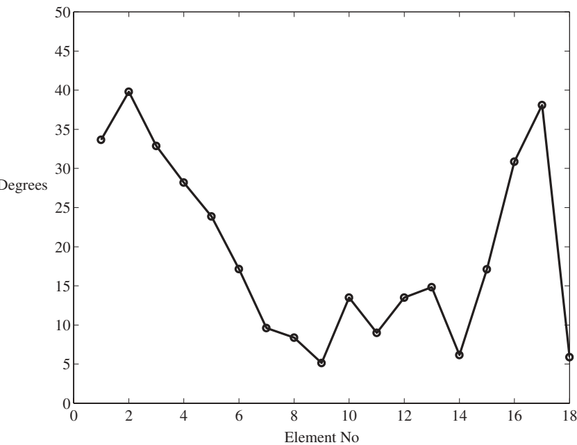
Figure 10.17. The change in the phase excitation due to the mutual coupling.
