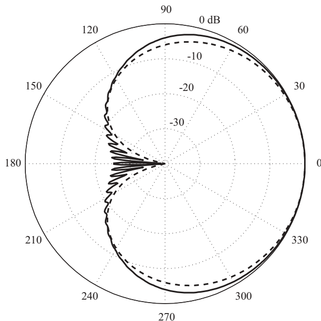
Figure 2.15. Slot pattern (solid line) and 1 + \cos \phi pattern (dashed) compared in the angular domain.
