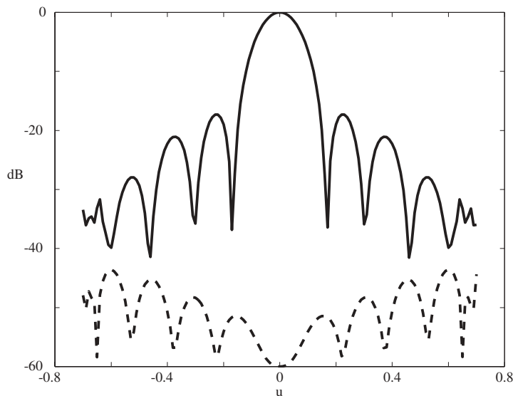
Figure 8.38. Radiation patterns (decibels vs. sine space) for a six ring paraboloidal array, h/D = 0.1 . The solid line is the co-polar pattern and the dashed line the cross-polar pattern.
