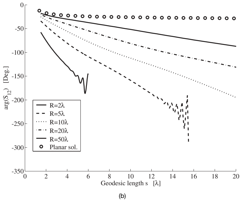
Figure 6.5. The isolated H -plane mutual coupling along the circumferential direction of cylinders with different radii. (a) The amplitude. (b) The phase, with the free space wave contribution subtracted.
