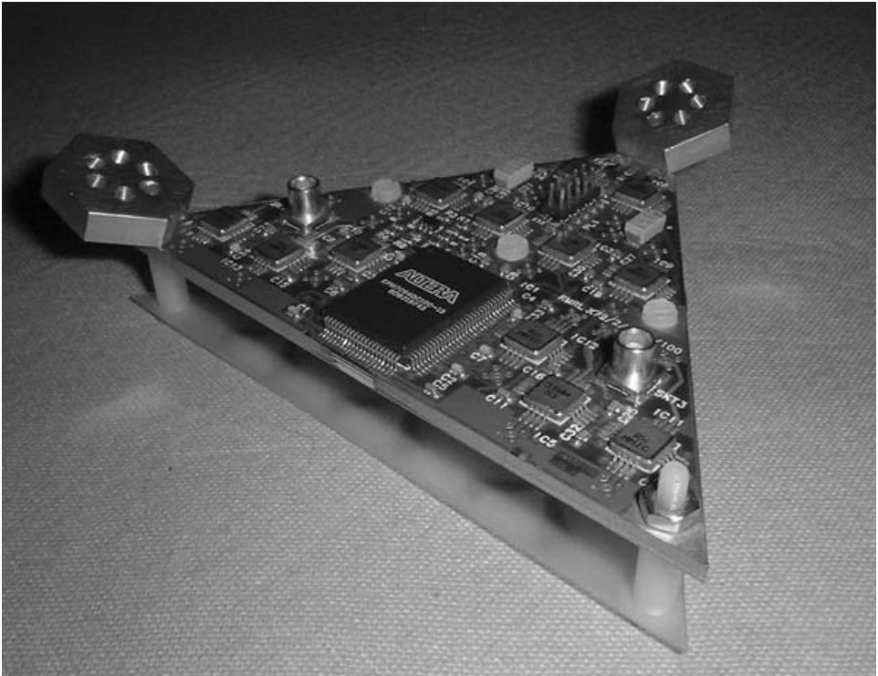
Figure 8.4. One of the triangular facets of the array in Figure 1.8 (rear side shown). Each facet has GaAs MMIC circuits for transmission and receiving functions. (Courtesy of Roke Manor Research Ltd., Roke Manor, Romsey, Hampshire, UK.)
