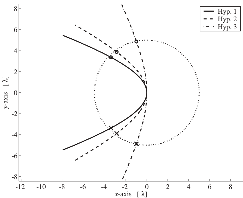
Figure 6.32. The hyperbolic geometry and the position of the first aperture (cross) and the final position of the second aperture (circle). The circular cylinder ( R = 5\lambda ) is also shown for geometrical reference.
