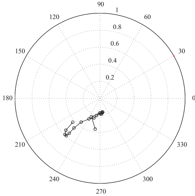
Figure 8.21. Reflection coefficient plot for the array with the beam steered 30° in Figure 8.15.
