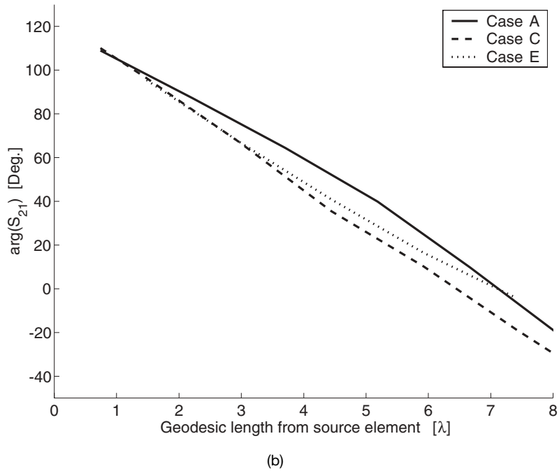
Figure 7.20. The array mutual coupling ( E plane) along the y axis of the experimental antenna ( f = 8.975 GHz). Three sets of data are shown. “Case A” shows the case when element -y_{11} is fed, “Case C” shows the case when element -y_6 is fed, and “Case E” shows the case when the element at vertex is fed [Lanne and Josefsson 2002]. (a) Amplitude. (b) Phase.
