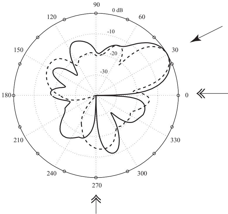
Figure 9.23. Cylindrical array pattern with (solid line) and without interference suppression (dashed line). Signal direction 30°, interfering signals at 0° and 270°.
