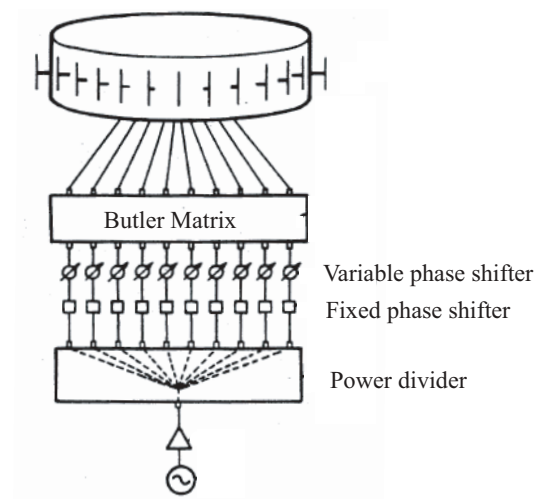
Figure 9.8. A Butler-matrix-fed array with variable phase shifters for scanning the beam [Sheleg 1968].
