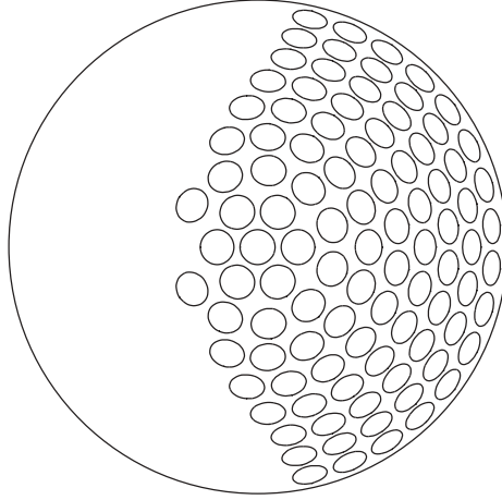
Figure 3.11. Active elements for 30° scan direction.
