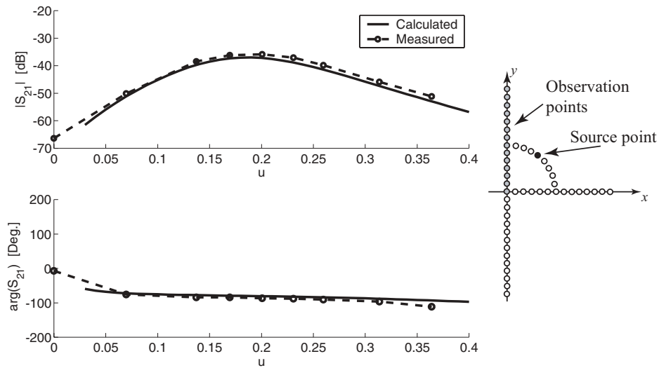
Figure 7.13. Isolated coupling, [\phi, \phi] polarization. The source point is element c_5 . Solid line: calculated; dashed line: measured.
