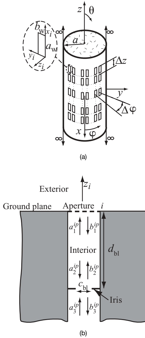
Figure 11.25. (a) The conformal array antenna. (b) The interior and exterior domains at aperture i . ( continued )
