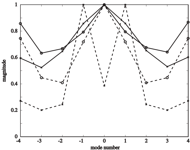
Figure 10.5. Circular array phase mode excitations for array with 10 elements and 9 phase modes. Legend: element spacings 0.3 \lambda (rings) and 0.35 \lambda (crosses). Dashed line: isotropic elements, solid line: directive (1 + \cos \phi) elements.
