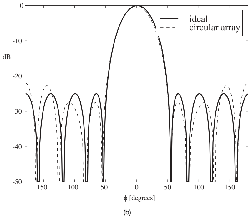
Figure 10.3. (a) Excitation function with samples at the element positions, (b) Radiation pattern (dashed line) compared to the ideal case (solid line) from Figure 10.1 (b). Ten radiating elements spaced 0.4 \lambda .
