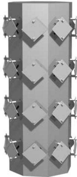
Figure 3.25. Faceted cylindrical microstrip patch array (CAD model). [Raffaelli and Johansson 2003]. See also color plate 11. (Courtesy of Ericsson AB, Göteborg, Sweden.)
