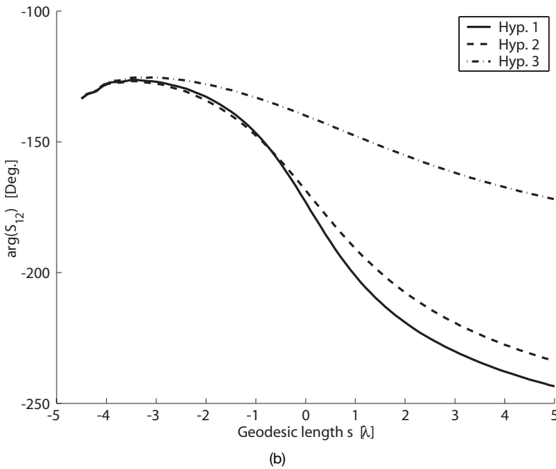
Figure 6.33. The isolated mutual coupling in the circumferential direction ( E plane) for apertures at hyperbolic cylinders. (a) The amplitude. (b) The phase.
