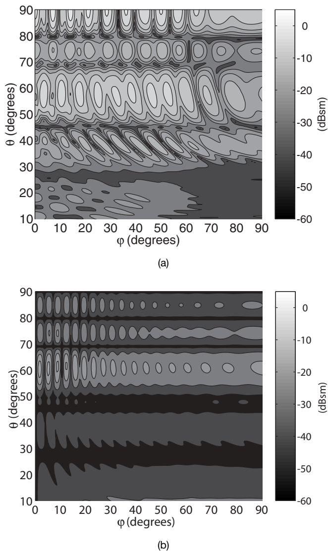
Figure 11.11. RCS at 6.8 GHz with mutual coupling and 15 modes. (a) \sigma_{TETE} , (b) \sigma_{TETM} .
