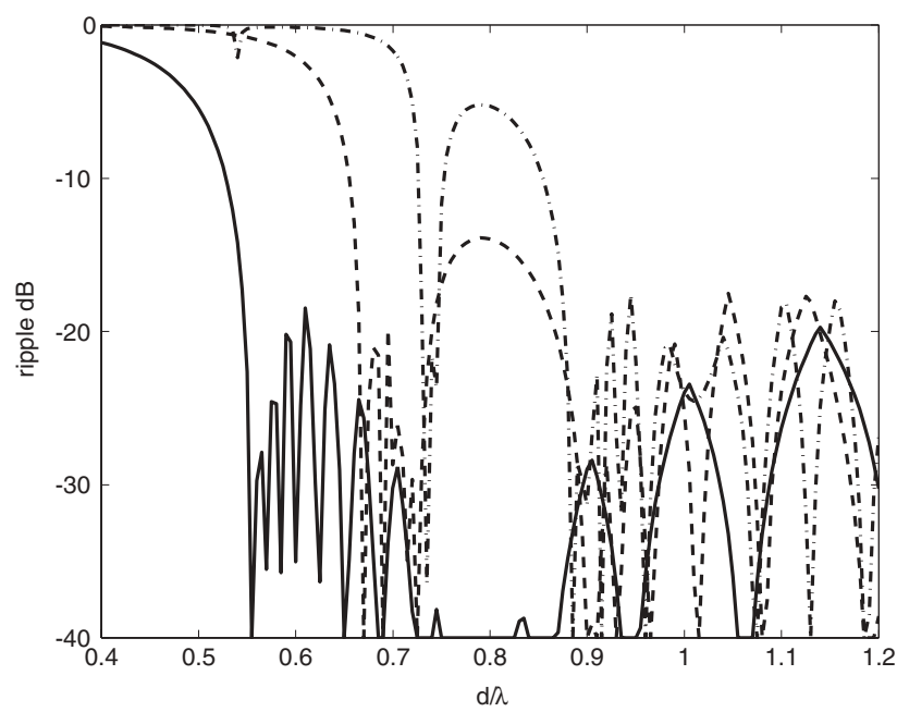
Figure 2.17. The ripple amplitude for circular arrays with isotropic elements; four elements (solid line), eight elements (dashed line), and 16 elements (dash-dotted line).
