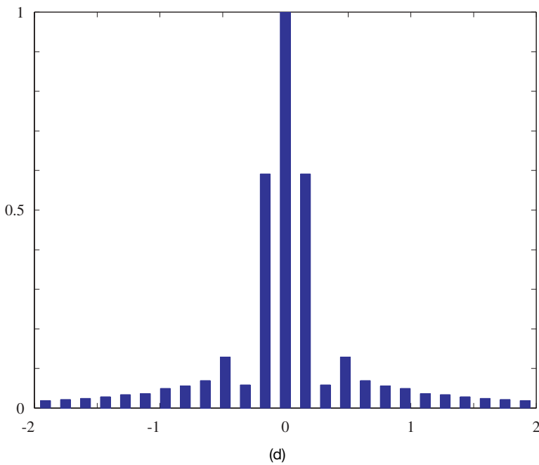
Figure 2.14 ( continued ). Typical element patterns in the Fourier domain: (c) (\cos \phi) , and (d) slot element in cylinder.
