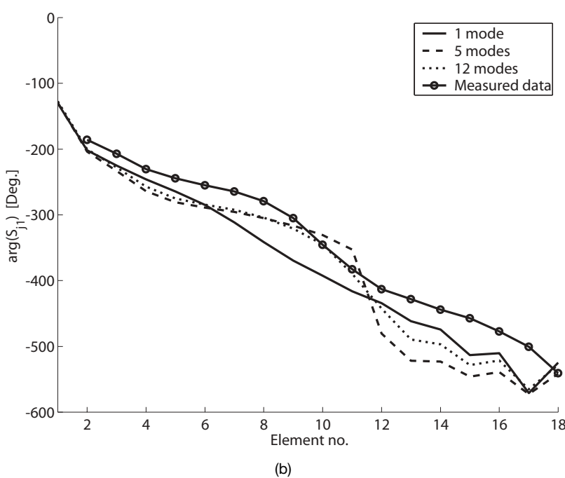
Figure 6.51. The mutual coupling ( E plane) for an array of apertures with a lossy dielectric coating. The calculated results are obtained using 1, 5, and 12 modes; the air gap between the PEC cylinder and the coating is not included. The results are compared with measured results (line with circles). (a) Amplitude. (b) Phase.
