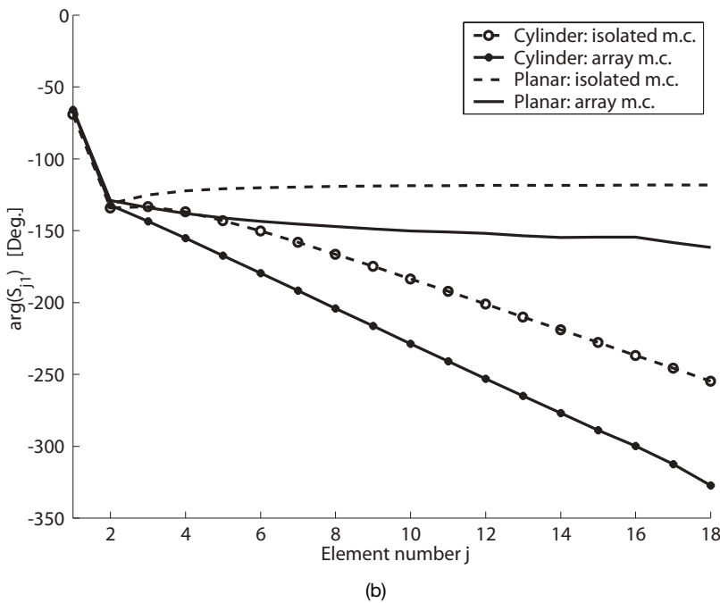
Figure 6.11. A comparison between the array and isolated mutual coupling for a single-row array on a cylinder for the E plane (lines with circles). The corresponding planar case is also shown for a single row of 18 elements. Single-mode results.
