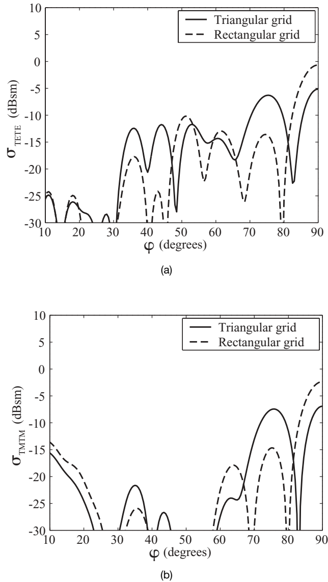
Figure 11.14. H -plane results for triangular grid (solid line) and rectangular grid (dashed line). (a) \sigma_{TETE} . (b) \sigma_{TMTM} . 6.8 GHz and 15 modes.
