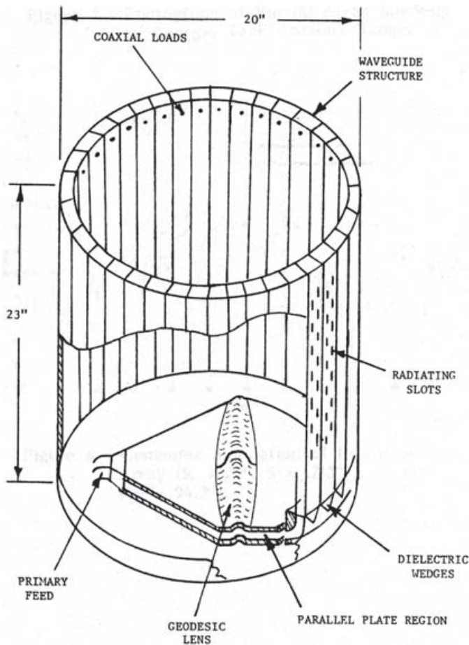
Figure 9.14. A Ku band mechanically commutating cylindrical array with a rotating geodesic lens feed [Bodnar et al. 1980].
