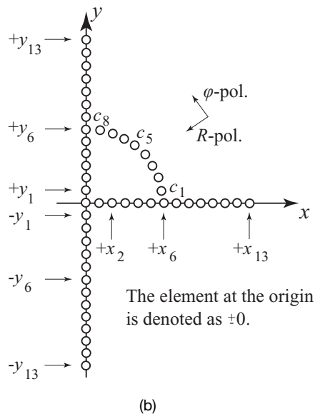
Figure 7.1. (a) The geometry of the experimental doubly curved antenna with the coordinate system used in the analysis. (b) The antenna from (a), together with the numbering of the elements. (continued)
