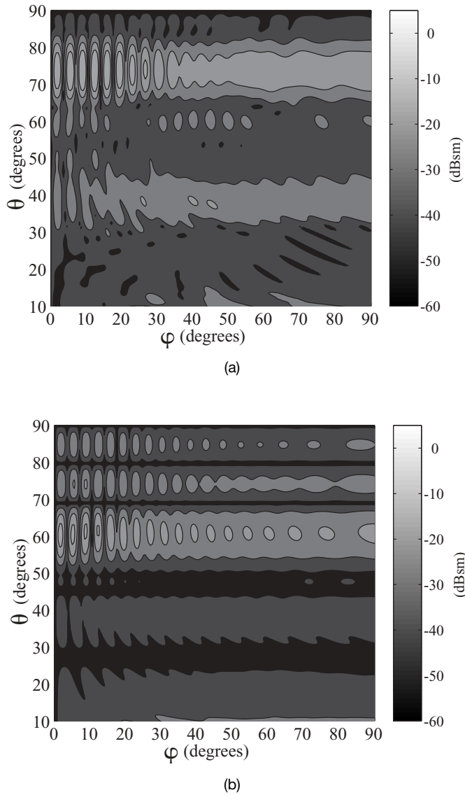
Figure 11.16. \sigma_{\text{TETM}} at 6.8 GHz with 15 modes. (a) Triangular grid, (b) rectangular grid.
