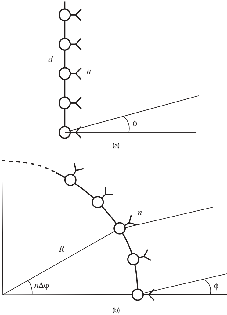
Figure 2.6. Linear array (a); part of a circular array (b).
