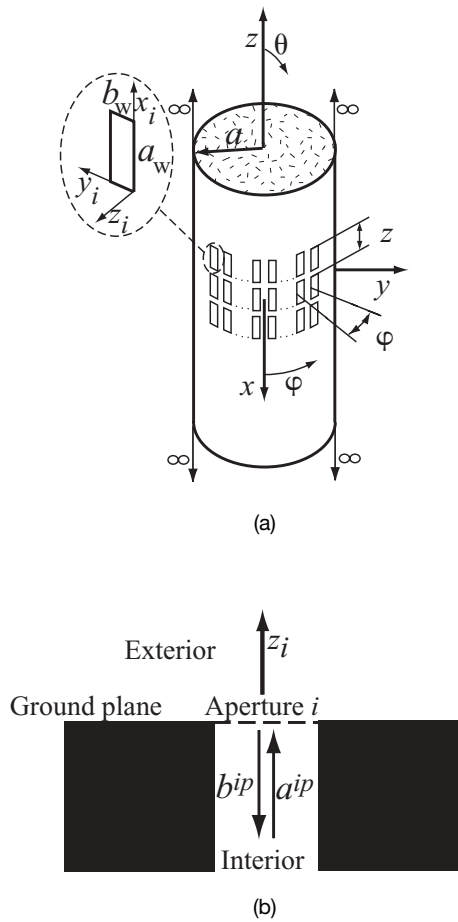
Figure 11.1. (a) The conformal array antenna. (b) The interior and exterior regions near an aperture.
