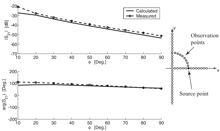
Figure 7.7. Isolated coupling along the circle arc, [\varphi, \varphi] polarization. The source point is element +x_6 . Solid line: calculated; dashed line: measured.
