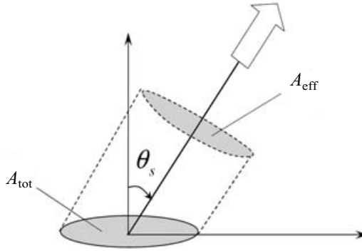
Figure 3.2. Effective (projected) area of a planar array antenna.
