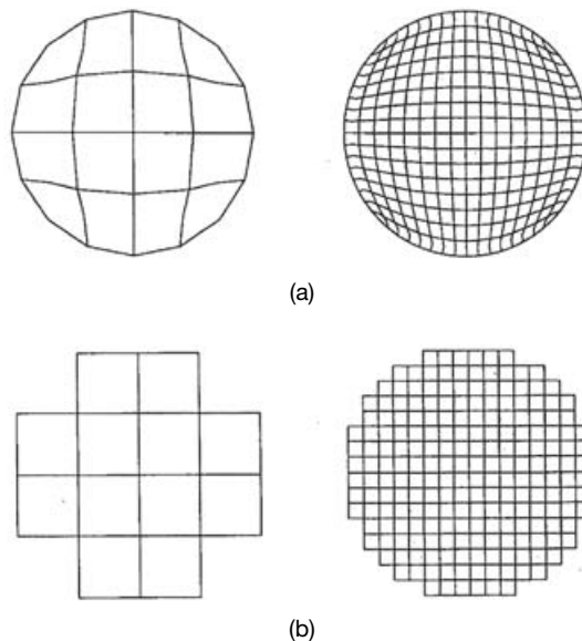
Figure 4.4. (a) Sparse and dense nonorthogonal grids for a cylindrical cavity. (b) Sparse and dense staircase grids for a cylindrical cavity. [Harms et al. 1992.]
