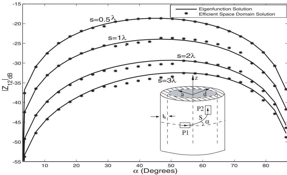
Figure 6.64. Mutual impedance Z_{12} between \varphi - and z -directed current modes (cross-polarization) for a coated cylinder with R = 3\lambda_0 , t = 0.06\lambda_0 , and \epsilon_r = 3.25 [Ertürk 2000]. a = R and d = R + t .
