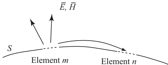
Figure 4.1. The problem: find the field outside the curved surface S due to one or more radiating elements on the surface S .
