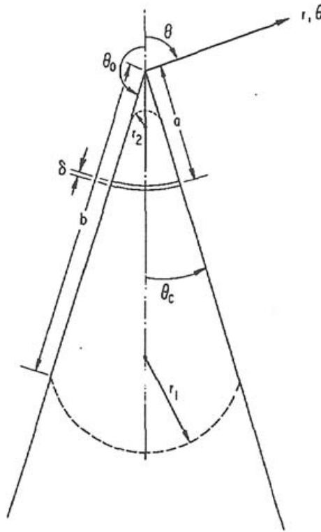
Figure 6.78. The cone geometry [Pridemore-Brown and Stewart 1972].
