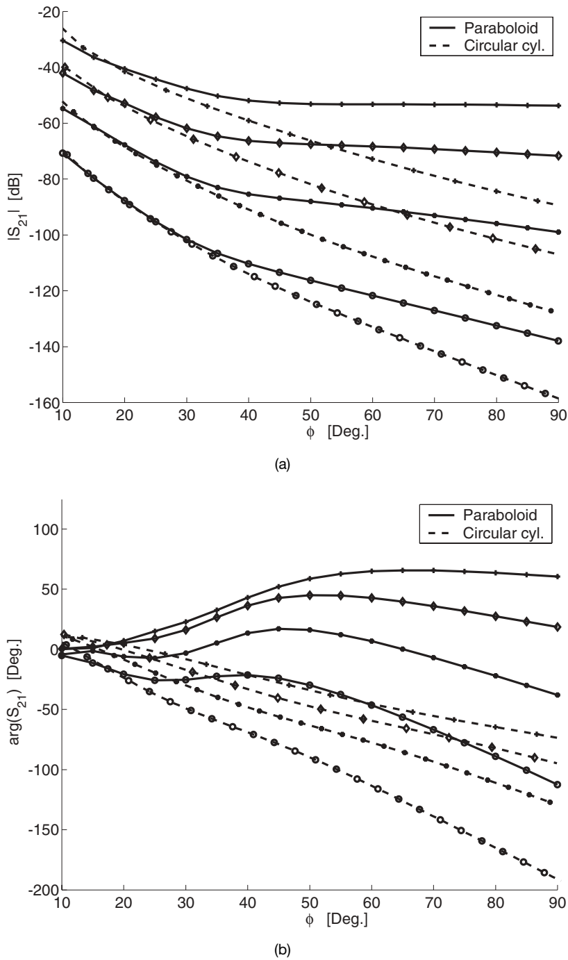
Figure 7.10. The circular cylinder (dashed lines) is used as an approximation for the isolated coupling along circle arcs located at different positions at the paraboloid (solid lines). The polarization is [R, R] and the different rows are starting with elements +x_6 (+), +x_{13} (diamonds), and two fictitious rows located further away from the vertex (stars and circles), respectively. (a) Amplitude. (b) Phase.
