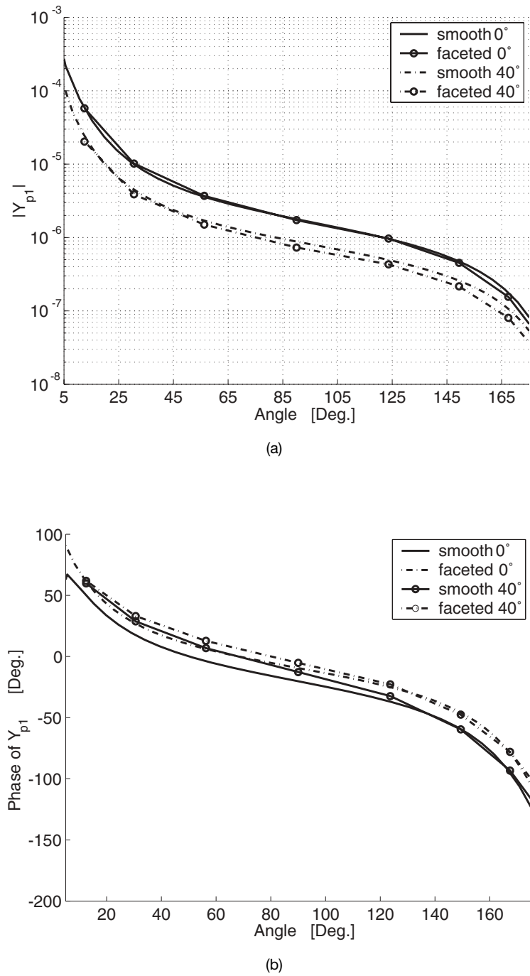
Figure 6.43. The isolated mutual coupling (admittance) ( \Omega^{-1} ) for a faceted elliptic cylinder (lines with circles), \alpha = 0^\circ and 40^\circ . Results for a smooth elliptic surface is also included for comparison. The transmitting aperture is located at the most strongly curved part of the surface [Marcus et al. 2003]. (a) Amplitude. (b) Phase.
