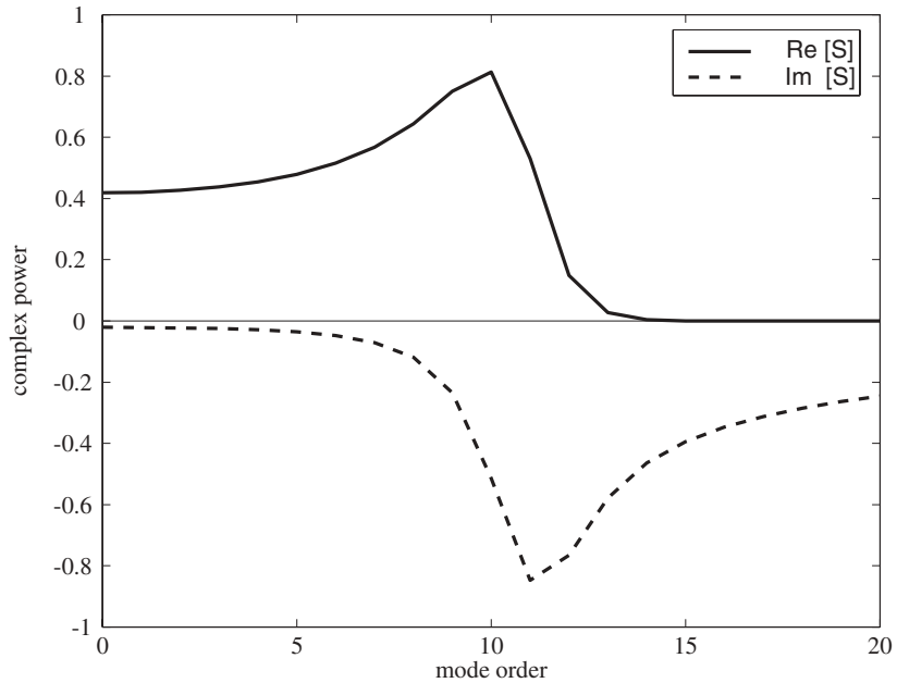
Figure 8.24. Real (solid line) and imaginary (dashed line) parts of the complex power (normalized); also representing the modal conductance and susceptance. Cylinder size kR = 10 .
