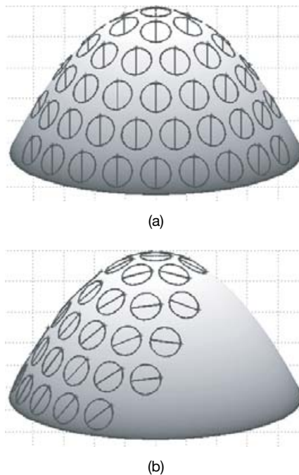
Figure 8.37. Radiation elements are rotated for polarization alignment in the main beam. The array is shown at 0^\circ and 90^\circ azimuth angles.
