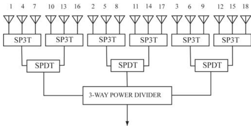
Figure 9.2. A switch matrix feed for activating 3 elements out of 18, after [Gregor-wich 1974].
