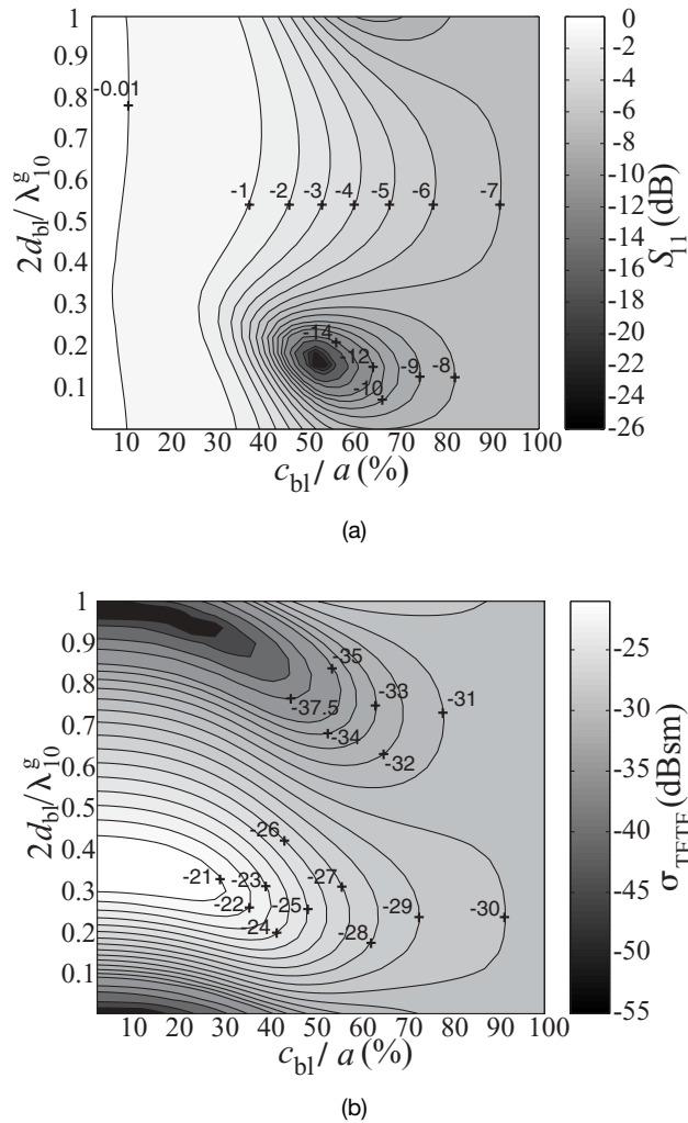
Figure 11.28. Reflection coefficient and RCS as a function of iris gap and iris position ( f = 6.8 GHz). (a) S_{11} , (b) \sigma_{TETE} ( \theta = 90^\circ , \varphi = 0^\circ ).
