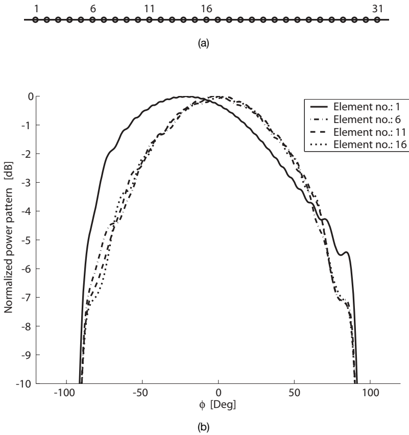
Figure 6.37. Embedded-element patterns in the E plane due to apertures in a sector array containing 31 elements, infinite ground-plane. The element-to-element distance equals 0.5\lambda . (a) The geometry. (b) The results.
