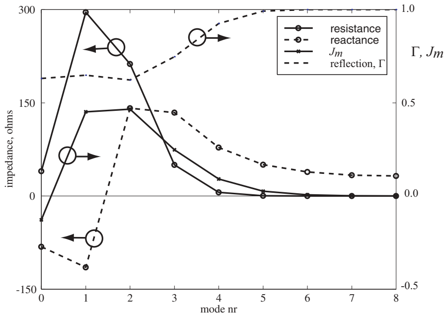
Figure 8.23. Circular dipole array phase-mode impedance performance. Solid line with circles: resistance. Dashed line with circles: reactance. Dashed line: reflection coefficient. Solid line with crosses: the Bessel function J_m(kR) .
