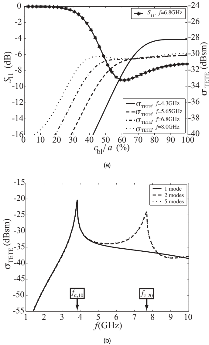
Figure 11.30. (a) Reflection coefficient and RCS as a function of iris gap for a single element with an iris placed 1 mm from the aperture (15 modes, \theta = 60^\circ ). (b) The RCS for a single element without iris as a function of frequency ( \theta = 60^\circ ).
