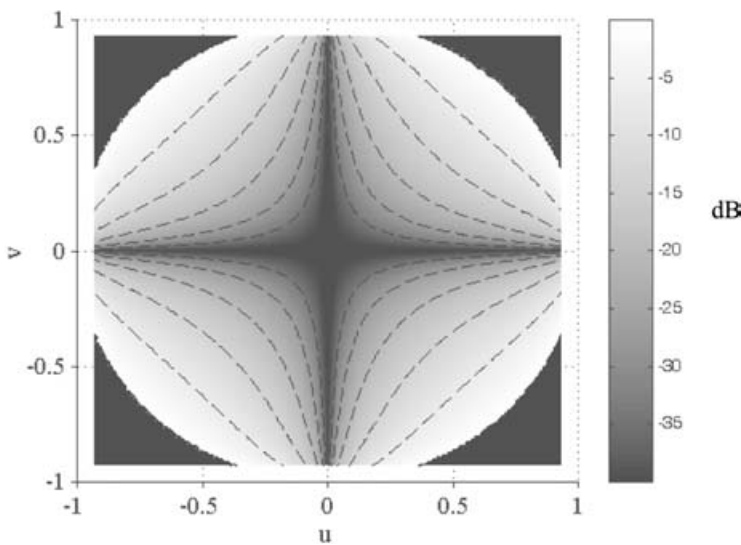
Figure 8.44. Cross polarization isolation for a dipole pair.
