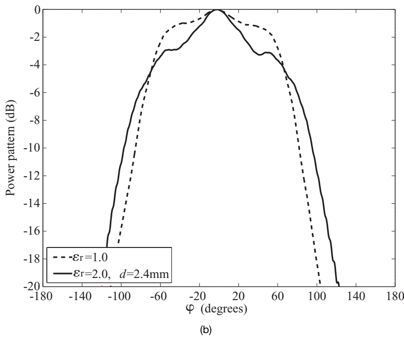
Figure 6.56. Normalized E -plane embedded-element pattern for the element in the middle of a 4 \times 32 elements array (solid line). The noncoated result is also included for comparison (dashed line). (a) f = 5.65 GHz. (b) f = 6.8 GHz [Thors et al. 2003].
