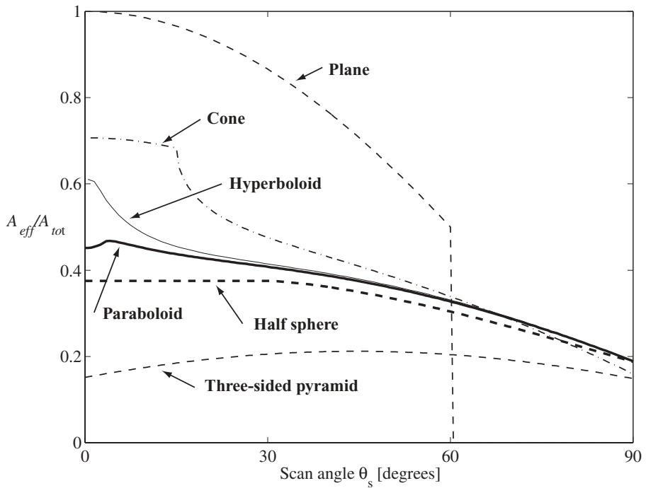
Figure 3.20. The normalized effective area versus scan angle from the zenith; h/R = 1 .
