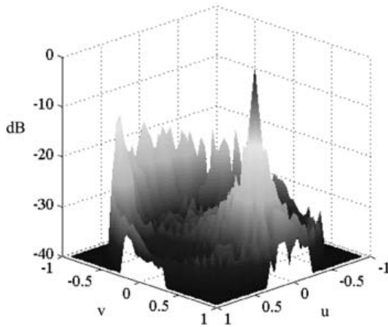
Figure 8.39. The E_\theta component of the radiated field in (u, v) space.
