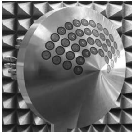
Figure 8.2. Dual-polarized patch elements on a cone. See also color insert, Figure 4. (Courtesy of FGAN Research Establishment for Applied Science, Wachtberg-Werthhoven, Germany.)
