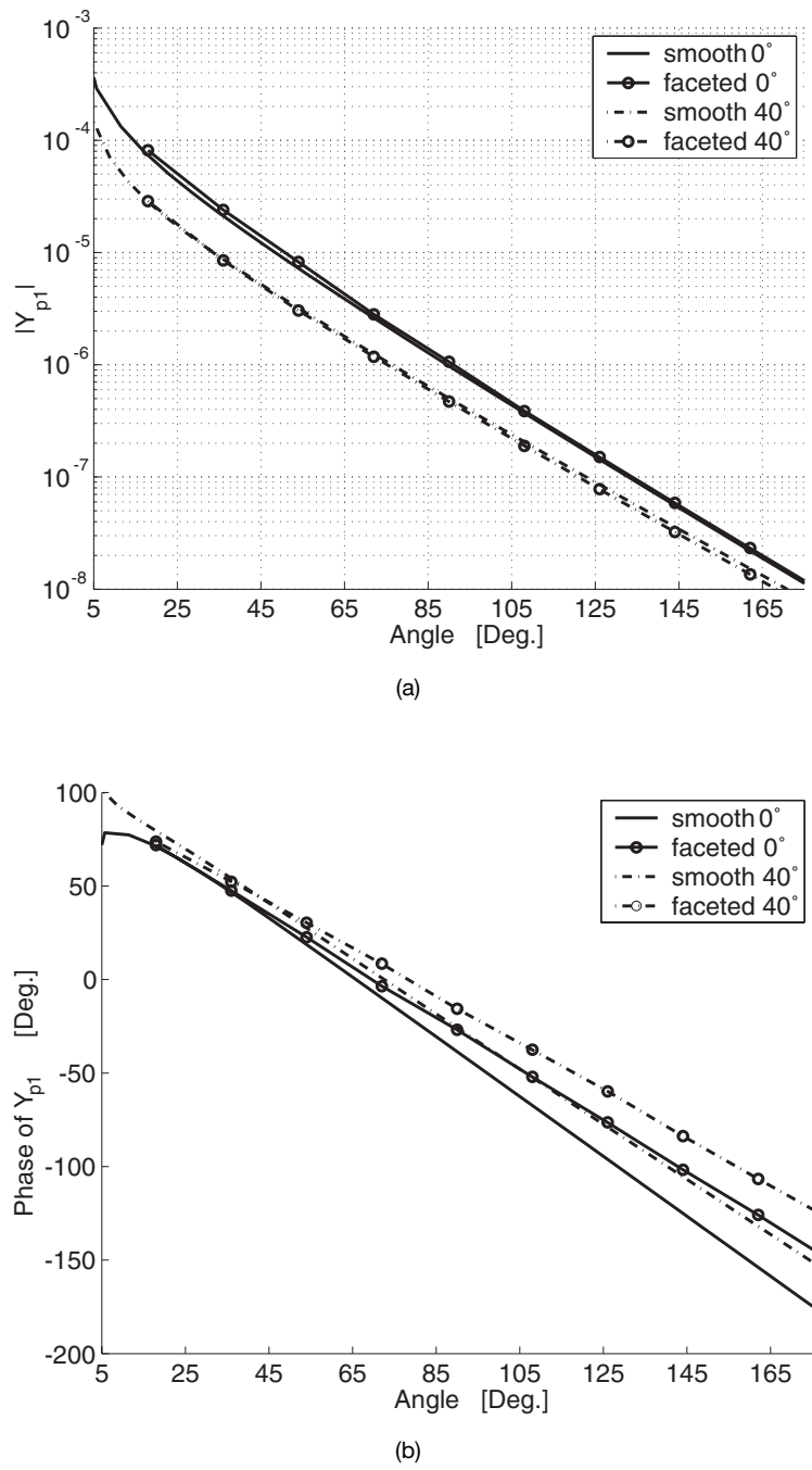
Figure 6.42. The isolated mutual coupling (admittance) ( \Omega^{-1} ) for a faceted circular cylinder (lines with circles), \alpha = 0^\circ and 40^\circ . Results for a smooth circular cylinder are also included for comparison [Marcus et al. 2003]. (a) Amplitude. (b) Phase.
