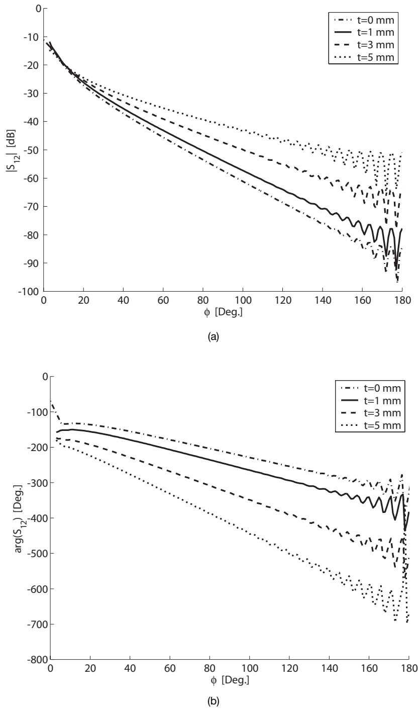
Figure 6.48. Isolated E -plane coupling along the cylindrical surface in the azimuth ( \alpha = 0^\circ ). Here, the coupling is studied with respect to the thickness of the lossless coating; a single-waveguide mode is used. (a) The amplitude. (b) The phase with the free-space contribution subtracted.
