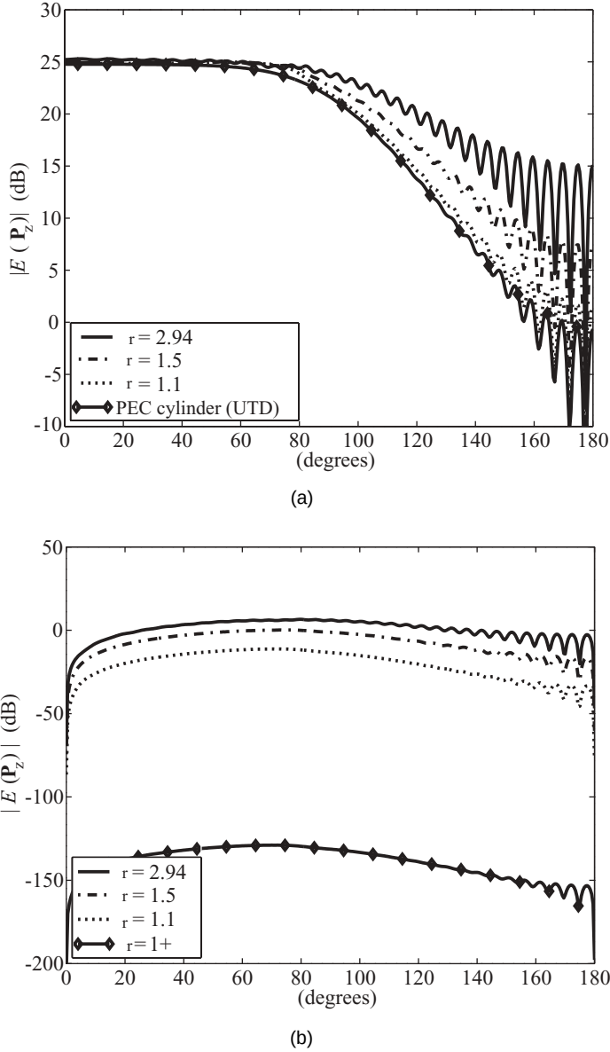
Figure 6.53. Radiation patterns from a \hat{z} -directed magnetic dipole ( \theta = 50^\circ ) versus the relative permittivity of the lossless coating. The noncoated result is also included for comparison (line with diamonds). (a) |E(\mathbf{P}_z)| . (b) |E(\mathbf{P}_z)| ( \epsilon = 10^{-6} ) [Thors and Rojas 2003]. Copyright 2003 American Geophysical Union. Reproduced/modified by permission of American Geophysical Union.
