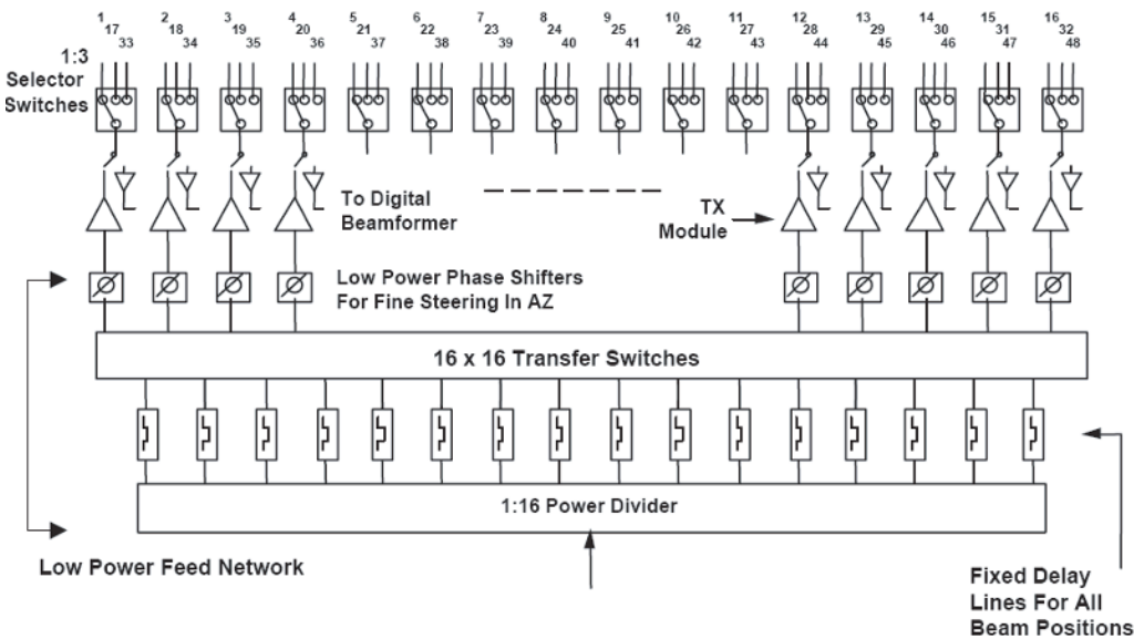
Figure 9.5. Beam forming network according to [Lee et al. 2002] with amplifiers in the transmit paths.
