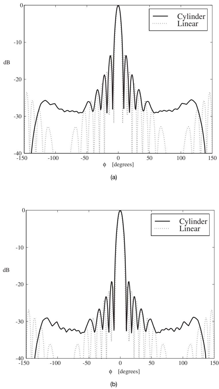
Figure 8.13. 16 elements with 0.5 \lambda spacings on a 120^\circ arc. No tapering (a), -20 dB Taylor (b), and -30 dB Taylor (c). (continued)
