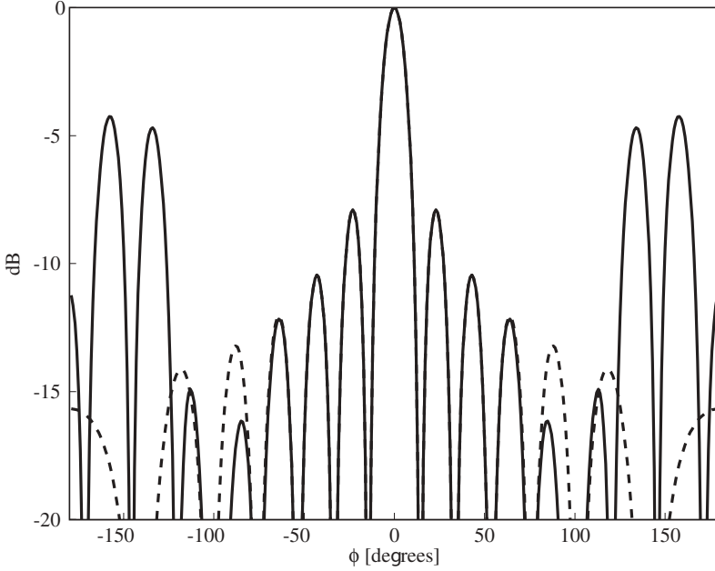
Figure 2.26. Radiation patterns for a continuous circular ring source pattern (dashed line) and a corresponding discrete array with 16 isotropic elements spaced at 0.6 \lambda (solid line).
