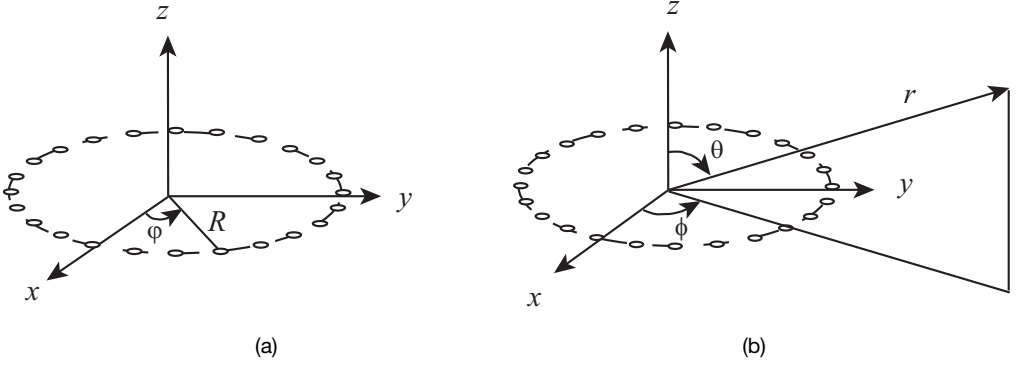
Figure 2.5. Local (a) and far-field (b) coordinates for the circular array.
