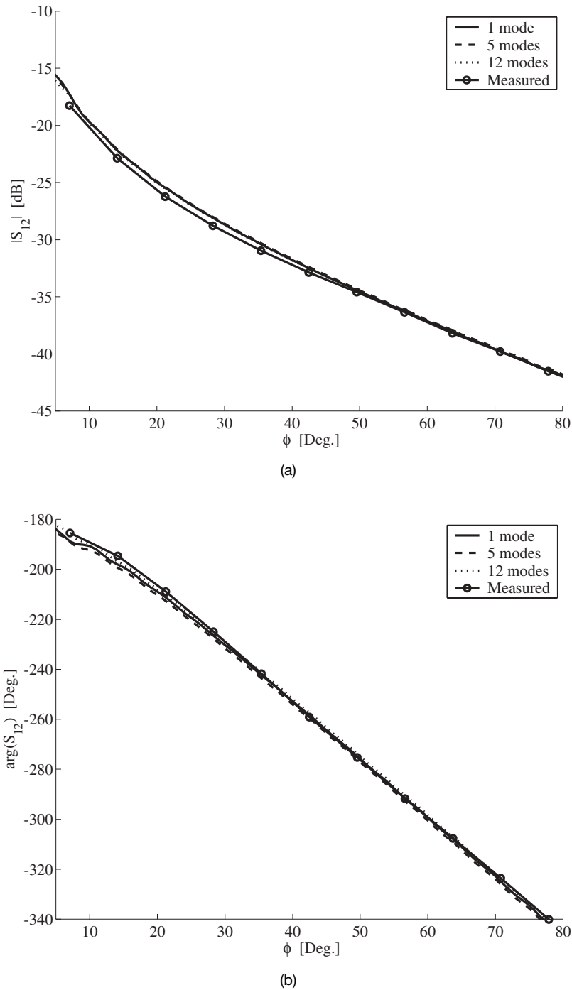
Figure 6.49. Isolated E -plane coupling along the cylindrical surface in the azimuth ( \alpha = 0^\circ ). Here, the coupling is studied with respect to the number of modes used when \epsilon_r = 2.32 and t = 3.99 mm. Measured data are also included (line with circles). (a) The amplitude. (b) The phase with the free-space contribution subtracted.
