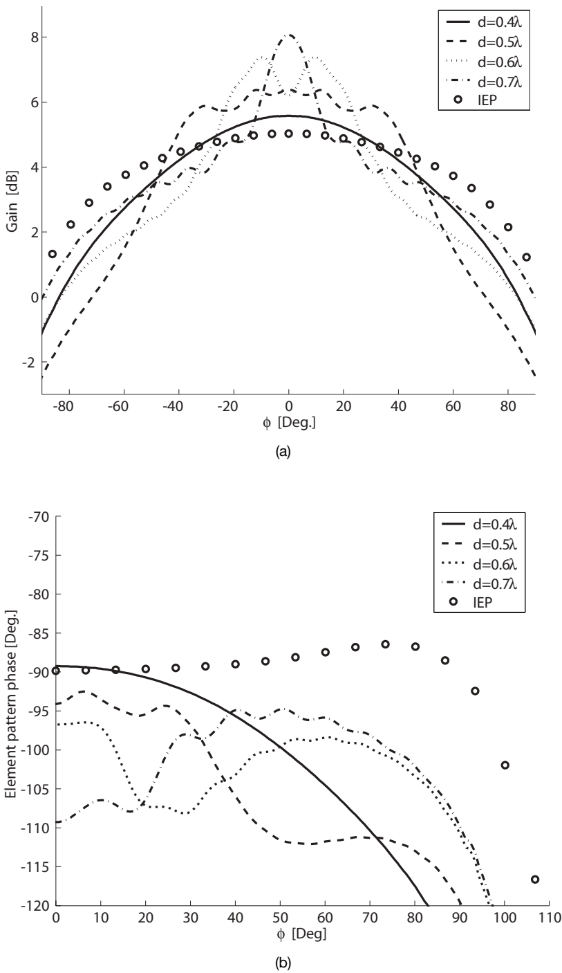
Figure 6.21. The gain of the E -plane embedded-element pattern for a single-ring array versus the element spacing for a fixed radius ( R = 5\lambda ). The isolated element pattern (IEP) is also shown for comparison (circles). (a) Gain. (b) Phase.
