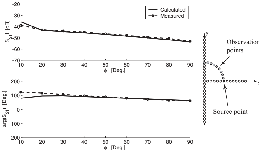
Figure 7.8. Isolated coupling along the circle arc, [R, \phi] polarization. The source point is element +x_6 . Solid line: calculated; dashed line: measured.
