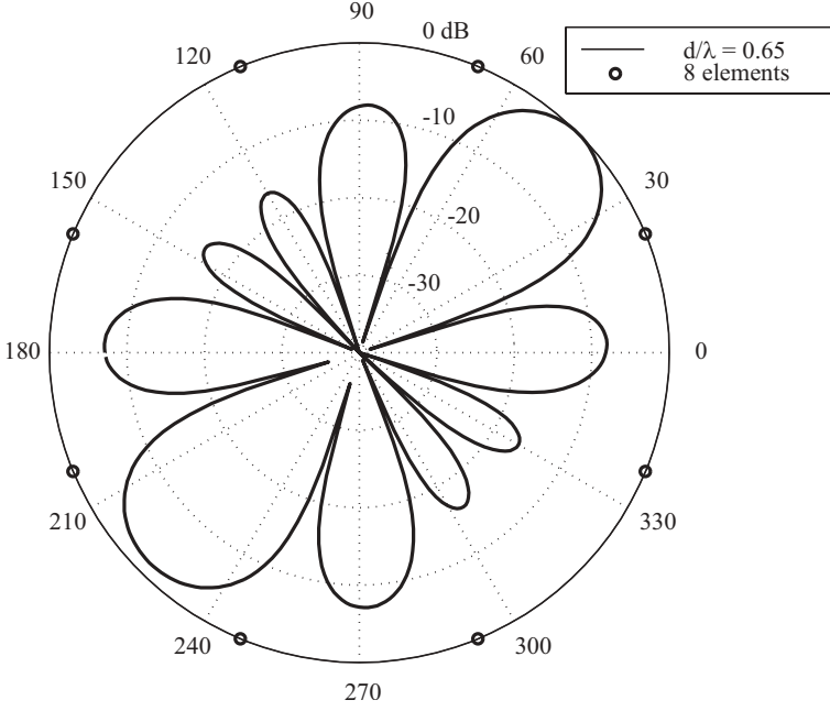
Figure 2.8. A cophasal beam scanned to +45^\circ .
