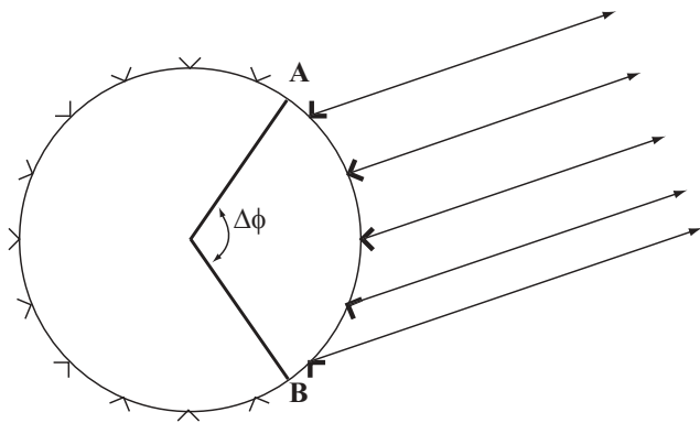
Figure 8.14. Phase steering with a fixed active region (between A and B).
