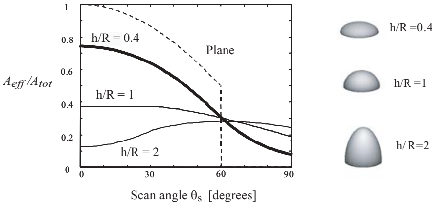
Figure 3.16. Normalized effective area for ellipsoidal shapes with different heights.
