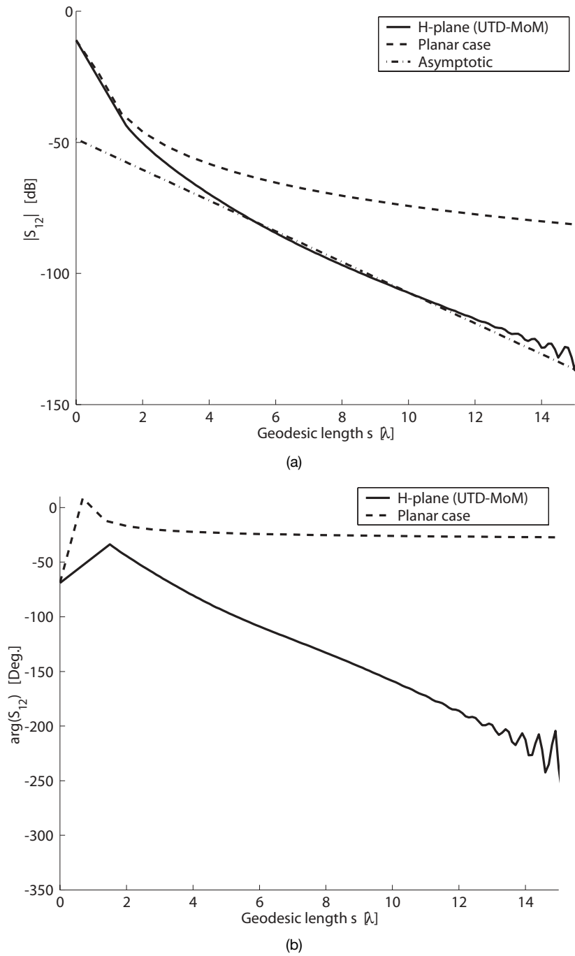
Figure 6.3. The isolated mutual coupling along the circumferential direction of a cylinder while using axially polarized elements, that is, the isolated coupling in the H plane (solid line). The result is compared with the corresponding planar case (dashed line). Note that the distance in wavelengths corresponds to an angular interval of approximately 180^\circ at the cylinder. (a) Amplitude. The result is also compared with an asymptotic formula in Table 6.1 (dash-dotted line). (b) Phase.
