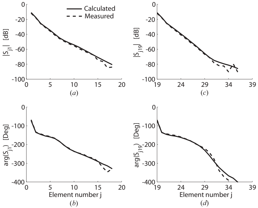
Figure 6.15. The array mutual coupling in the E plane for the first row (elements 1 \rightarrow 18 ) and the second row (elements 19 \rightarrow 36 ). Five-mode approximation, f = 5.65 GHz. Solid line: calculated, dashed line: measured. (a) Amplitude, first row. (b) Phase, first row. (c) Amplitude, second row. (d) Phase, second row [Persson and Josefsson 2001].
