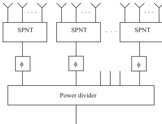
Figure 9.3. A switch matrix feed with phase shifters for fine steering of the beam.
