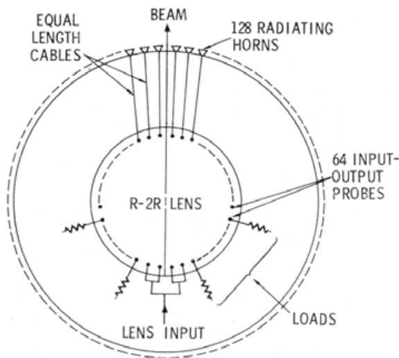
Figure 9.9. The R-2R lens feed system [Boyns et al. 1968].
