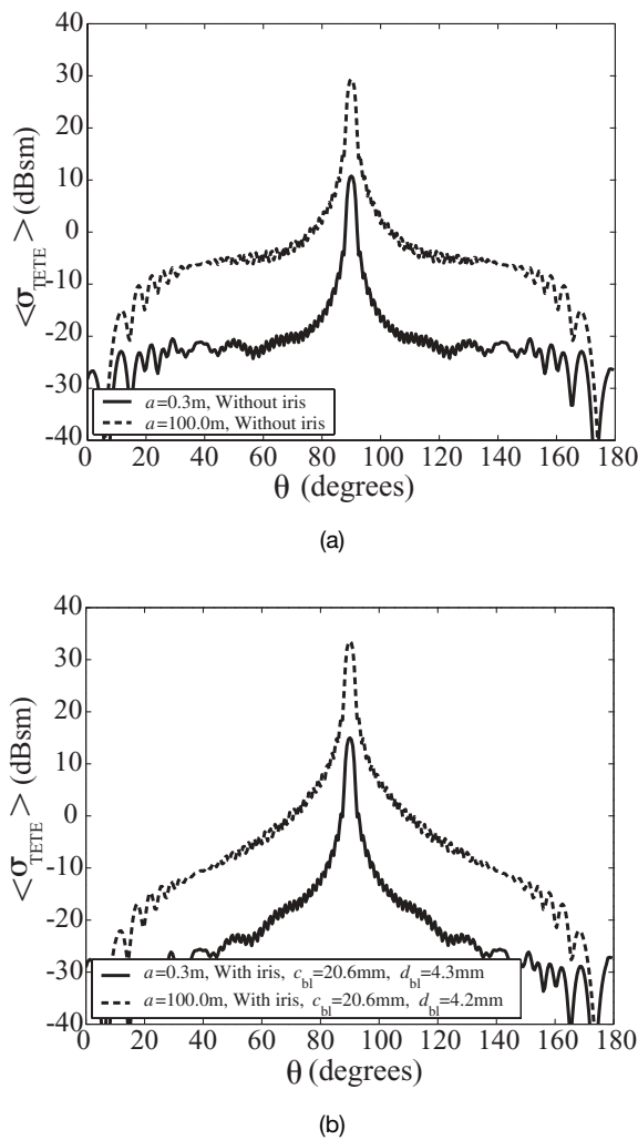
Figure 11.32. The H -plane RCS ( 2^\circ sliding window average) of a cylindrical (solid line) and a planar (dashed line) array antenna (triangular grid, 40 \times 32 elements, 6.8 GHz, 15 modes). (a) Without irises. (b) With irises (matched).
