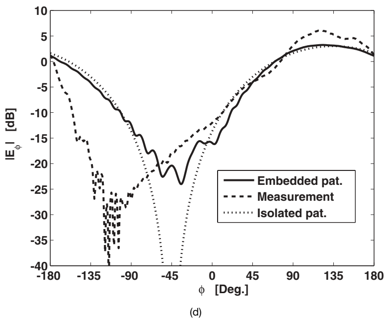
Figure 6.69. (cont.) (c) Edge element, vertical polarization. (d) Edge element, horizontal polarization.
