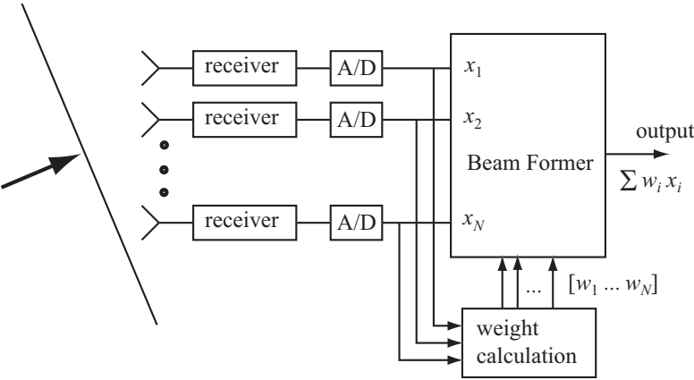
Figure 9.21. An adaptive beam forming antenna system with received signals [x_1, \dots, x_N] forming the signal vector.
