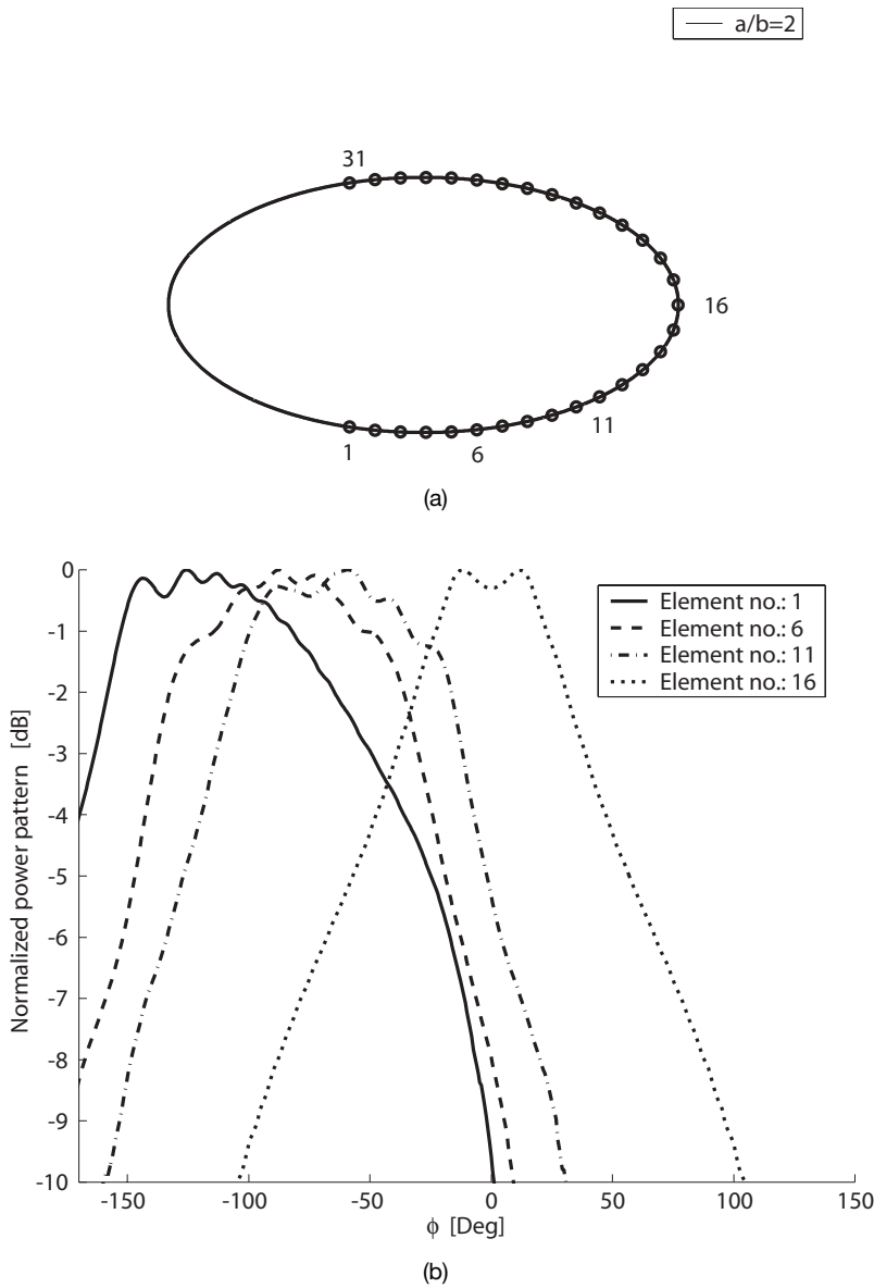
Figure 6.39. Embedded-element patterns in the E plane due to apertures in a sector array containing 31 elements, elliptic cylinder ( a/b = 2 , a = 5 \lambda ). The element-to-element distance equals 0.5 \lambda . (a) The geometry. (b) The results.
