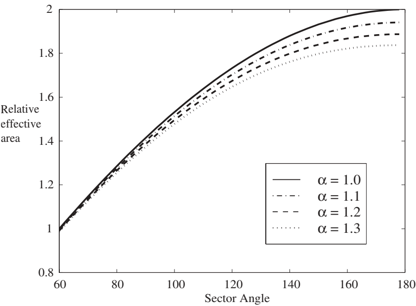
Figure 3.7. Relative effective area versus sector angle for different values of \alpha .
