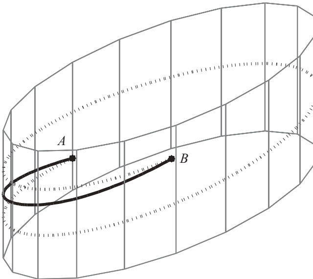
Figure 5.6. The first- and second-order geodesics connecting A and B on an elliptic cylinder with the following parameters: a = 0.3 , b = 0.8 , \alpha_1 = 0.14 , \beta_1 = 0 , \alpha_2 = 0.0396 , and \beta_2 = 0 .
