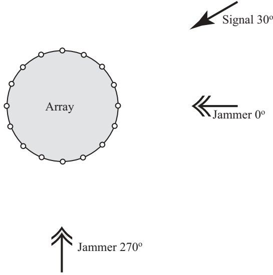
Figure 9.22. Test scenario with one signal competing with two jamming signals.
