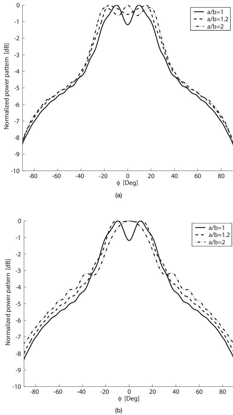
Figure 6.36. The embedded-element pattern versus the shape of elliptic surfaces with an element-to-element distance of 0.6\lambda . \phi is a relative angle and equals zero at the element position. (a) The element on the flattest part is excited. (b) The element on the most strongly curved part is excited.
