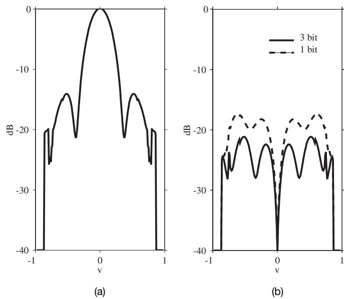
Figure 8.46. Co-polarization (a) and cross polarization (b) with different polarization control resolutions.
