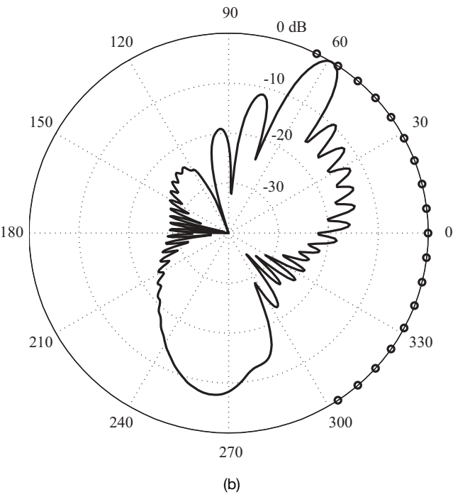
Figure 8.15. Phase scanning (fixed active region, uniform amplitude). The element locations are marked with small circles. (a) 30°, (b) 60°, and (c) 90° scan angles. ( continued )
