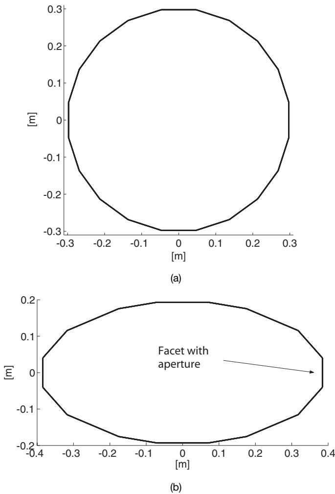
Figure 6.41. Faceted geometries, f = 10 GHz. (a) The circular cylinder with a radius of 10\lambda ; the number of facets is 20. (b) The elliptic cylinder, the facet with the source aperture is shown. The ellipticity is a/b \approx 2 and the number of facets is 16 [Marcus et al. 2003].
