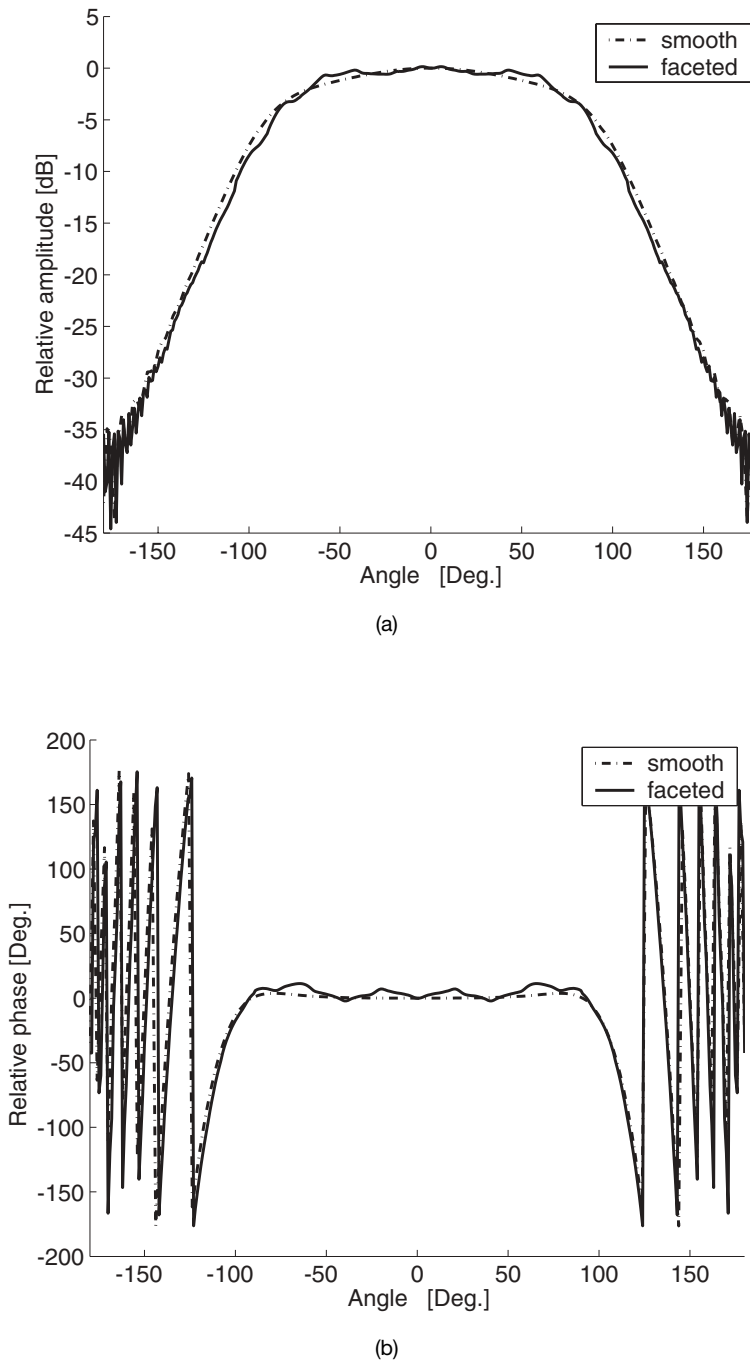
Figure 6.44. The isolated-element pattern for a faceted circular cylinder (solid line). The radius of the cylinder is 10\lambda and the number of facets is 20. Results for a smooth circular cylinder are also included for comparison (dash-dotted line) [Marcus et al. 2003]. (a) Amplitude. (b) Phase.
