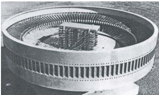
Figure 9.1. A 128 element vector transfer-matrix-fed S-band array [Boyns et al. 1970].
