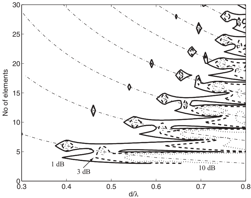
Figure 2.19. Ripple amplitude contour lines (1 dB solid, 3 dB dashed, and 10 dB dotted) for circular ring arrays with isotropic elements and m = 0 mode excitation. Along the dash-dotted lines, J_0(kR) = 0 .
