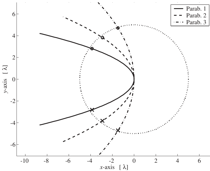
Figure 6.30. The parabolic geometry and the position of the first aperture (cross) and the final position of the second aperture (circle). The circular cylinder ( R = 5\lambda ) is also shown for geometrical reference.
