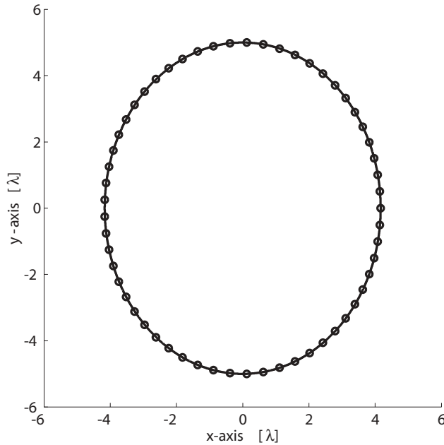
Figure 6.34. The elliptic cylinder array with an element-to-element distance of 0.5\lambda , a/b = 1.2 .
