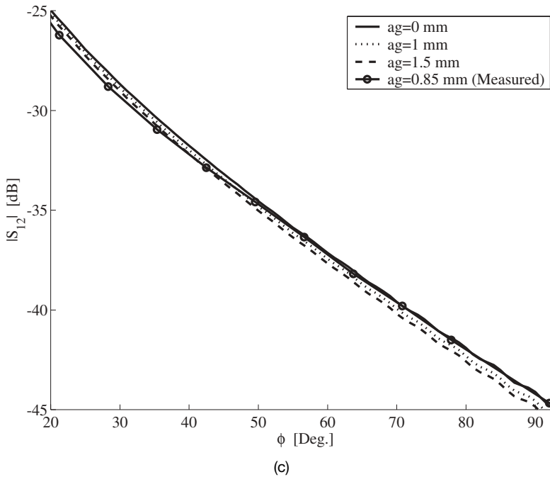
Figure 6.50. (cont.) (c) Close-up view of the amplitude result.
