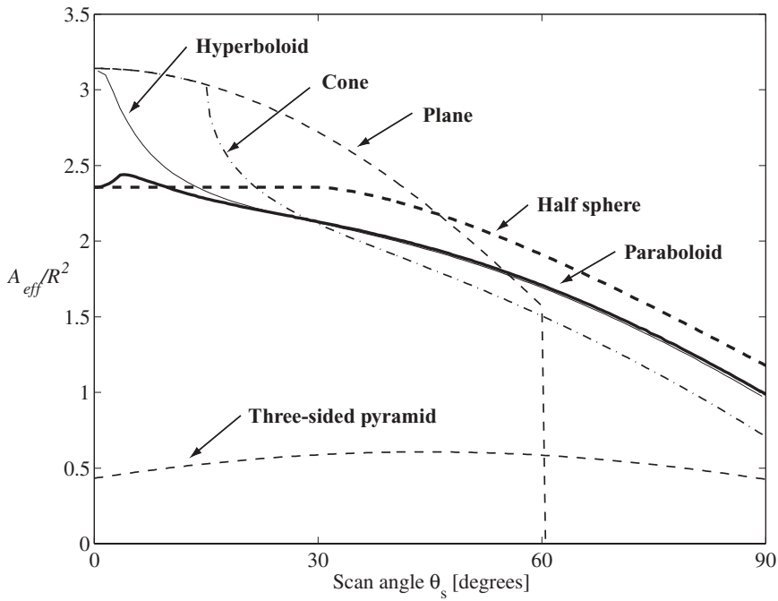
Figure 3.19. The effective area for several types of surfaces; h/R = 1 .
