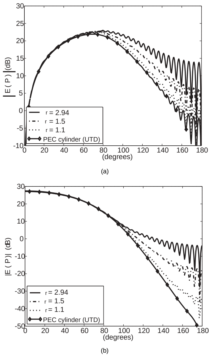
Figure 6.54. Radiation patterns from a - directed magnetic dipole ( \theta = 50^\circ ) versus the relative permittivity of the lossless coating. The noncoated result is also included for comparison (line with diamonds). (a) |E| . (b) |E| . Copyright 2003 American Geophysical Union. Reproduced/modified by permission of American Geophysical Union.
