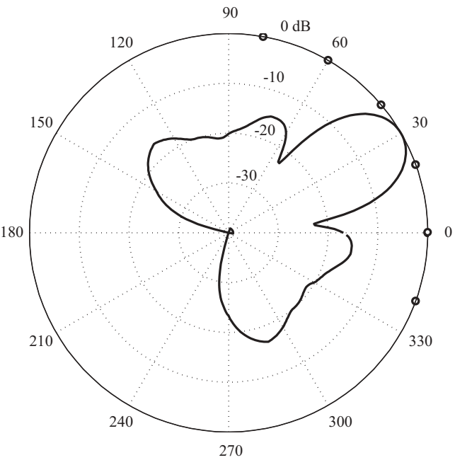
Figure 8.12. Radiation pattern with a 120^\circ sector active.
