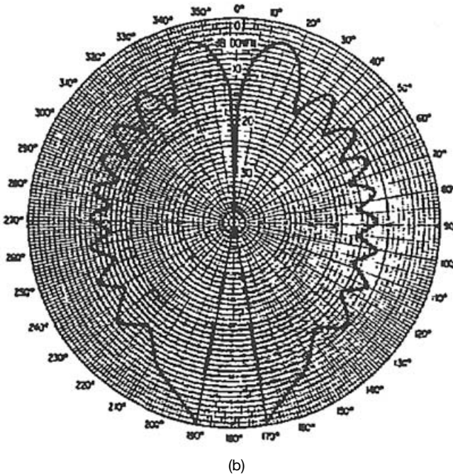
Figure 6.79. Calculated single element pattern due to a circumferential slot for the half-cone angle \theta_c = 10^\circ [Pridemore-Brown and Stewart 1972]. (a) k_0 a = 10 . (b) k_0 a =
