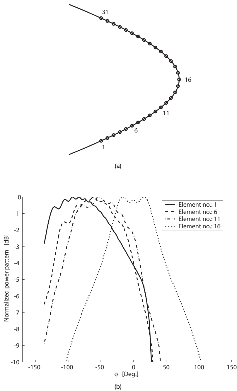
Figure 6.40. Embedded-element patterns in the E plane due to apertures in a sector array containing 31 elements, hyperbolic cylinder ( b/a = 0.3 , a = 16.67\lambda ). The element-to-element distance equals 0.5\lambda . (a) The geometry. (b) The results.
