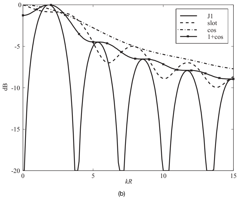
Figure 2.16. Mode stability for modes m = 0, 1, 2 , and 5 in (a) to (d), respectively. Element types: isotropic (solid line), slot (dashed), \cos \phi (dash-dotted), and 1 + \cos \phi (solid line with crosses).
