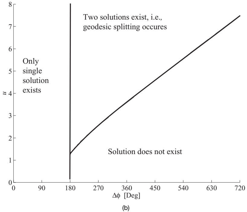
Figure 5.15. The set of parameters for which no solution exists, one solution exists, and two solutions exist to the geodesic equation when (a) a = 0.5 and (b) a = 1.6 . Note that the second-order geodesics begin at \Delta\phi = 360^\circ in both cases. Furthermore, it is also possible to find third-order geodesics in some cases ( \Delta\phi \geq 720^\circ ).
