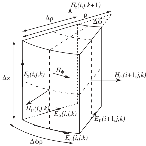
Figure 4.8. Field components placement in the FDTD unit cell in cylindrical coordinates, after [Marcano et al. 1998].
