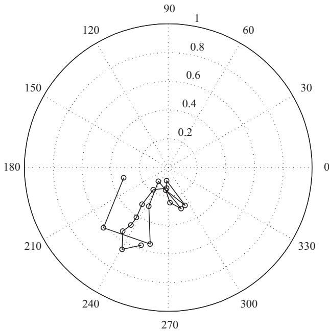
Figure 10.18. The active reflection coefficient for the 18 elements.
