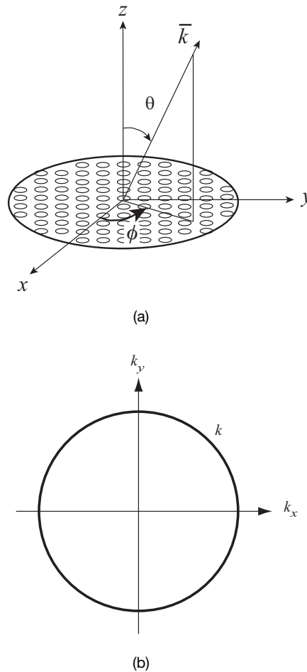
Figure 8.8. A planar array (a), and the visible space inside the circle with radius k (b).
