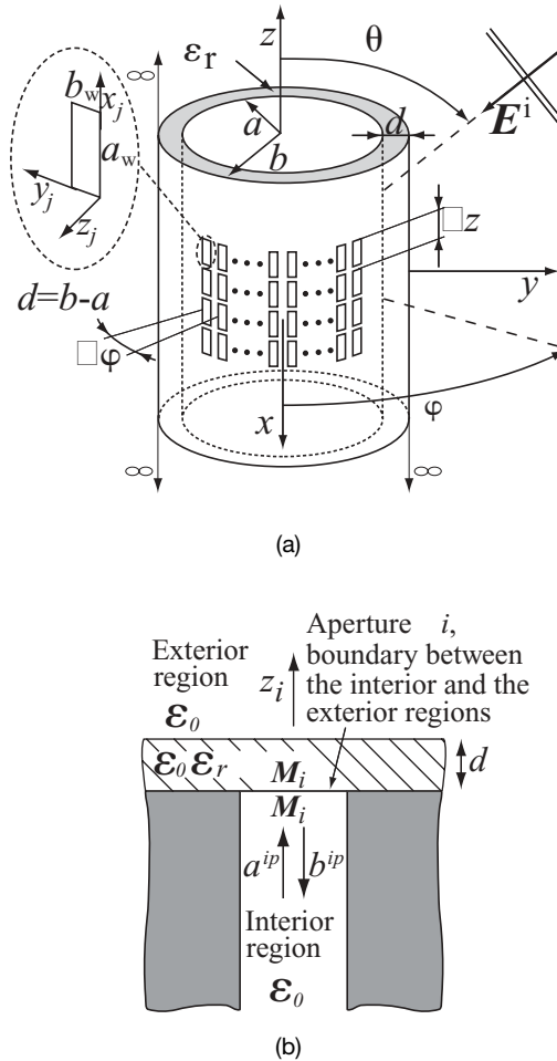
Figure 11.3. (a) The conformal array antenna coated with a dielectric layer with relative permittivity \epsilon_r (b) The exterior and the interior regions of aperture i .
