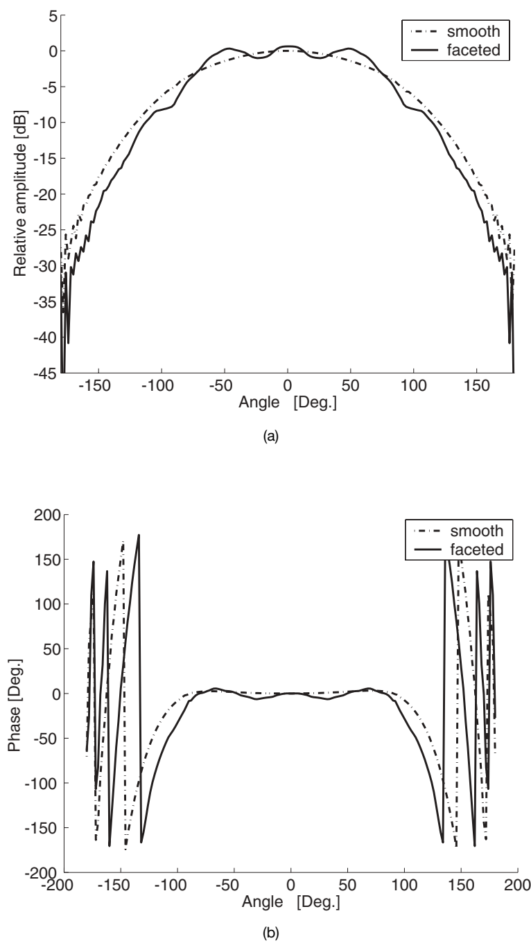
Figure 6.45. The isolated-element pattern for a faceted elliptic cylinder (solid line). The ellipticity is a/b \approx 2 and the number of facets is 16. Results for a smooth elliptic cylinder are also included for comparison (dash–dotted line) [Marcus et al. 2003]. (a) Amplitude. (b) Phase.
