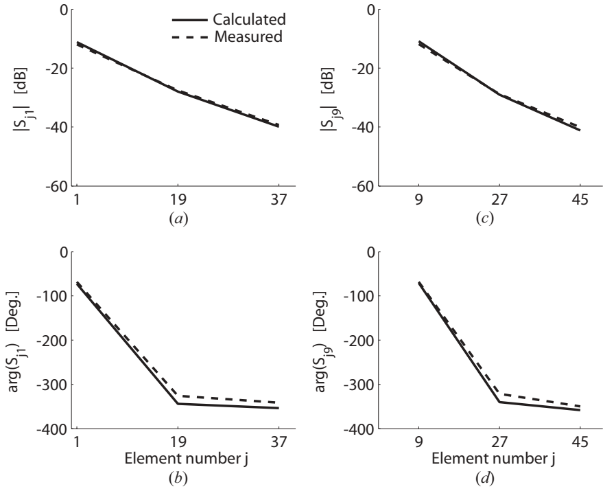
Figure 6.17. The array mutual coupling in the H plane for an edge column and for the center column. Ten-mode approximation, f = 5.65 GHz. Solid line: calculated, dashed line: measured. (a) Amplitude, edge column. (b) Phase, edge column. (c) Amplitude, center column. (d) Phase, center column.
