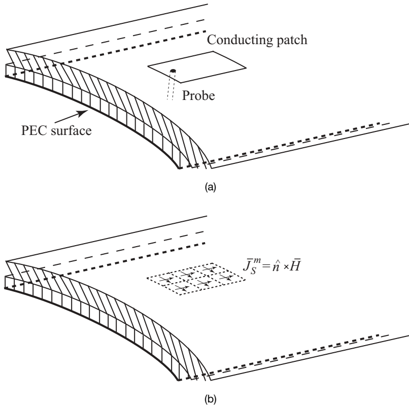
Figure 4.15. (a) The original problem of a probe-fed rectangular-patch antenna on a coated multilayer surface. (b) The equivalent problem.
