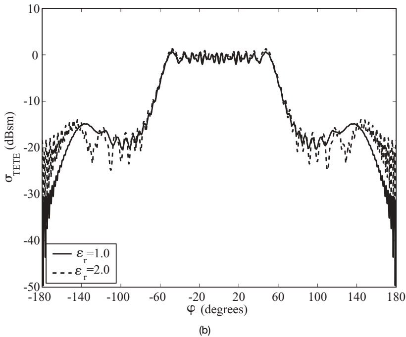
Figure 11.21. The E -plane RCS for a 4 \times 32 element array with a dielectric coating (dashed line). The noncoated case is included as reference (solid line). (a) 4.3 GHz. (b) 6.8 GHz.
