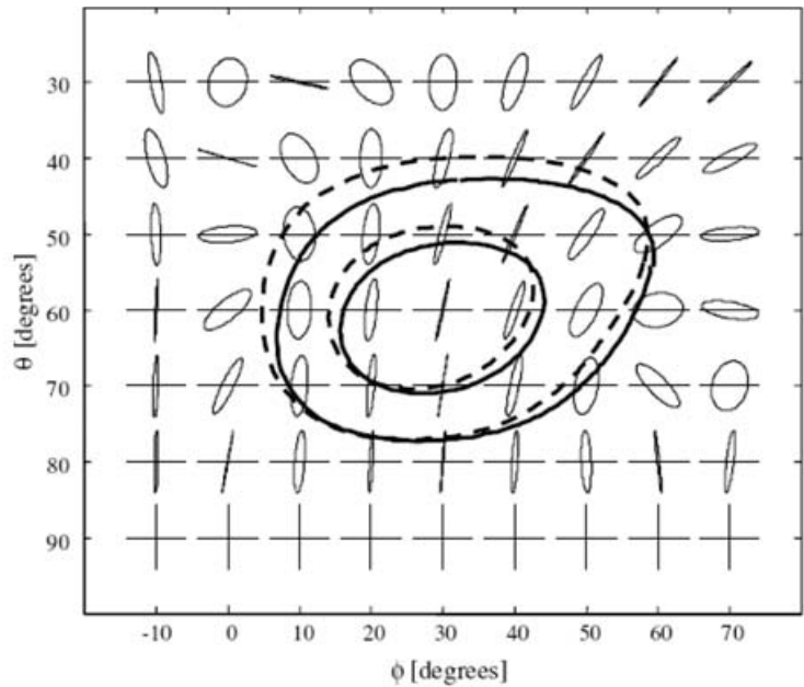
Figure 8.32. Polarization chart for a beam scanned 30^\circ both in elevation and azimuth. The -3 dB and -10 dB contours of the main beam are shown. The solid and dashed contours represent horizontal and vertical polarization, respectively.
