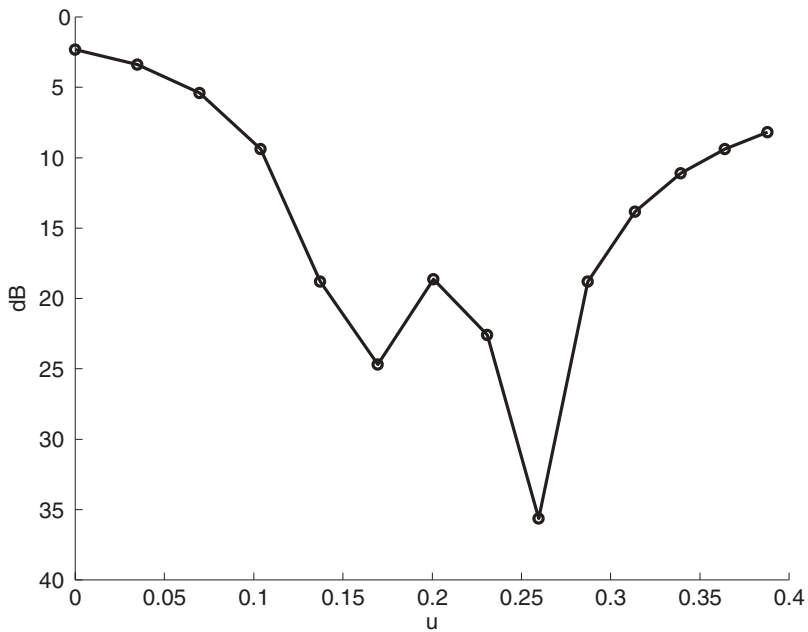
Figure 7.17. [R, R] polarization. Test of a geometrical approach for calculating the mutual coupling [Josefsson et al. 2002]; compare with Figure 7.12.
