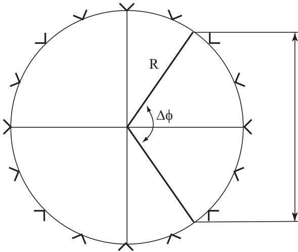
Figure 3.6. Active sector of a cylindrical array.
