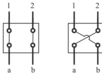
Figure 9.4. (a) A feed system using a transfer switch matrix. The transfer matrix allows routing of any input to any output. (b) The two states of a transfer switch.
