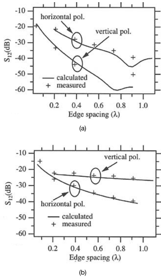
Figure 6.65. Calculated (solid line) and measured (+) isolated mutual couplings between two patches, for vertical and horizontal polarizations, versus edge spacing in wavelengths. (a) Separated in the horizontal direction. (b) Separated in the vertical direction [Raffaelli et al. 2005].
