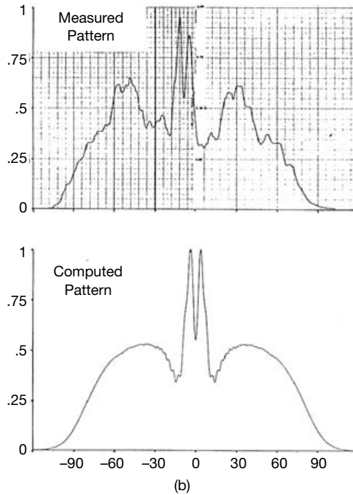
Figure 6.24. Measured and computed embedded-element patterns at broadside. (a) Azimuth spacing 0.73\lambda . (b) Azimuth spacing 0.79\lambda [Munger et al. 1971].
