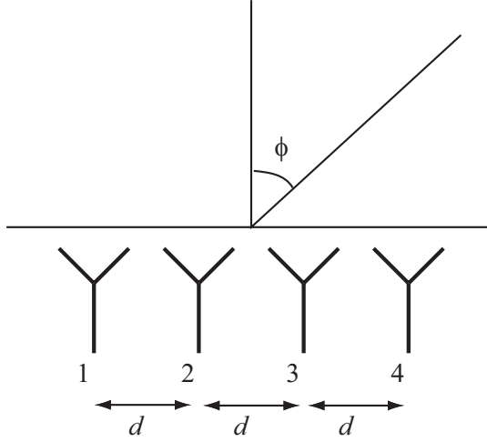
Figure 2.4. A linear array antenna with element spacings d .
