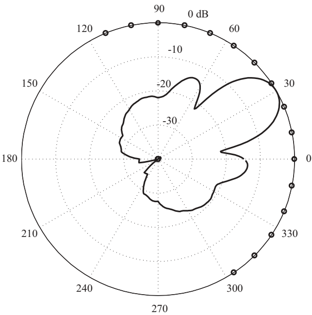
Figure 8.11. As for Figure 8.10, but with the element spacings reduced to 0.25 \lambda .
