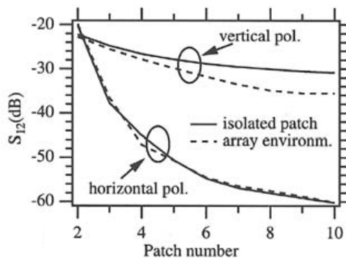
Figure 6.66. Mutual coupling in the z direction for horizontally and vertically polarized patches in a 5 \times 10 elements array (dashed line) compared to the mutual coupling between two isolated patches (solid line) [Raffaelli et al. 2005].
