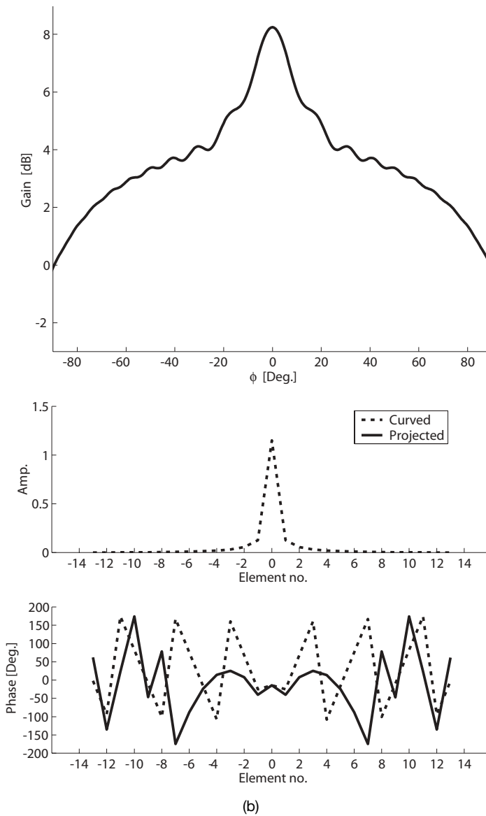
Figure 6.22. (cont.) (b) E -plane gain and element excitation for a 0.7\lambda element-to-element distance. The projected excitation (solid line) in both cases is the excitation of the elements when projected on a planar screen in front of the array.
