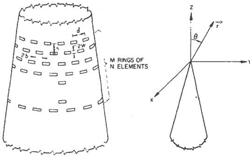
Figure 6.81. The conical array geometry [Balzano and Dowling 1974].
