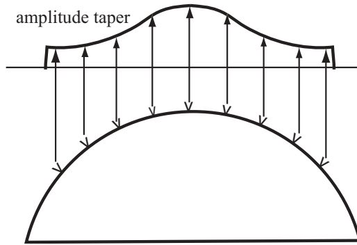
Figure 10.6. Projecting the element locations onto the planar aperture to sample excitation.
