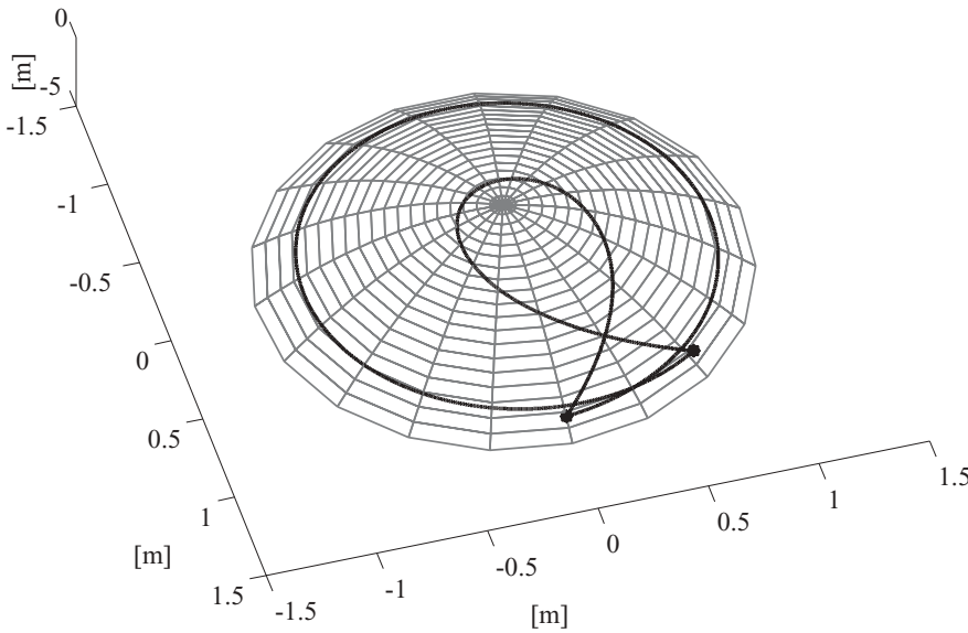
Figure 5.16. An example of geodesic splitting for second-order geodesics encircling the surface in the positive \varphi direction. In this case, a = 0.5 , u_A = 2 , \varphi_A = 0^\circ , and u_B = 2 , \varphi_B = 400^\circ , respectively. Note, there is also a first-order geodesic in the positive \varphi direction that is not included in this picture.
