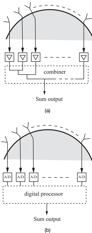
Figure 9.19. Analog beam forming (a) and digital beam forming (b) can in principle perform the same functions.
