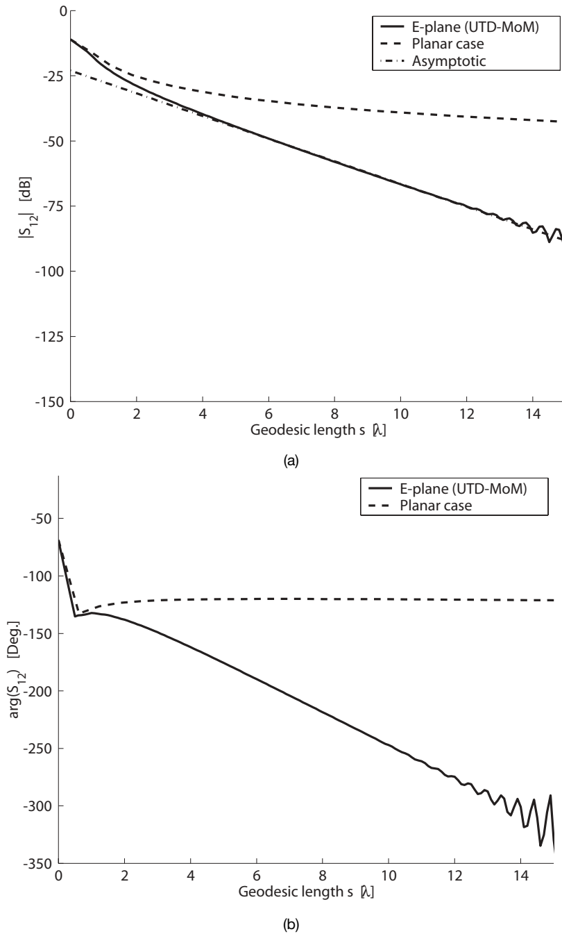
Figure 6.2. The isolated mutual coupling along the circumferential direction of a cylinder while using circumferentially polarized elements, that is, the isolated coupling in the E plane (solid line). The result is compared with the corresponding planar case (dashed line). Note that the distance in wavelengths corresponds to an angular interval of approximately 180^\circ at the cylinder. (a) Amplitude. The result is also compared with an asymptotic formula in Table 6.1 (dash-dotted line). (b) Phase.
