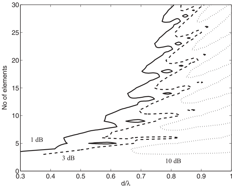
Figure 2.24. Ripple amplitude contour lines (1 dB solid, 3 dB dashed, and 10 dB dotted) for ring arrays with m = 0 mode excitation and 1 + \cos \phi element patterns.
