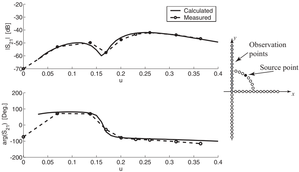
Figure 7.14. Isolated coupling, [R, \varphi] polarization. The source point is element c_5 . Solid line: calculated; dashed line: measured.
