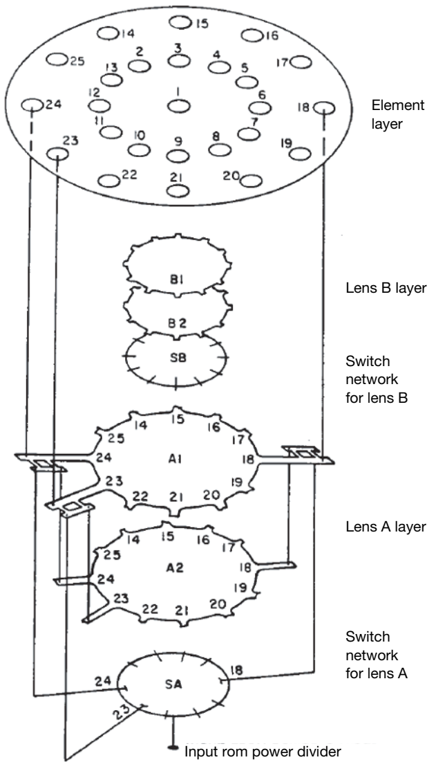
Figure 9.12. A four R-kR lens design for mobile communication [Bodnar et al. 1989].
