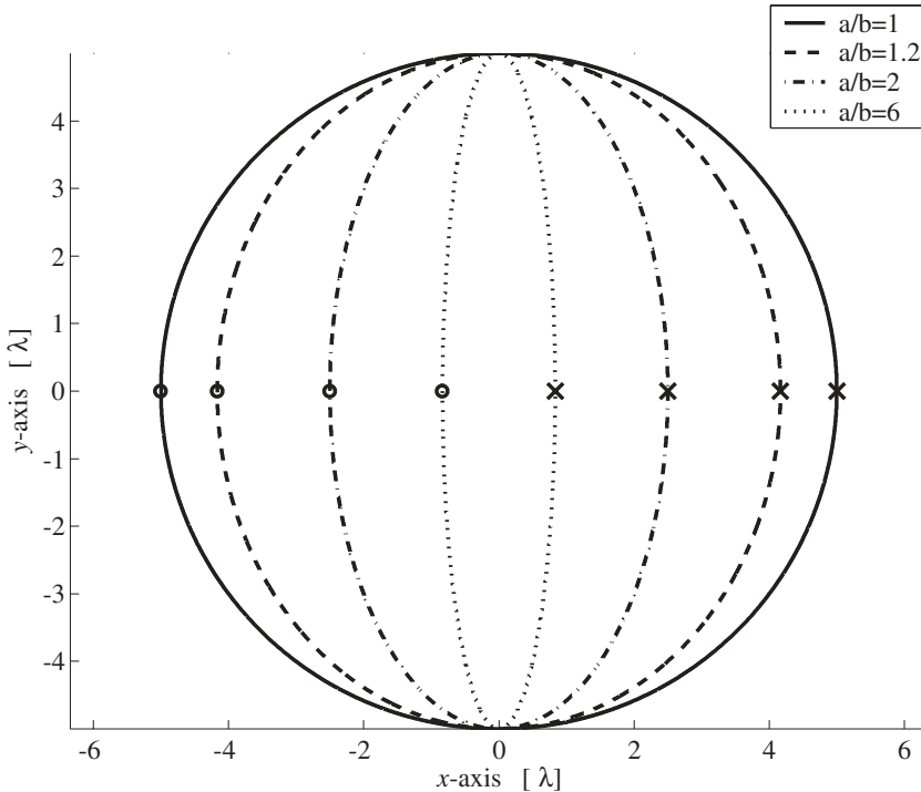
Figure 6.28. The elliptic geometry and the position of the first aperture (cross) and the final position of the second aperture (circle).
