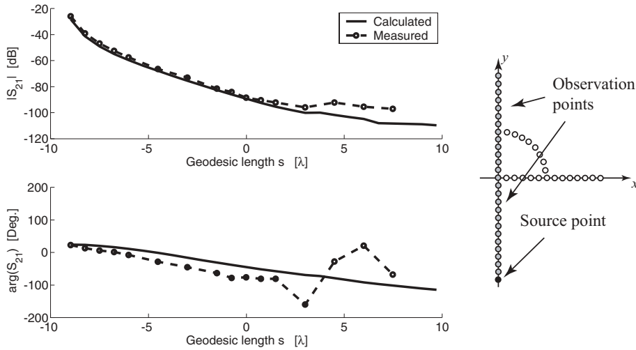
Figure 7.3. Isolated coupling along the y axis, H plane, or [\varphi, \varphi] polarization. The source point is element -y_{13} . Solid line: calculated; dashed line: measured.
