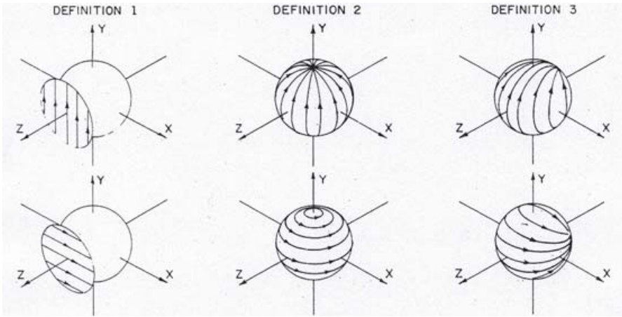
Figure 8.27. Polarization definitions according to [Ludwig 1973].
