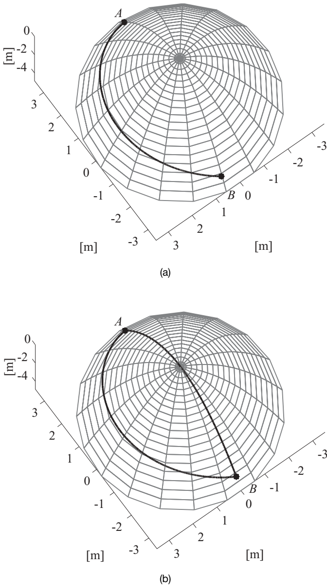
Figure 5.14. A sequence showing the splitting phenomenon and the appearance of the geodesics in the positive \varphi direction. As can be seen, the two geodesics move toward each other when the angular distance increases. Here, A is located at u_A = 2 , \varphi_A = 0^\circ , and a = 1.6 . The observation point B is located at u_B = 2 and the angular distance is (a) \varphi_B = 170^\circ , (b) \varphi_B = 180^\circ , (c) \varphi_B = 200^\circ , (d) \varphi_B = 220^\circ , and (e) \varphi_B = 225.6^\circ . Note that there are geodesics in the negative \varphi direction (not shown) in addition to the geodesics in the positive \varphi direction. ( continued )
