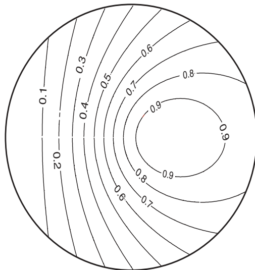
Figure 3.10. Contour plot showing cosine of the element look directions for 30^\circ scan from the zenith.
