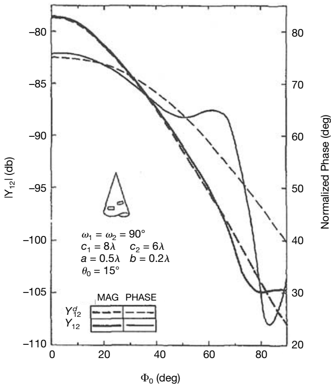
Figure 6.74. Mutual admittance between two circumferential slots on a cone versus the angular separation when separated by a small radial distance [Lee 1978].
