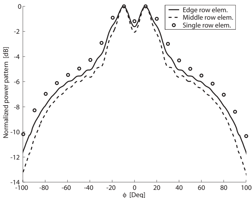
Figure 6.23. The embedded-element pattern for different elements in a 13 \times 52 elements array (solid line: edge-row element, dashed line: middle-row element). The radius equals R = 5\lambda and the element spacing in the azimuth and axial directions is 0.6\lambda and 0.68\lambda , respectively. The single-row result is also shown for comparison (circles).
