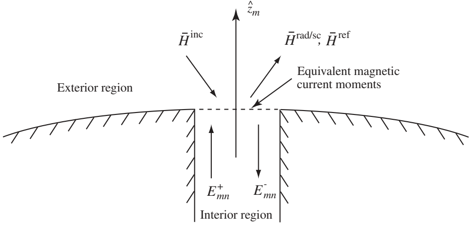
Figure. 4.13. The exterior and interior regions at aperture m for a noncoated PEC surface with the n th waveguide mode.
