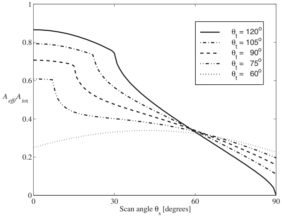
Figure 3.15. Cones with different cone angles. Normalized performance (effective area/cost) versus scan angle from zenith.
