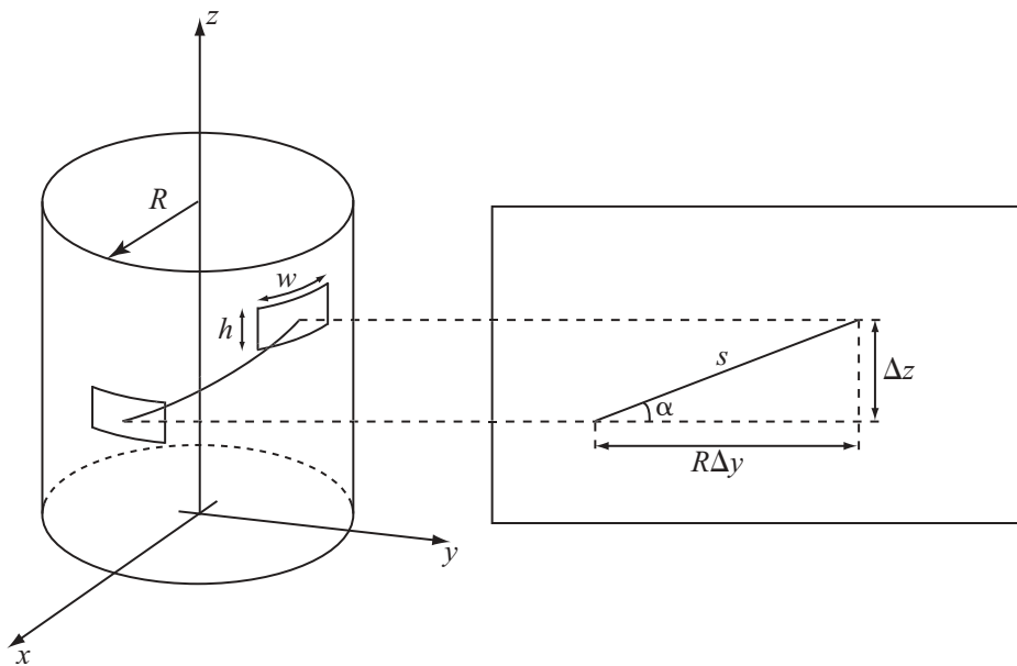
Figure 6.1. Geometry for the study of the characteristics of azimuthally oriented aperture antenna elements on circular cylinders—vertical polarization.
