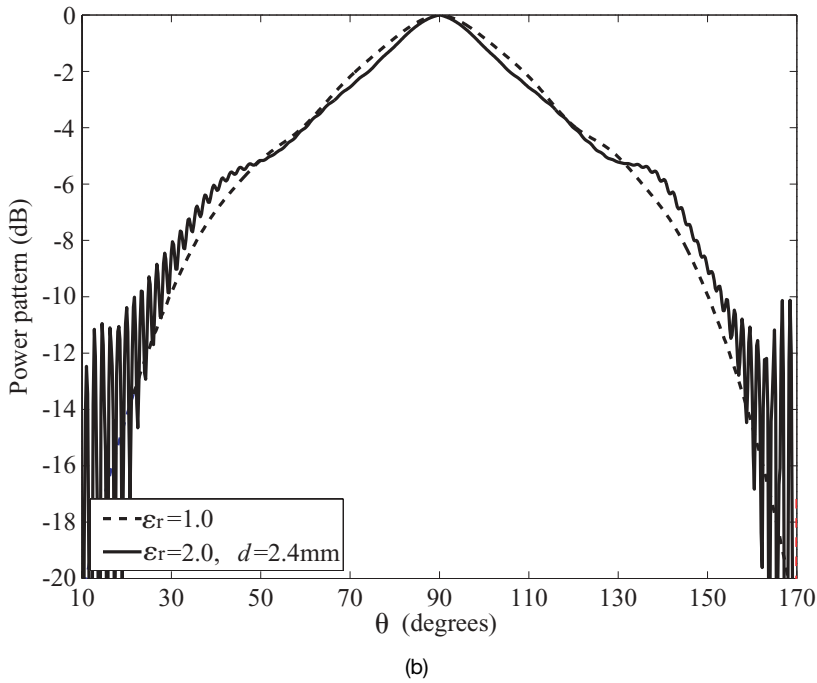
Figure 6.57. Normalized H -plane embedded-element pattern for the element in the middle of a 4 \times 32 elements array (solid line). The noncoated result is also included for comparison (dashed line). (a) f = 5.65 GHz. (b) f = 6.8 GHz [Thors et al. 2003].
