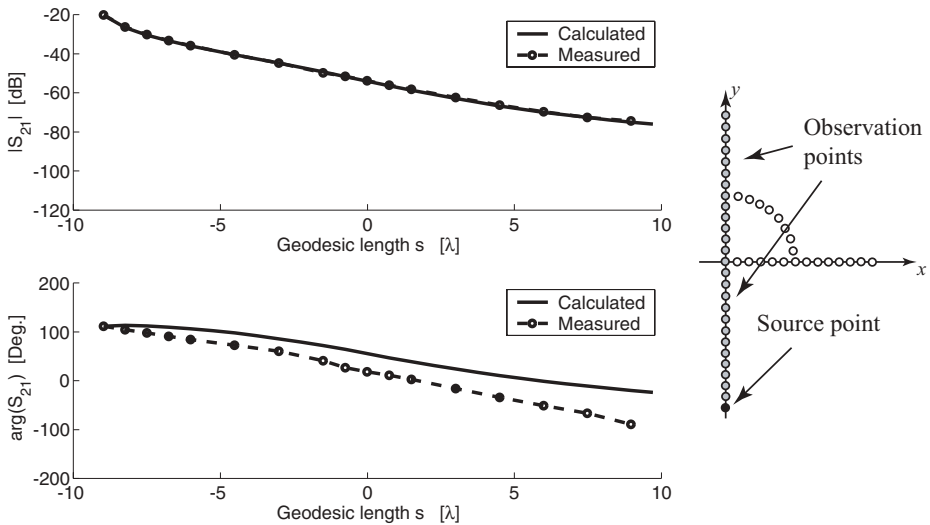
Figure 7.2. Isolated coupling along the y axis, E plane, or [R, R] polarization. The source point is element -y_{13} . Solid line: calculated; dashed line: measured.
