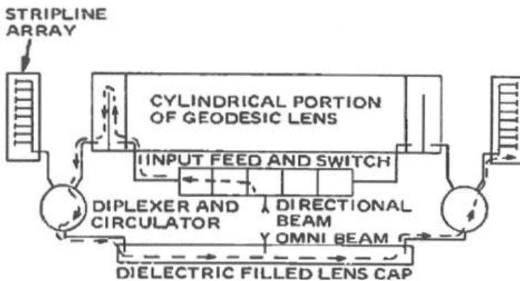
Figure 9.15. Geodesic lens feed system with signal flow in the transmission mode [Holley et al. 1974].
