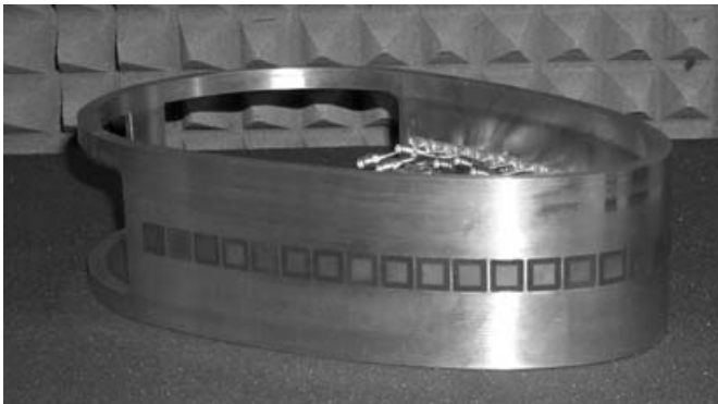
Figure 9.20. Elliptical array with dual-polarized patch elements in cavities for DBF experiments. See also color insert, Figure 9. (Courtesy of FGAN Research Establishment for Applied Science, Wachtberg-Werthhoven, Germany.)
