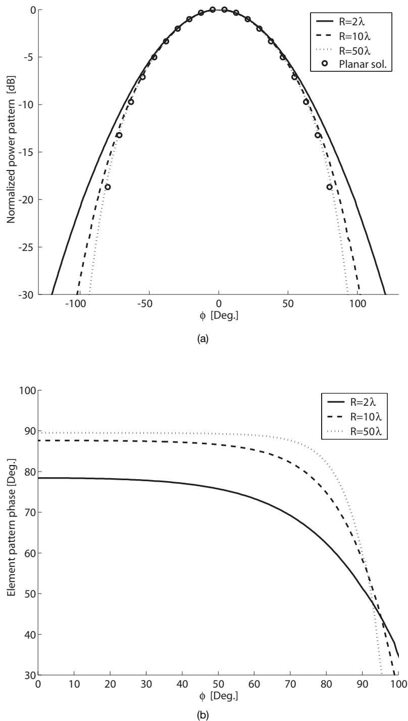
Figure 6.19. The H -plane isolated-element pattern in the azimuth versus the radius of the cylinder. (a) Amplitude. The planar case is also included (circles). (b) Phase.
