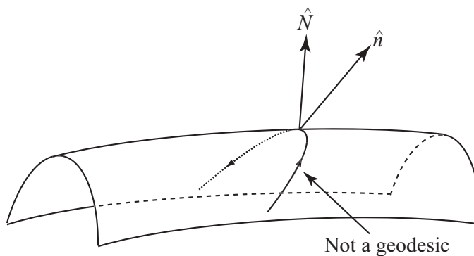
Figure 5.3. A curve along a surface, but not a geodesic surface ray.
