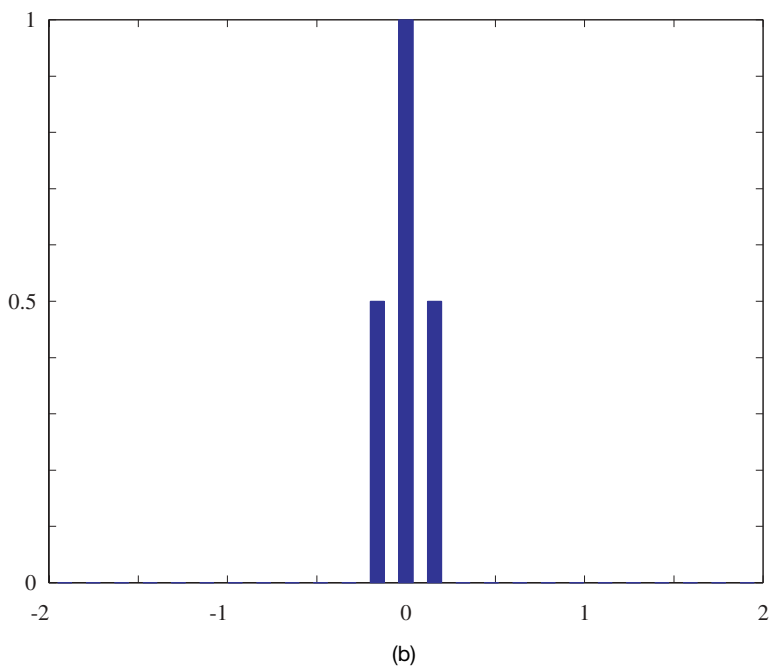
Figure 2.14. Typical element patterns in the Fourier domain: (a) isotropic, and (b) (1 + \cos \phi) . (continued)
