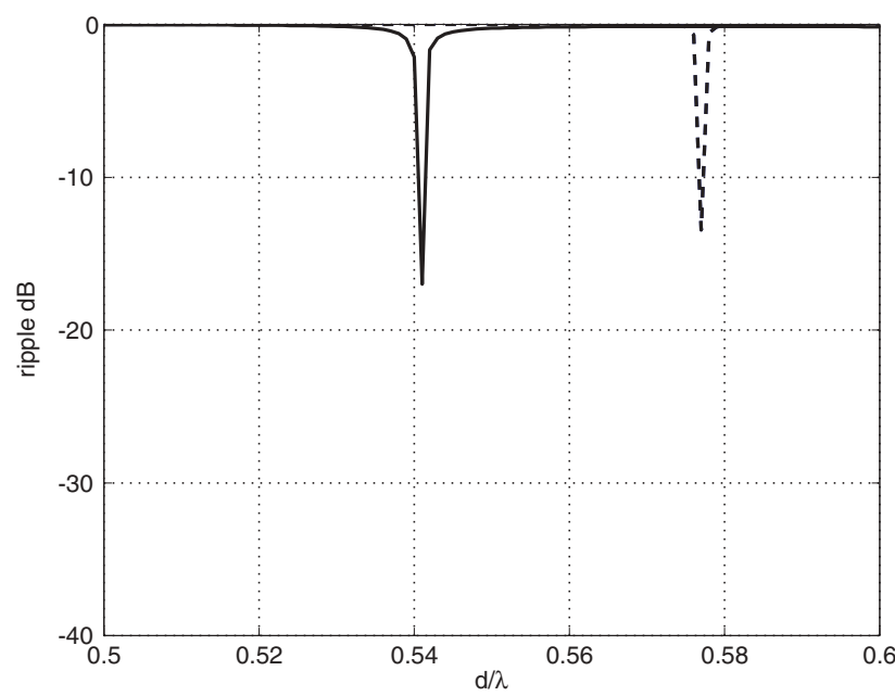
Figure 2.18. Ripple resonance effect with 15 (dashed line) and 16 elements (solid line). Isotropic radiators.
