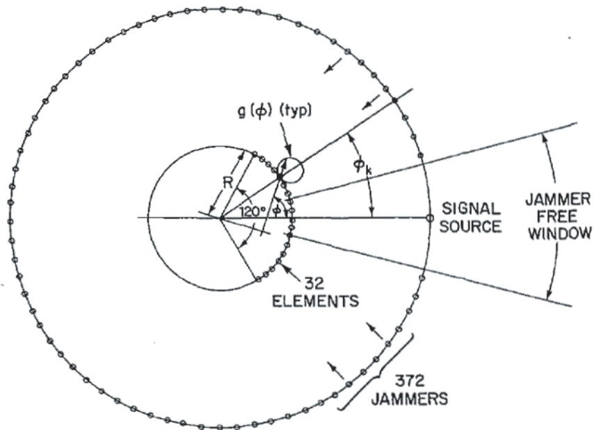
Figure 10.8. A jamming scenario according to [Sureau and Keeping 1982] for low sidelobe synthesis.
