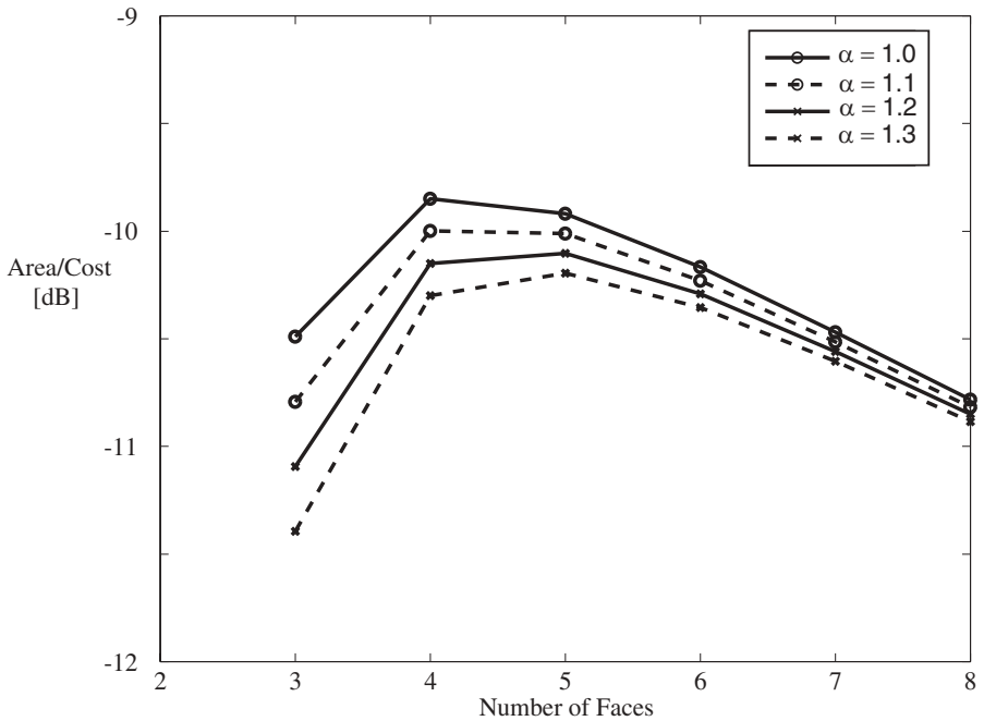
Figure 3.5. Normalized performance (effective area/cost) versus number of antenna faces for omnidirectional coverage (360°).
