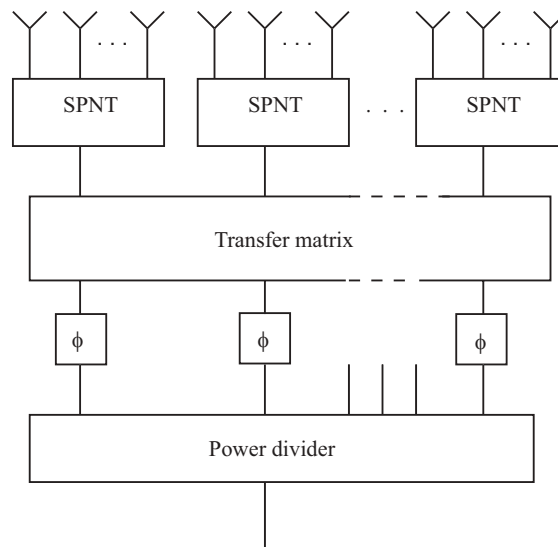
Figure 9.3. A switch matrix feed with phase shifters for fine steering of the beam.
