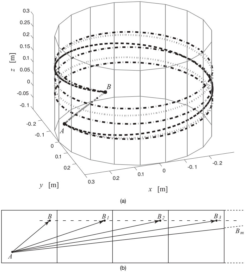
Figure 5.7. Illustration of different higher-order geodesics in one direction connecting A and B . (a) The closed circular cylinder. (b) The developed circular cylinder.
