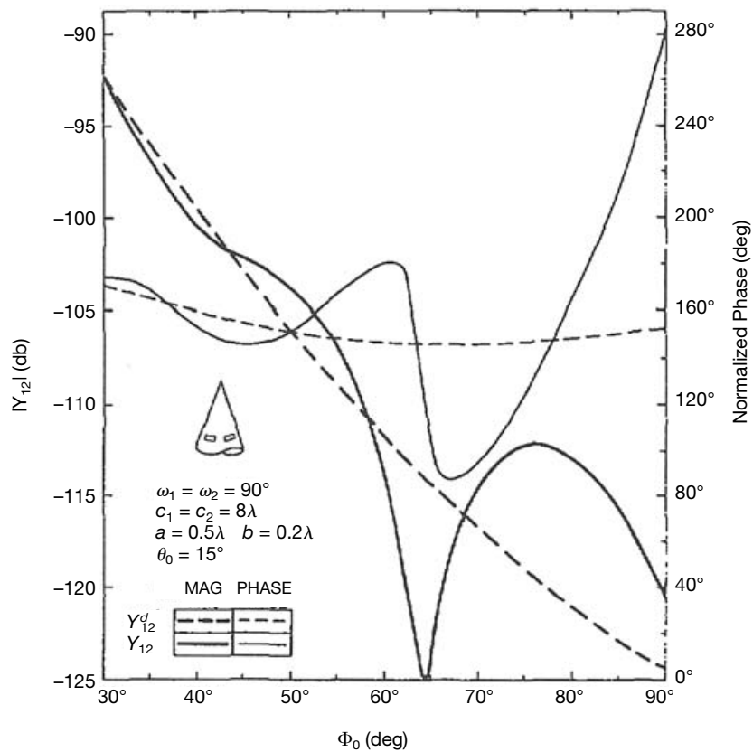
Figure 6.73. Mutual admittance between two circumferential slots on a cone at the same altitude versus the angular separation [Lee 1978].
