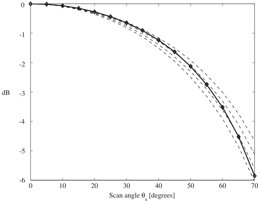
Figure 3.3. Total scan loss. Current sheet model (with diamonds) compared to the (\cos \theta_s)^\alpha model, with \alpha = 1.0, 1.1, 1.2 , and 1.3 (dashed curves, top to bottom).
