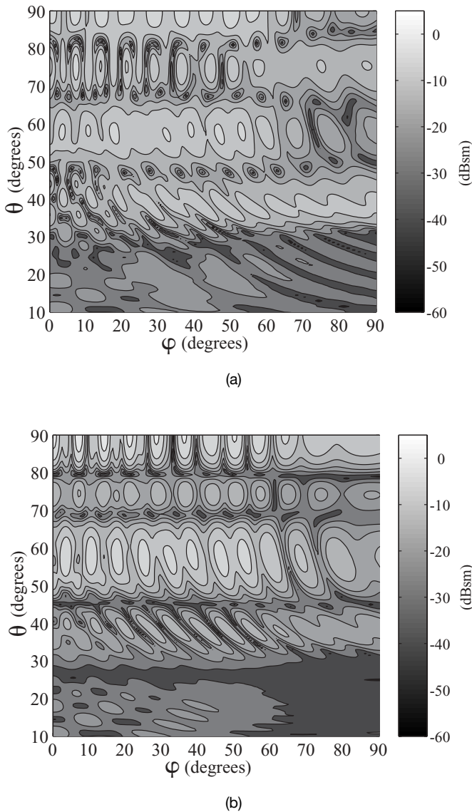
Figure 11.15. \sigma_{\text{TETE}} at 6.8 GHz with 15 modes. (a) Triangular grid. (b) Rectangular grid.
