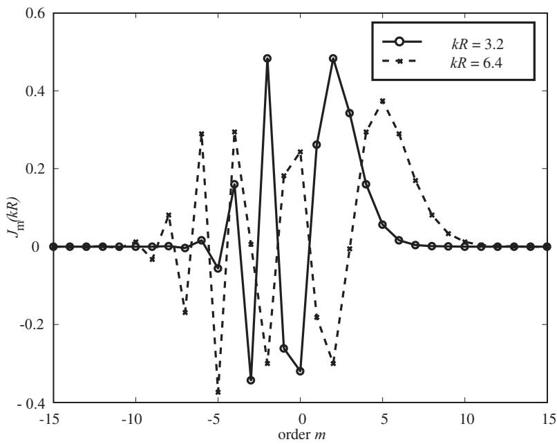
Figure 2.11. Variation of J_m(kR) versus mode number for two values of kR .
