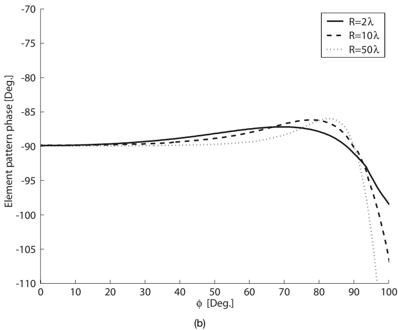
Figure 6.18. The E -plane isolated-element pattern in the azimuth versus the radius of the cylinder. (a) Amplitude. The planar case is also included (circles). (b) Phase.
