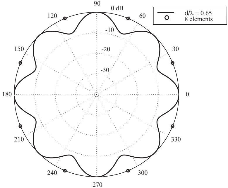
Figure 2.7. Radiation pattern with eight isotropic elements spaced at 0.65 wavelengths. Uniform excitation.
