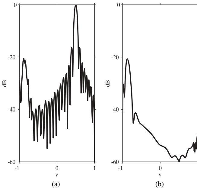
Figure 8.40. The E_\theta (a) and E_\phi (b) components in a cut through the pattern for u = 0 in Figure 8.39.
