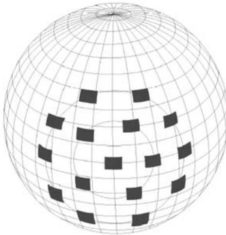
Figure 8.53. 16 patch elements on a sphere [Sipus et al. 2003]. Copyright 2003 Wiley Periodicals, Inc. Reproduced by permission of John Wiley & Sons, Inc.
