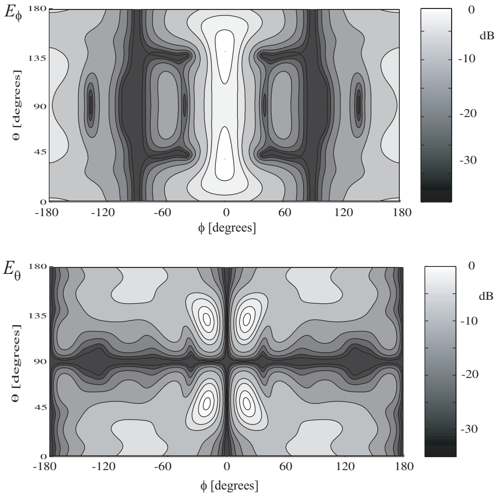
Figure 8.30. Co- and cross-polarization patterns for a focused dipole ring array.
