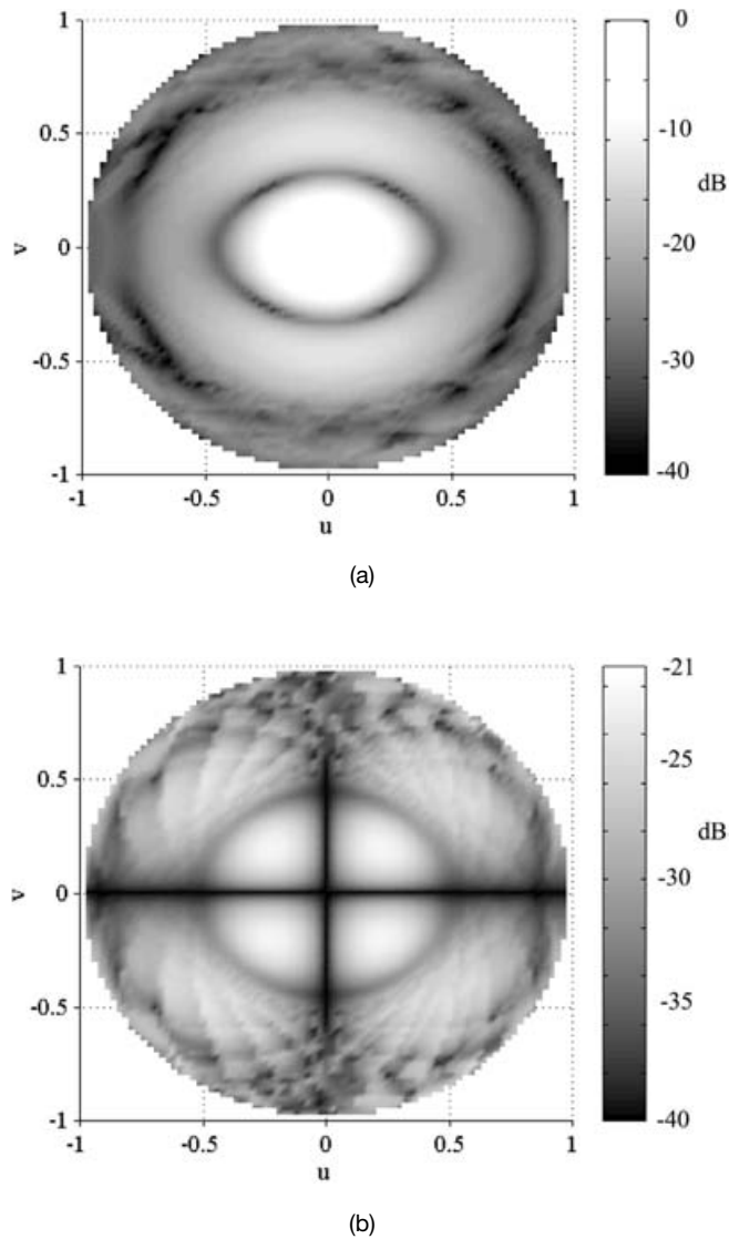
Figure 8.41. Patterns in the (u, v) plane for h/D = 0.5 . (a): the E_\theta component (co-polar), (b): the E_\phi component (cross-polar).
