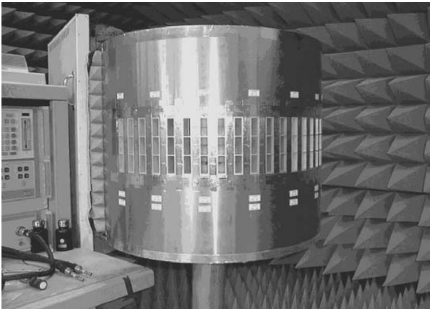
Figure 6.12. The experimental antenna. Courtesy of Ericsson Microwave Systems AB, Göteborg, Sweden. See also color insert, Figure 2.
