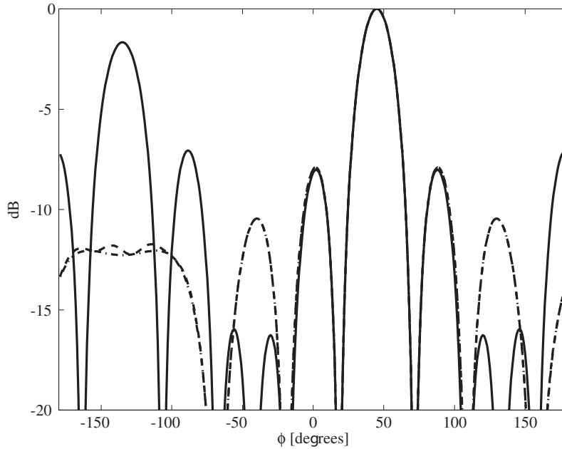
Figure 2.27. Patterns focused in the 45^\circ direction with a kR = 5.2 array. Eight elements (solid line), 13 elements (dashed line), and Bessel pattern (dash-dotted line).
