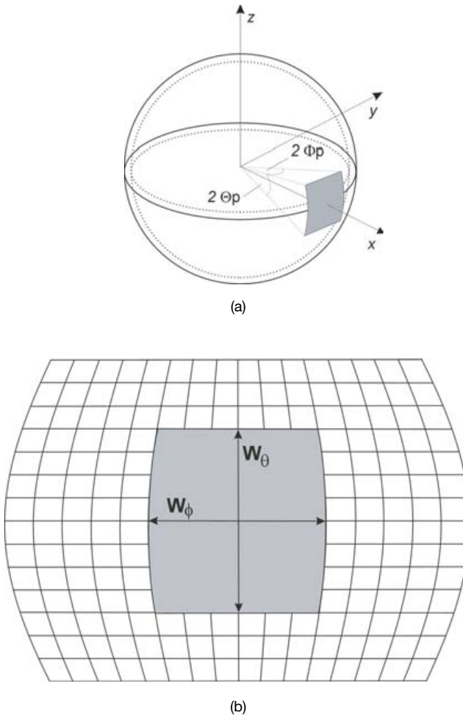
Figure 7.26. Geometry of the problem. (a) Rectangular patch on a spherical structure. (b) Azimuthal equatorial projection [Sipus et al. 2003a]. Copyright (2003) Wiley Periodicals, Inc. Reprinted by permission of John Wiley & Sons, Inc.
