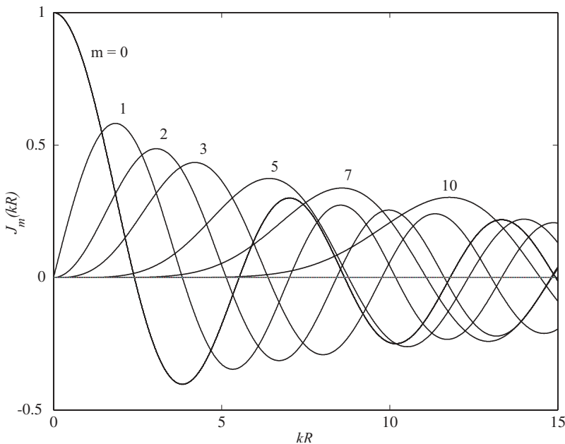
Figure 2.9. Bessel functions of first degree and orders from 1 to 10.
