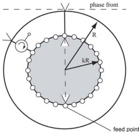
Figure 9.10. The R - kR lens, here with circulators.
