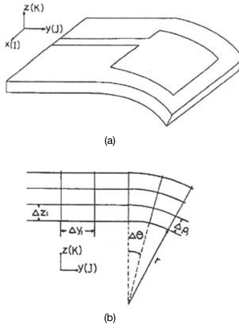
Figure 4.7. Typical grid when using FDTD in curvilinear coordinates [Kashiwa et al. 1994]. (a) Rectangular microstrip antenna on curved substrate. (b) Mesh configuration on yz cross section.
