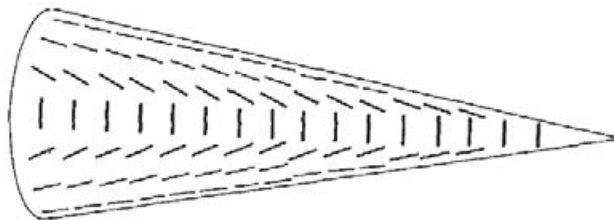
Figure 8.26. A conical array with slot elements oriented for correct linear polarization in the axial direction [Kummer 1974].
