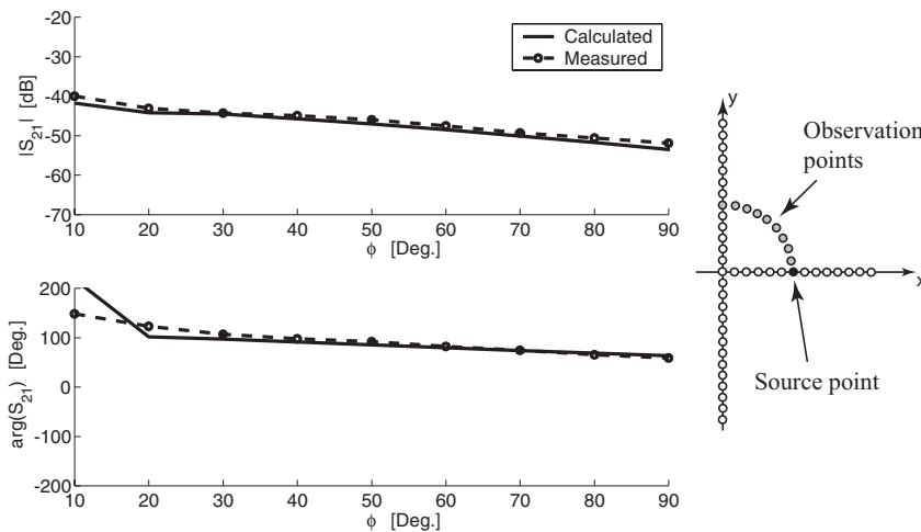
Figure 7.9. Isolated coupling along the circle arc, [\phi, R] polarization. The source point is element +x_6 . Solid line: calculated; dashed line: measured.
