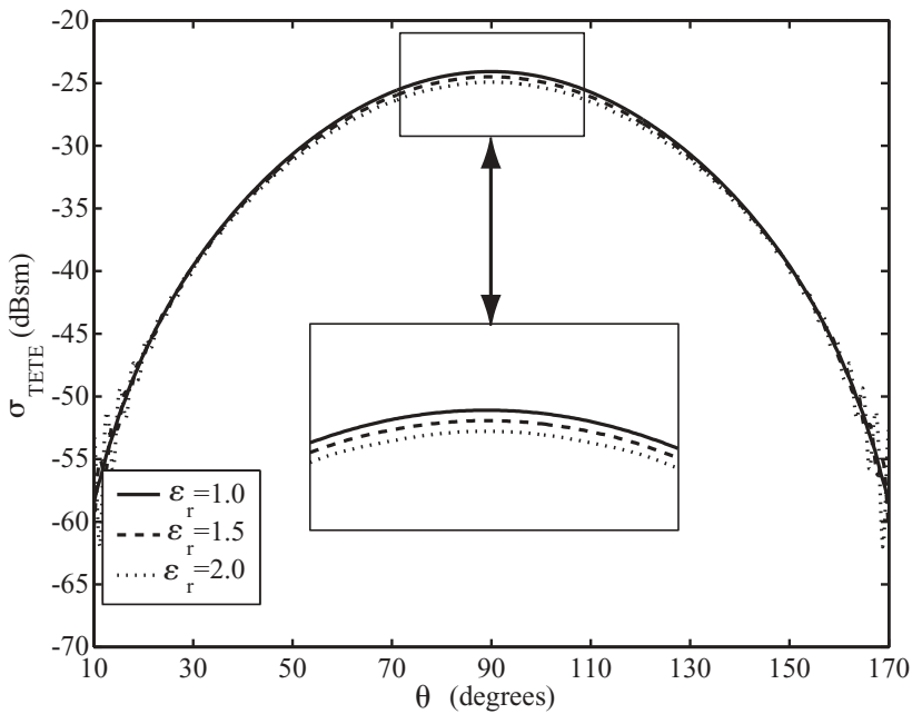
Figure 11.18. The H -plane RCS at 4.3 GHz for a single waveguide element on a cylinder with different dielectric coatings.
