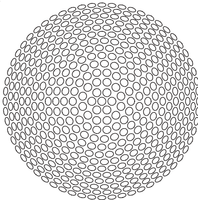
Figure 8.33. Element layout with about 500 radiators.
