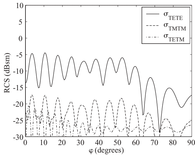
Figure 11.12. The level of cross-polarization \sigma_{TETM} (dash-dotted line) compared to the co-polarized cases \sigma_{TETE} (solid line) and \sigma_{TMTM} (dashed line). 6.8 GHz, 15 modes, and \theta = 60^\circ .
