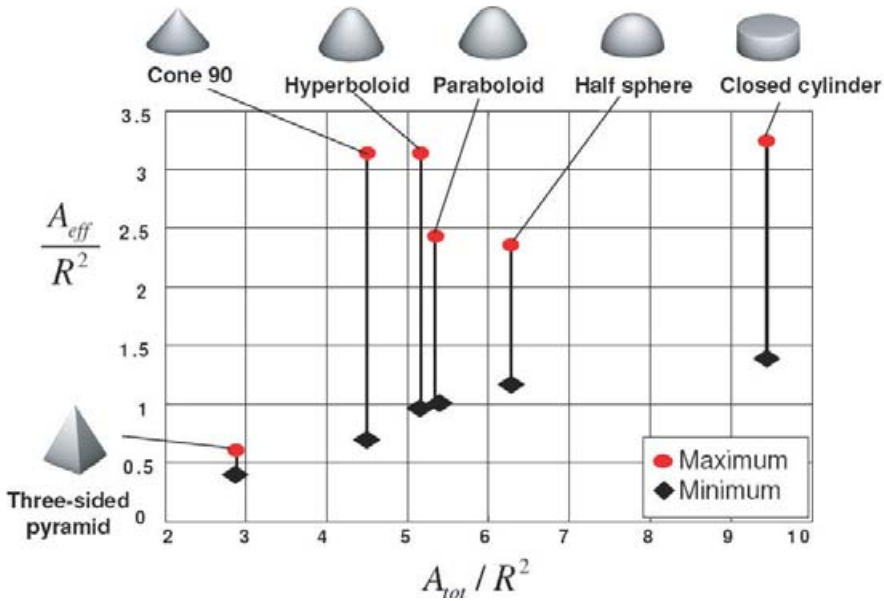
Figure 3.21. Maximum and minimum values of the effective antenna area versus the total antenna area for several conformal antenna shapes.
