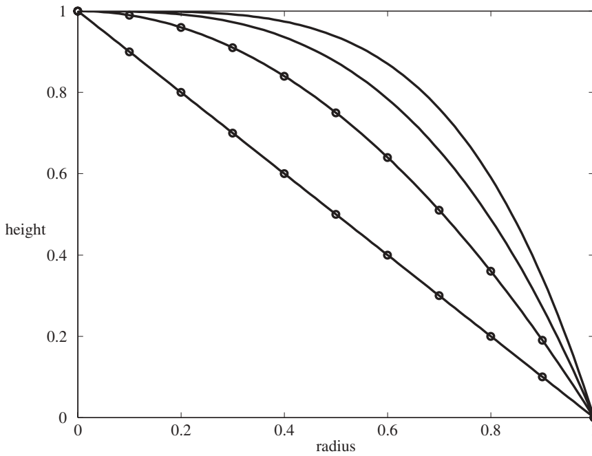
Figure 3.18. Paraboloidal shapes with \varepsilon = 0.5 (cone), 1.0 (paraboloid), 1.5, and 2 (paraboloid-type). The cone and the paraboloid are indicated by circles.
