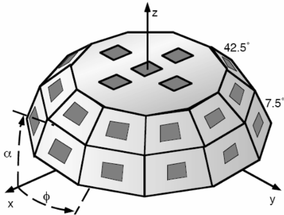
Figure 3.24. A multisurface solution approximating a half sphere [Wiesbeck et al. 2002].
