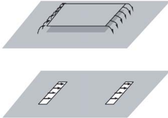
Figure 8.19. Equivalent slot model for a patch antenna.
