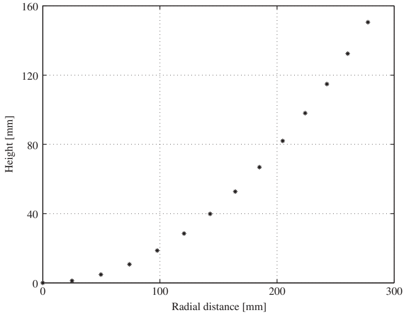
Figure 8.34. Elements evenly spaced along a parabola.
