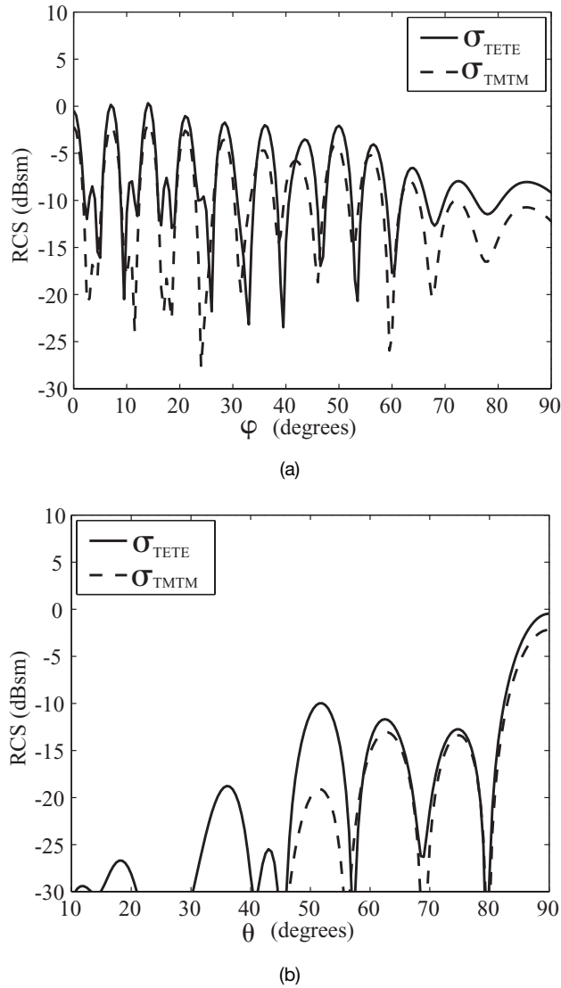
Figure 11.8. Calculated results for \sigma_{TETE} (solid line) and \sigma_{TMTM} (dashed line) with three waveguide modes at 6.8 GHz. (a) E plane. (b) H plane.
