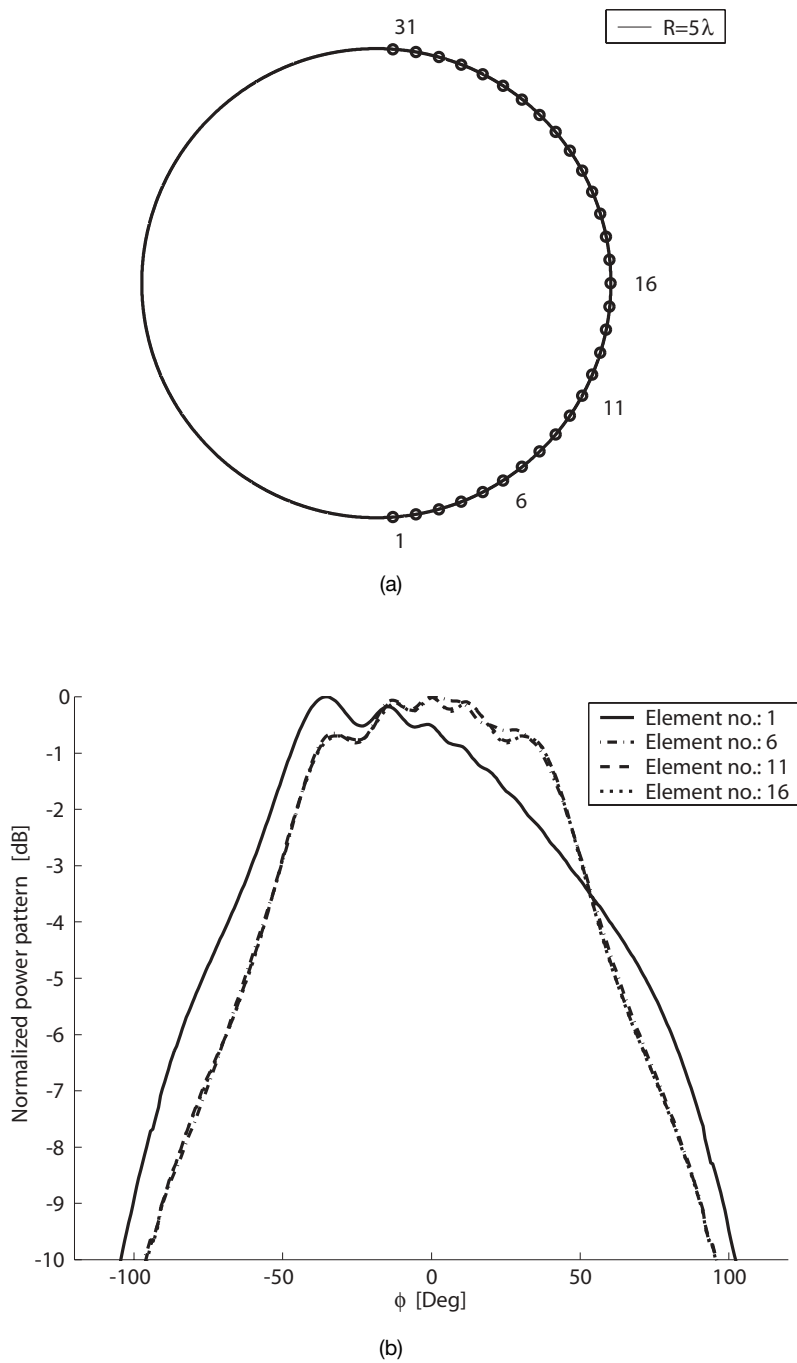
Figure 6.38. Embedded-element patterns in the E plane due to apertures in a sector array containing 31 elements, circular cylinder ( R = 5 \lambda ). The element-to-element distance equals 0.5 \lambda . \phi is a relative angle and equals zero at the element position. (a) The geometry. (b) The results.
