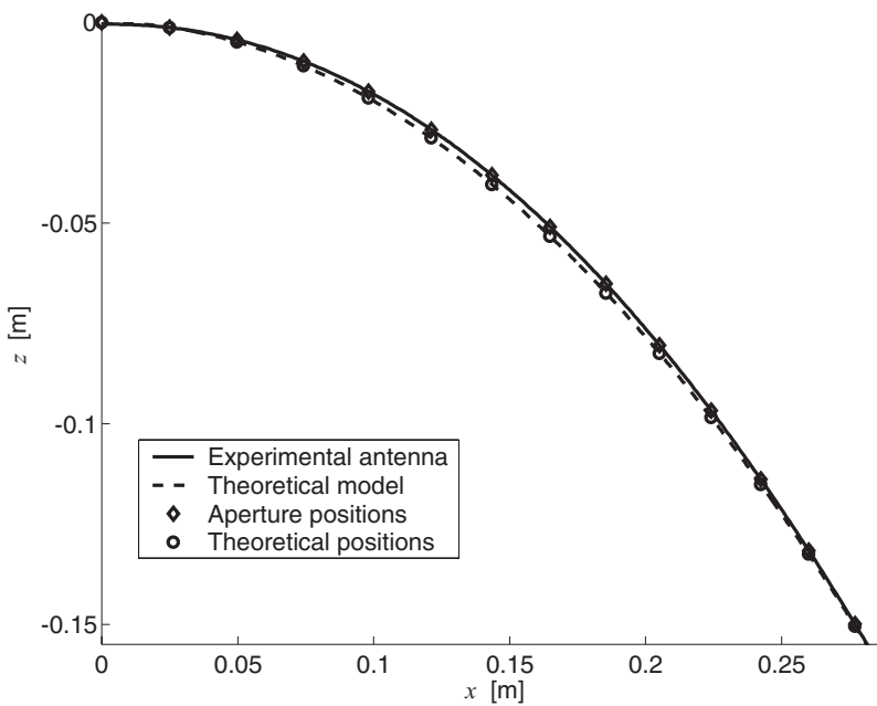
Figure 7.18. A comparison between the theoretical model of the antenna and the experimental antenna itself.
