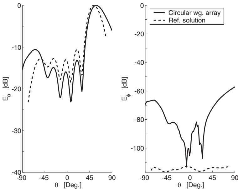
Figure 8.56. The E_\theta and E_\phi components in the symmetry plane with the beam scanned 60^\circ from the zenith direction. Dashed line: idealized dipole element patterns. Solid line: TE_{11} mode circular aperture elements [Persson and Josefsson 2003].
