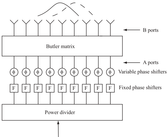
Figure 9.6. Commutating by means of a Butler matrix. The active output is shifted by means of the variable phase shifters.
