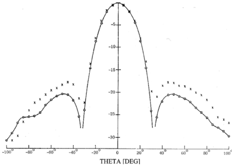
Figure 8.51. Radiation pattern in two orthogonal cuts (solid line and crosses) for an array with 31 uniformly excited elements on a spherical surface with a 90° active region [Sengupta et al. 1968].
