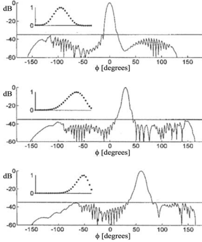
Figure 8.18. Patterns with amplitude weightings (see inserts) for a circular arc array when scanned at 0°, 30°, and 60° scan angles, respectively (top to bottom). After [Boeringer and Werner 2004].
