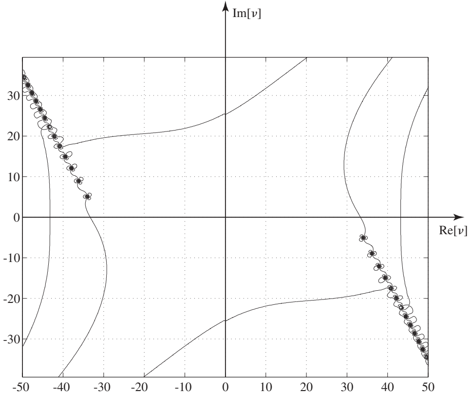
Figure 4A.2. The real part of one component of the Green's function for a coated PEC cylinder with some pole locations shown in the complex \nu plane. Here, k_z is real.
