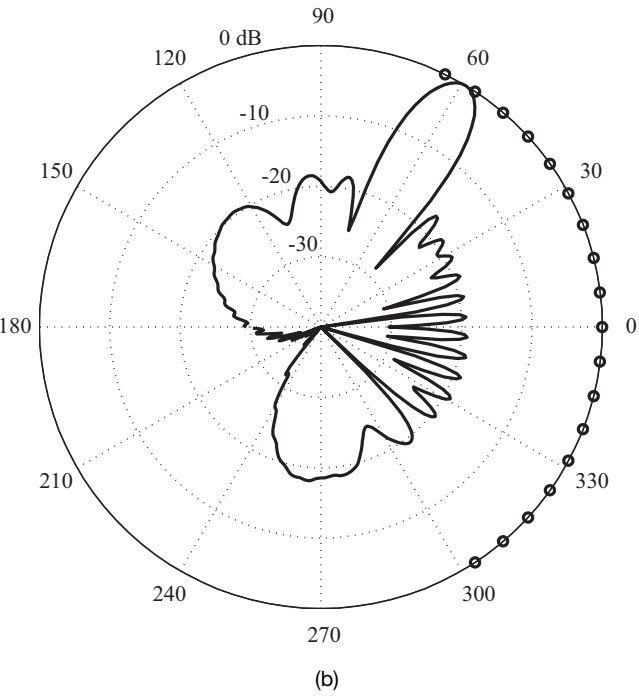
Figure 8.16. Phase scanning with optimized element amplitudes. Same array as in Figure 8.15 [Josefsson and Persson 1999a]. (a) 30°, (b) 60°, and (c) 90° scan angles. (continued)
