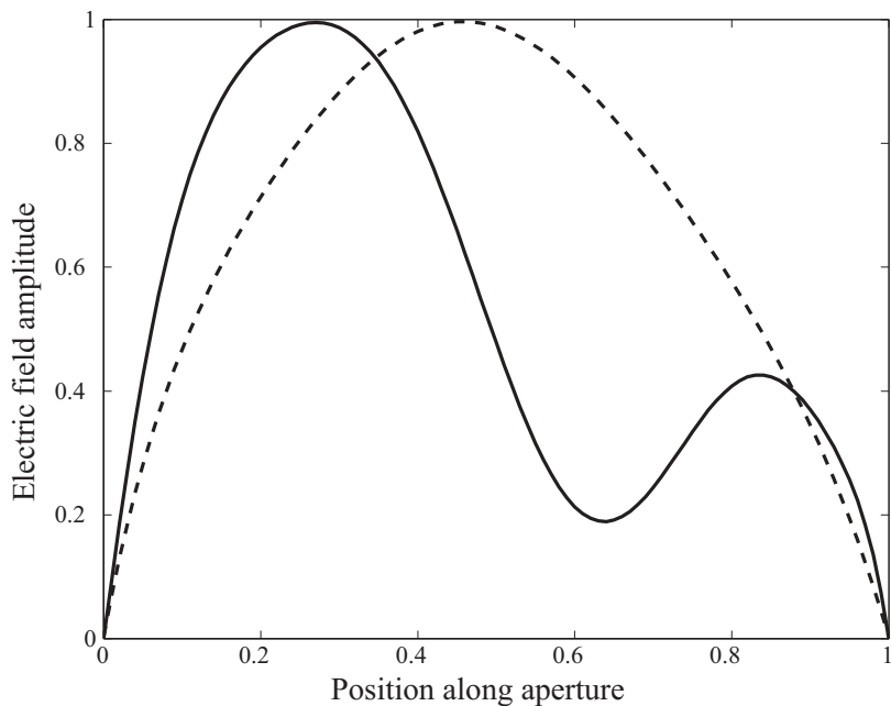
Figure 11.34. The electric field distribution along a narrow aperture (slot) illuminated at \theta = 60^\circ from normal incidence ( H plane). Dashed line is near resonance (9.375 GHz) and solid line at 14 GHz. From [Josefsson 1990].
