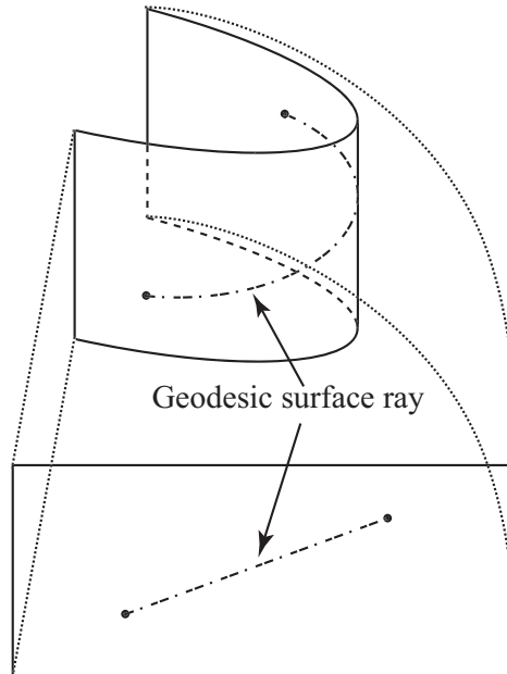
Figure 5.4. A developed cylindrical surface.
