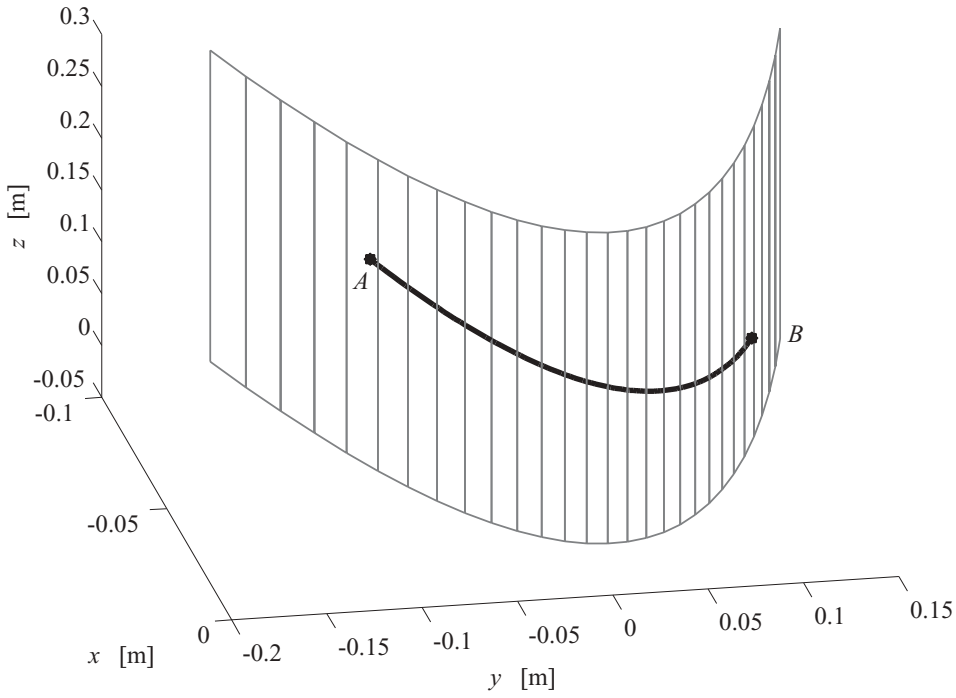
Figure 5.5. The geodesic connecting A and B on a parabolic cylinder. Here, a = 0.5 , \alpha = -0.414 , and \beta = 0.13 .
