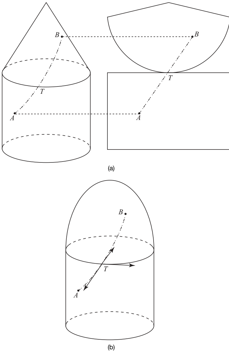
Figure 5.18. (a) One example of a hybrid surface, here a circular cylinder fitted with a circular cone. (b) A hybrid surface in which a circular cylinder and a general paraboloid of revolution (GPOR) are combined.
