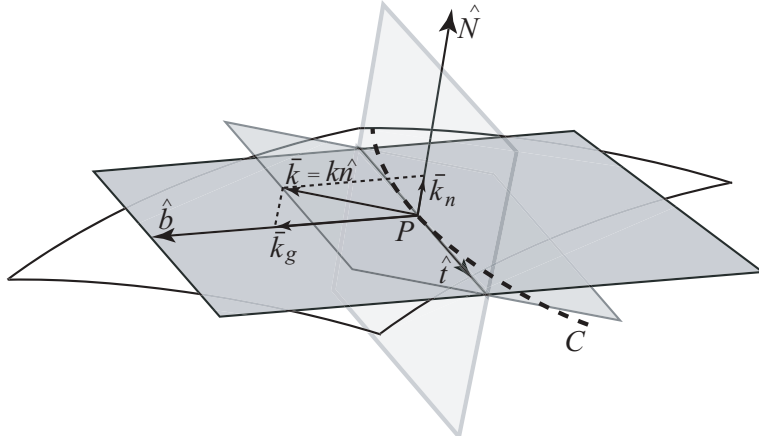
Figure 5.2. An arc C passing through a point P with the curvature vector \bar{k} and unit tangential vector \hat{t} shown.
