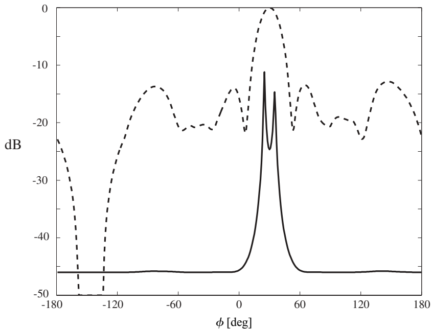
Figure 9.24. The MUSIC spectrum (solid line) with sources at 25^\circ and 35^\circ . The dashed line is the regular antenna pattern with the main beam pointing between the two sources.
