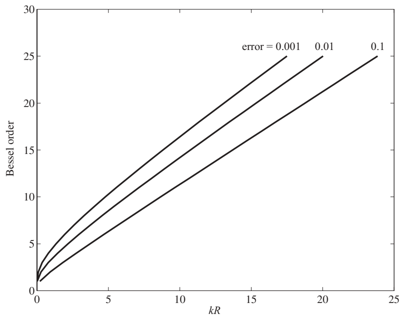
Figure 2.10. The required Bessel function order (required mode number) for given error limits.
