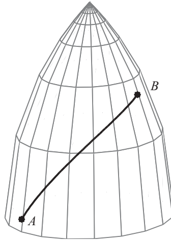
Figure 5.10. A solution to the geodesic equation for an ogive with R = 0.5 and a = 3\pi/4 . Here \alpha = 0.1329 and \beta = -6.7907^\circ .
