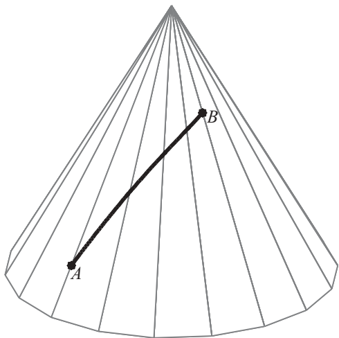
Figure 5.8. A solution to the geodesic equation for a cone with \theta_0 = 30^\circ . Here \alpha = -0.0869 and \beta = -221^\circ .
