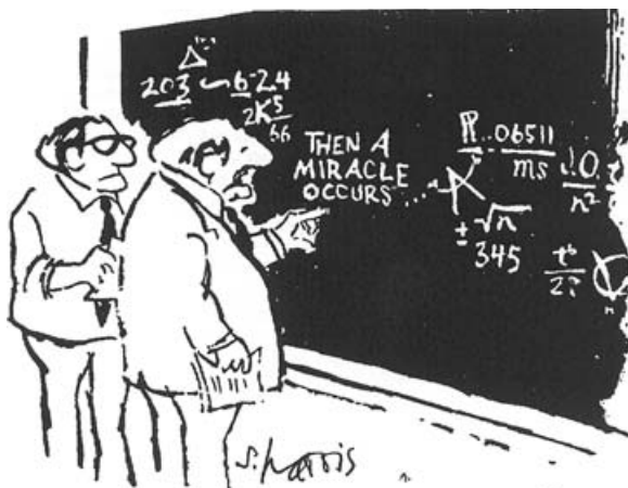
Figure 4A.3. The development of UTD for a general smooth convex surface? [Gordon 1985]
