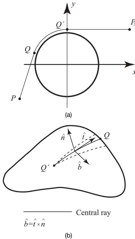
Figure 4.12. Ray surface diffraction on a convex surface. (a) Overview. (b) A surface ray strip connecting Q' and Q together with the surface ray coordinates at a point along the geodesic.
