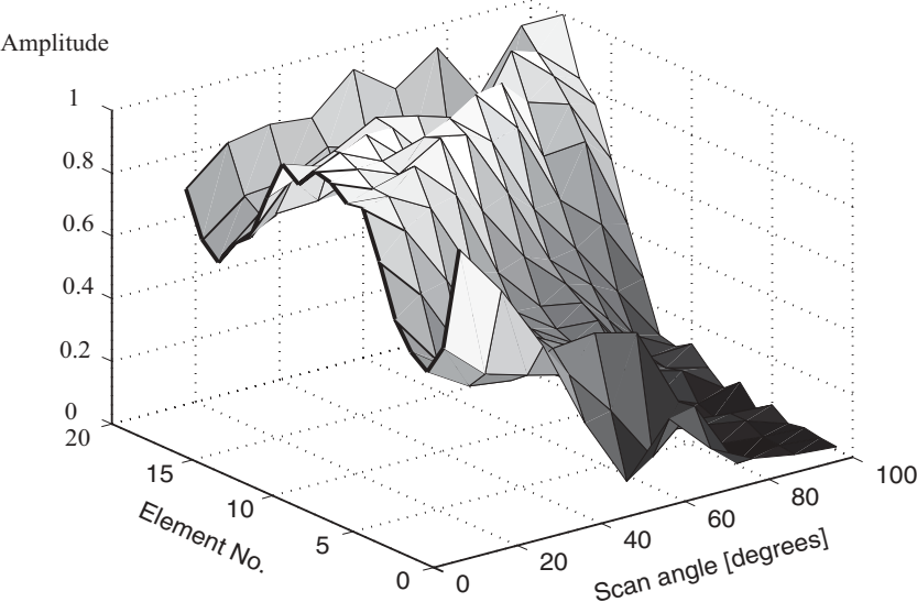
Figure 8.17. The variation of optimized amplitudes for a cylindrical array when the scan angle is changed.
