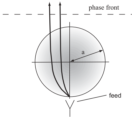
Figure 9.13. A Luneburg lens with radially varying refractive index.
