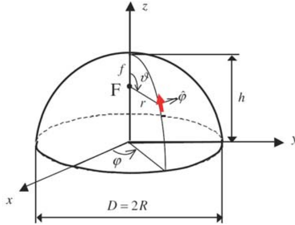
Figure 3.17. Polar coordinates with a radiating element indicated at position (r, \vartheta) .
