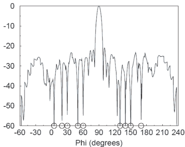
Figure 10.10. A -25 dB sidelobe pattern synthesized with the genetic algorithm method and nulls imposed by the adaptive array method [Virga and Zhang 2000].
