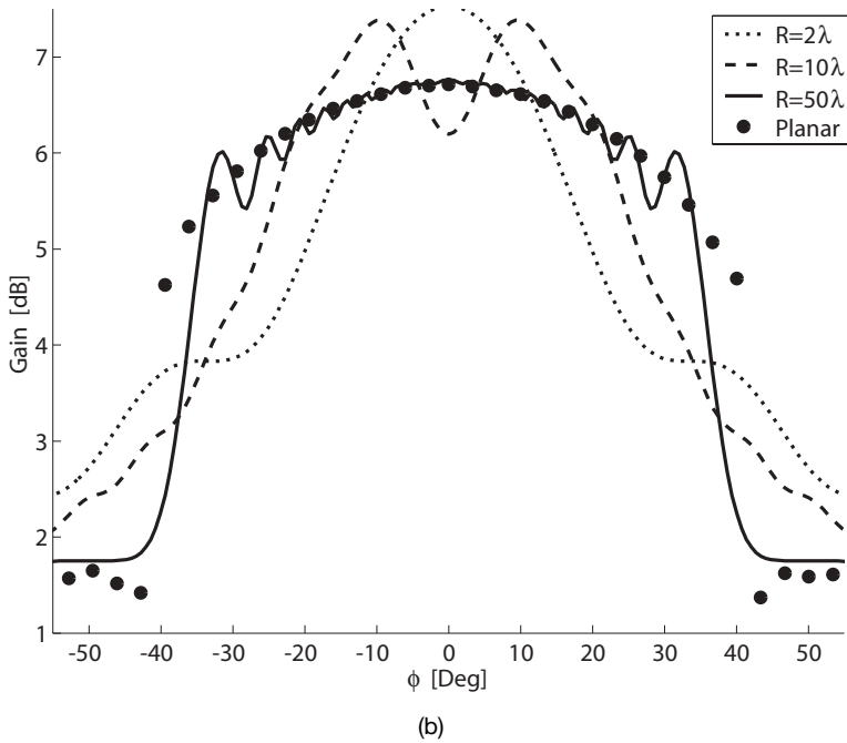
Figure 6.20. The gain of the E -plane embedded-element pattern for a single-ring array in the azimuth versus the radius of the cylinder for a fixed-element spacing ( d = 0.6 \lambda ). (a) Overview for R = 2\lambda , 10\lambda , and 50\lambda . (b) The corresponding planar case is also shown (dots) in a close-up view.
