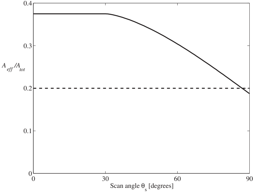
Figure 3.13. Hemisphere. Normalized performance (effective area/cost) versus scan angle from the zenith. The dashed line is for an extended sphere with constant effective area.
