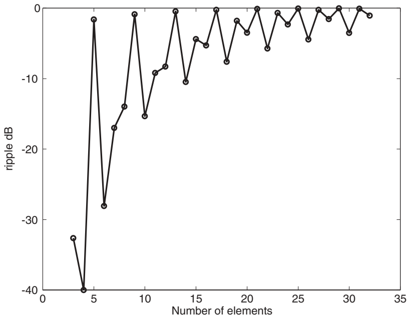
Figure 2.20. Omnidirectional pattern ripple as a function of the number of elements when d/\lambda = 0.8 .
