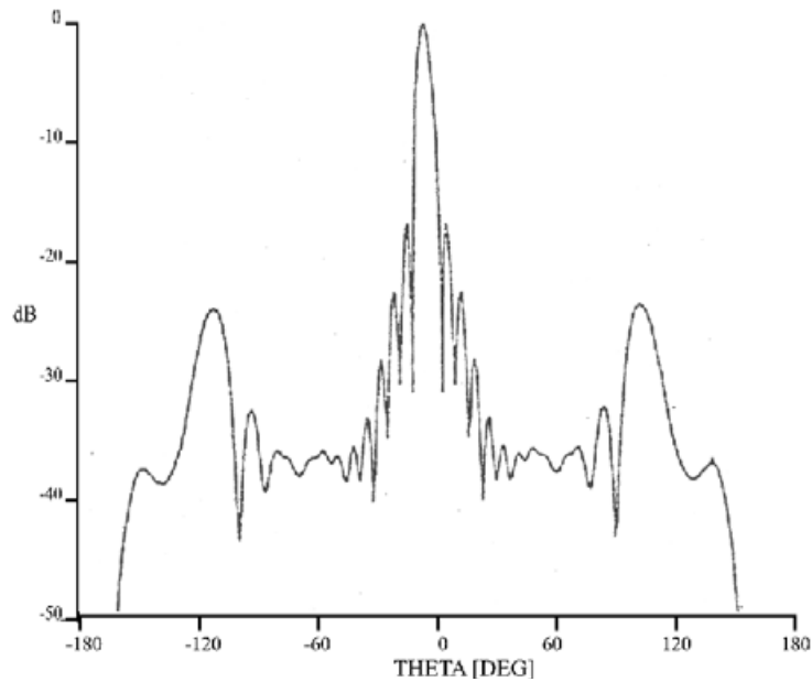
Figure 8.52. Pattern for a spherical array with 316 elements spaced 0.66 \lambda in a triangular lattice; from [Saito et al. 1987].
