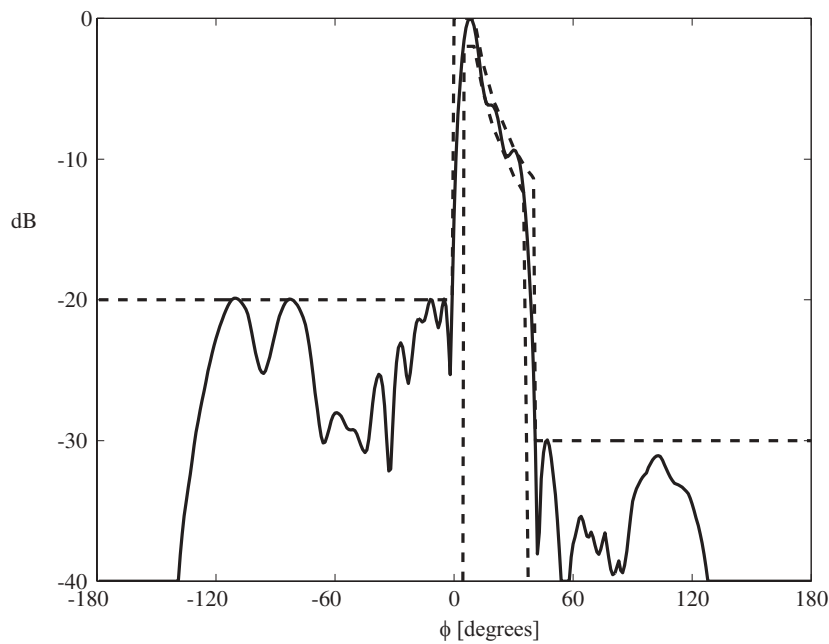
Figure 10.13. Synthesized pattern after 100 iterations.
