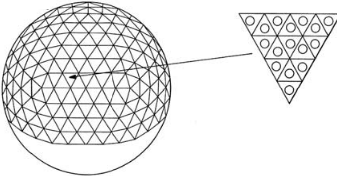
Figure 3.22. A spherical surface built from triangular planar facets [Bondyopadhyay 2002].
