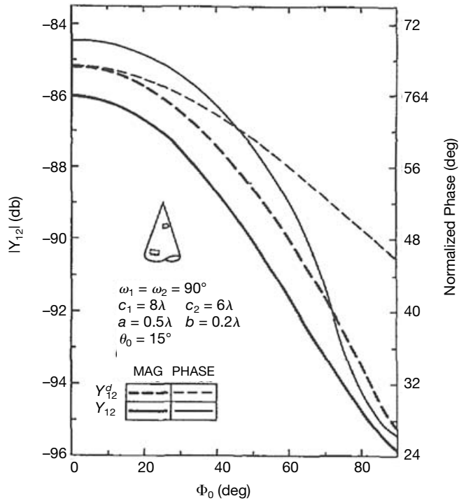
Figure 6.75. Mutual admittance between two circumferential slots on a cone versus the angular separation when separated by a large radial distance [Lee 1978].
