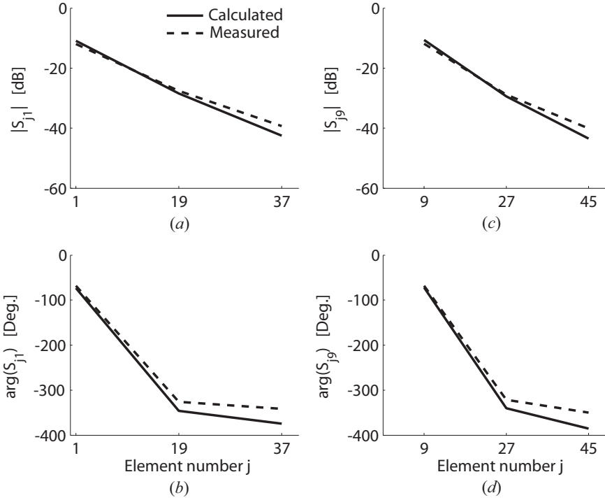
Figure 6.16. The array mutual coupling in the H plane for an edge column and for the center column. Single-mode approximation, f = 5.65 GHz. Solid line: calculated, dashed line: measured. (a) Amplitude, edge column. (b) Phase, edge column. (c) Amplitude, center column. (d) Phase, center column.
