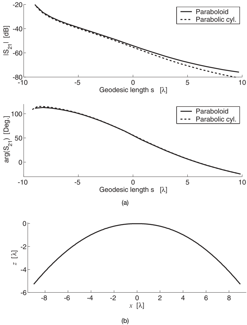
Figure 7.4. The same case as in Figure 7.2 ( [R, R] polarization, solid line) compared with the results obtained using a parabolic cylinder (dashed line) with the same cross section as the paraboloid. (a) Amplitude and phase. (b) The cross section (cf. Figure 7.1).
