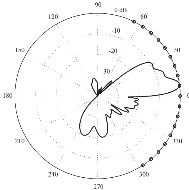
Figure 10.14. Synthesized pattern with coupling, also showing element locations.
