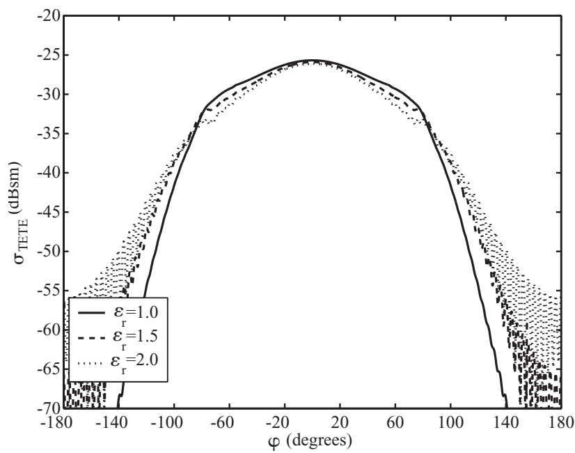
Figure 11.19. The E -plane RCS at 6.8 GHz for a single waveguide element on a cylinder with different dielectric coatings.
