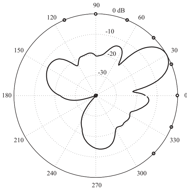
Figure 8.10. As for Figure 8.9, but with rear-side elements not excited.
