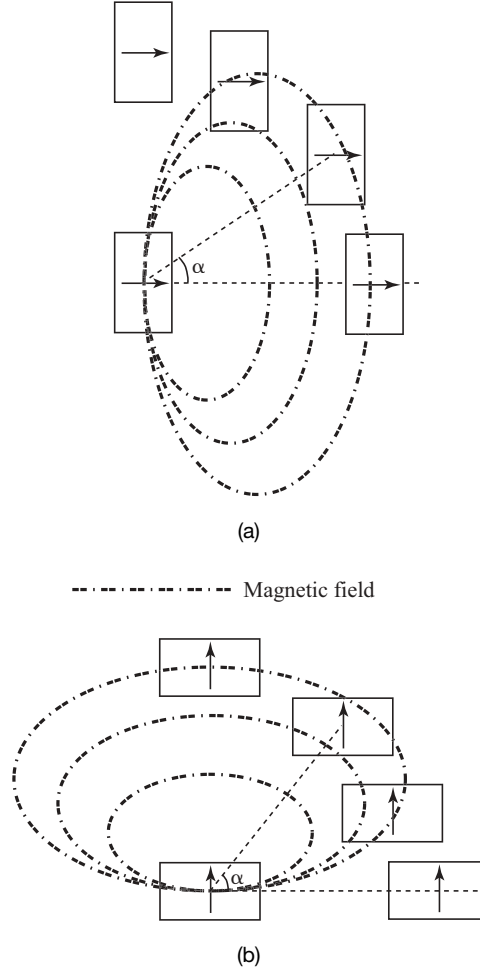
Figure 6.8. A two-dimensional sketch of the planar magnetic field of the source element and its interaction with another aperture. (a) E -plane type coupling along the horizontal line. (b) H -plane type coupling along the horizontal line.
