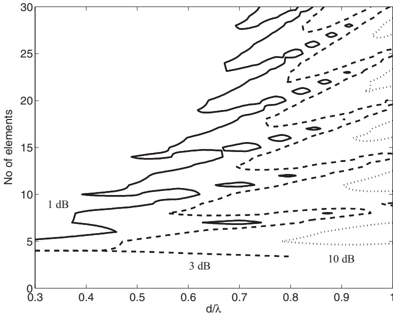
Figure 2.23. Ripple amplitude contour lines (1 dB solid, 3 dB dashed, and 10 dB dotted) for ring arrays with m = 0 mode excitation and \cos \phi element patterns.
