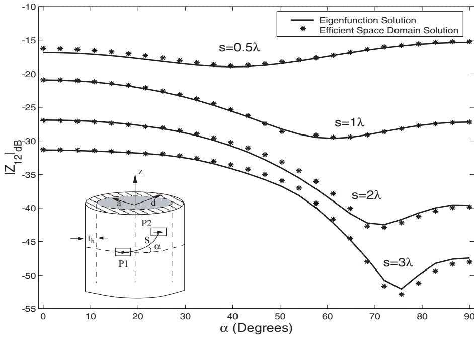
Figure 6.63. The mutual impedance Z_{12} between two \varphi -directed current modes for a coated cylinder with R = 3\lambda_0 , t = 0.06\lambda_0 , and \epsilon_r = 3.25 [Ertürk 2000]. a = R and d = R + t .
