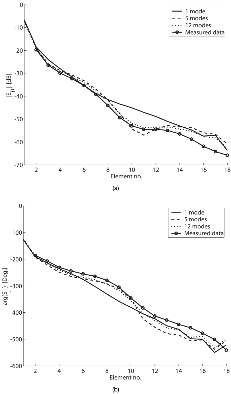
Figure 6.52. The array mutual coupling ( E plane) for an array of apertures with a lossy dielectric coating. The calculations were made using 1, 5, and 12 modes, including a small air gap (0.85 mm) between the PEC cylinder and the coating. The result is compared with the measured results (line with circles). (a) Amplitude. (b) Phase.
