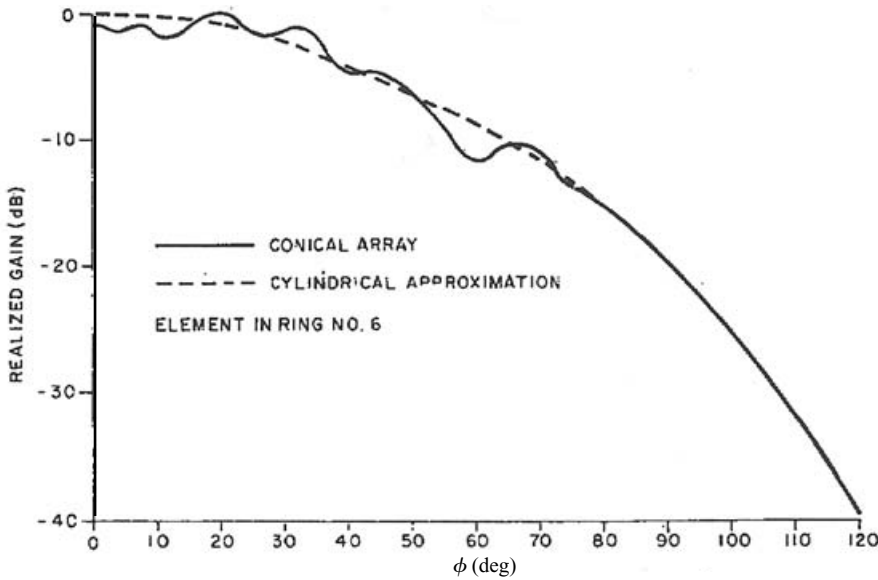
Figure 6.83. Circumferential element pattern ( H plane) compared with the pattern of an equivalent cylinder array [Balzano and Dowling 1974].
