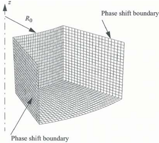
Figure 4.9. Schematic three-dimensional view of a sector computational volume when using cylindrical FDTD [Martin et al. 2003a].
