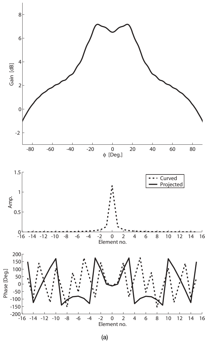
Figure 6.22. A study of the dependence of the element spacing for a single-row array located at a circular cylinder with a 6\lambda radius. (a) E -plane gain and element excitation for a 0.6\lambda element-to-element distance. (continued)
