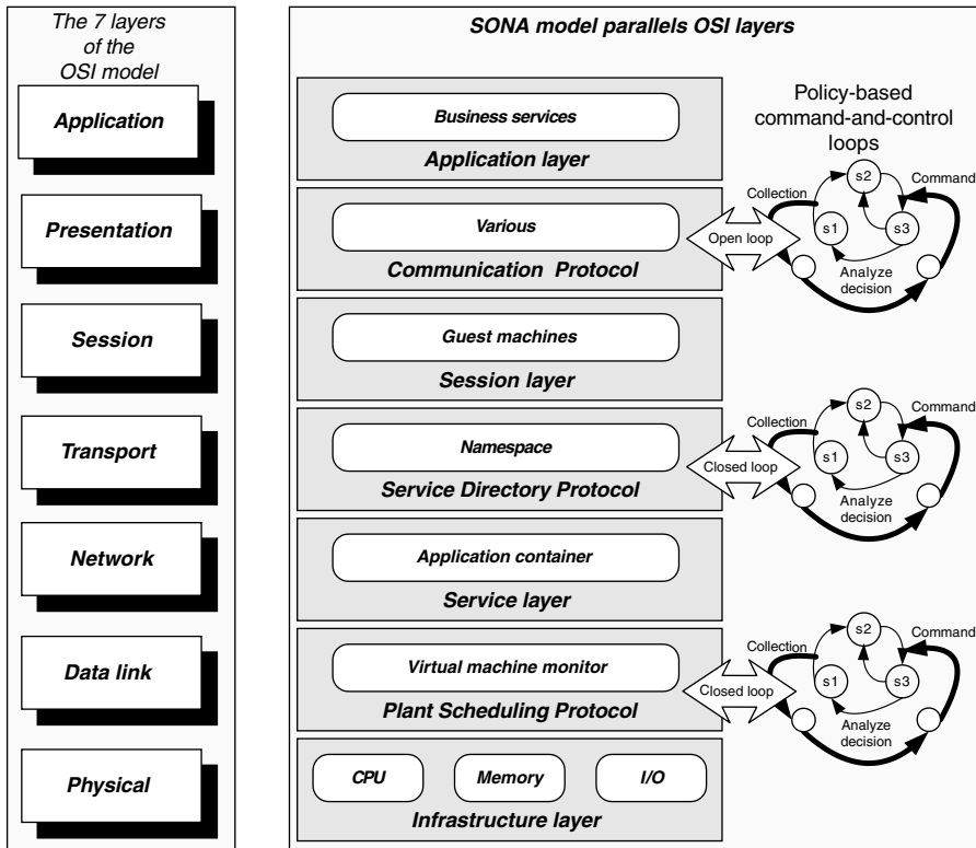
Figure 18.5. SONA layers parallel the OSI seven-layer model.
