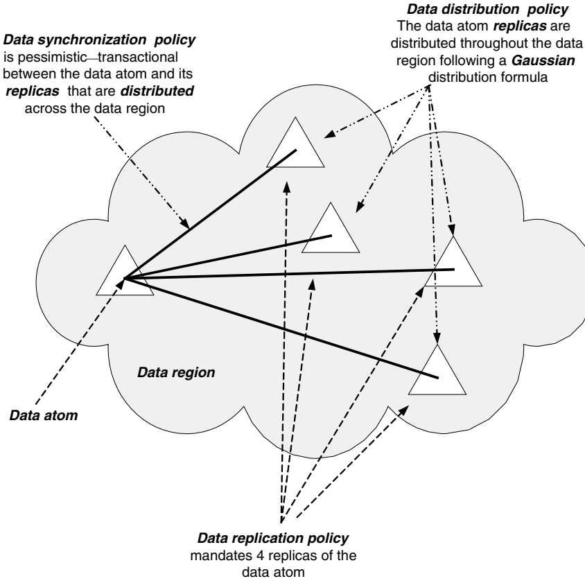
Figure 9.3. Relationship between data replication, distribution, and synchronization policies.
