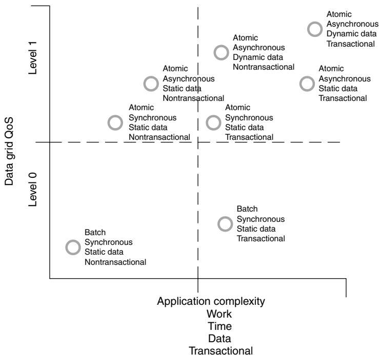
Figure 13.2. QoS-application requirement quadrant graph.
