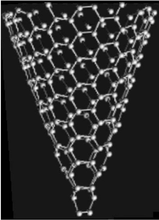
FIGURE 4.9 Nanocones (nanohorns).
