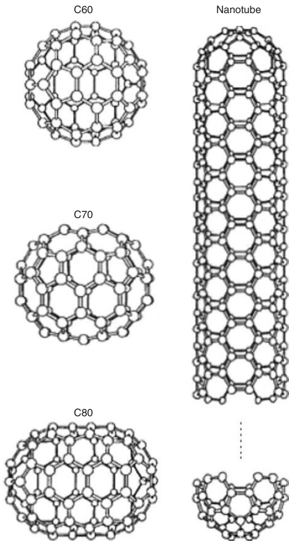
FIGURE 4.2 Fullerenes.
