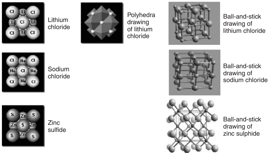
FIGURE 3.9 Two-atom geometries.
