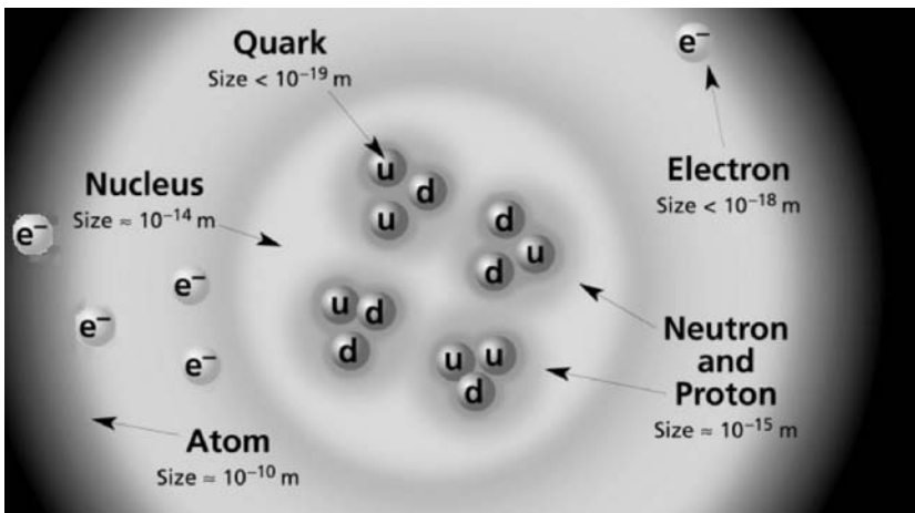
FIGURE 2.2 Another view of an atom.
