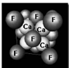
Fluorite ( \text{CaF}_2 )
