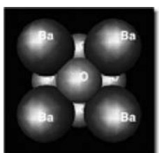
Perovskites ( \text{BaTiO}_3 )
