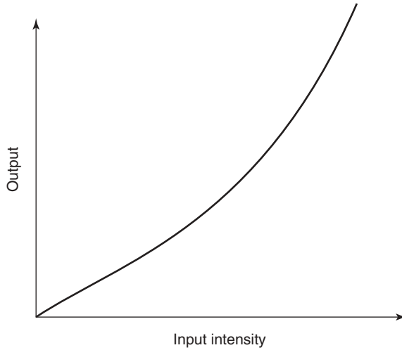
FIGURE 5.9 Nonlinearity.
