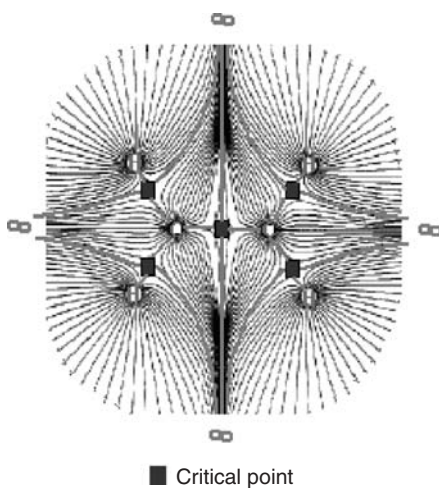
FIGURE D.5 Ethene ( \text{C}_2\text{H}_4 ) gradient trajectories that originate at critical points and terminate at the attractors and/or infinity.
