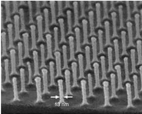
100-nm period posts in Si
