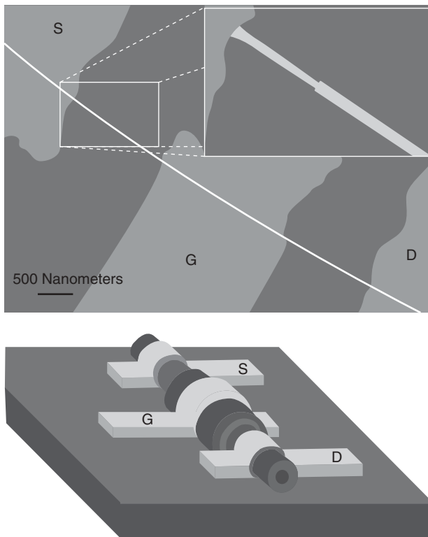
FIGURE 4.8 Use of nanowires in next-gen computer chips. This image and the diagram below it show a transistor made from a multilayer nanowire. The core of the nanowire is doped silicon and the first layer is germanium. The second layer is the insulator silicon oxide. The outer layer is doped germanium. S is the source electrode, G is the gate electrode, and D is the drain electrode. (Source: Lieber Group, Harvard University).
