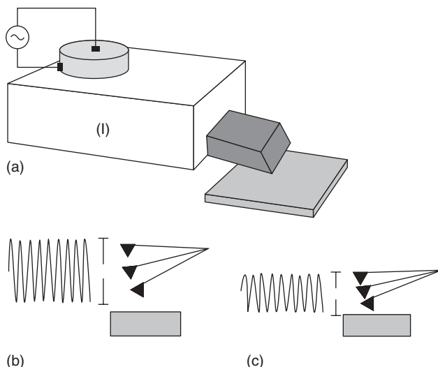
FIGURE F.5 Acoustic AC mode: (a) transducer attached to a cantilever housing is used to excite a cantilever into oscillation; (b) the amplitude of oscillation when the tip is far from the surface and; (c) reduced amplitude as the tip approaches the surface.
