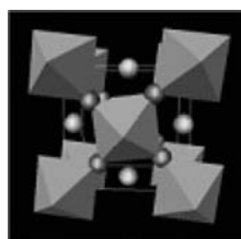
FIGURE 3.11 Ferroelectric types.
