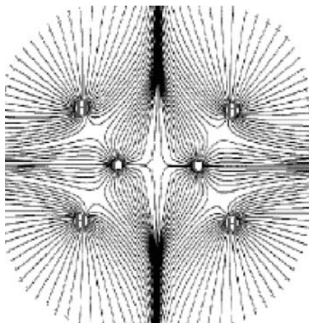
FIGURE D.3 Ethene ( \text{C}_2\text{H}_4 ) gradient trajectories that terminate at the nuclei of the carbon and hydrogen atoms.
