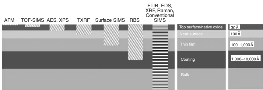
FIGURE F.2 Analysis depth. (Courtesy: Charles Evans & Associates).
