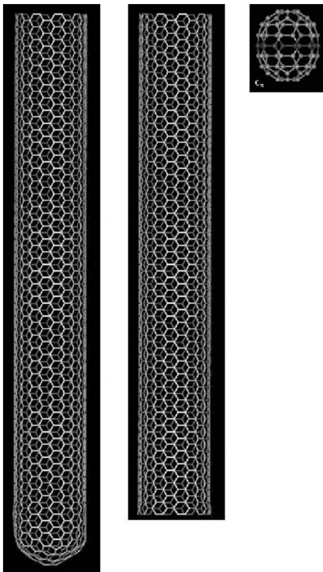
FIGURE 4.3 SWNT: (left) Section of a (10, 10) single-walled carbon nanotube with cap, (center) section of a (10, 10) single-walled carbon nanotube without cap, and (right) shortest nanotube. (Courtesy: Carbon Nanotechnologies Incorporated).
