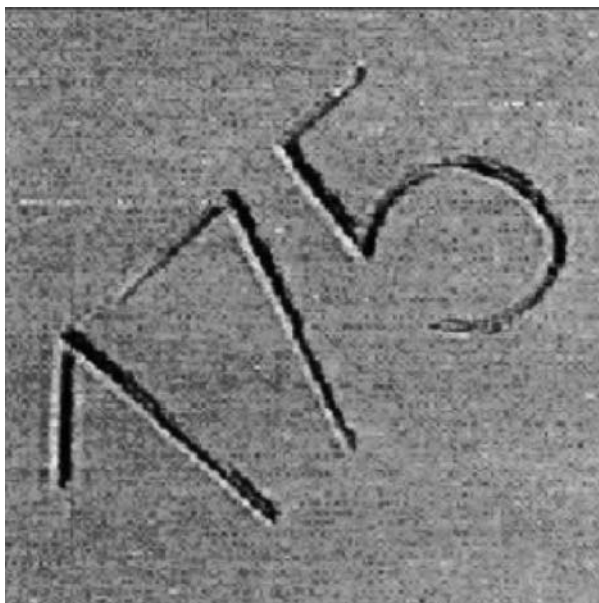
FIGURE F.8 Example of ATM usage: 9-nm lines in mica written with an AFM. (Courtesy: DFG-Center for Functional Nanostructures, Universität Karlsruhe, Germany).
