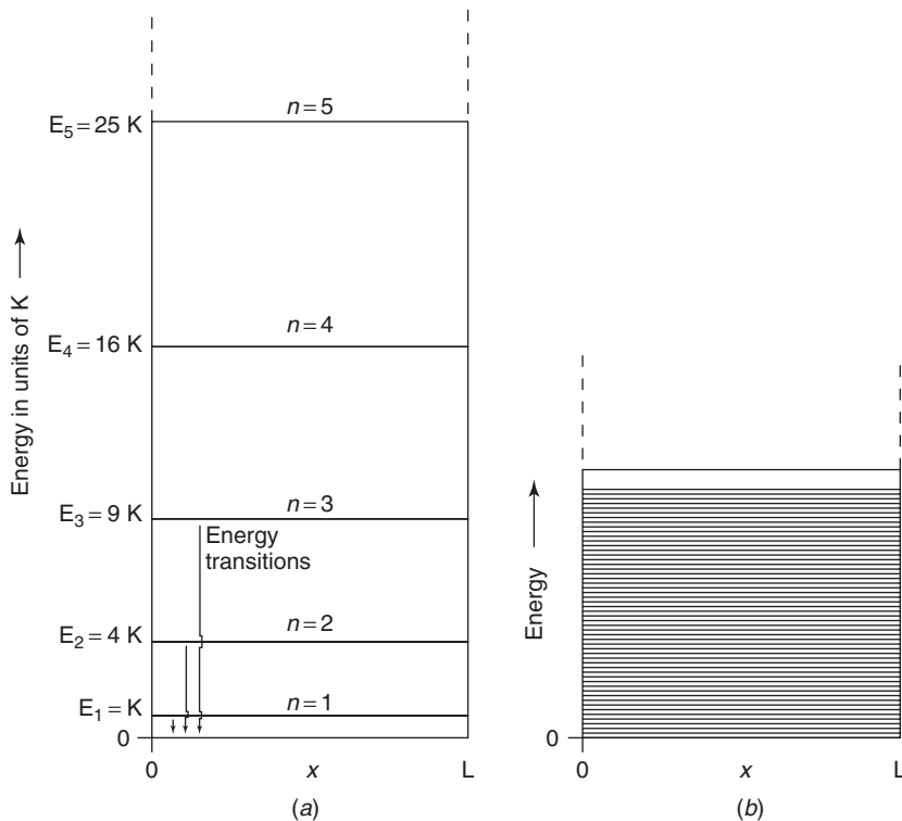
FIGURE D.9 Energy-level graphs for an electron/particle moving in a constrained manner on a line of length L . (a) Quantum behavior (only the first 5 levels are depicted). Note that a line spectrum (emitted energy) is a direct result of the quantization of energy. (b) Classical behavior. The energy can vary in a continuous manner and can assume any value. Diagram shows an “infinite” number of lines with infinitesimally small spacings from one line to the next. Note that a continuum of possible energy values produces a continuous spectrum of frequencies of emitted energy (not shown).
