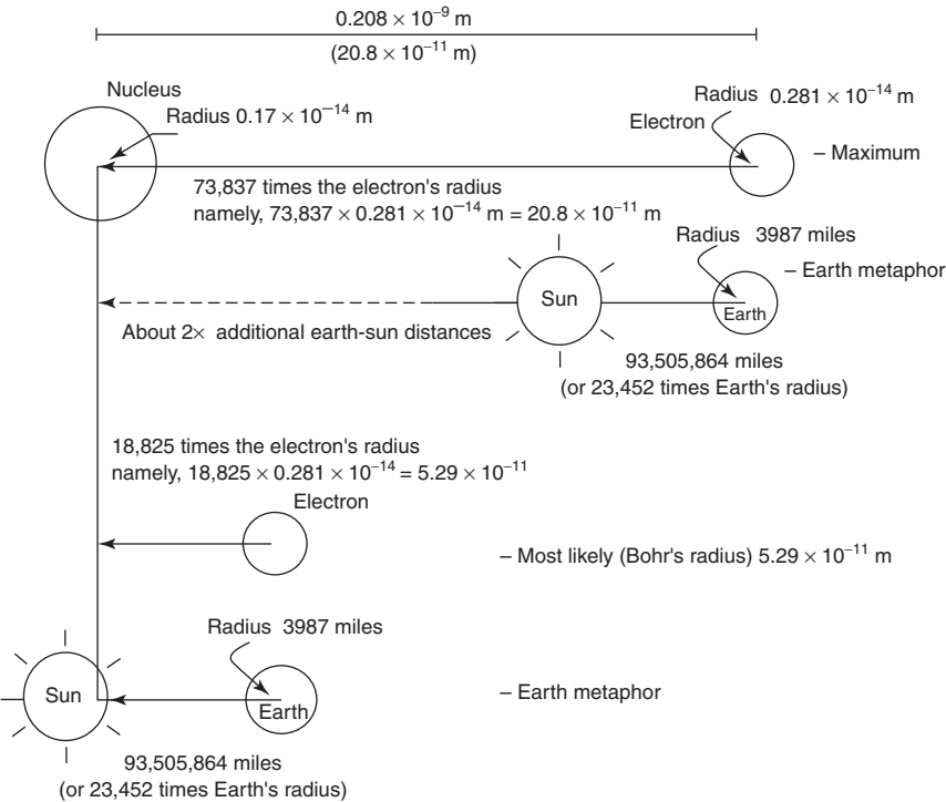
FIGURE 2.4 Some atomic distances and some metaphors.
