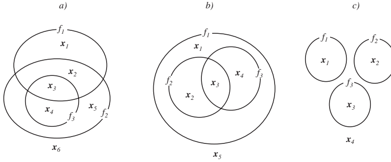
Figure 9.2: Patterns \mathbf{x}_i , represented as d -tuples of binary features f_i , can be placed in Venn diagram (here d = 3 ); the diagram itself depends upon the classification problem and its constraints. For instance, suppose f_1 is the binary feature attribute has_legs , f_2 is has_right_arm and f_3 the attribute has_right_hand . Thus in part a) pattern \mathbf{x}_1 denotes a person who has legs but neither arm nor hand; \mathbf{x}_2 a person who has legs and an arm, but no hand; and so on. Notice that the Venn diagram expresses the biological constraints associated with real people: it is impossible for someone to have a right hand but no right arm. Part c) expresses different constraints, such as the biological constraint of mutually exclusive eye colors. Thus attributes f_1 , f_2 and f_3 might denote brown , green and blue respectively and a pattern \mathbf{x}_i describes a real person, whom we can assume cannot have eyes that differ in color.
