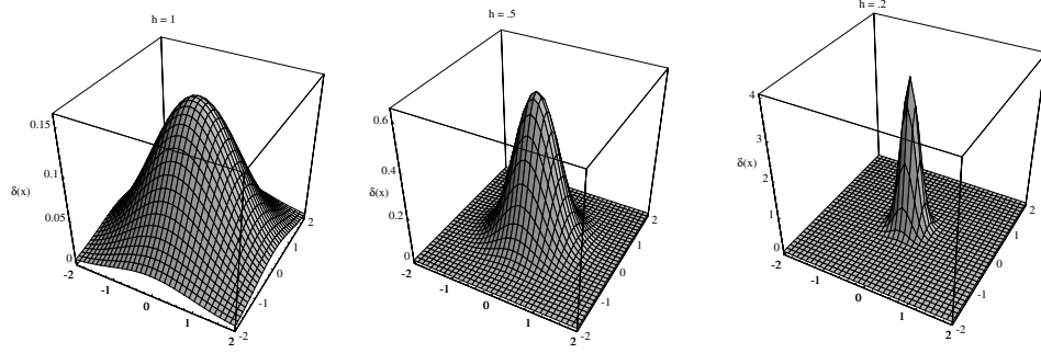
Figure 4.3: Examples of two-dimensional circularly symmetric normal Parzen windows \varphi(\mathbf{x}/h) for three different values of h . Note that because the \delta_k(\cdot) are normalized, different vertical scales must be used to show their structure.
