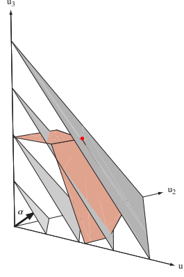
Figure 5.18: Surfaces of constant z = \mathbf{a}^t \mathbf{u} are shown in gray, while constraints of the form \mathbf{A} \mathbf{u} \cdot \boldsymbol{\beta} are shown in red. The simplex algorithm finds an extremum of z given the constraints, i.e., where the gray plane intersects the red at a single point.
