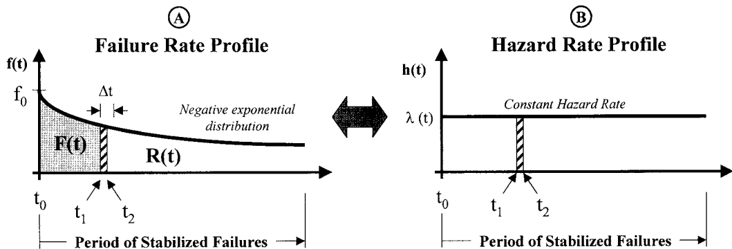
Figure 50.5 Contrasting Failure Density Profile and Hazard Rate Profile
