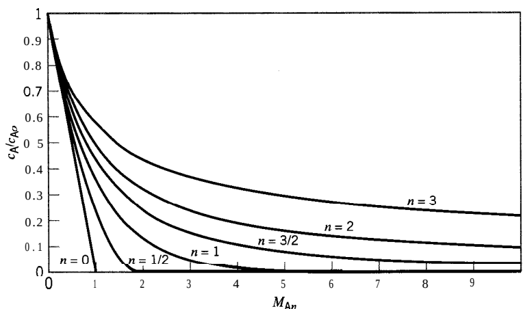
Figure 4.3 Comparison of c_A/c_{A0} for various orders of reaction in a BR or PFR (for conditions, see footnote to Table 4.1)
