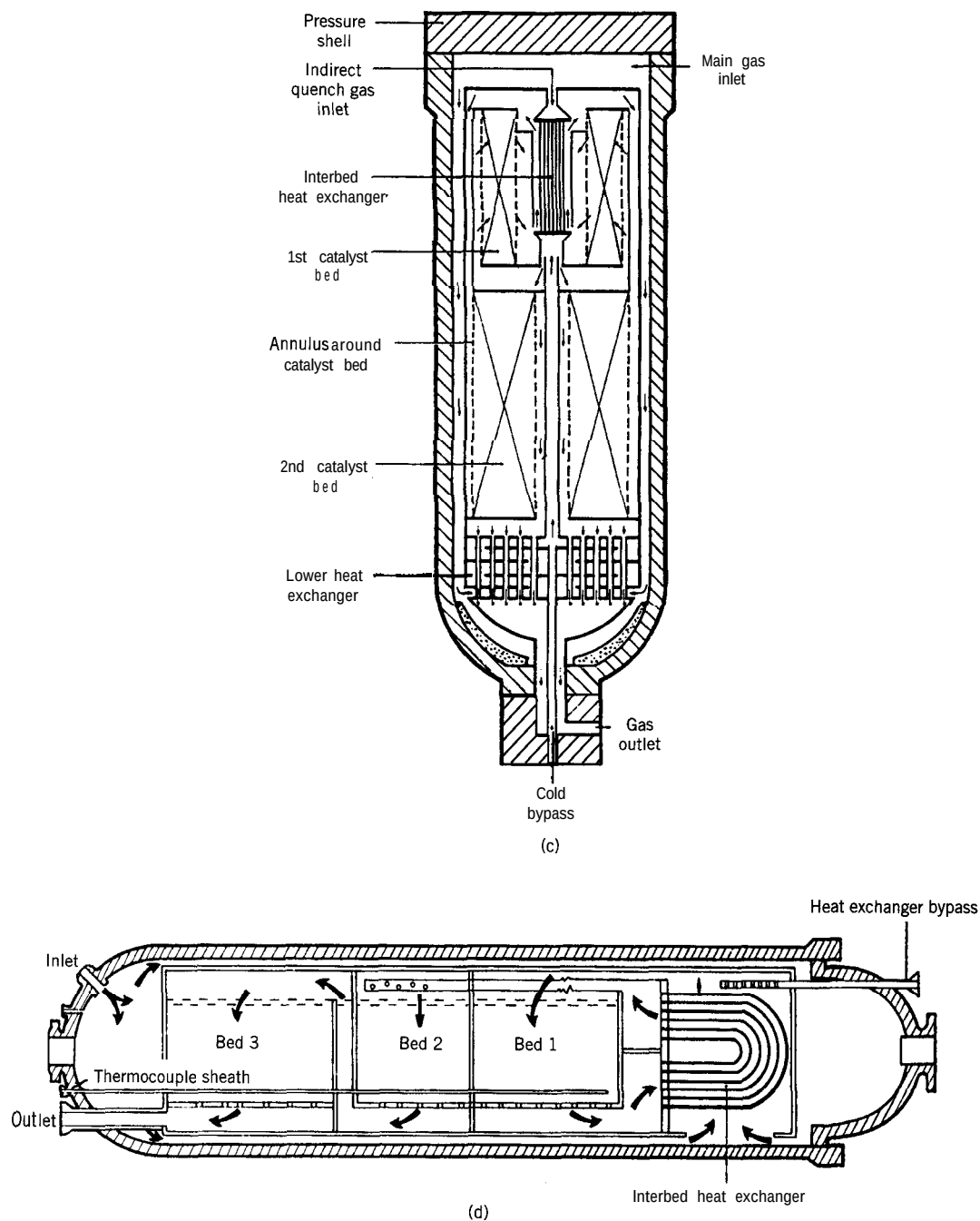
Figure 11.5 (cont'd) (c) Topsøe S 200 converter combines two radial-flow beds with interstage cooling by heat exchange; (d) Kellogg horizontal converter with cross-flow and interstage heat exchange (Twigg, 1996, pp. 437,432; reproduced with permission from Catalyst Handbook, ed. M.V. Twigg, Manson Publishing Company, London, 1996)
