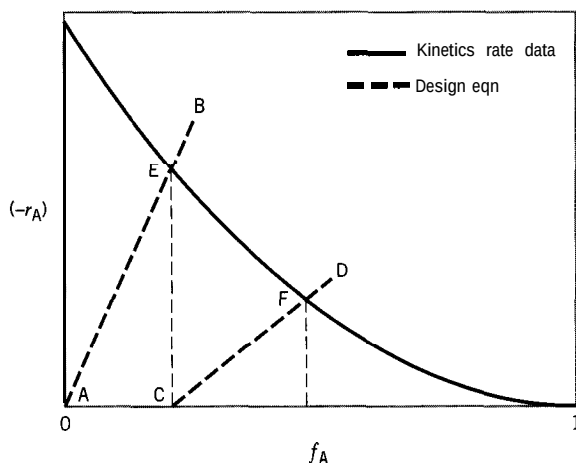
Figure 14.11 Basis for graphical solution for multistage CSTR (for A \rightarrow \dots \rightarrow \text{products} )
