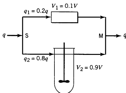
Figure 17.9 Vessel configuration for Problem 17-16
