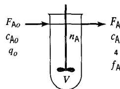
Figure 14.1 Quantities in material-balance equation for CSTR
