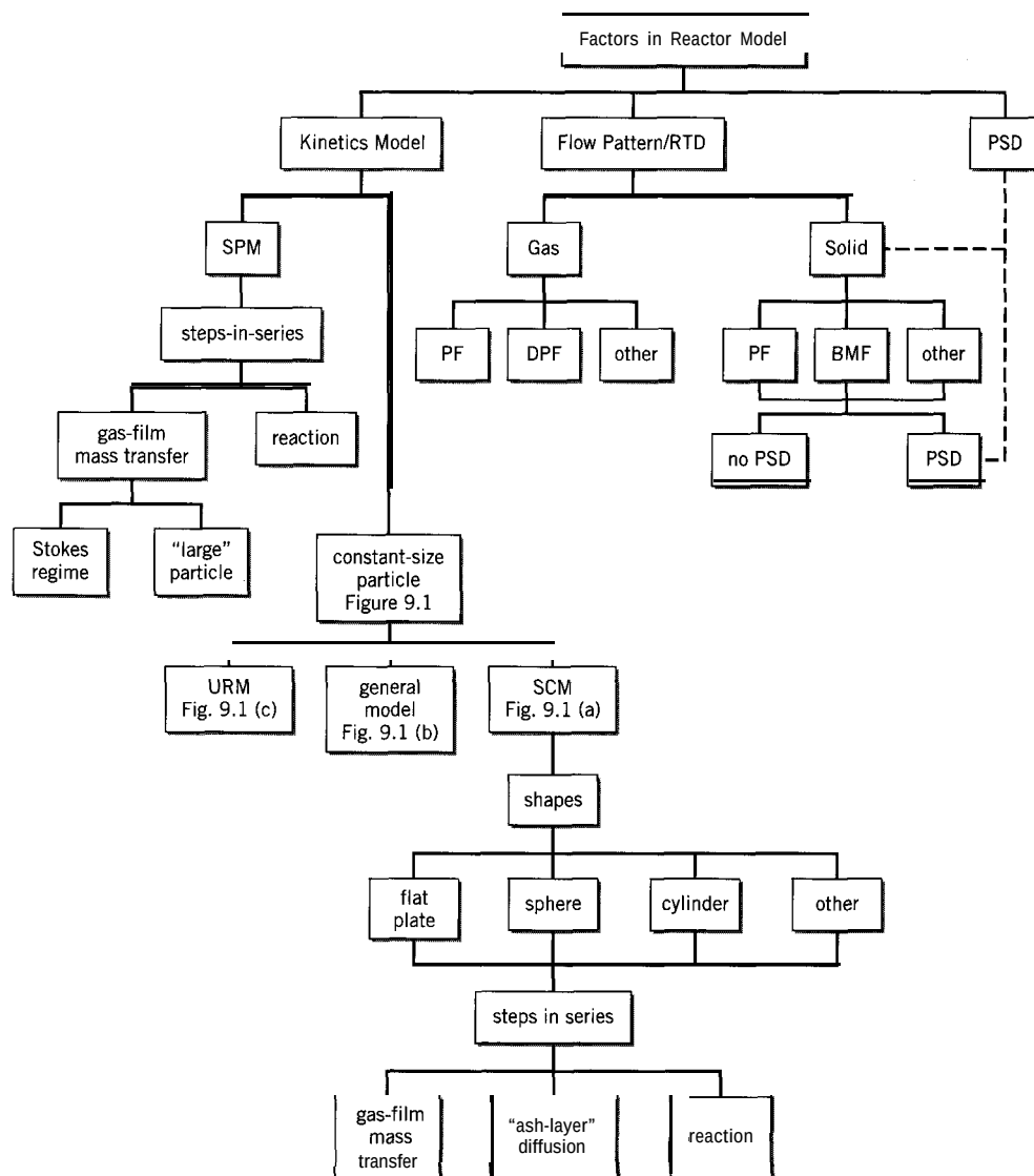
Figure 22.1 Factors affecting reactor performance for a fluid (A) + solid (B) reaction, A + bB \rightarrow products
