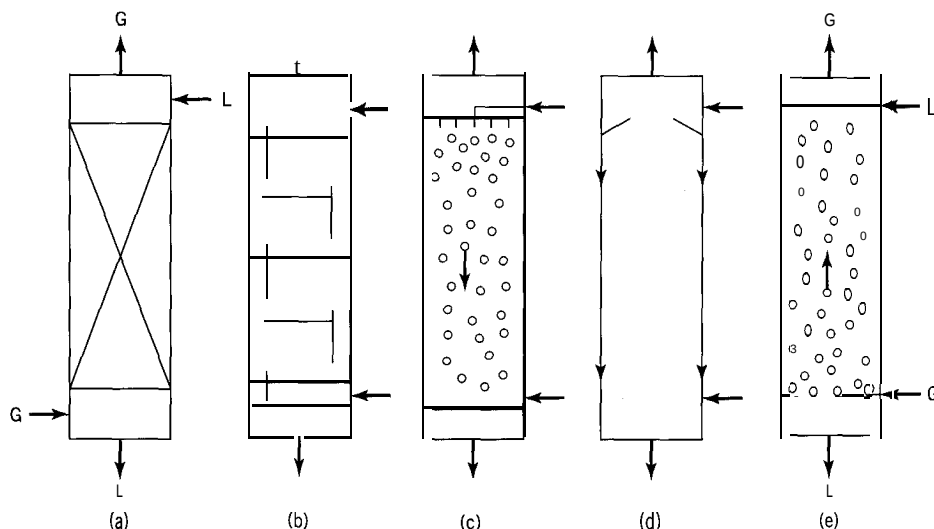
Figure 24.1 Types of tower or column reactors for gas-liquid reactions: (a) packed tower; (b) plate tower; (c) spray tower; (d) falling-film tower; (e) bubble column
