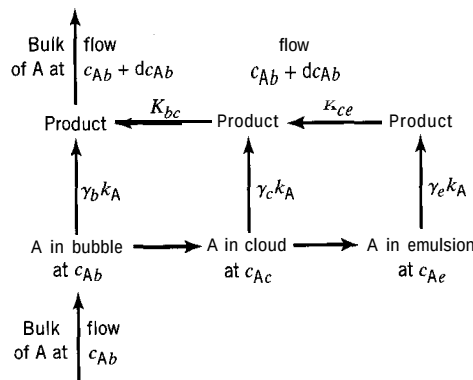
Figure 23.8 Flow/kinetics scheme for bubbling-bed reactor model for reaction A(g) + \cdot \rightarrow \text{product(s)}
