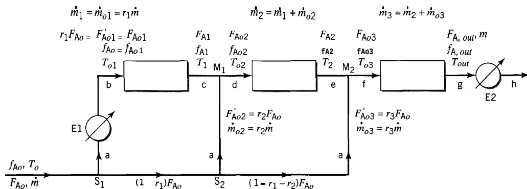
Figure 21.11 Flow diagram and notation for three-stage FBCR with cold-shot cooling
