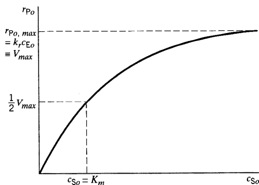
Figure 10.1 Initial-rate plot for S + E \rightarrow P + E showing interpretation of r_{Po, max} in terms of rate Parameters; constant c_{Eo} , T , pH
