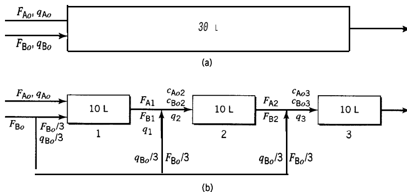
Figure 18.4 Vessel configuration for parallel reactions in Example 18-6: (a) single PFR; (b) three PFRs of same total volume in series with F_{Bo} split evenly among them
