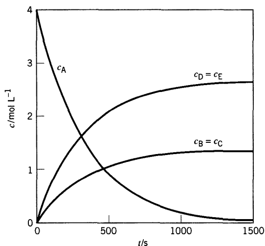
Figure 5.3 Concentration profiles for parallel reaction network in Example 5-6
