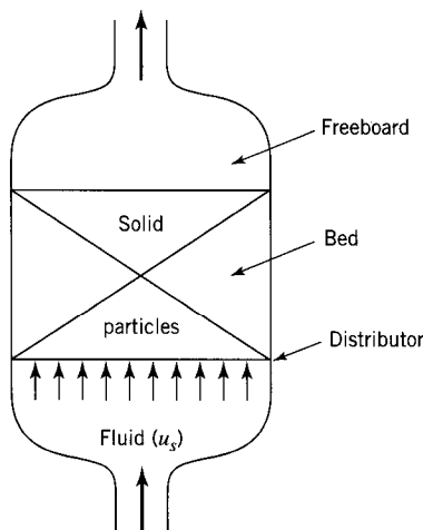
Figure 23.1 Schematic representation of (incipient) particle movement brought about by upward flow of a fluid, leading to fluidization
