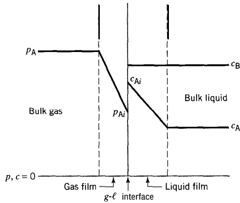
Figure 9.5 Two-film model (profiles) for relatively slow reaction A(g) + bB(l) \rightarrow \text{products} (nonvolatile B)
