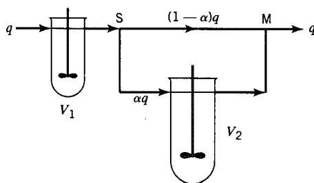
Figure 17.8 Vessel configuration for Problem 17-15
