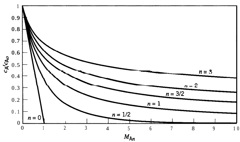
Figure 4.4 Comparison of c_A/c_{A0} for various orders of reaction in a CSTR (for conditions, see footnote to Table 4.1)
