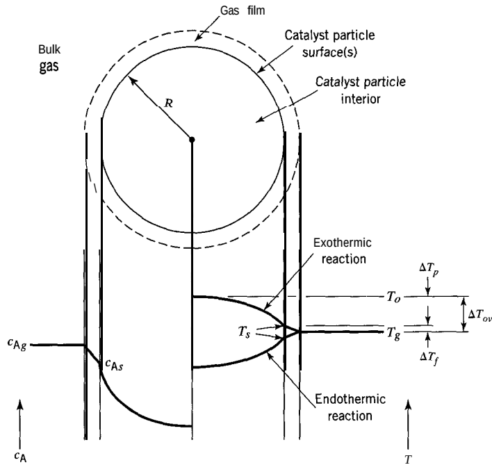
Figure 8.9 Concentration ( c_A ) and temperature ( T ) gradients (schematic) in a porous catalyst particle (spherical or end-on cylindrical)
