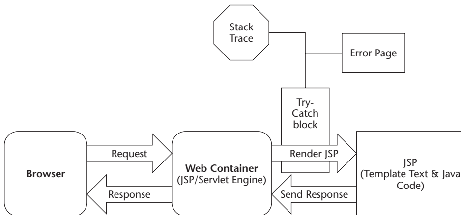
Figure 4.1 Rendering a JSP.
