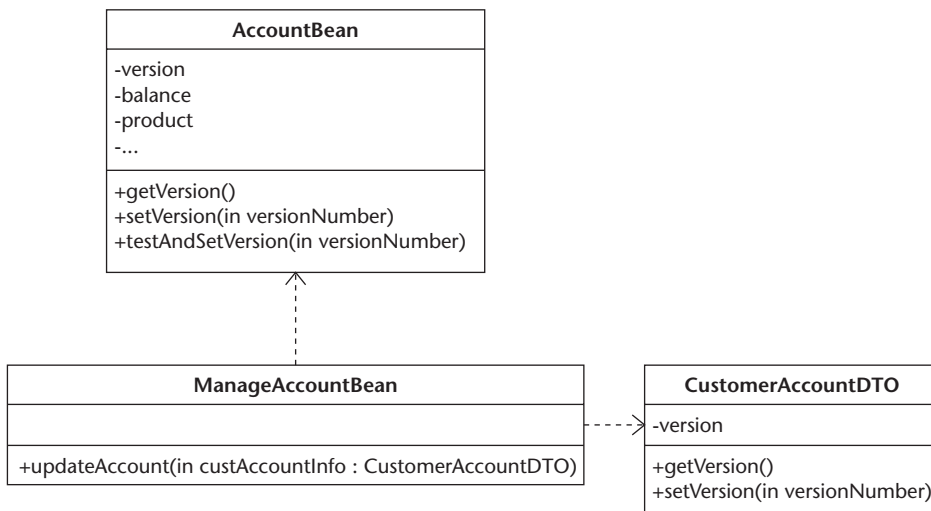
Figure 2.7 After refactoring.
