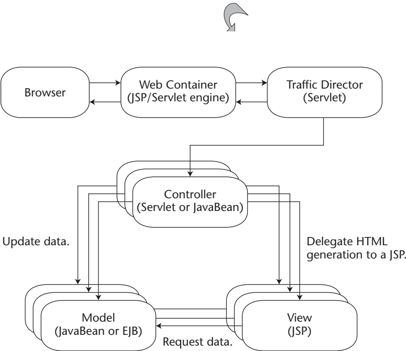
Figure 5.7 After refactoring.
