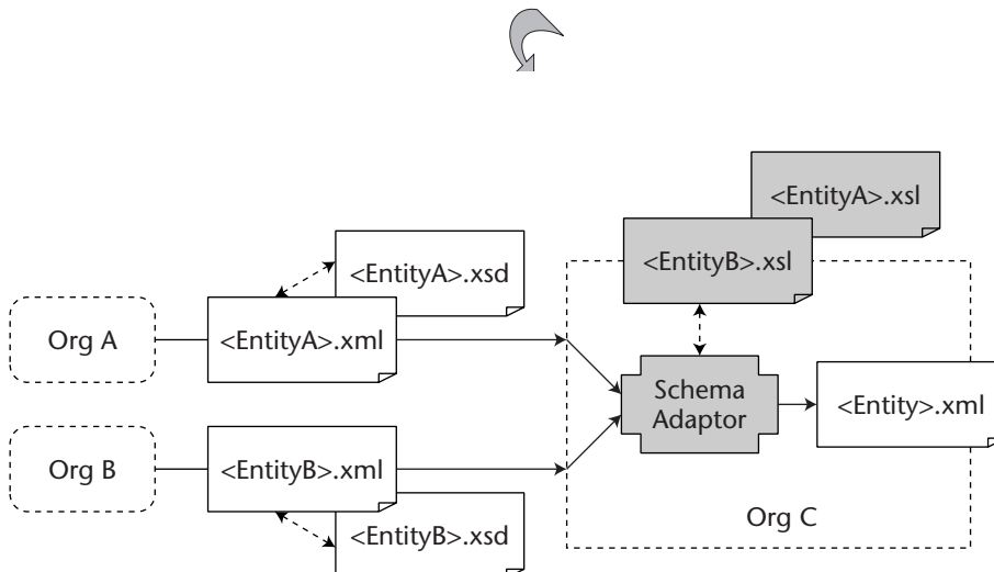
Figure 9.8 After refactoring.
