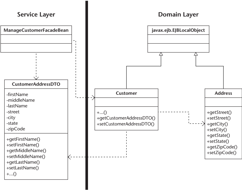
Figure 6.13 Before refactoring.
