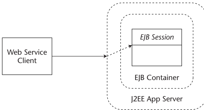
Figure 9.10 Before refactoring.
