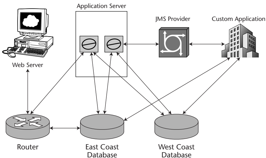
Figure 1.14 Partitioning data.
