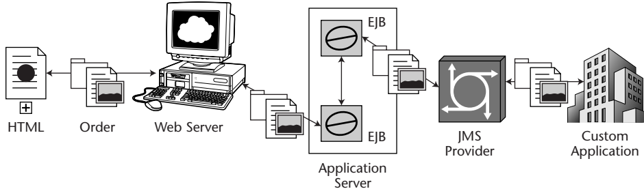
Figure 1.8 Big orders in the system.
