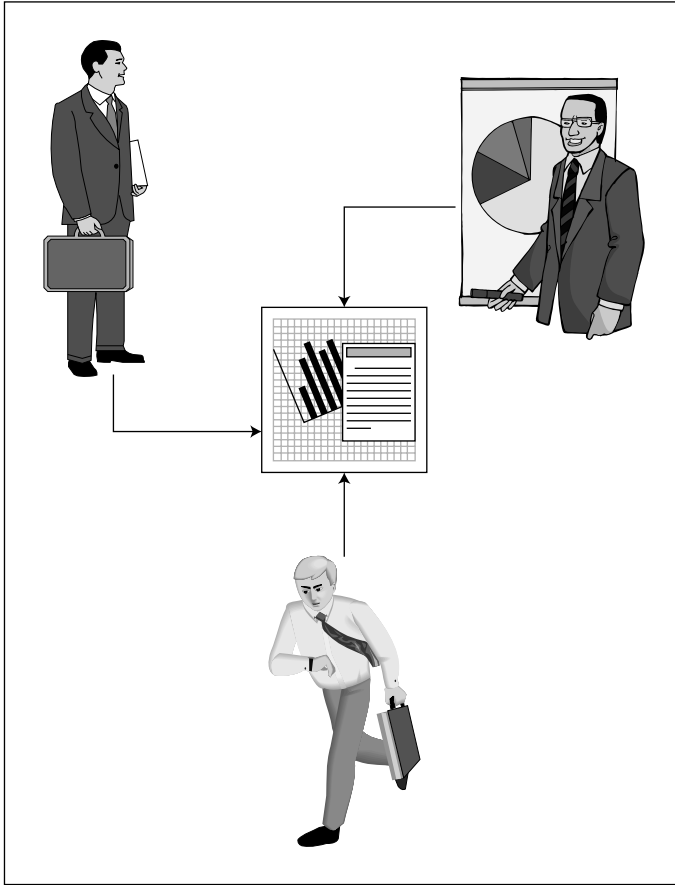
Figure 1.16 After refactoring.
