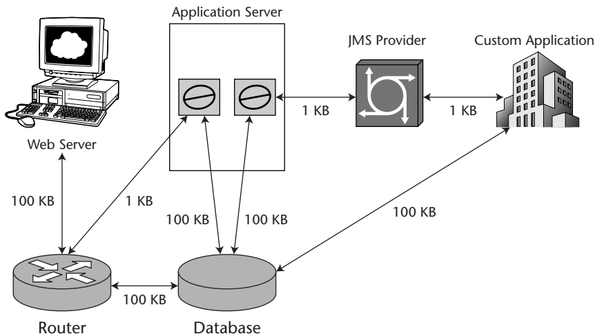
Figure 1.11 Hubs with bandwidth data—database hub.
