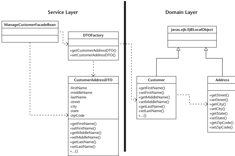
Figure 6.14 After refactoring.
