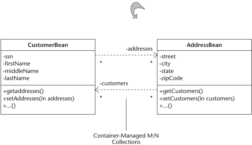
Figure 2.9 After refactoring.
