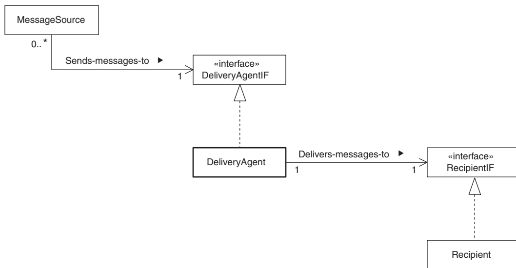
FIGURE 6.9 Retransmission pattern.
