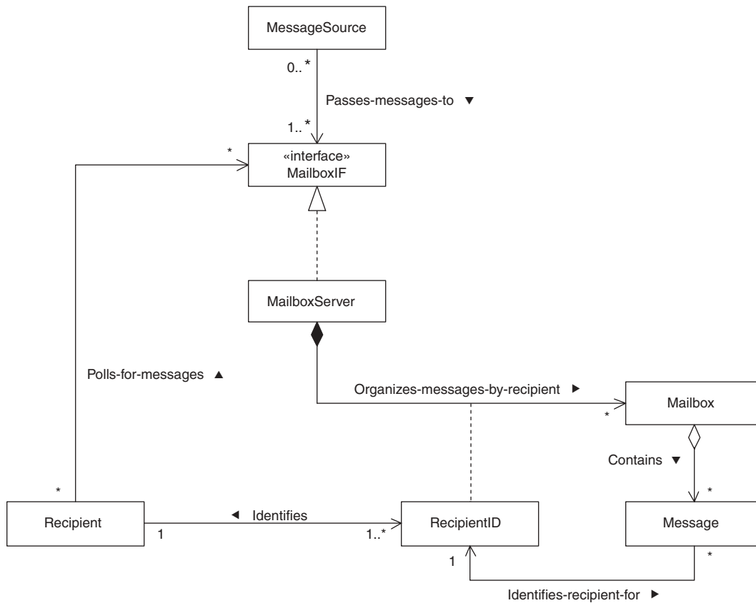
FIGURE 6.11 Mailbox pattern.
