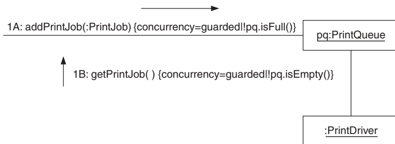
FIGURE 2.29 Print queue.
