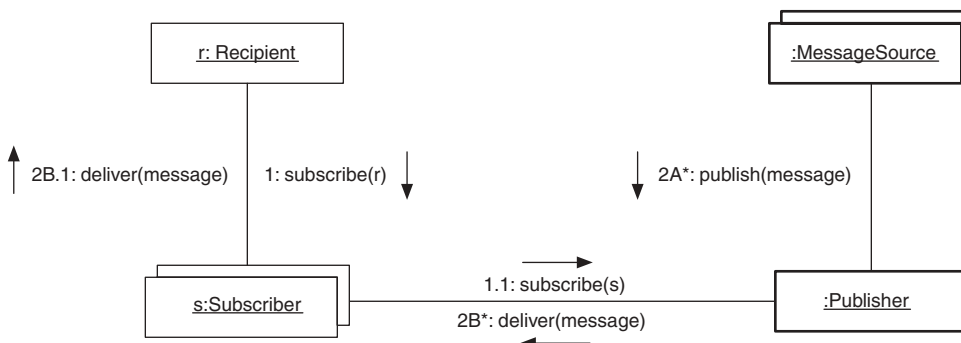
FIGURE 6.8 Publish-Subscribe collaboration.
