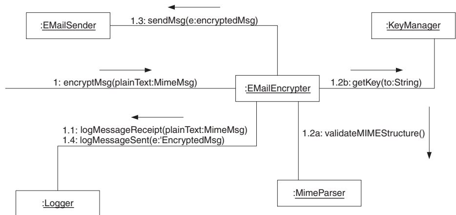
FIGURE 2.24 E-mail encrypter.
