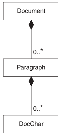
FIGURE 2.12 Composite aggregation.
