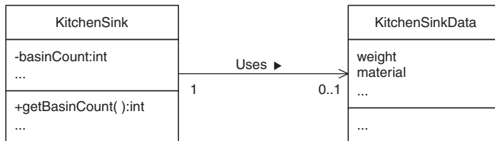
FIGURE 6.12 Class organization.
