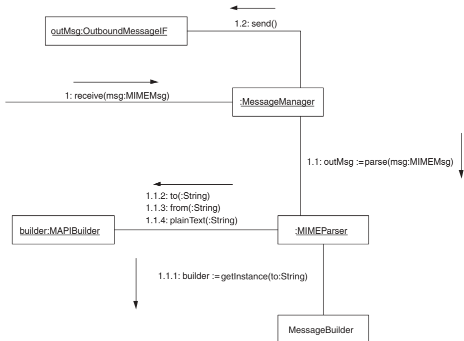
FIGURE 2.21 Collaboration diagram.
