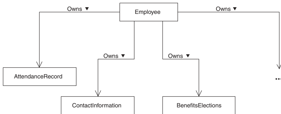
FIGURE 9.13 HRMS design.
