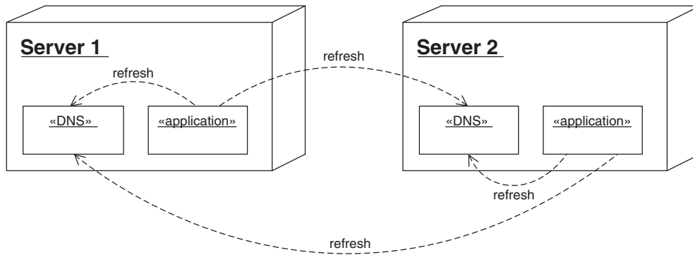
FIGURE 2.35 Deployment diagram.
