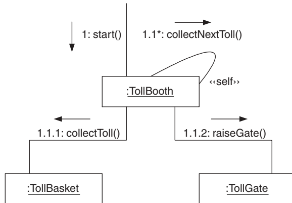
FIGURE 2.25 Tollbooth.
