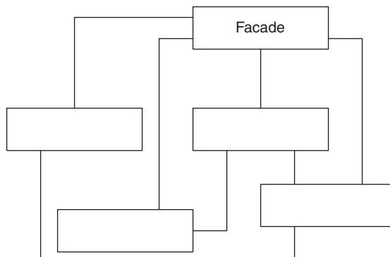
FIGURE 2.19 Blank objects.
