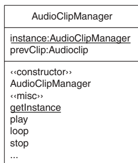
FIGURE 2.3 Simplified class.
