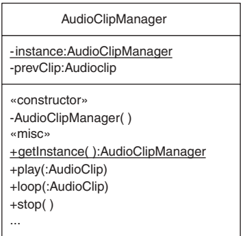
FIGURE 2.1 Basic class.
