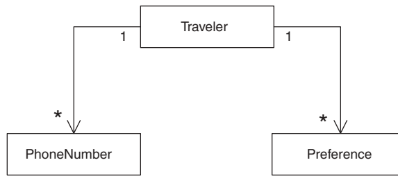
FIGURE 9.12 Complex object.
