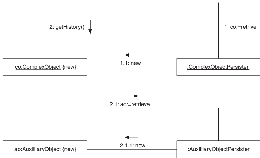
FIGURE 9.14 Lazy Retrieval pattern.
